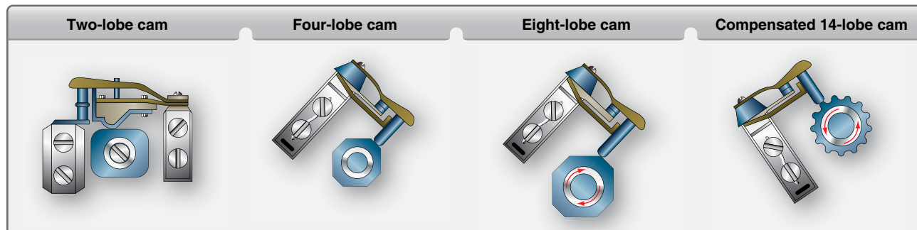
Figure 4-9. Typical breaker assemblies.
