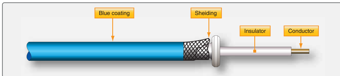
Figure 4-12. Ignition lead.
