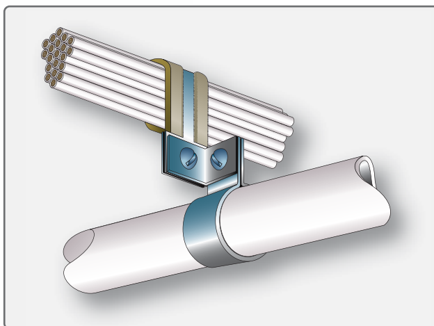
Figure 4-91. Separation of wires from plumbing lines.
