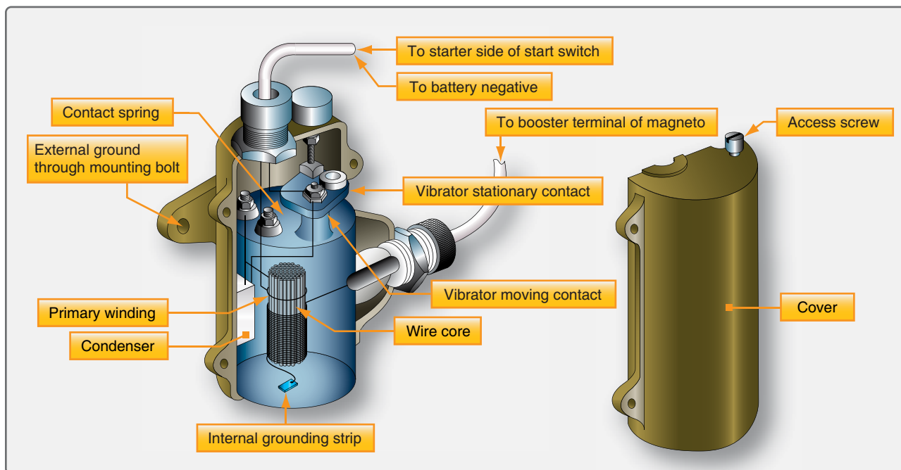
Figure 4-25. Booster coil.
