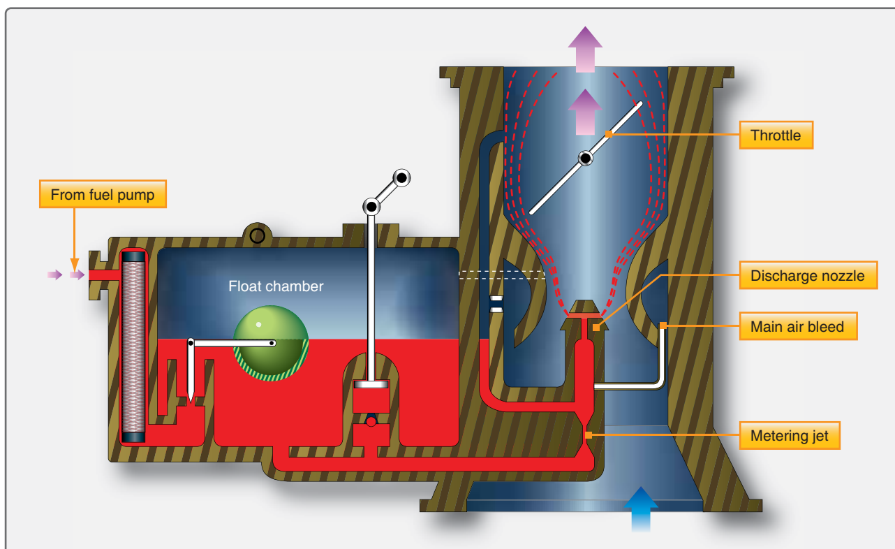
Figure 2-10. A float-type carburetor.
