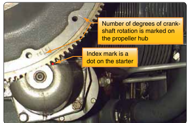
Figure 4-37. Lycoming timing marks.
