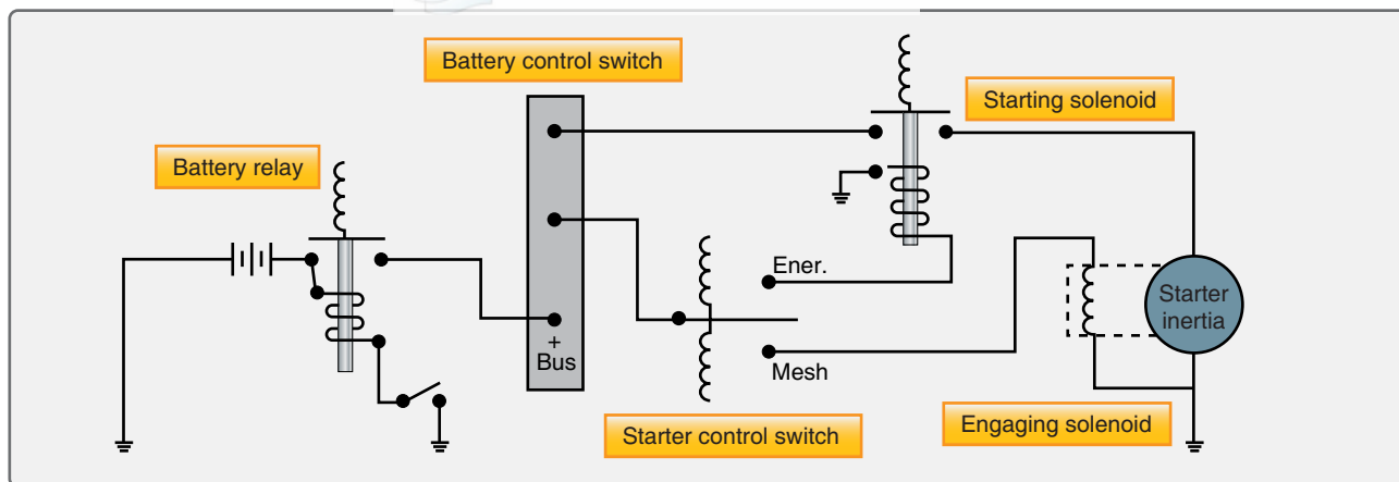
Figure 5-2. Electric inertia starting circuit.
