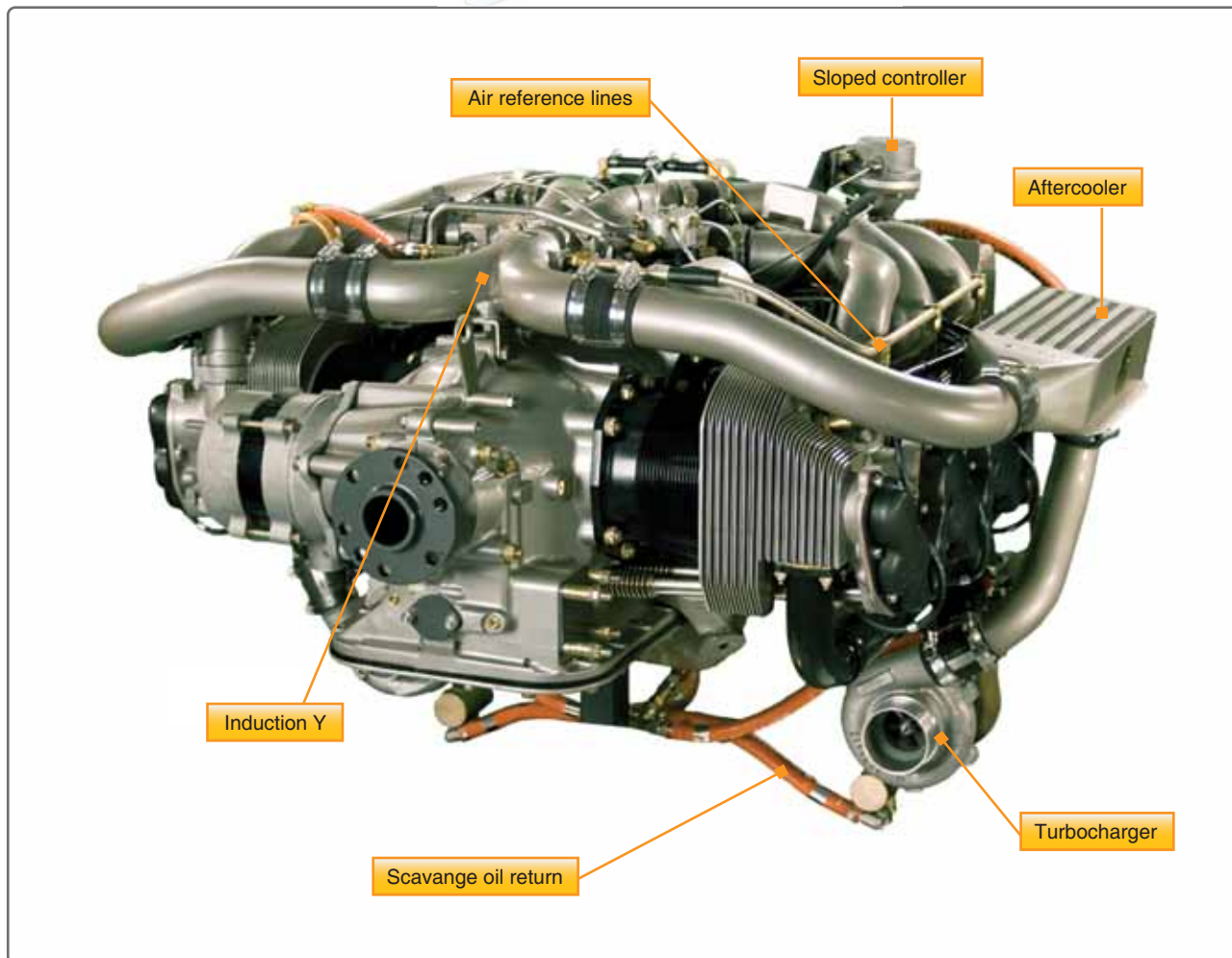
Figure 3-20. An aftercooler installation.
