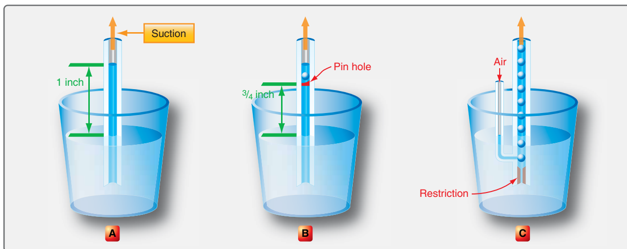
Figure 2-13. Air bleed principle.
