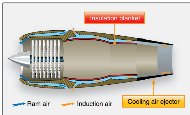
Figure 1-73. Exhaust system insulation blanket.
