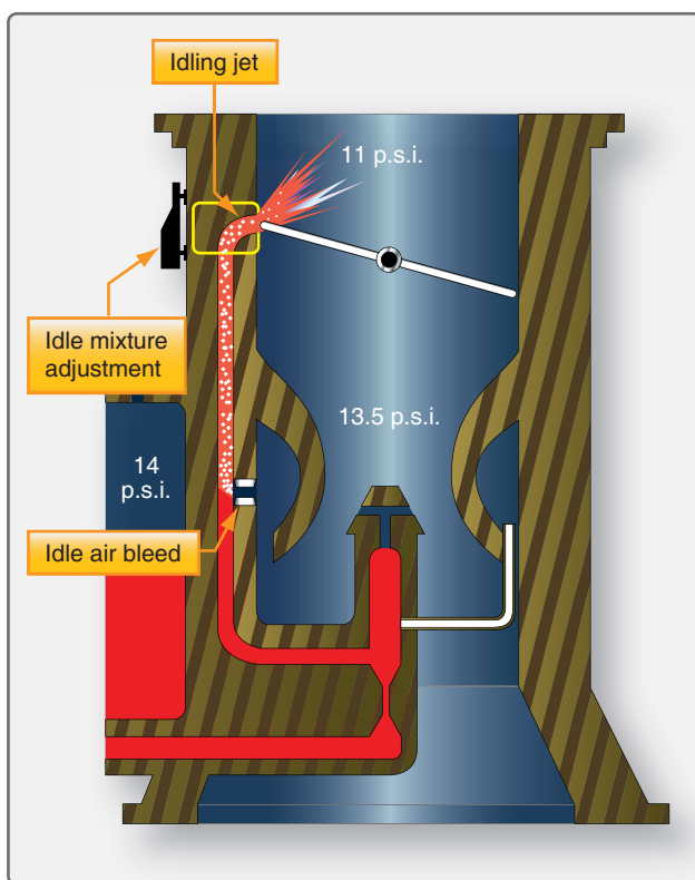
Figure 2-15. Idling system.
