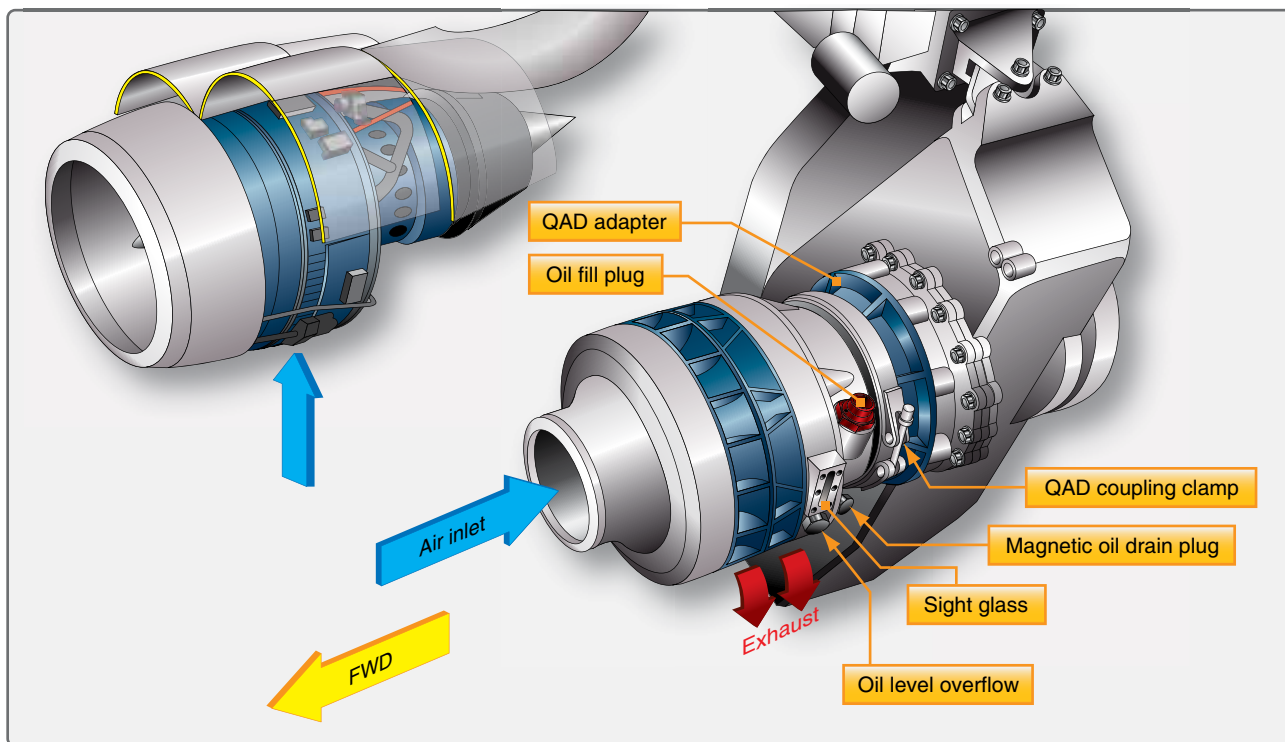
Figure 5-22. Air turbine starter.
