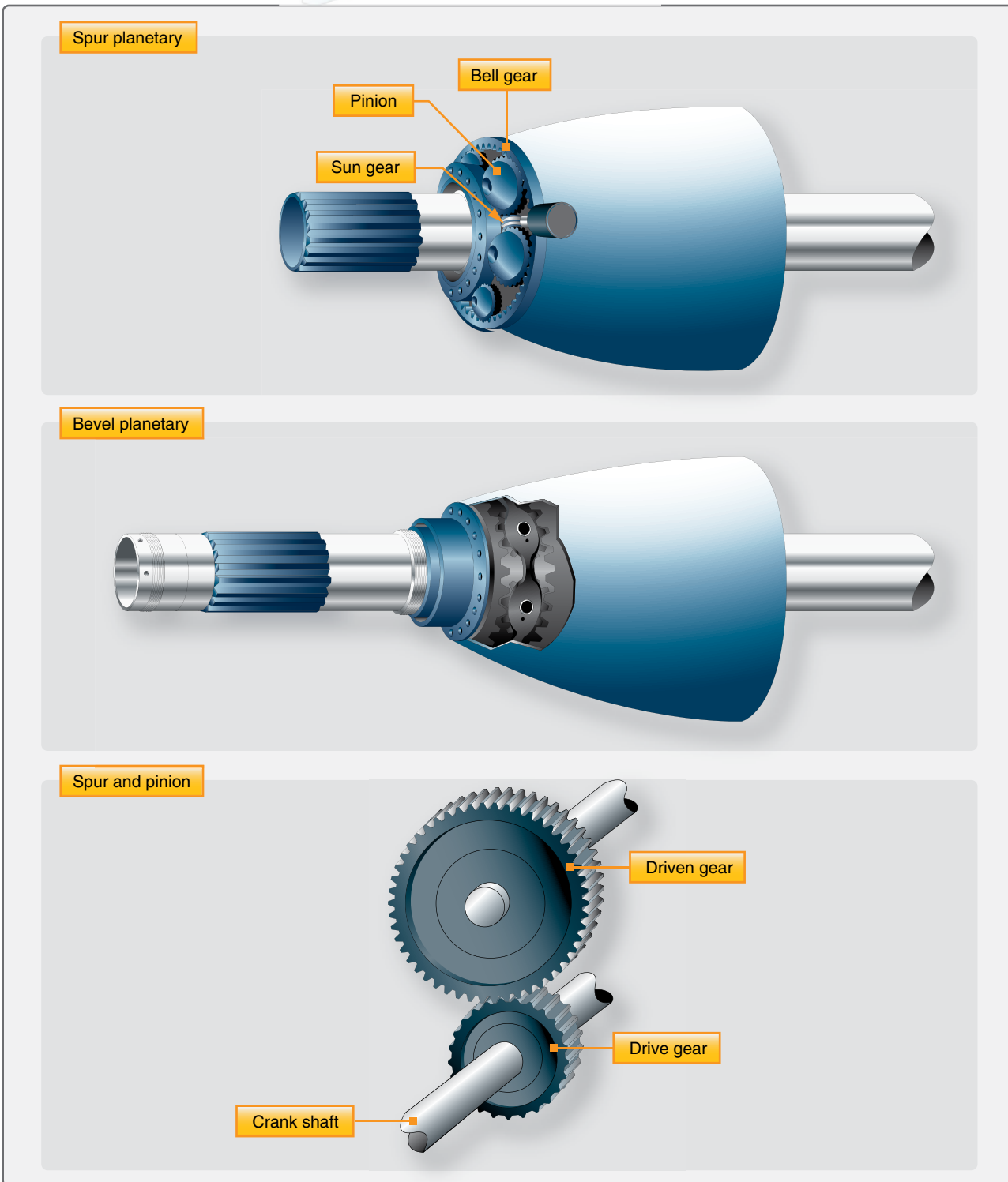
Figure 1-34. Reduction gears.
