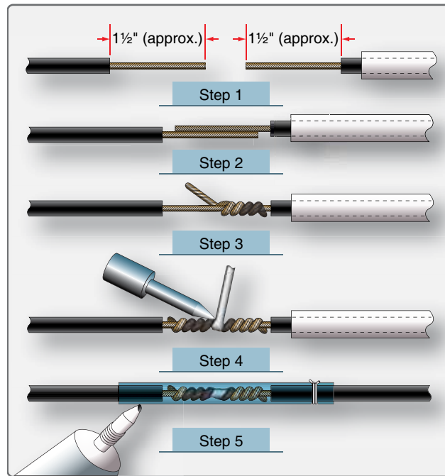
Figure 4-108. Repairing broken wire by soldering and potting.
