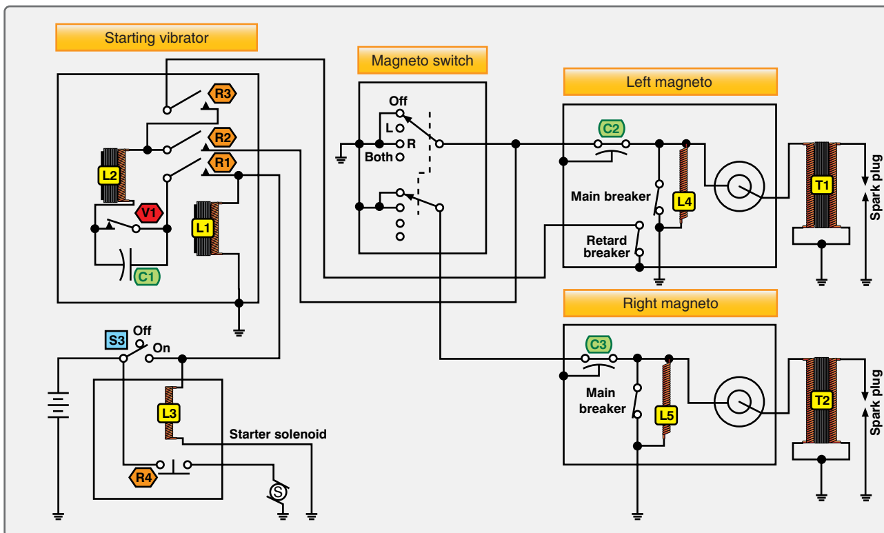
Figure 4-20. Simplified low-tension ignition system schematic.
