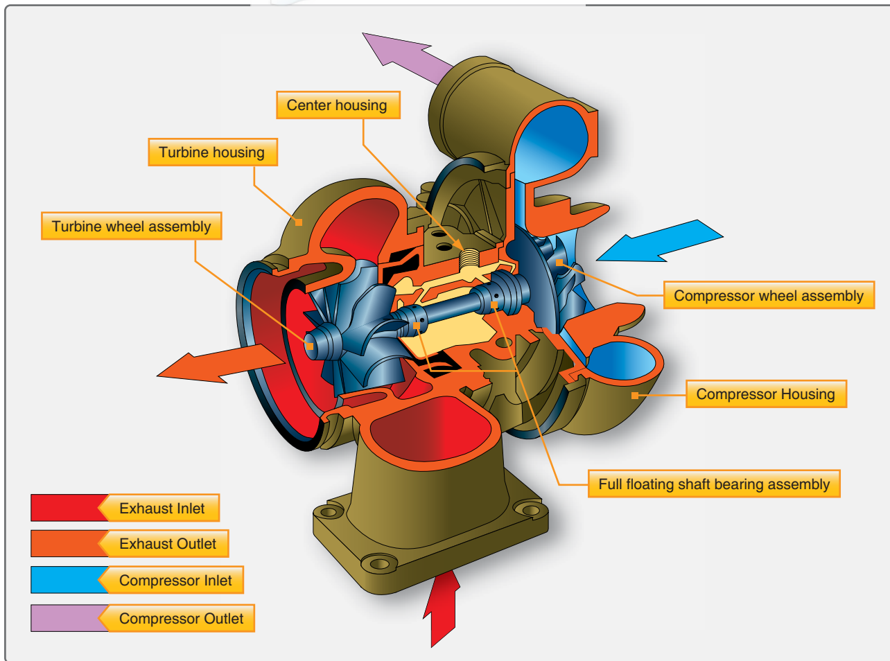
Figure 3-12. A typical turbosupercharger and its main parts.
