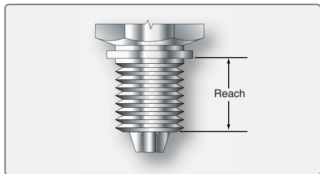
Figure 4-36. Spark plug reach.
