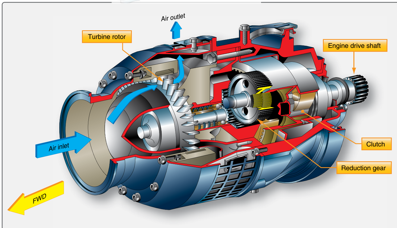
Figure 5-21. Cutaway view of an air turbine starter.
