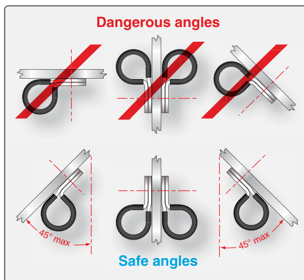
Figure 4-92. Proper mounting angle for cable clamps.
