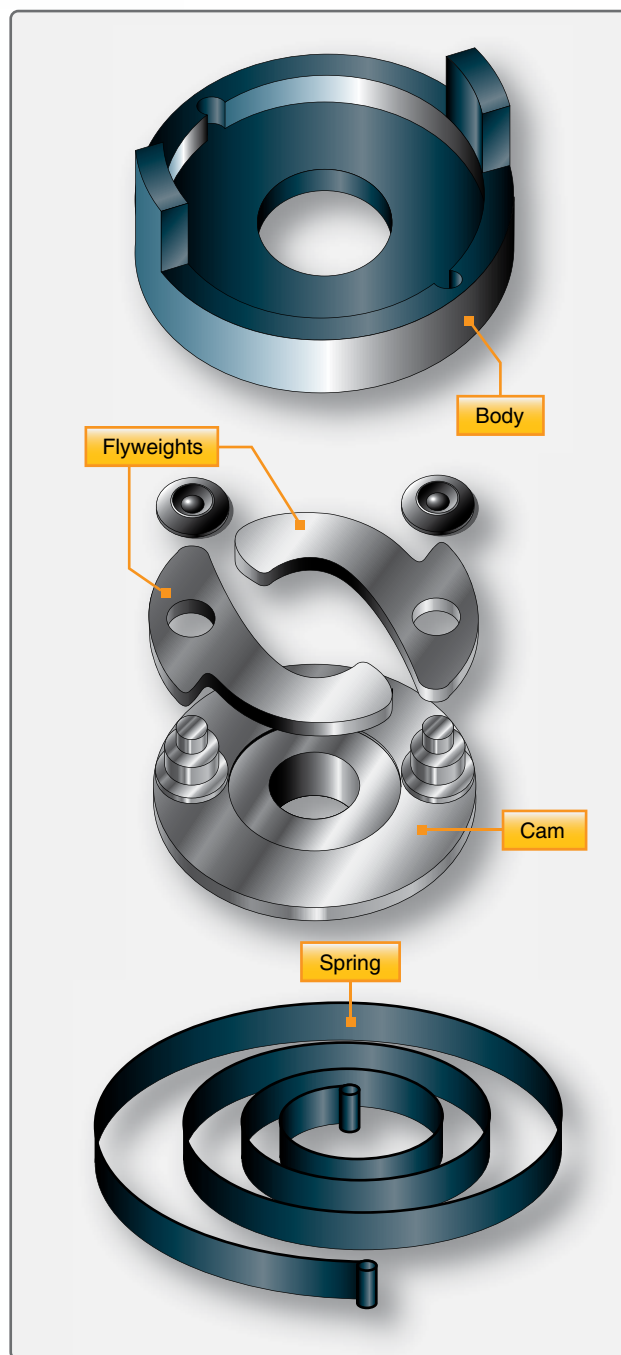
Figure 4-27. Parts of an impulse coupling.
