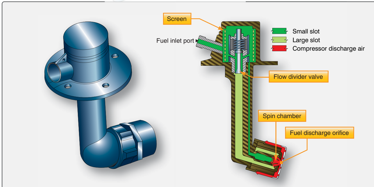
Figure 2-66. Duplex fuel nozzle.
