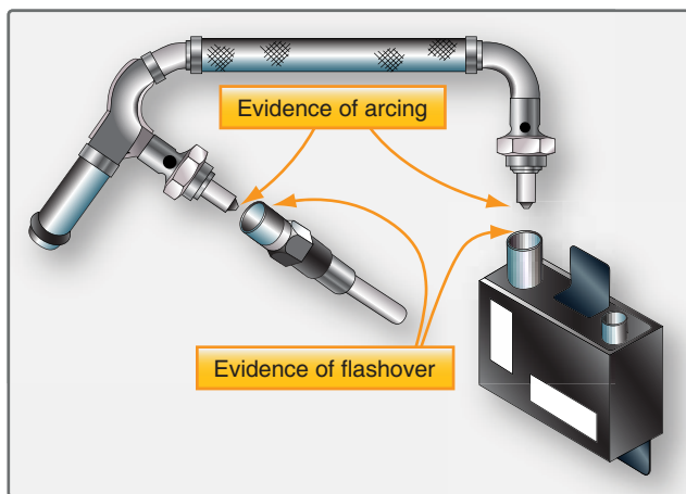
Figure 4-71. Flashover inspection.
