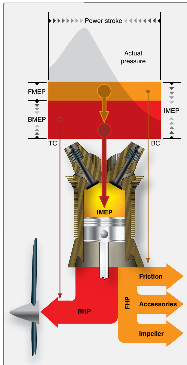
Figure 1-41. Power and pressure.
