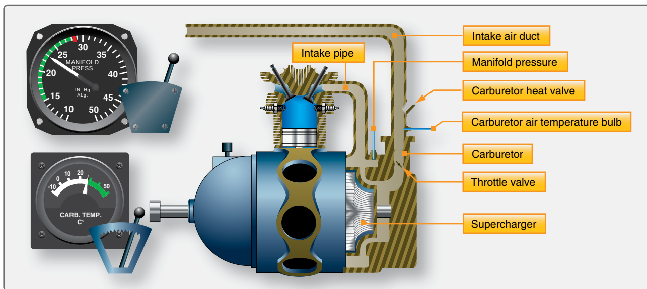
Figure 3-10. Internally driven supercharger induction system.
