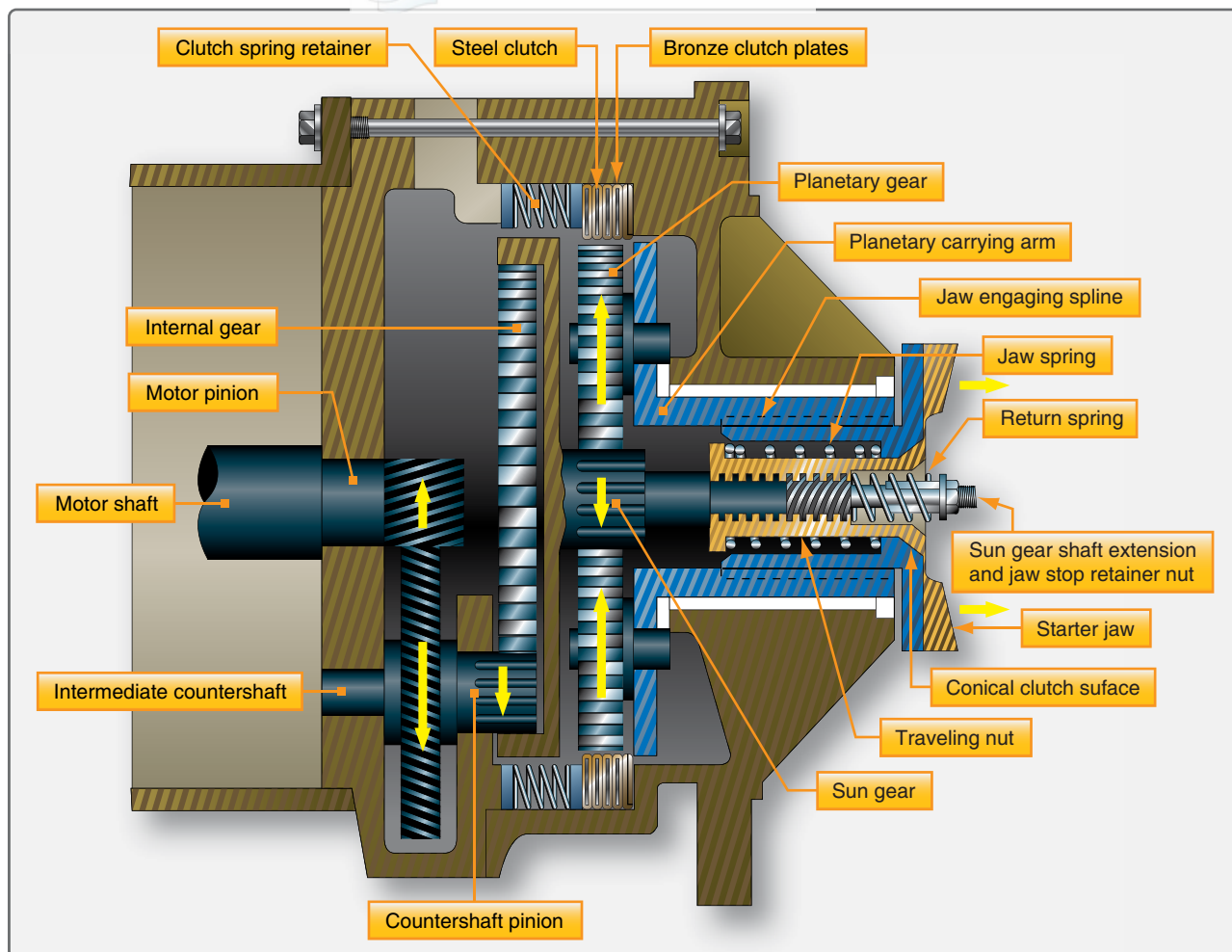
Figure 5-6. Starter gear section.
