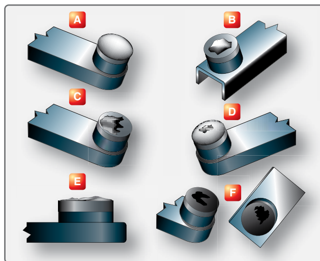
Figure 4-62. Examples of contact surface conditions.
