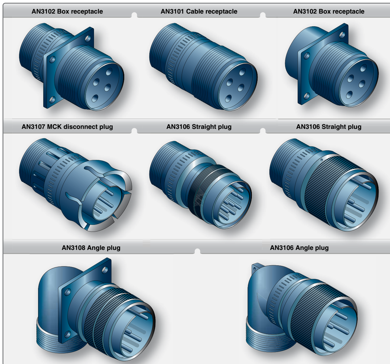
Figure 4-115. AN connectors.
