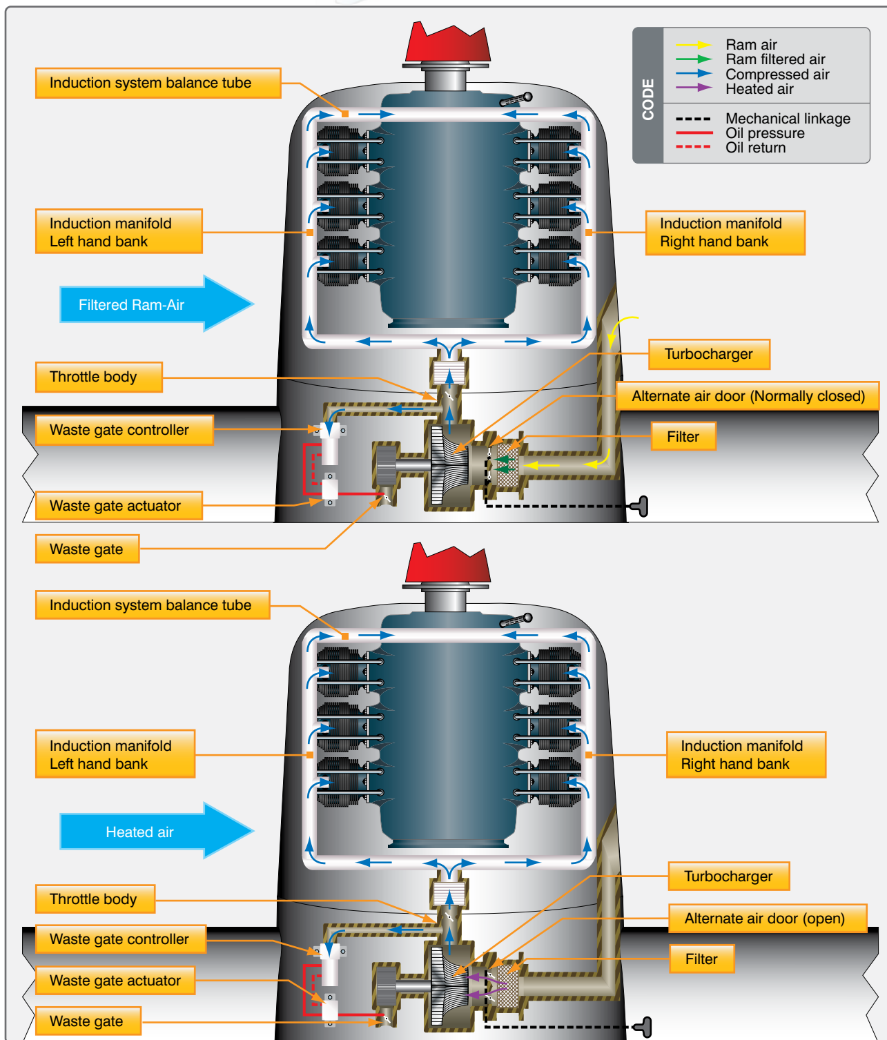
Figure 3-17. A turbocharger air induction system.
