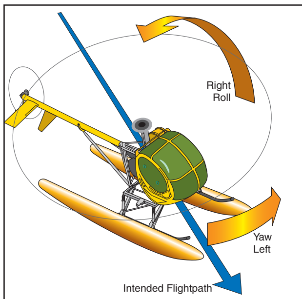
Figure 9-4. Float instability.
