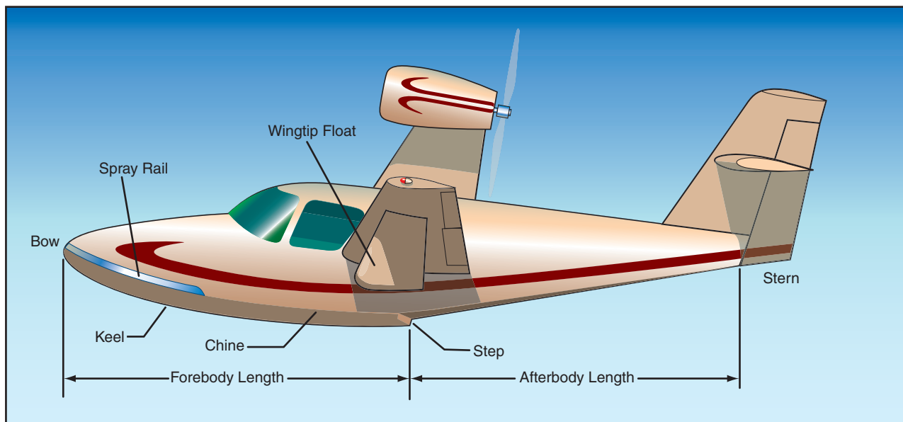
Figure 2-2. Hull components.
