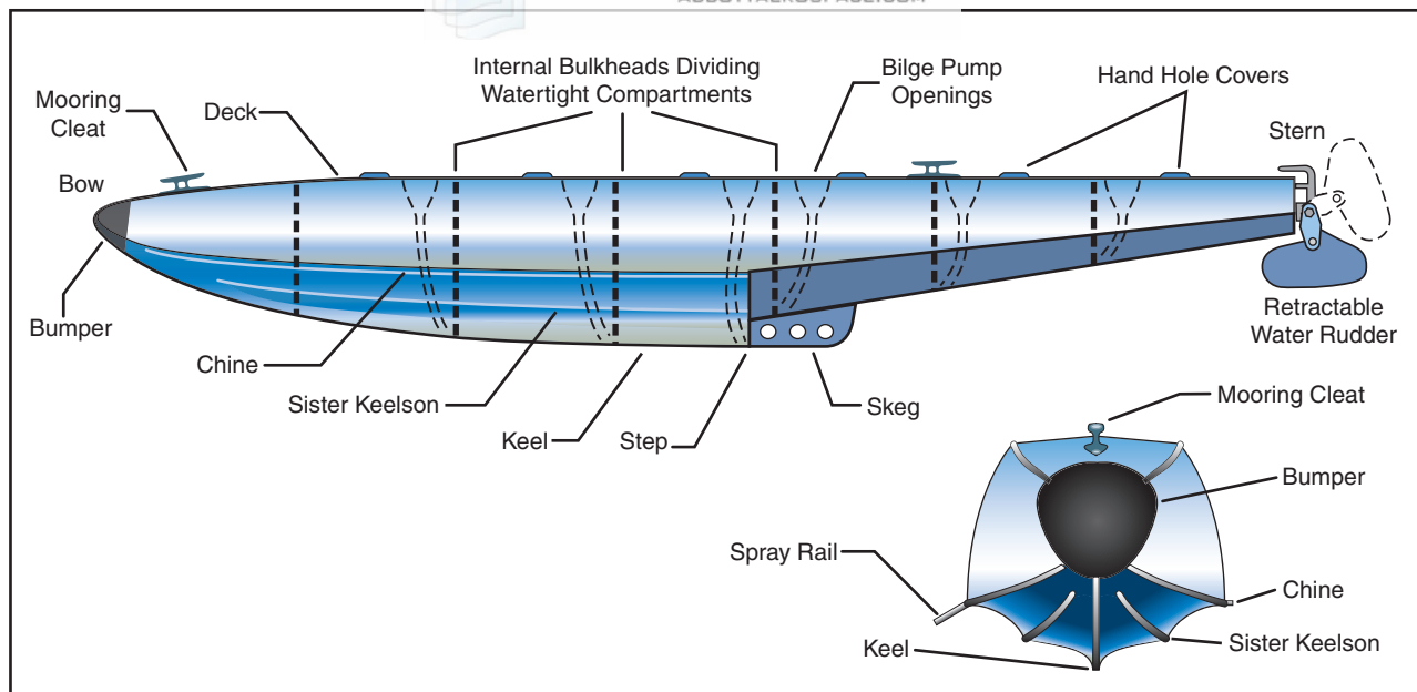
Figure 2-3. Float components.
