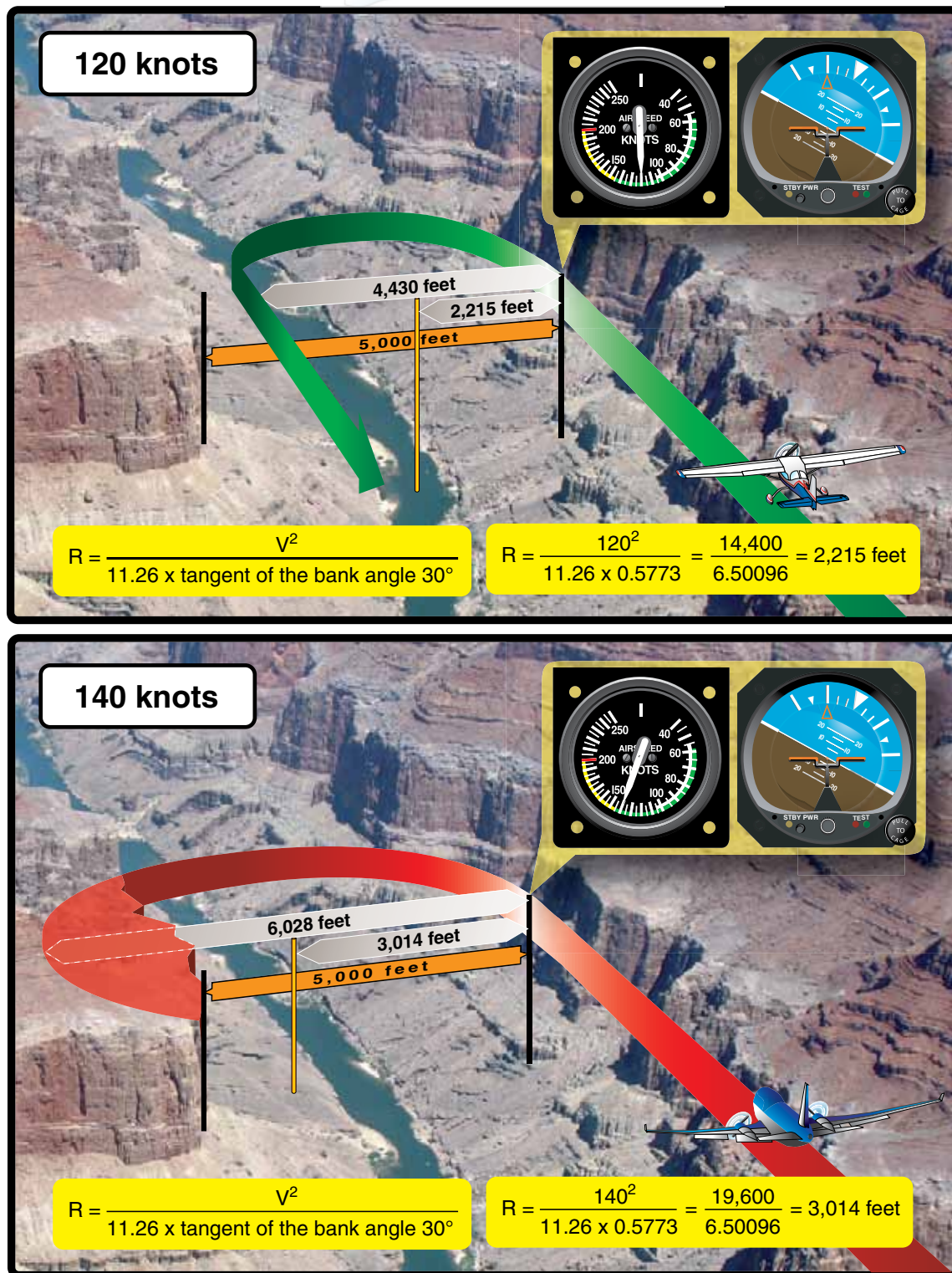
Figure 5-9. Two aircraft have flown into a canyon by error. The canyon is 5,000 feet across and has sheer cliffs on both sides. The pilot in the top image is flying at 120 knots. After realizing the error, the pilot banks hard and uses a 30° bank angle to reverse course. This aircraft requires about 4,000 feet to turn 180°, and makes it out of the canyon safely. The pilot in the bottom image is flying at 140 knots and also uses a 30° angle of bank in an attempt to reverse course. The aircraft, although flying just 20 knots faster than the aircraft in the top image, requires over 6,000 feet to reverse course to safety. Unfortunately, the canyon is only 5,000 feet across and the aircraft will hit the canyon wall. The point is that airspeed is the most influential factor in determining how much distance is required to turn. Many pilots have made the error of increasing the steepness of their bank angle when a simple reduction of speed would have been more appropriate.
