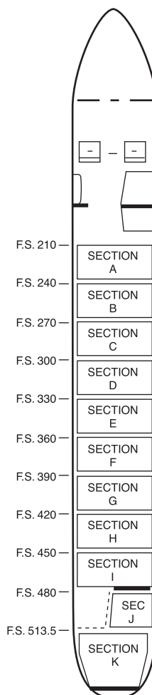
Figure 7-14. Loading data for cargo configuration.
