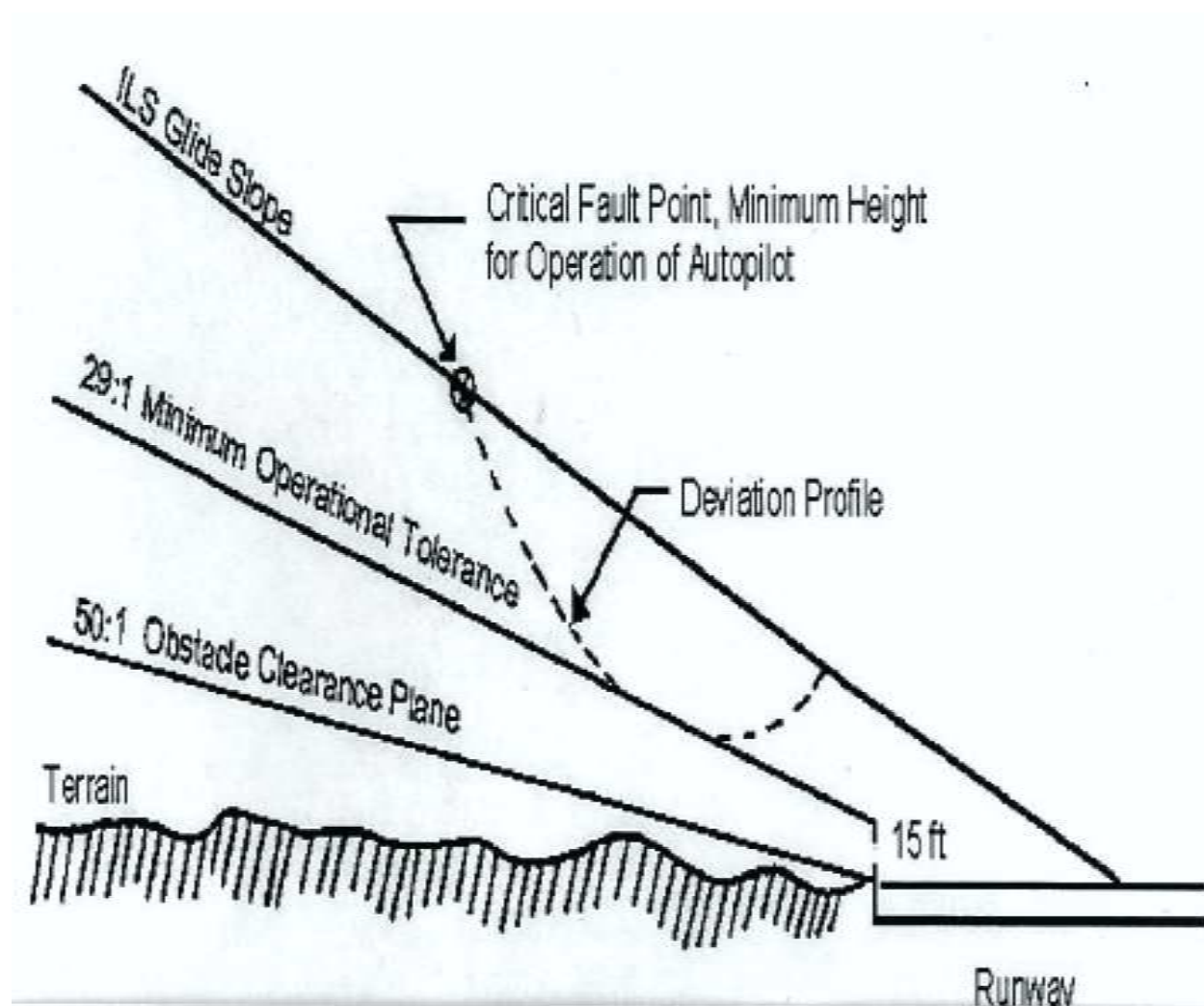
FIGURE AC 27.1329-3 DEVIATION PROFILE
