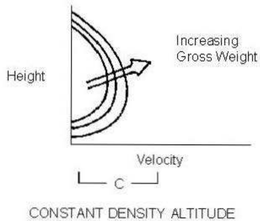
FIGURE AC 27.79-2 ALTITUDE/WEIGHT ACCOUNTABILITY
