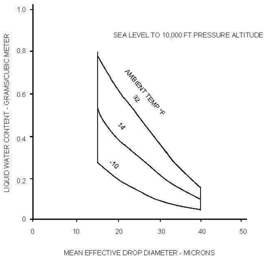
FIGURE 27.1419-3 CONTINUOUS ICING-LIQUID WATER CONTENT VS. DROP DIAMETER
