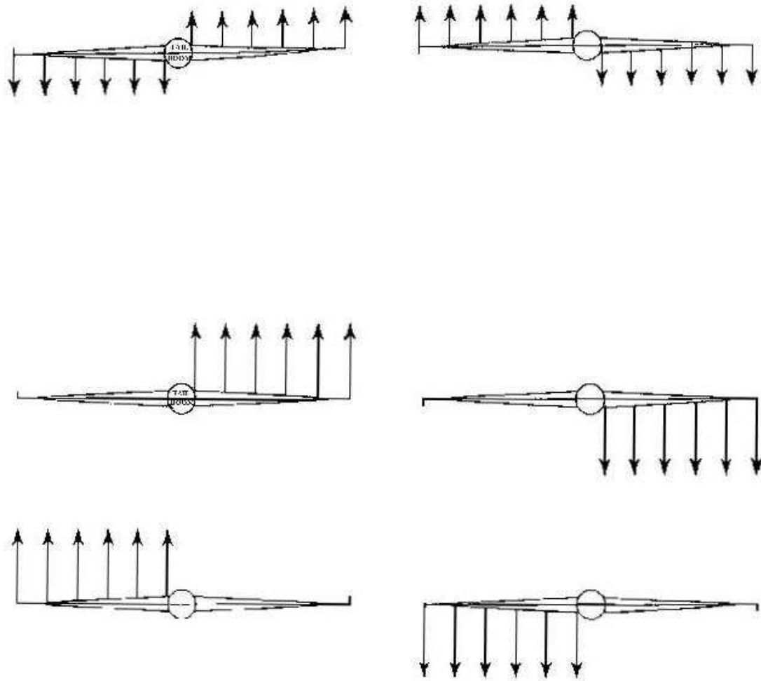
Figure AC 27.427-1 (View Looking Forward)
