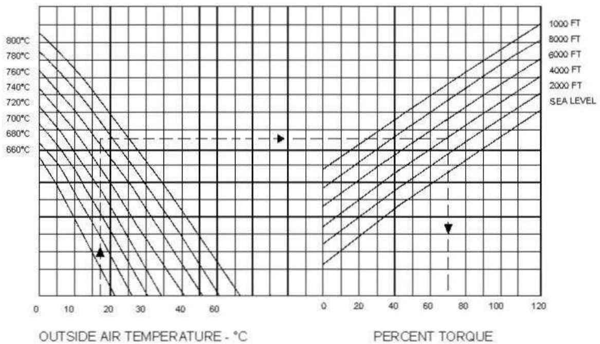
FIGURE AC 27-45-6 POWER ASSURANCE CHECK CHART
