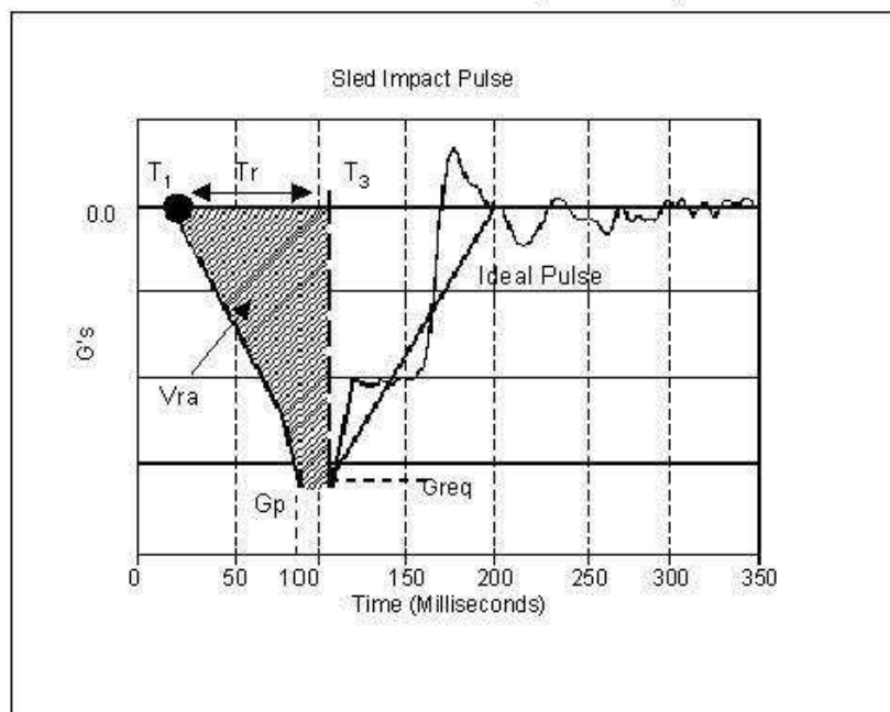
FIGURE AC 27.562-8. Change in Velocity ( V_{ra} )
