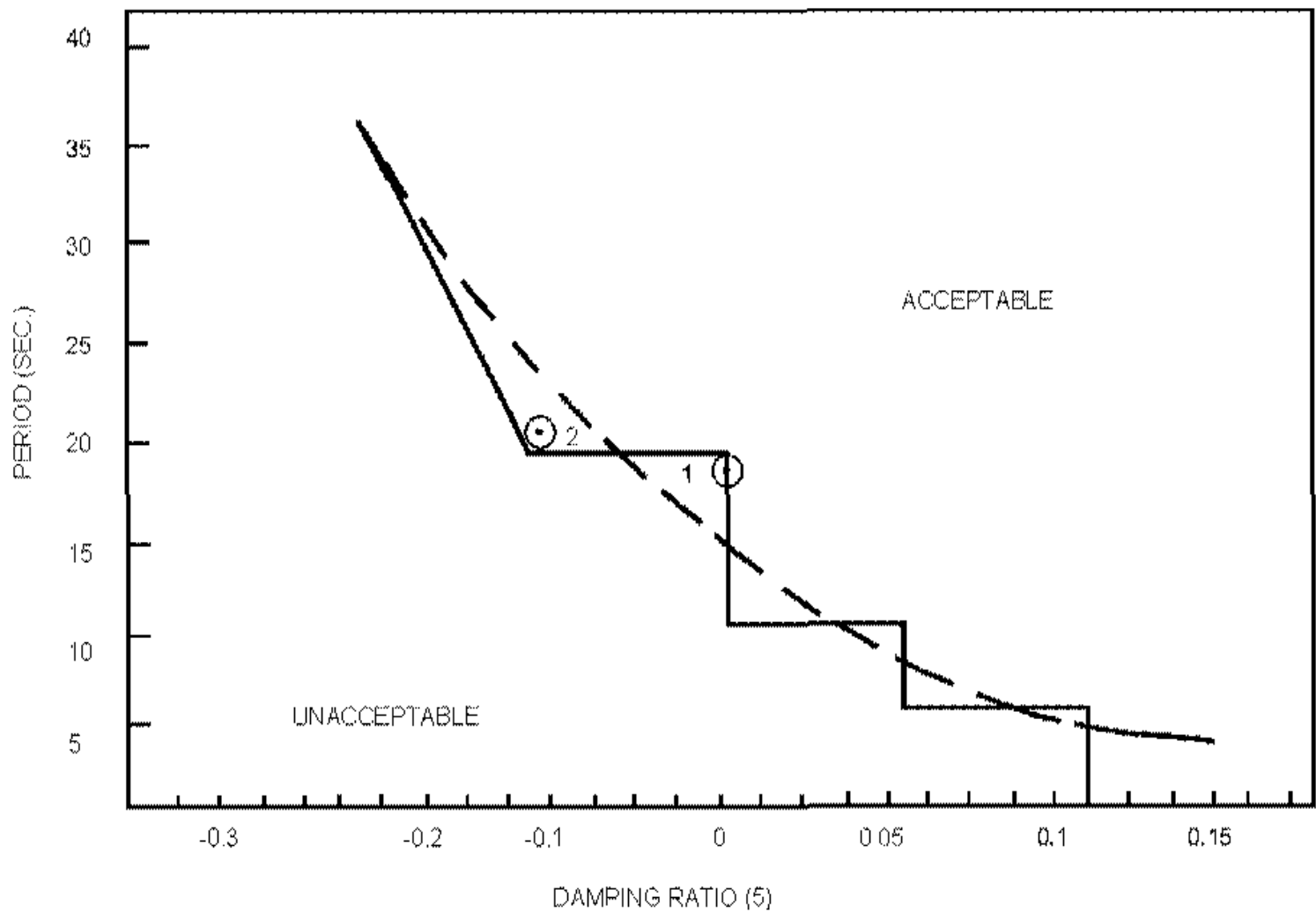
FIGURE AC 27-APX B-1 ROTORCRAFT DYNAMIC STABILITY REQUIREMENTS FOR IFR
