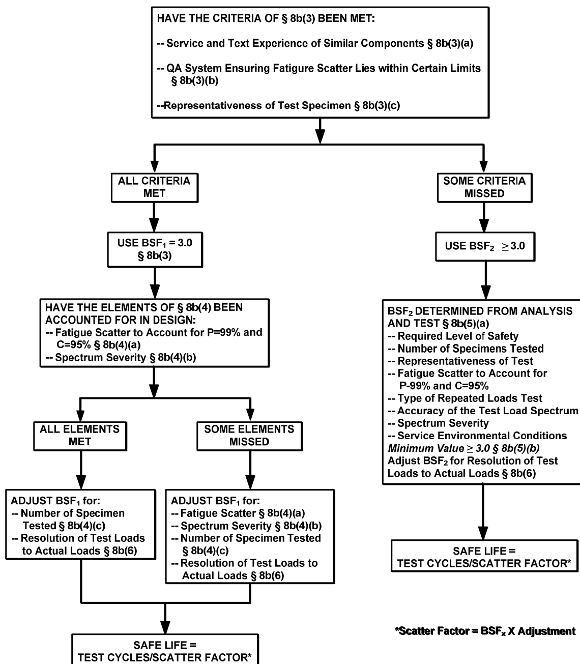
Figure 1 – Safe-Life Determination
