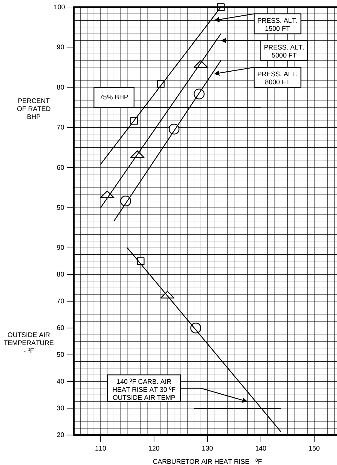
Figure 28 - Carburetor Air Heat Rise Plots
