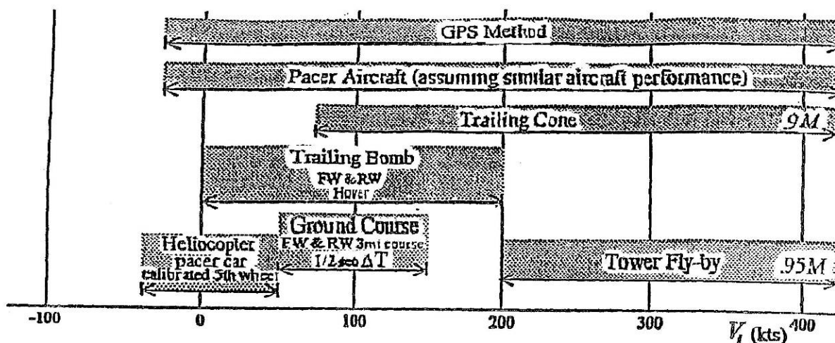
Figure A9-2 - Summary of PEC Test Methods
