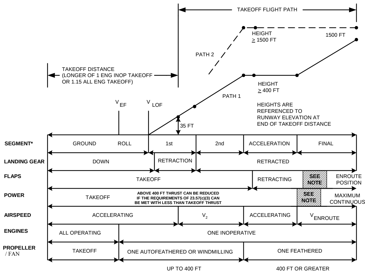
Figure 11 - Takeoff Segments and Nomenclature
