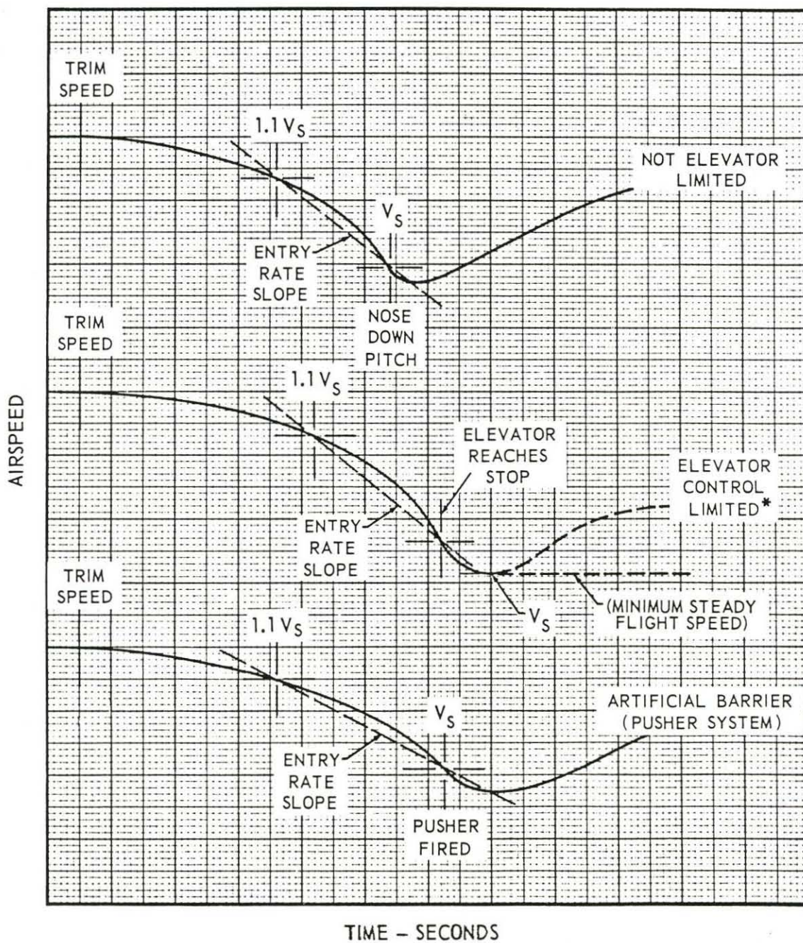
Figure 1 Stall Speed
