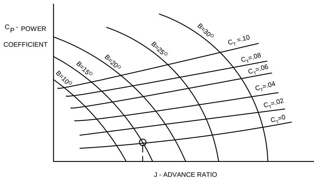
Figure 2 Propeller Coefficients
