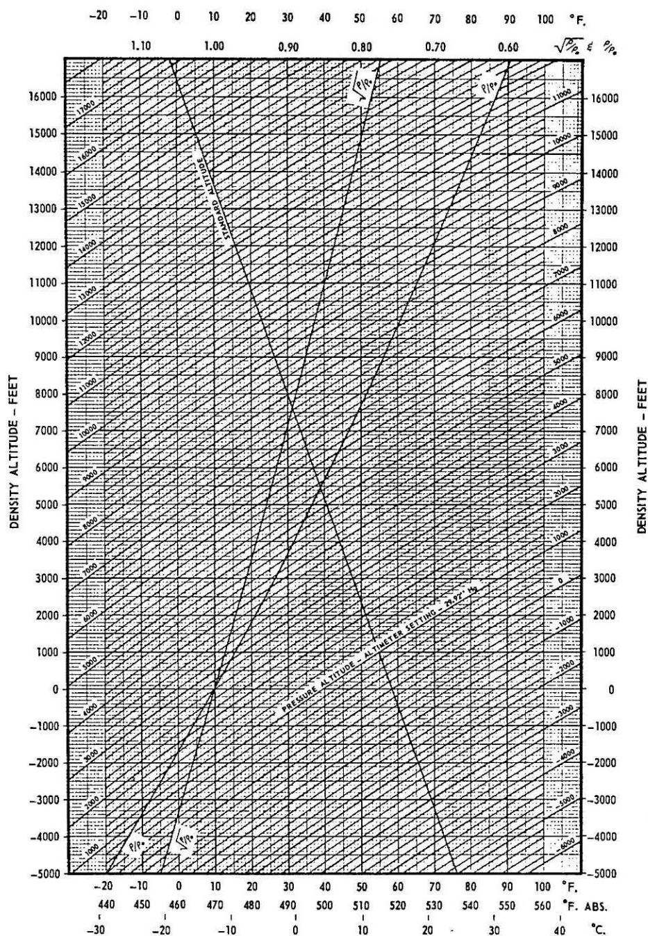
Figure A7-4 – Density/Pressure Altitude Conversion
