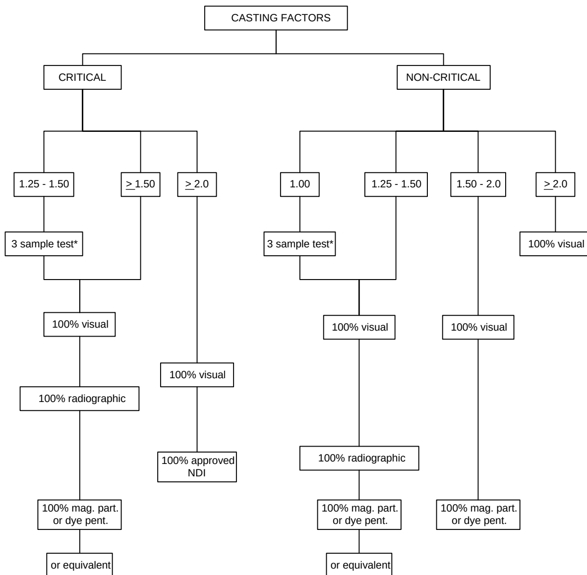
FIGURE 10 CASTING FACTOR INSPECTION REQUIREMENTS
