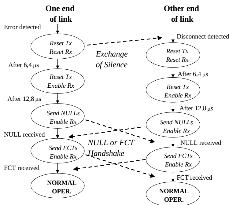
Figure 4-5: Link restart
