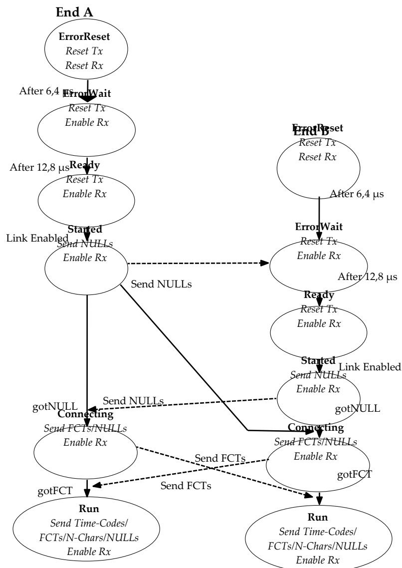
Figure 8-5: Example of typical initialization sequence
