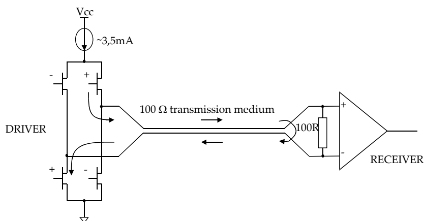
Figure 4-2: LVDS operation
