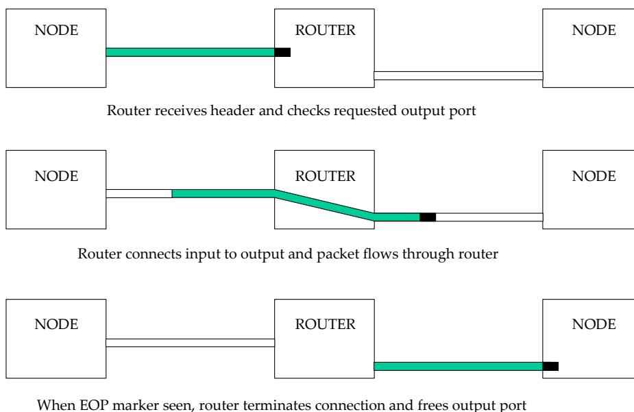
Figure 10-2: Wormhole routing
