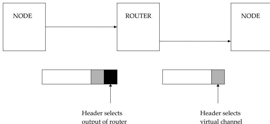
Figure 10-3: Header deletion
