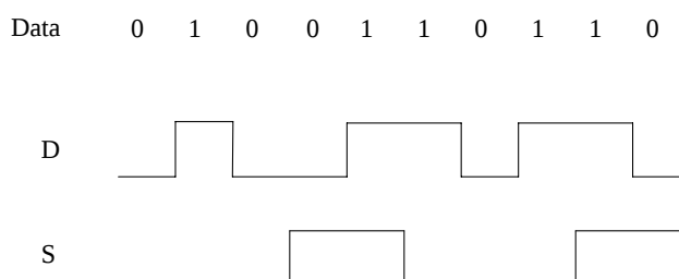
Figure 4-3: Data-Strobe (DS) encoding
