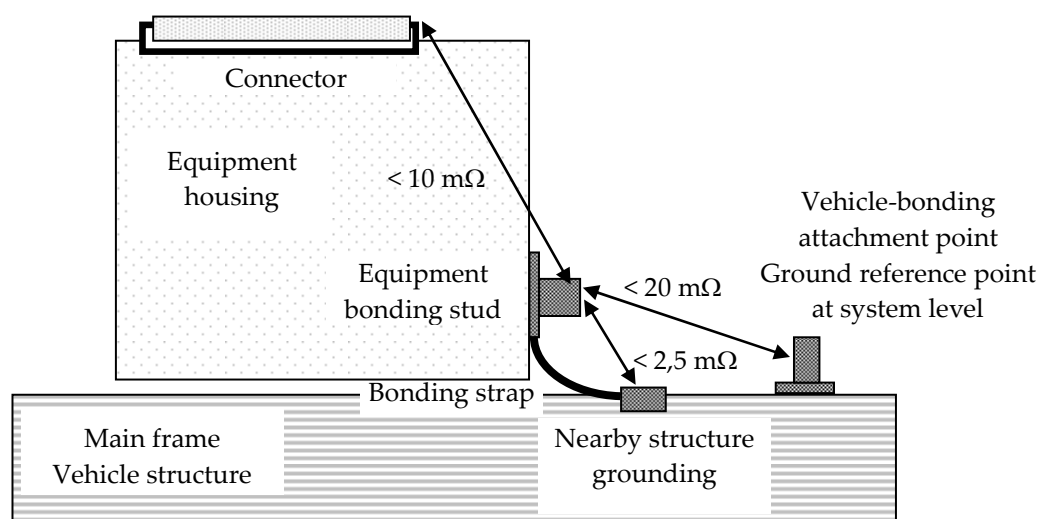
Figure 4-1: Bonding requirements
