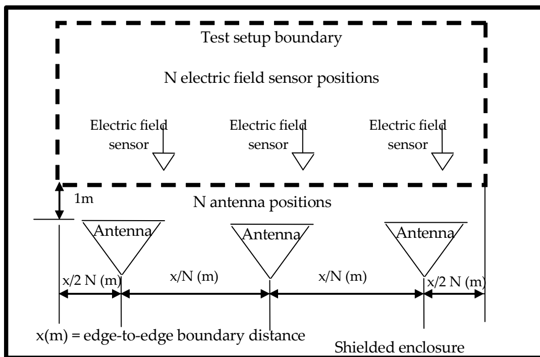
Figure 5-27: RS Electric field. Multiple test antenna positions
