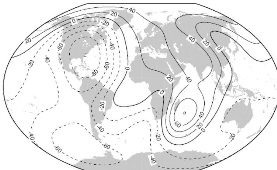
Figure E-1: The IGRF-10 field strength (nT, contour level = 4 000nT, at 2005) and secular variation (nT yr -1 , contour level = 20 nT yr -1 , valid for 2005), at geodetic altitude 400 km with respect to the WGS-84 reference ellipsoid).
