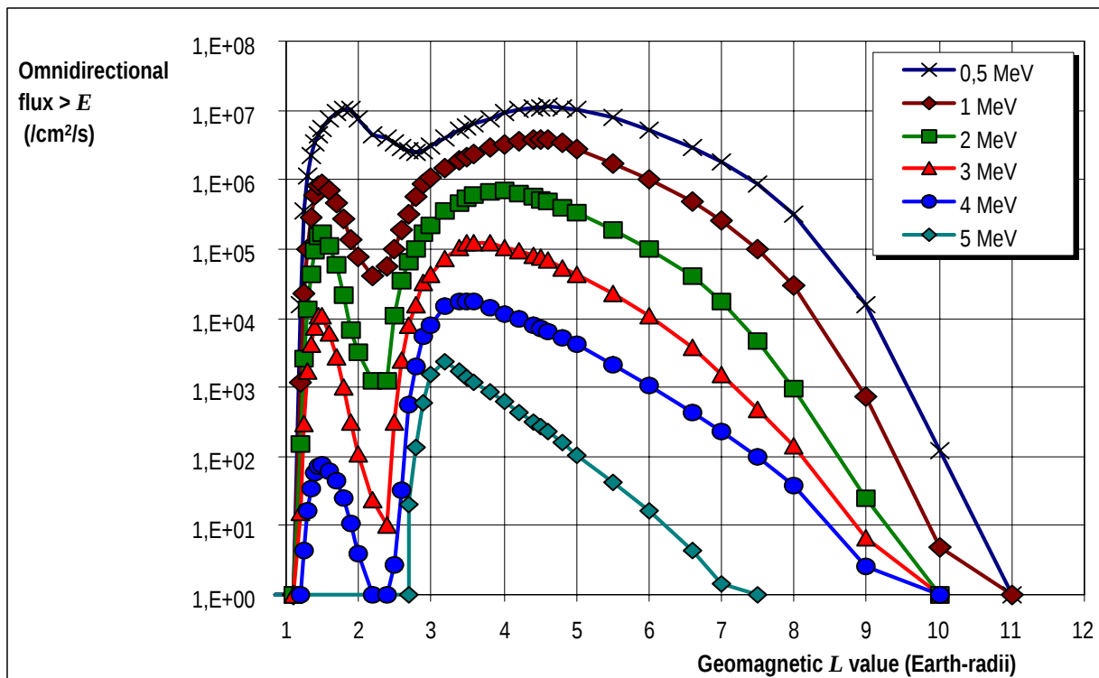
(a) Electron
