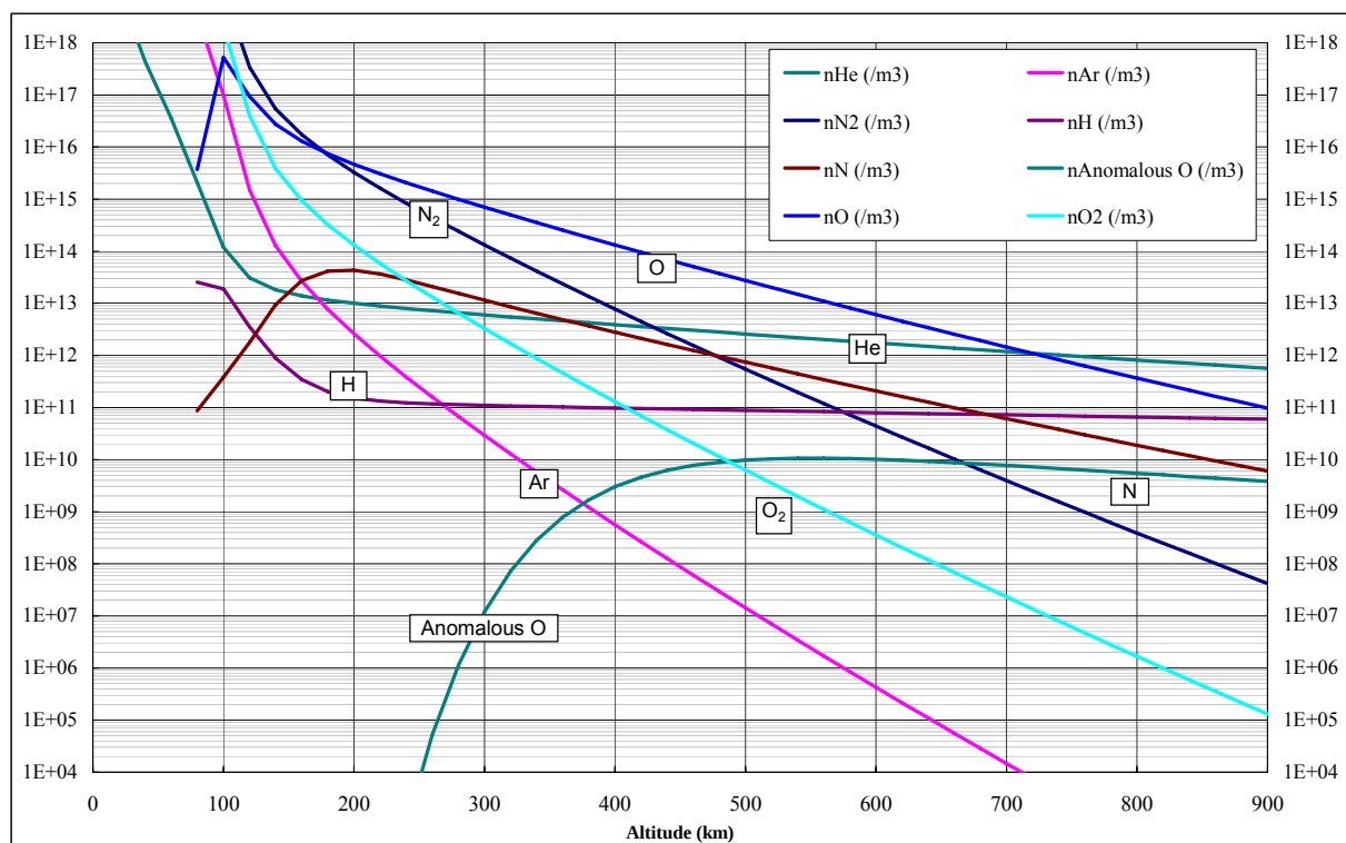
Figure G-4: Variation of the NRLMSISE-00 mean concentration profile of the atmosphere constituents N_2 , O , O_2 , He , Ar , H , N and anomalous O with altitude for moderate solar and geomagnetic activities ( F_{10.7} = F_{10.7_{avg}} = 140 , A_p = 15 )
