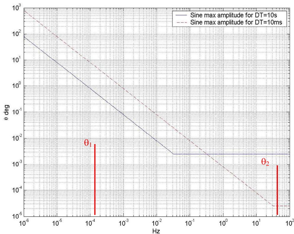
Figure C-9: Frequency stability templates for requirements C.3a3 and C.3a4
