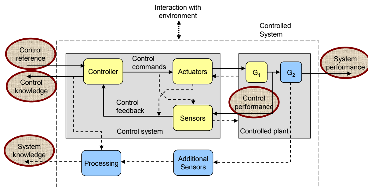
Figure 4-2 General control structure extended up to system level
