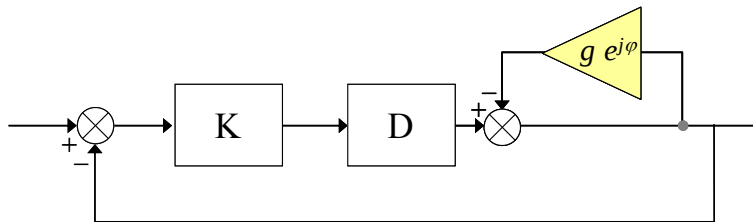
Figure A-6: Output feedback uncertainty
