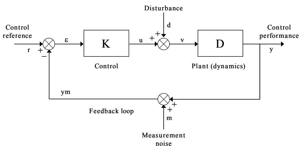
Figure 6-1 Simplified scheme for a closed-loop controlled system
