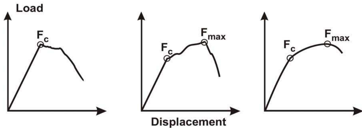
Figure F-14: Carbon fibre tube inserts: Definition of the critical insert failure load, F_c
