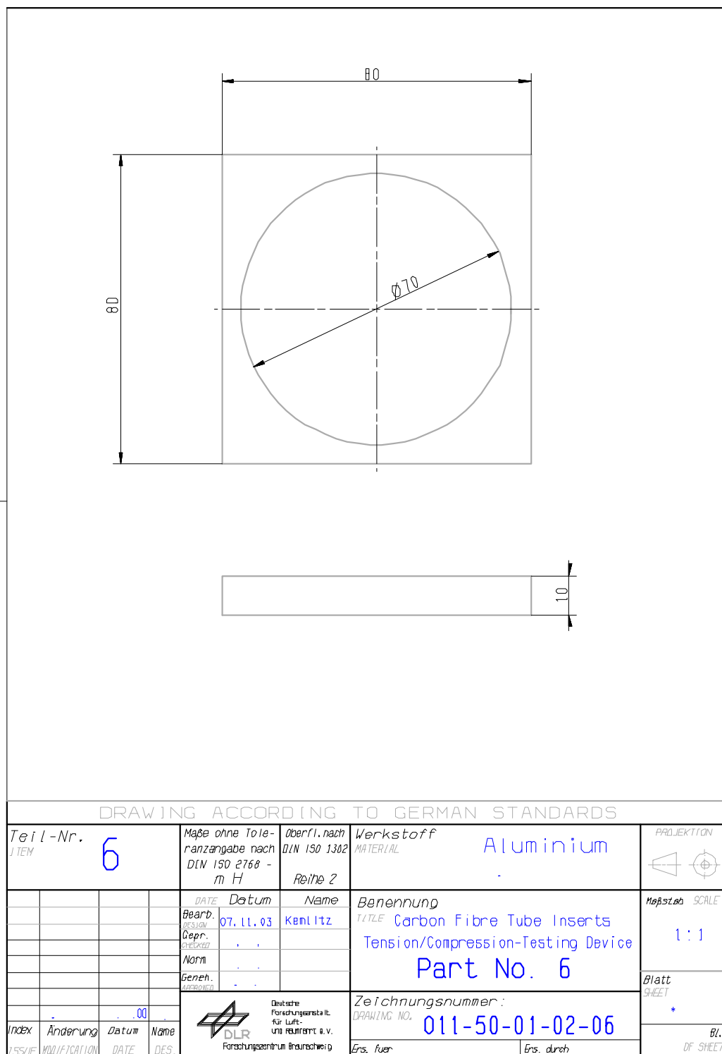
Figure H-7: Test fixture: Tension-compression load – part 6
