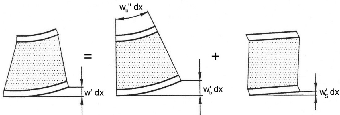
Figure 8-3: Deformed sandwich beam element: deflection contributions from both bending and shearing
