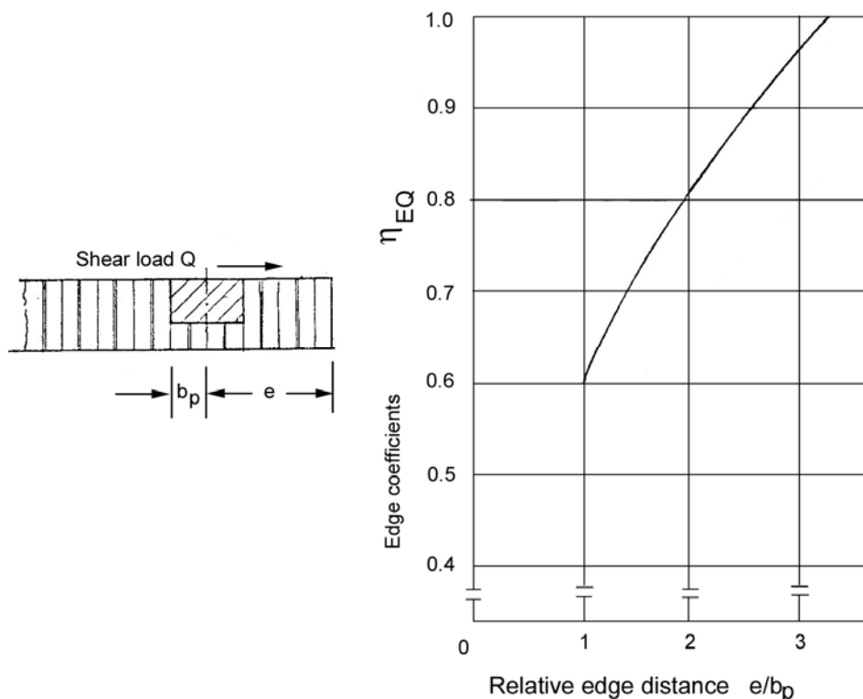
Figure 14-8: Shear strength: Influence of edge distance
