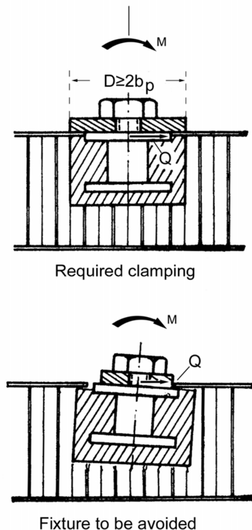
Figure 15-1: Inserts loaded in bending: Clamping conditions
