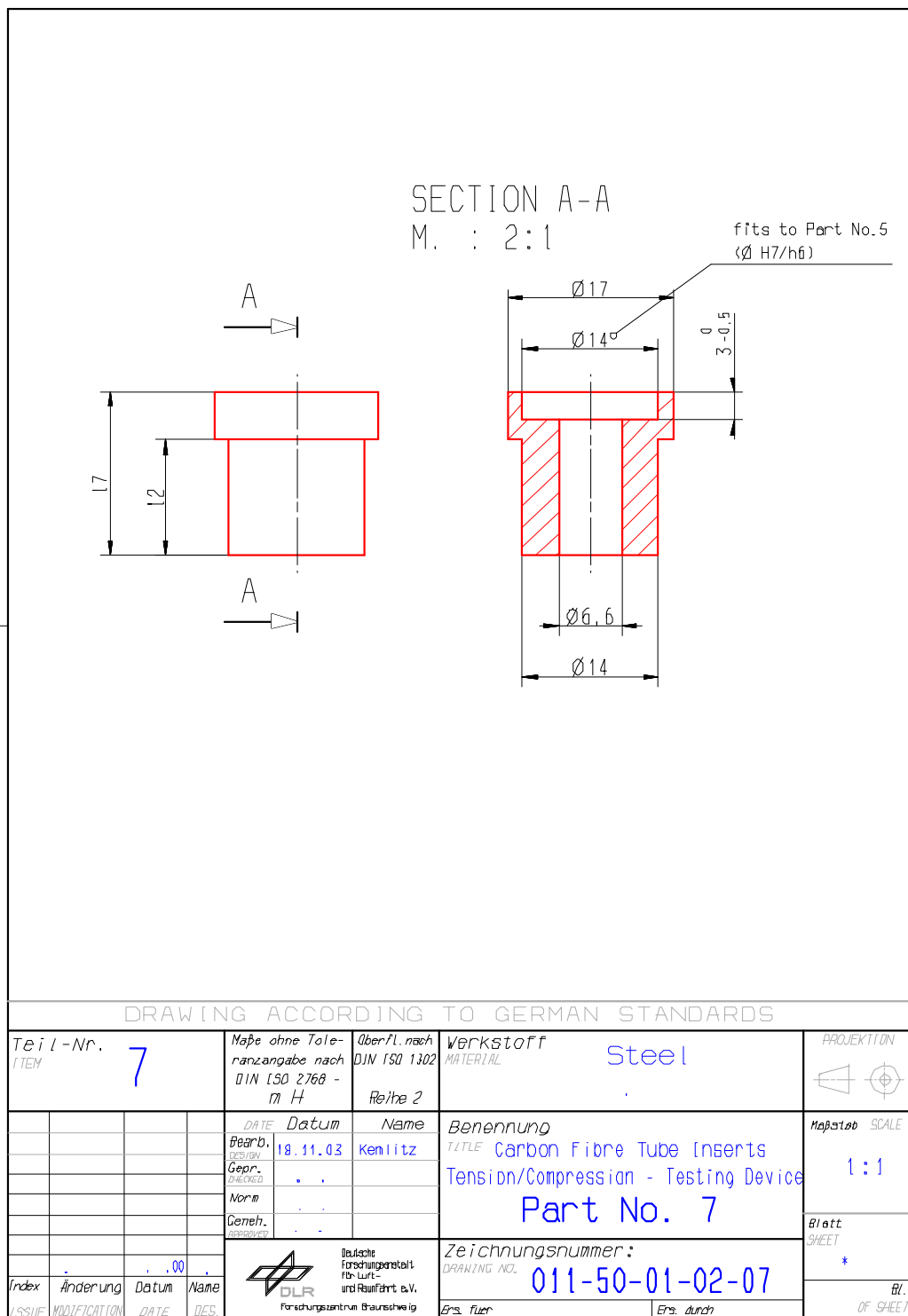
Figure H-8: Test fixture: Tension-compression load – part 7
