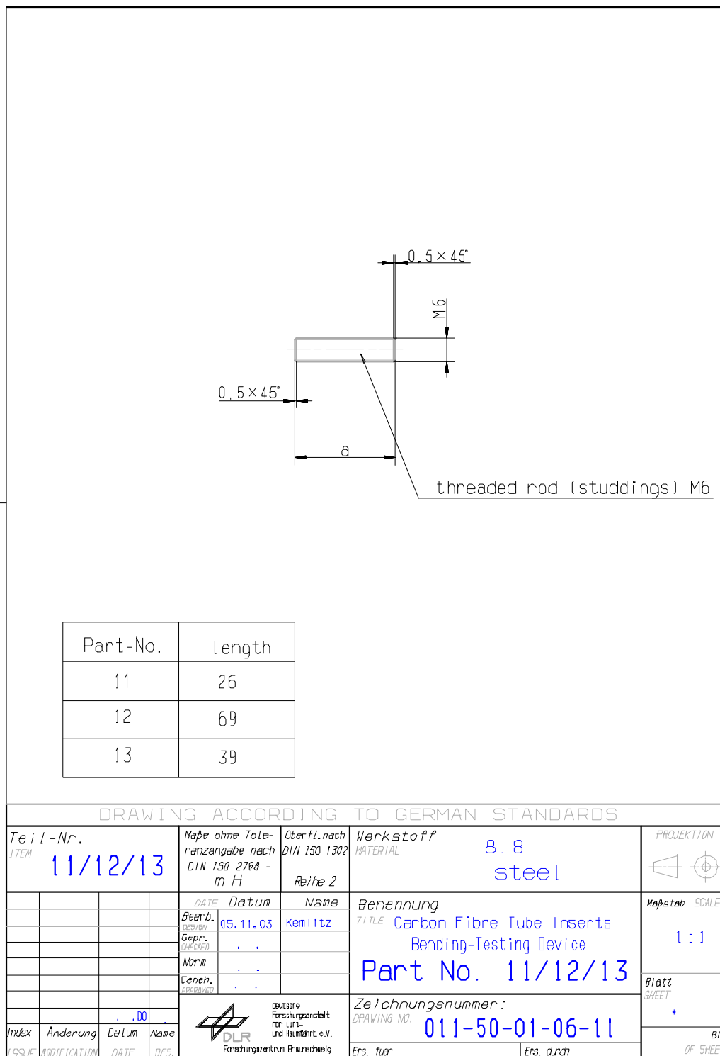
Figure H-29: Test fixture: Bending – parts 11, 12 and 13
