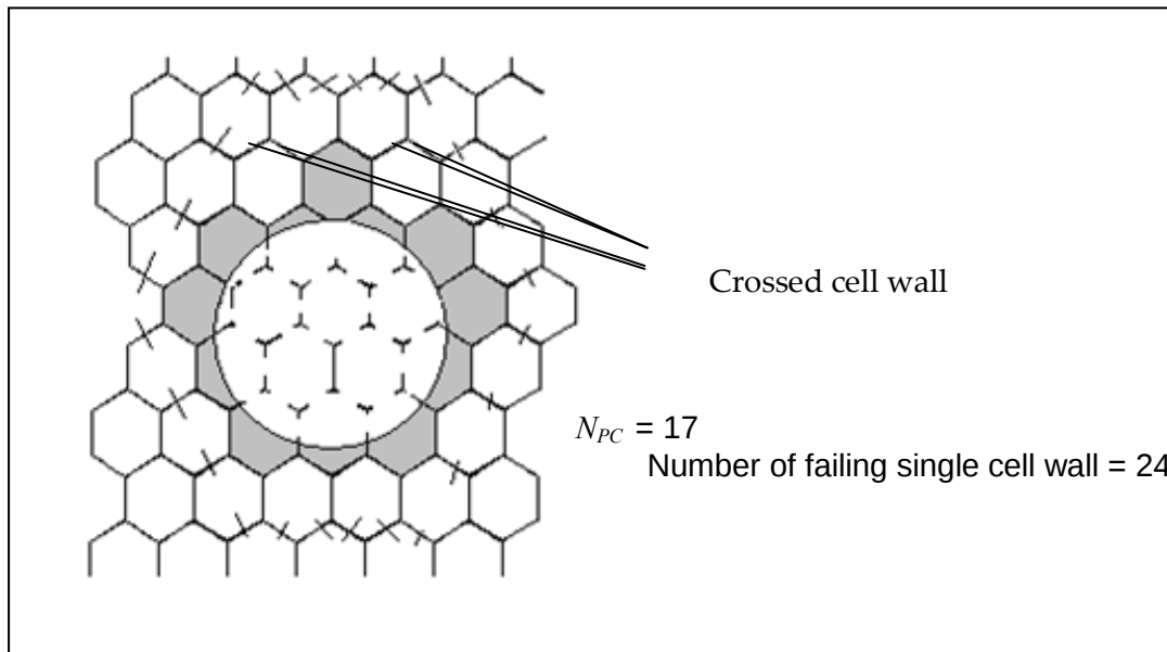
Figure 10-18: Failure modes: Unsymmetrical potting and crossed cell
