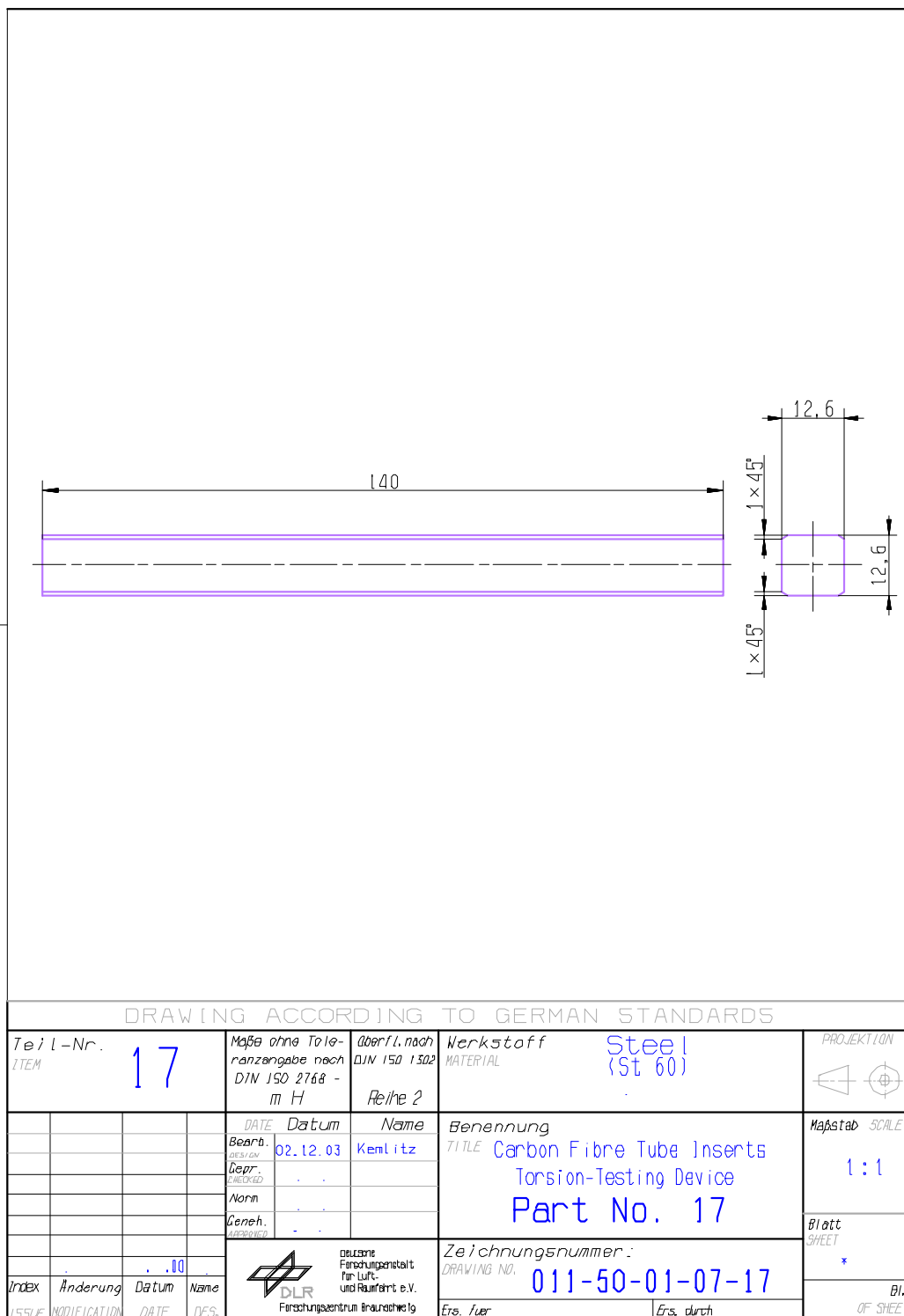
Figure H-48: Test fixture: Torsion – part 17
