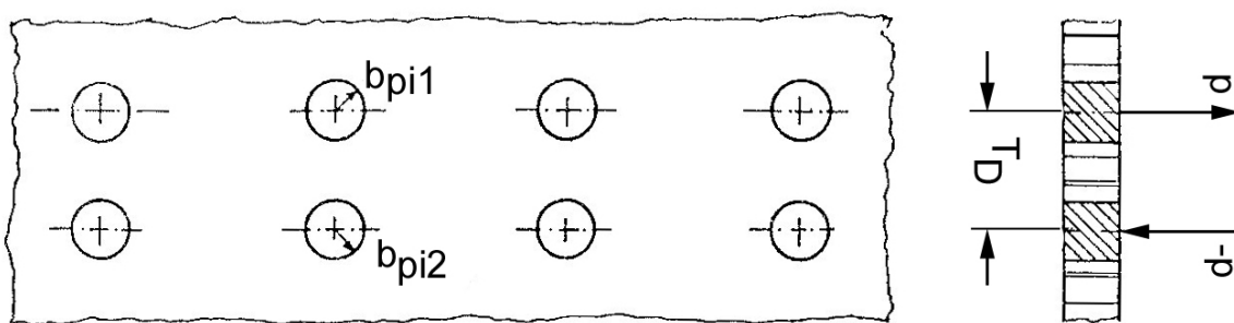
Figure 19-3 Insert groups: series of inserts loaded in opposite directions
