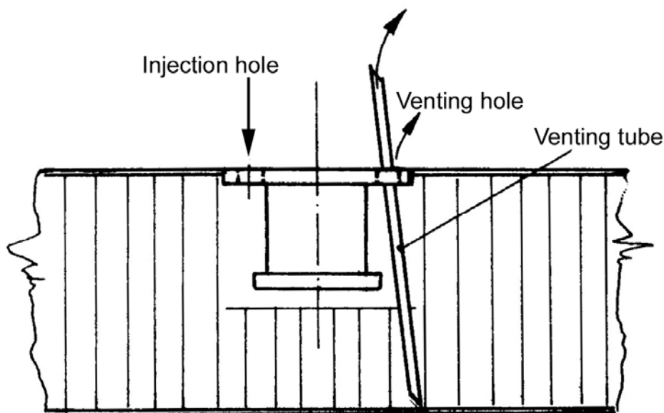
Figure 23-3: Venting of non-perforated core
