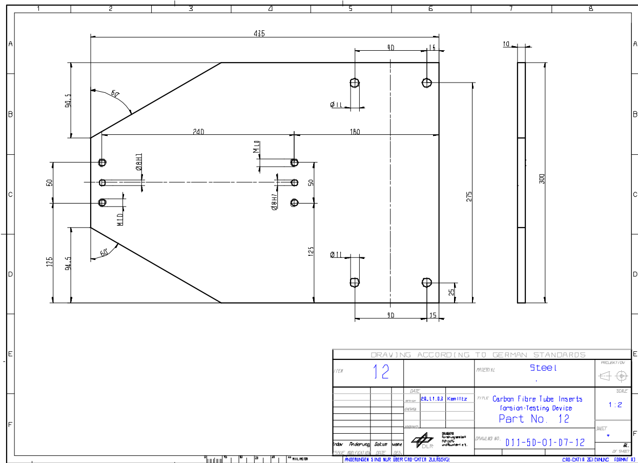
Figure H-43: Test fixture: Torsion – part 12
