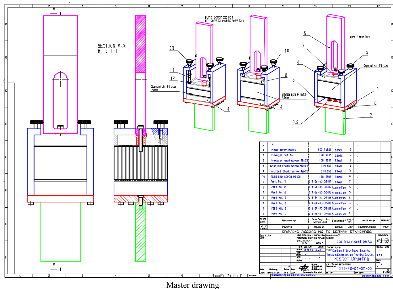
Figure H-1: Test fixture: Tension-compression load – master drawing
