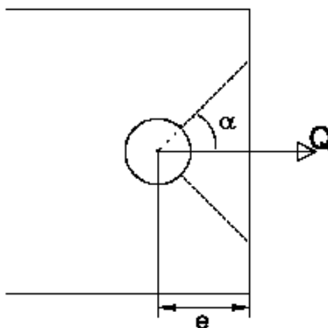
Figure 14-6: Shear strength: Failure angle
