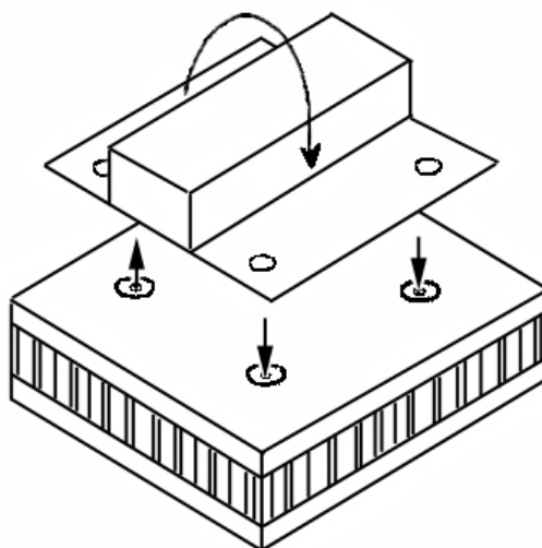
Figure 10-14: Failure modes: Moment load
