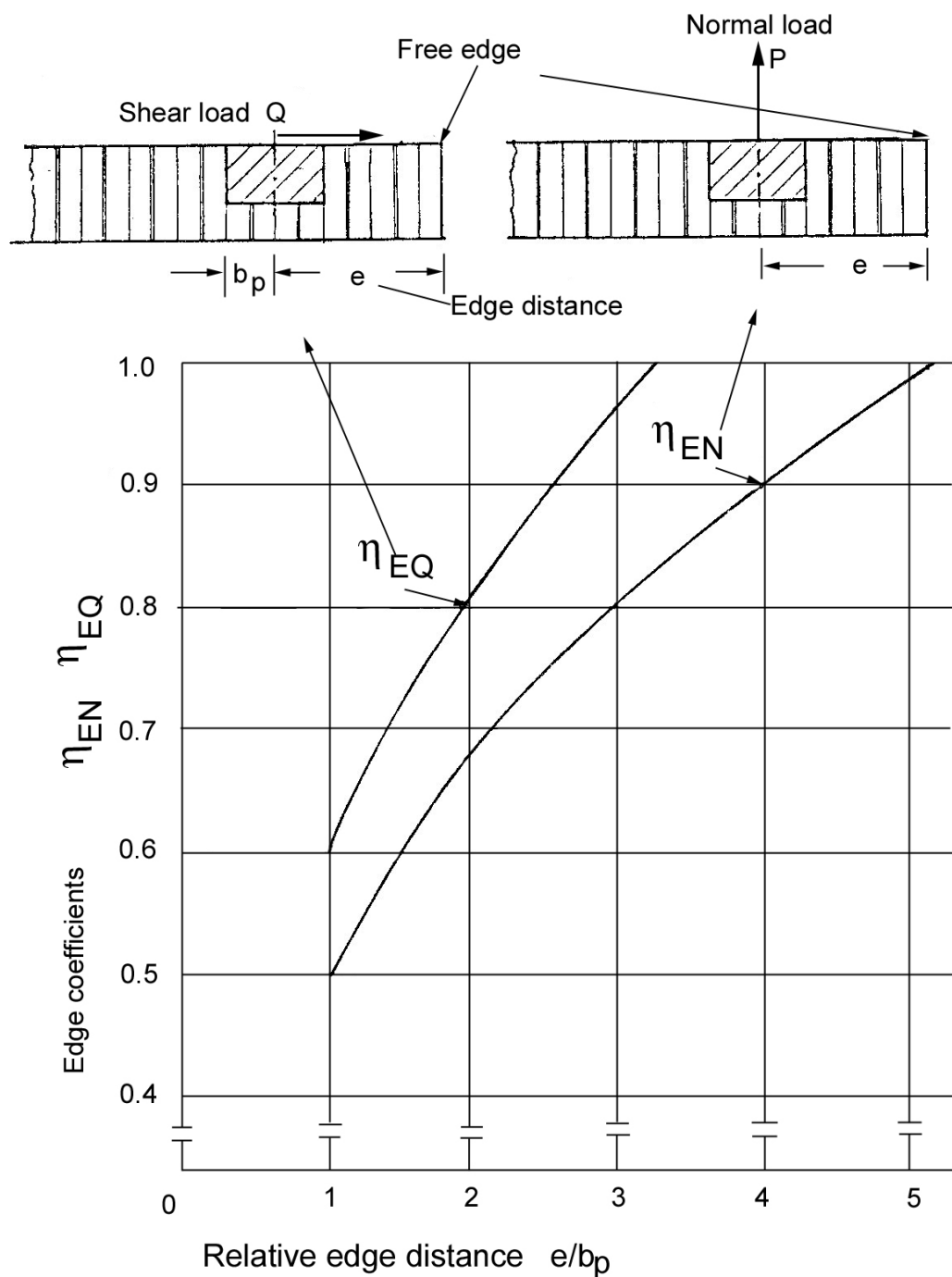
Figure 18-1: Edge distance: Effect on insert static strength capability
