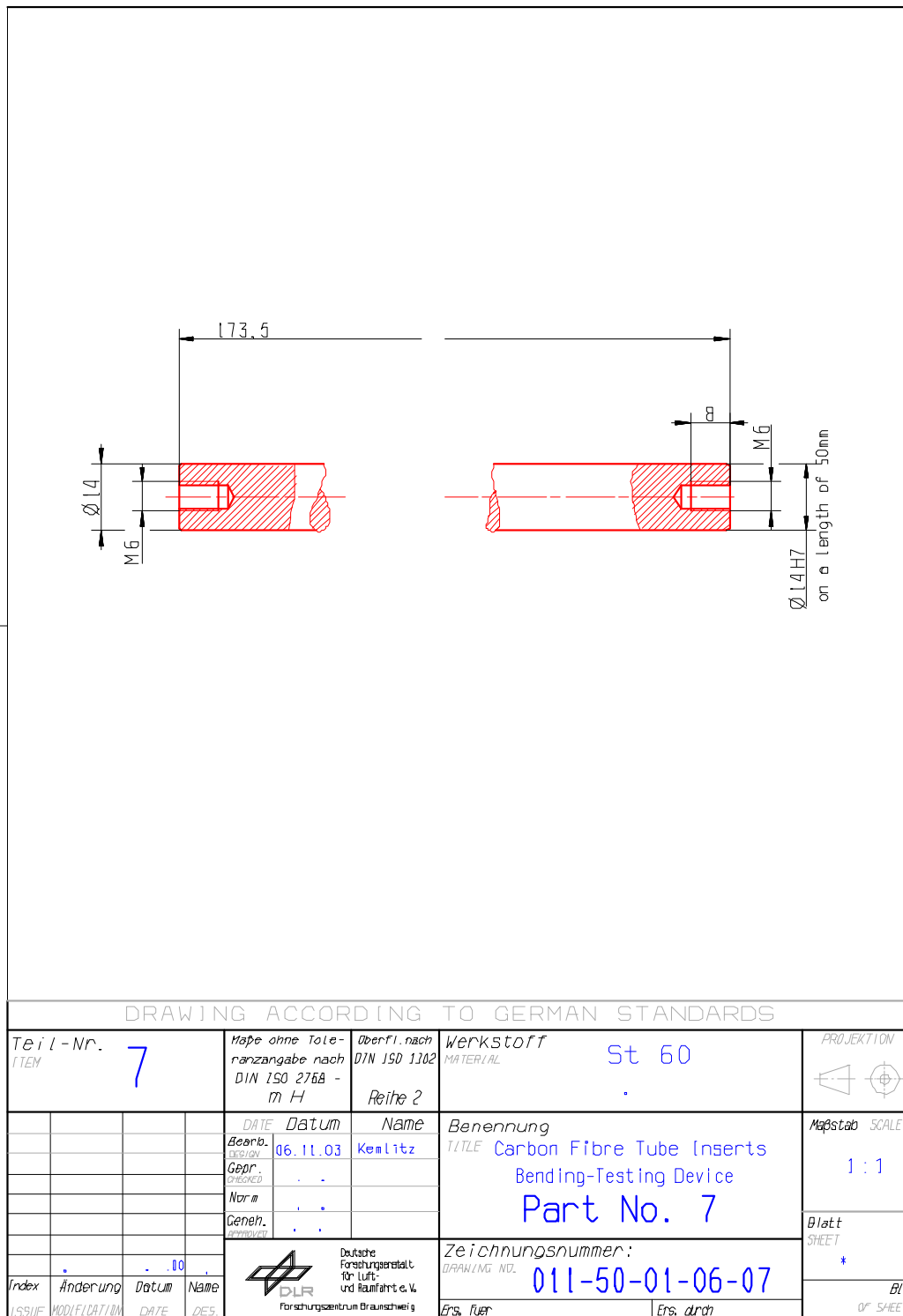
Figure H-25: Test fixture: Bending – part 7
