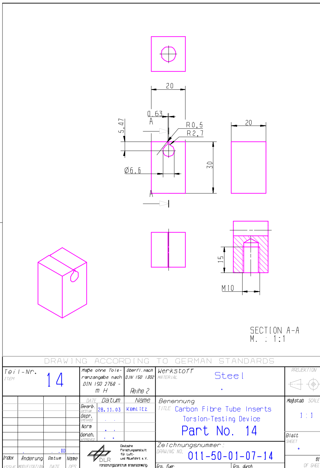
Figure H-45: Test fixture: Torsion – part 14
