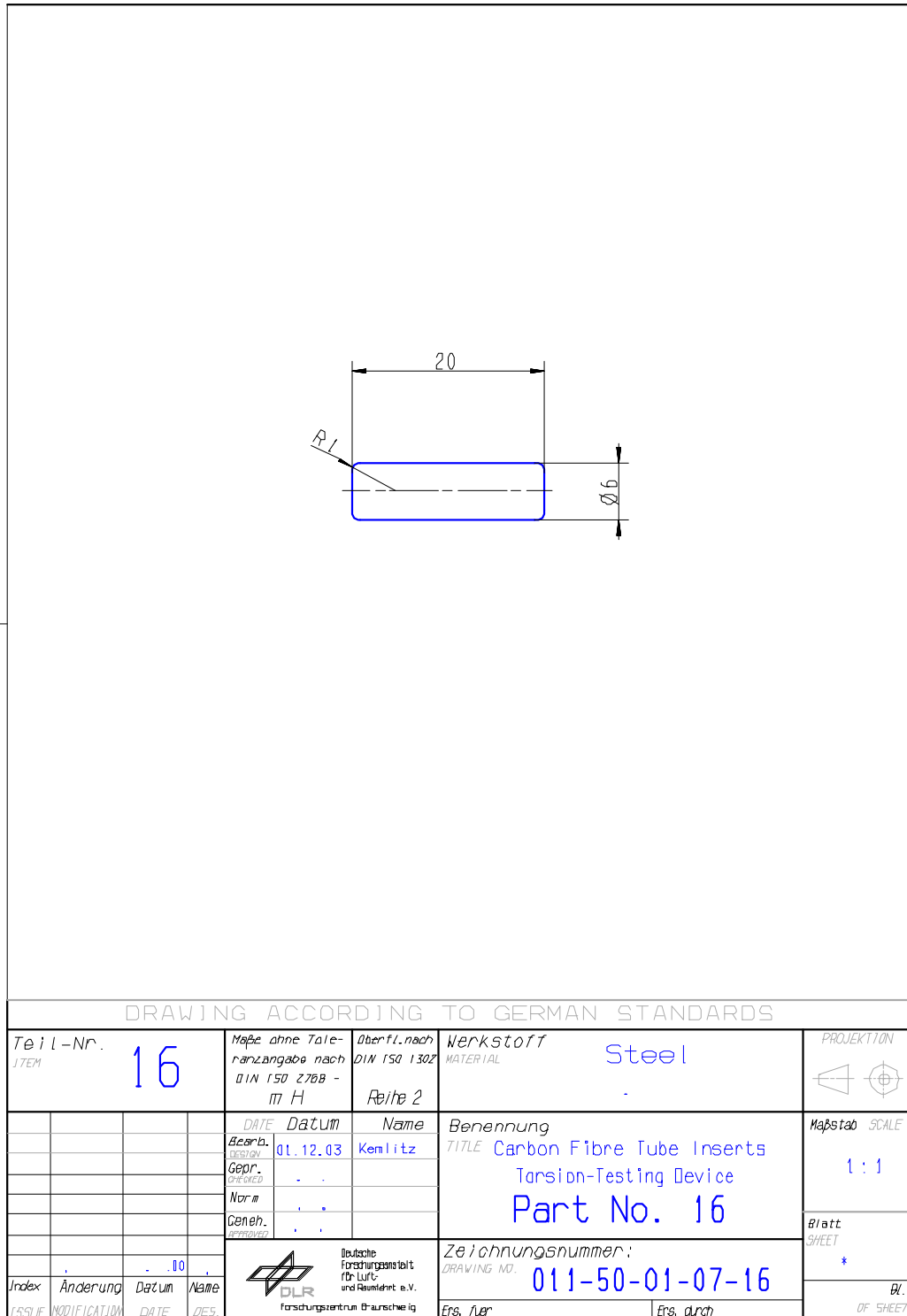
Figure H-47: Test fixture: Torsion – part 16
