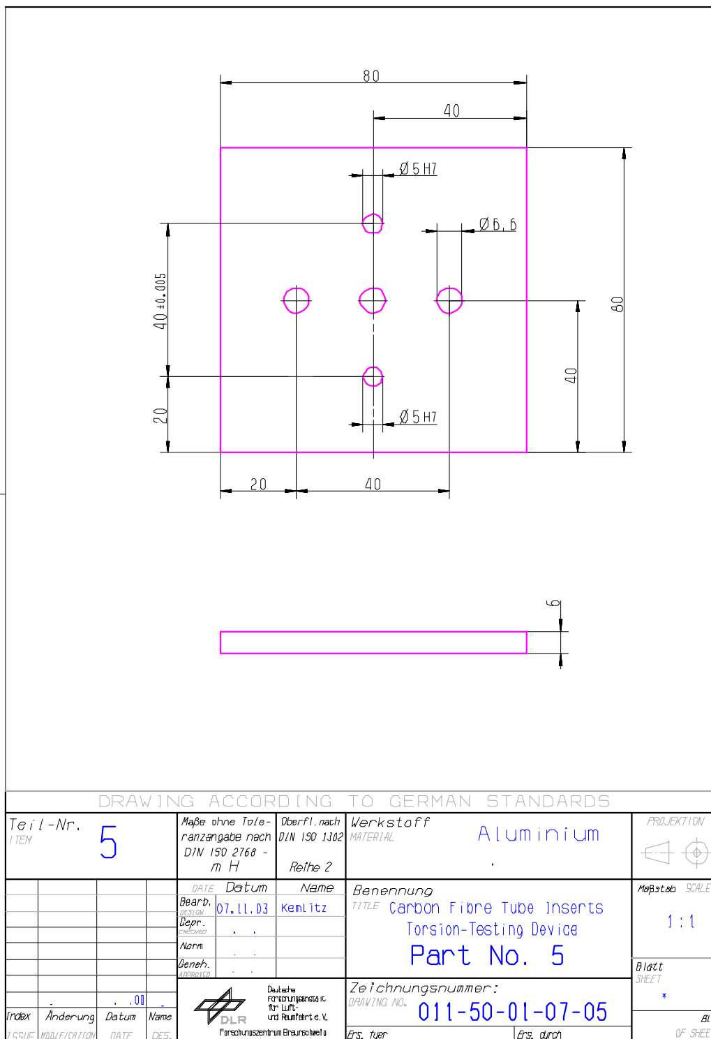
Figure H-36: Test fixture: Torsion – part 5
