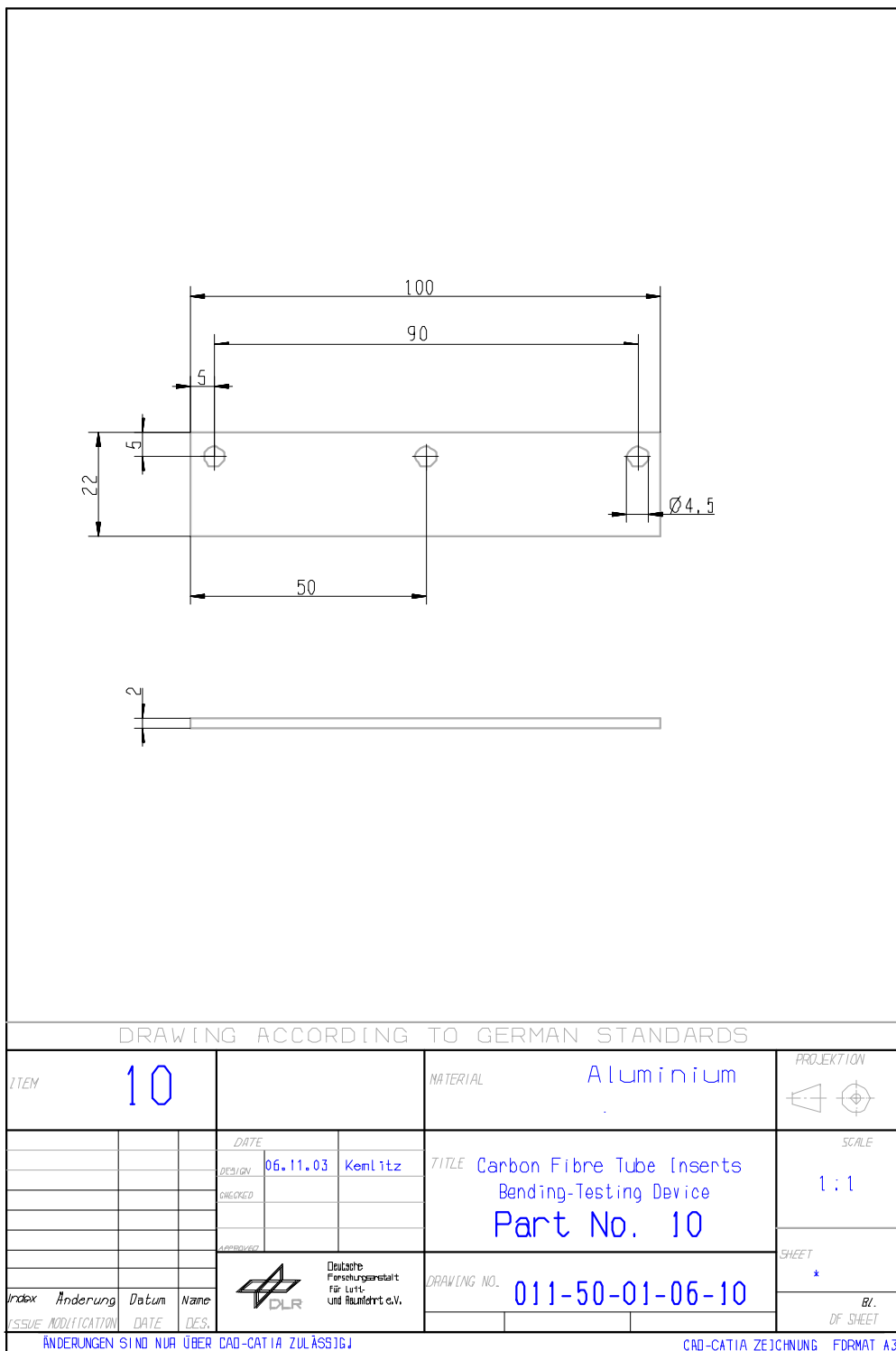
Figure H-28: Test fixture: Bending – part 10
