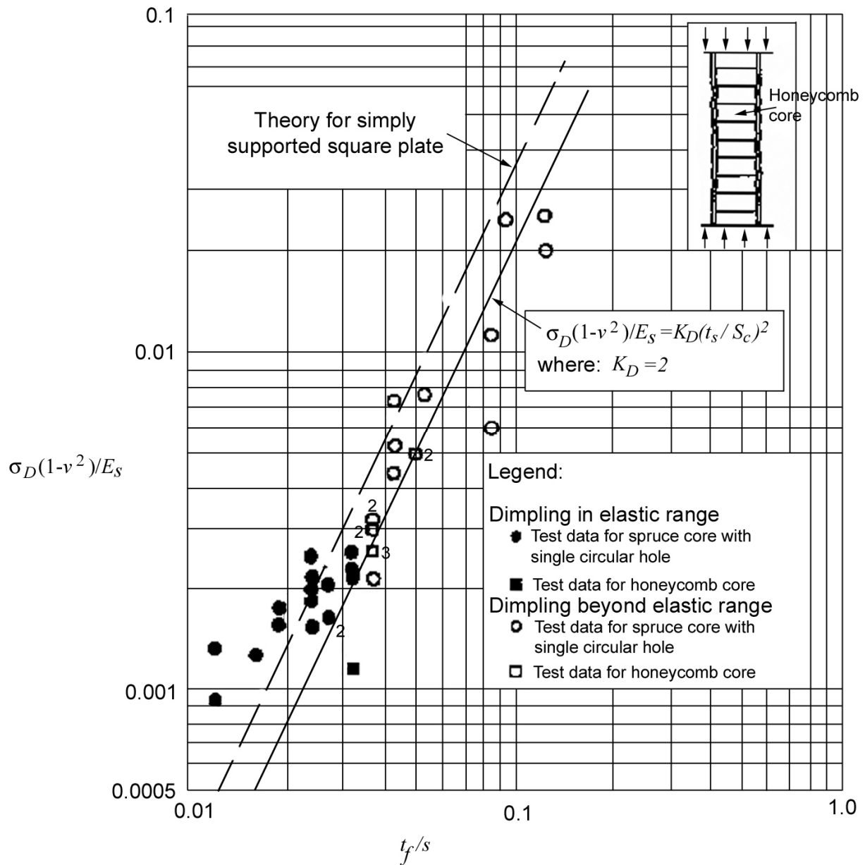
Figure 14-7: Shear strength: Critical stresses for intracellular buckling (dimpling) under uniaxial compression
