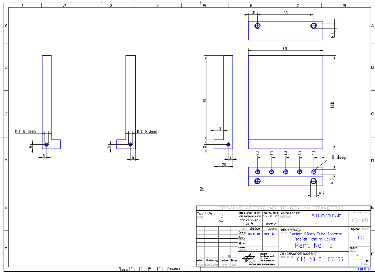
Figure H-34: Test fixture: Torsion – part 3
