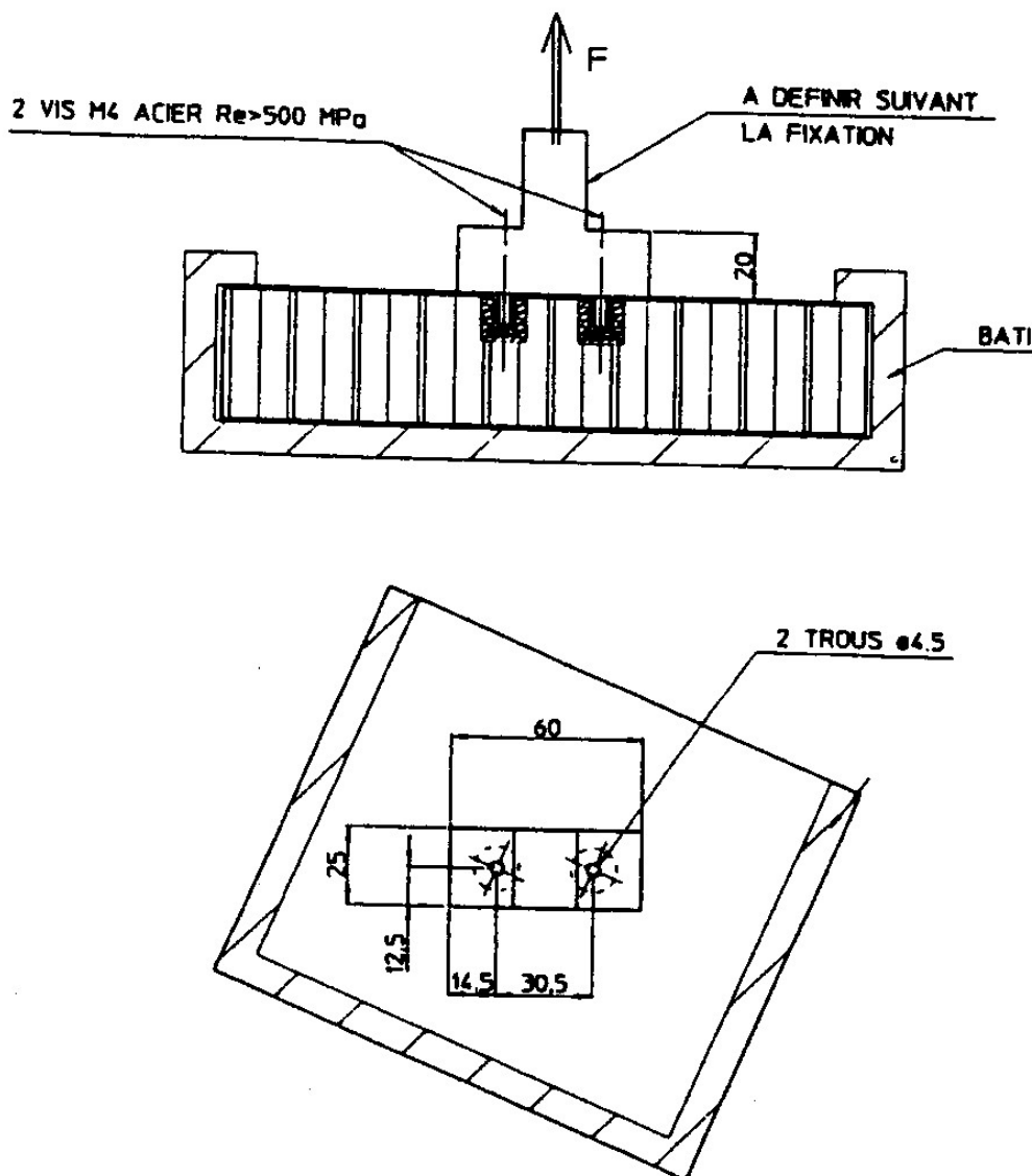
Figure F-9: Case study: ASAP 4 (AR4) - tensile (pull-out) method B
