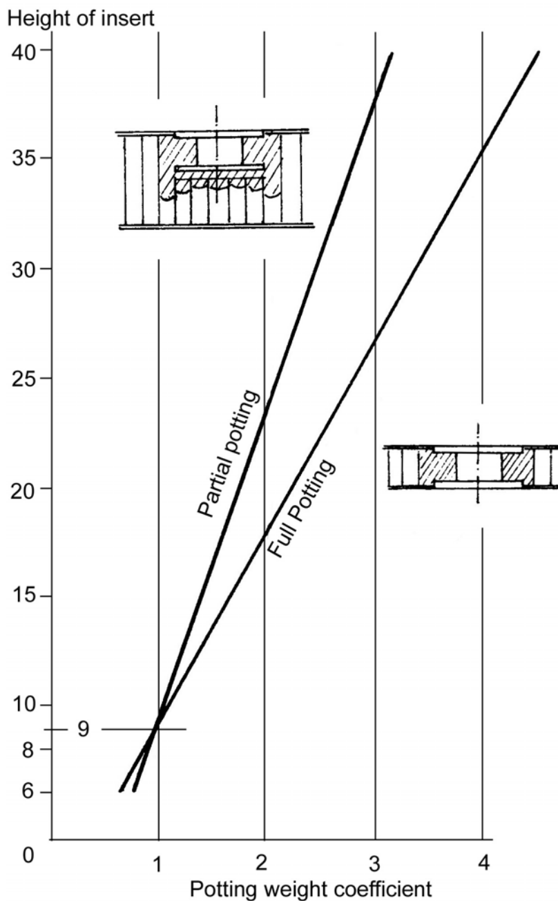
Figure 7-6: Correction coefficient for weight of insert heights
