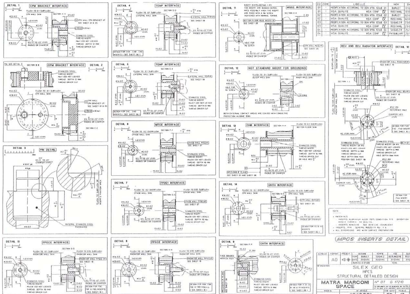
Figure F-20: Case study: SILEX GEO MPCS – insert
