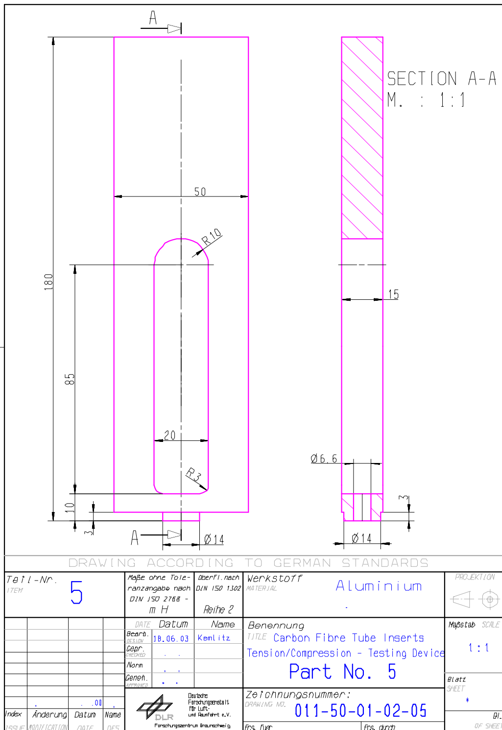
Figure H-6: Test fixture: Tension-compression load – part 5
