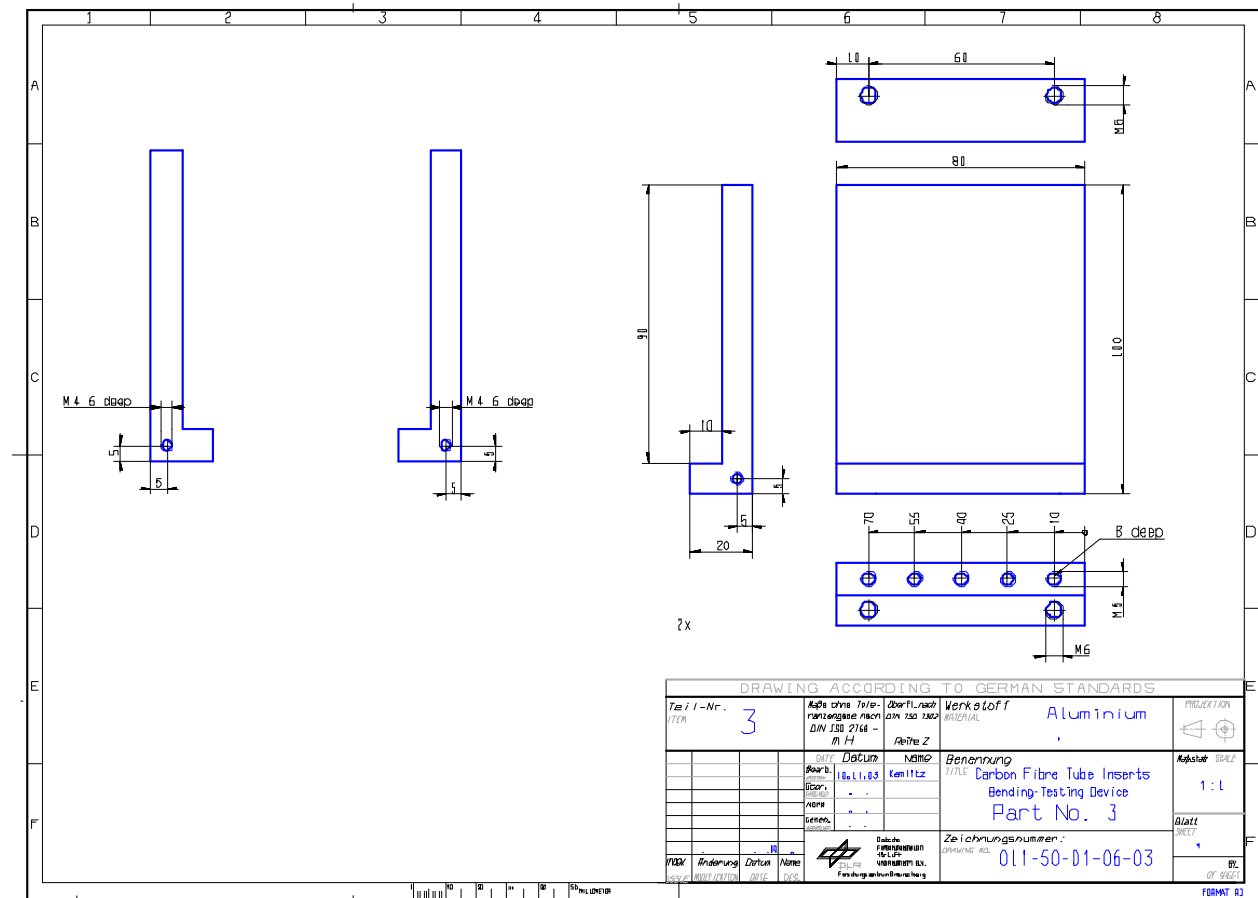
Figure H-21: Test fixture: Bending – part 3
