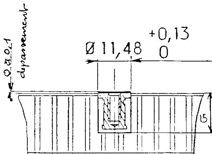
Figure F-1: Case study: ARIANE 1 equipment bay / ASAP 4 - tensile (pull-out) test method
