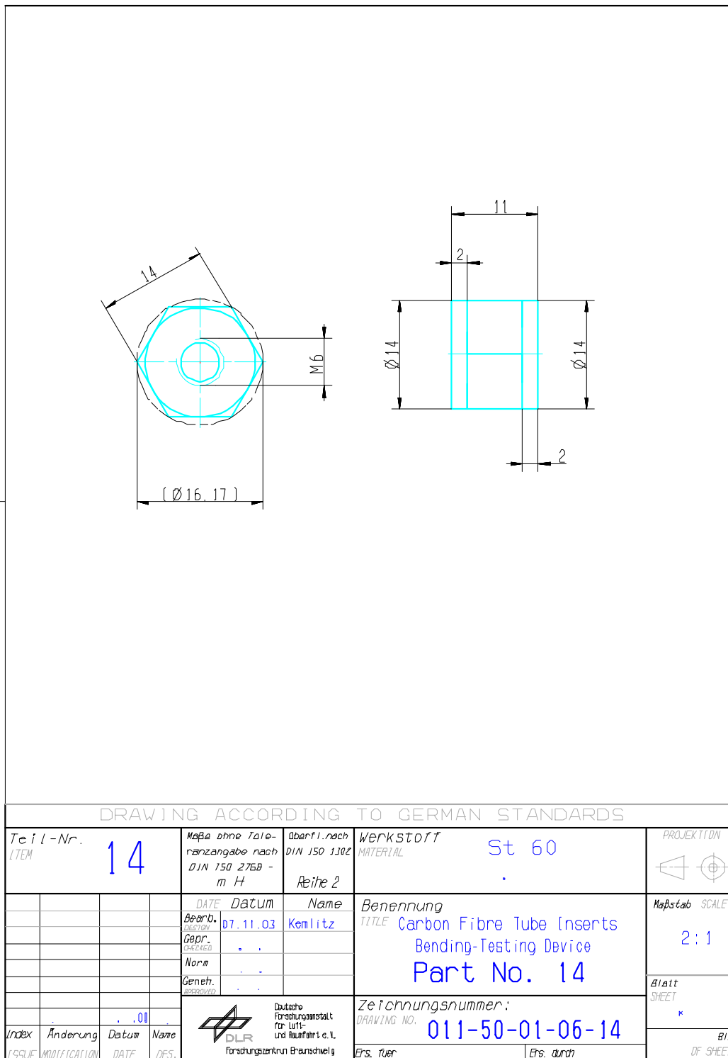
Figure H-30: Test fixture: Bending – part 14
