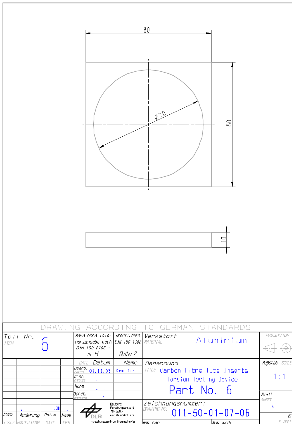
Figure H-37: Test fixture: Torsion – part 6
