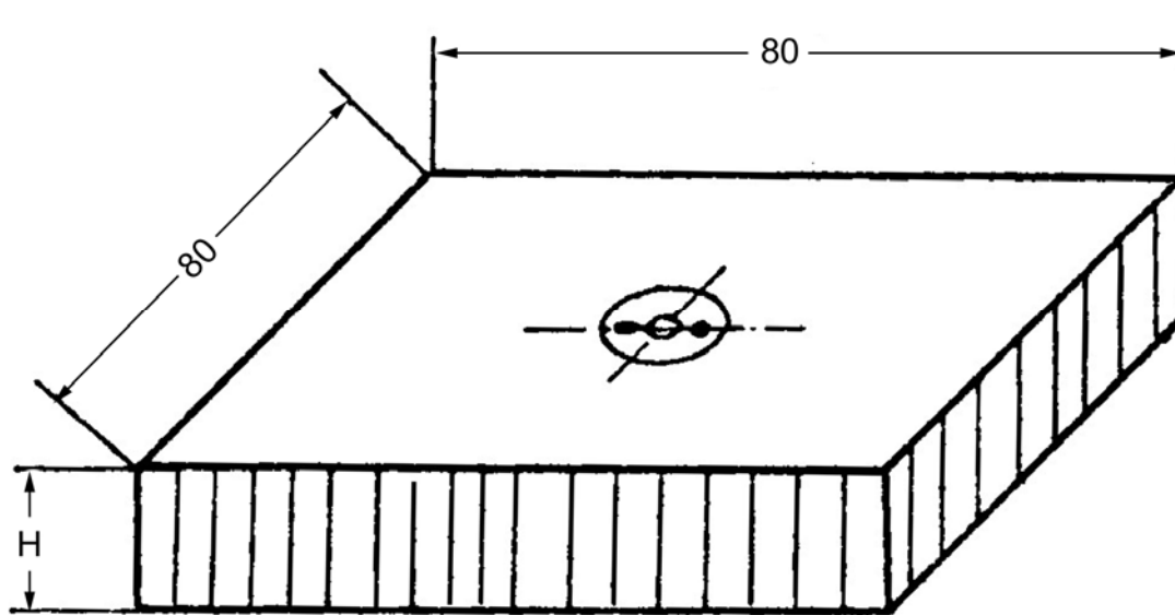
Figure 23-4: Reference sample: Pull-out strength test specimen Proof load
