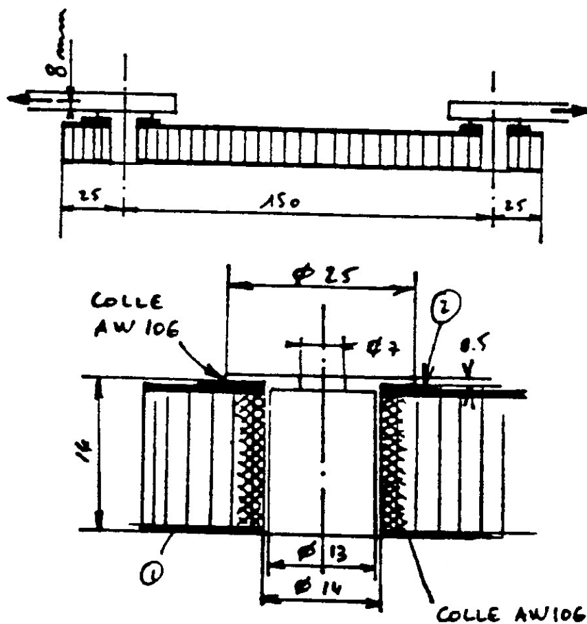
Figure F-5: Case study: ARIANE 4 - shear test method
