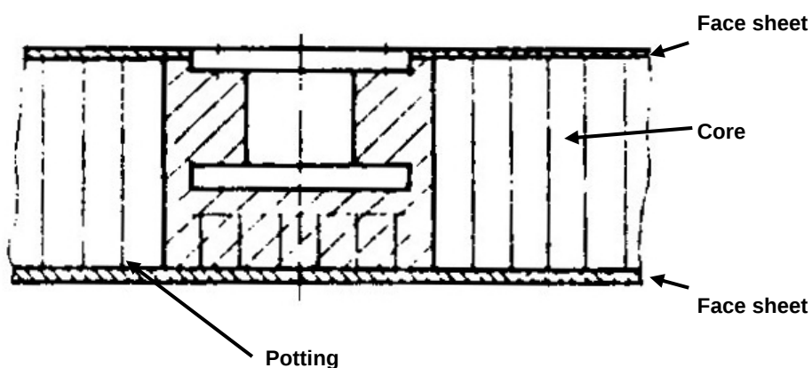
A – Typical standard-type insert
