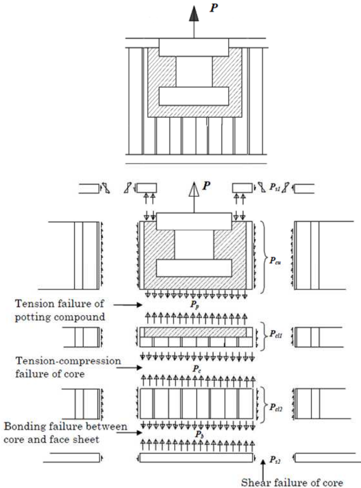
Figure 10-15: Failure modes: Load transfer in out-of-plane case
