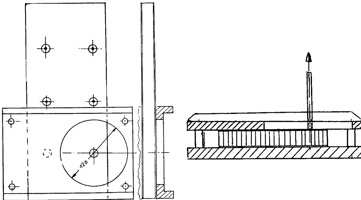
Figure 29-5: Testing: Edge distance fixture
