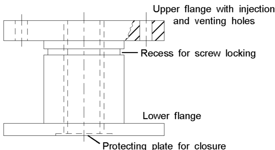
Figure 5-1: Typical insert
