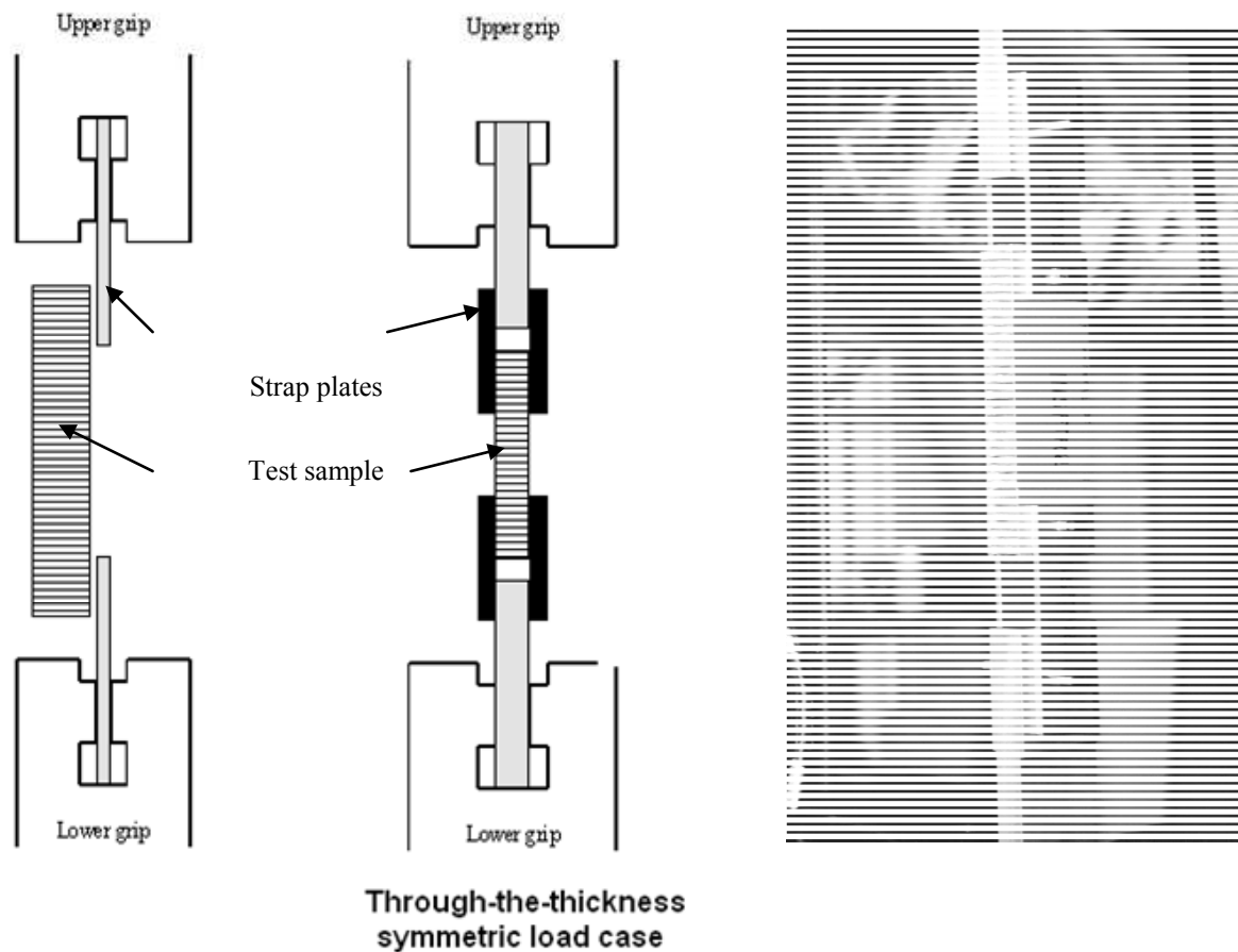
Figure 29-3: Testing: ASTM insert static in-plane strength fixture
