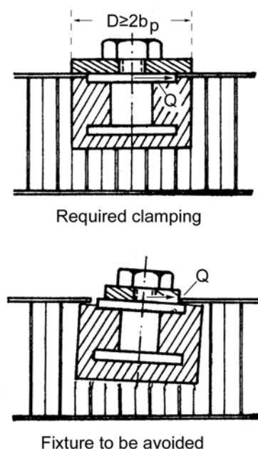
Figure 14-1: Shear-loaded inserts: Clamping conditions
