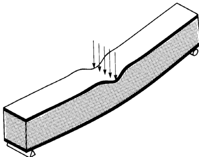
Figure 8-6: Schematic of 'local' bending effects in sandwich beam subjected to 3-point bending
