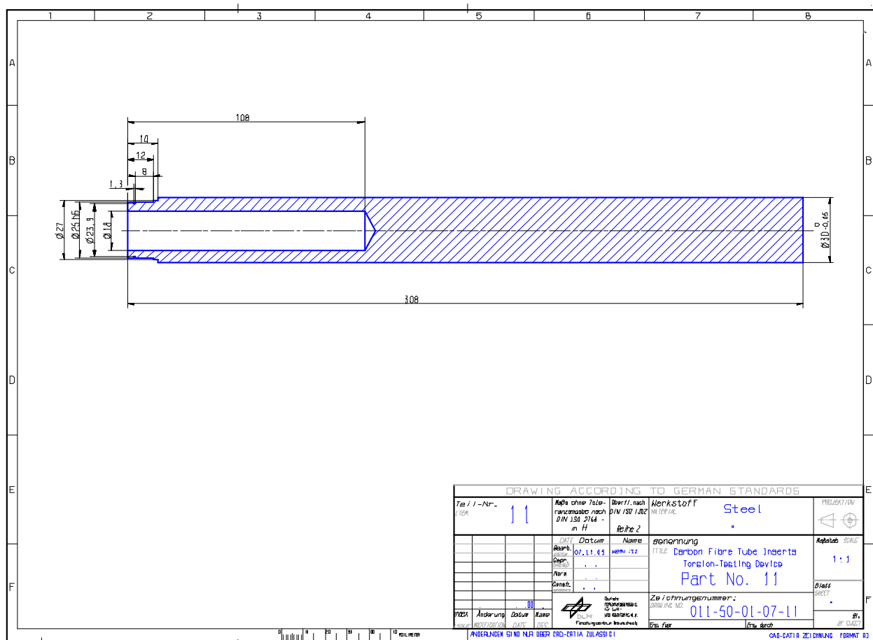
Figure H-42: Test fixture: Torsion – part 11
