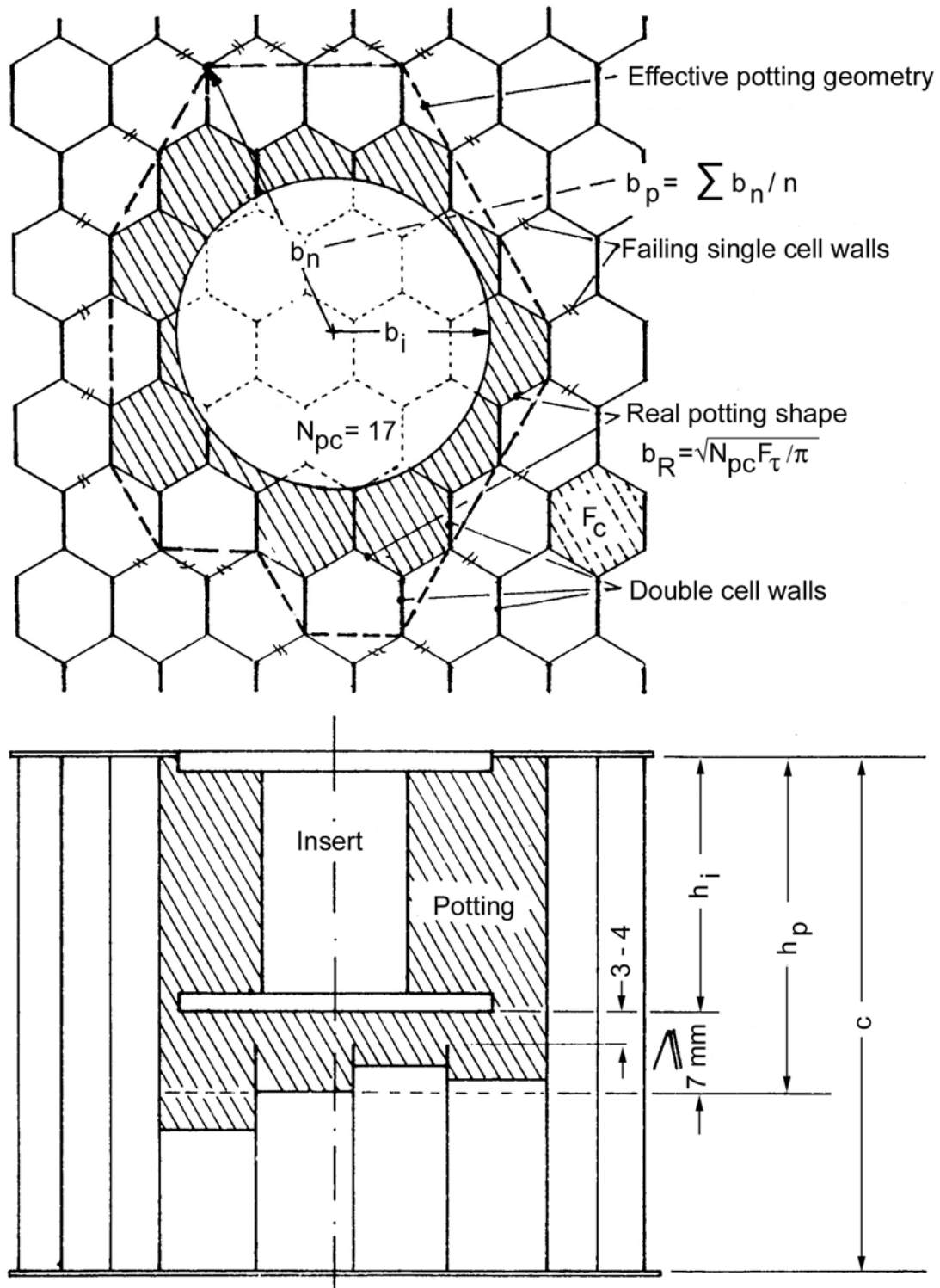
Figure 7-1: Potting geometry
