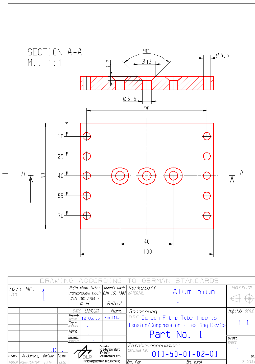
Figure H-2: Test fixture: Tension-compression load – part 1
