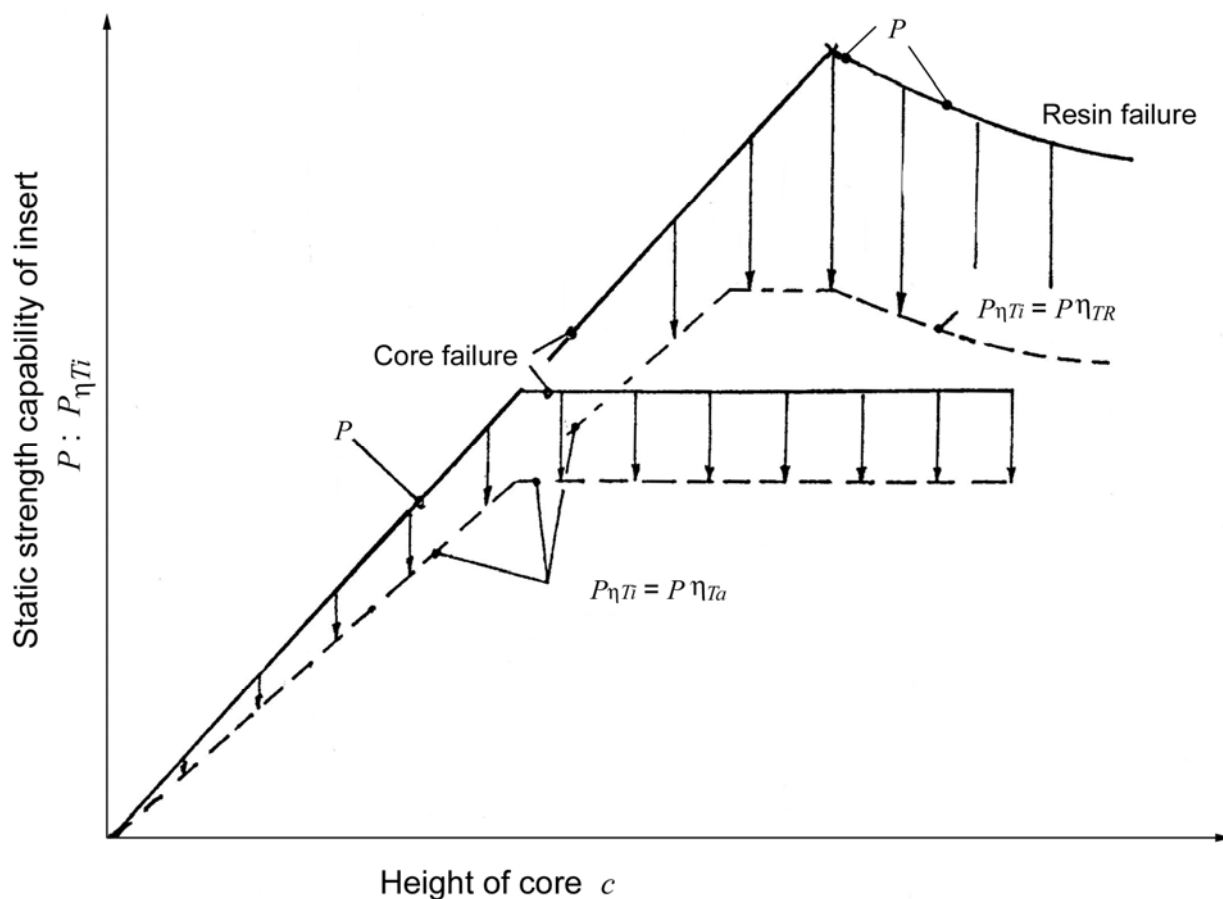
Figure 22-3: Thermal effects: Coefficient of thermal degradation
