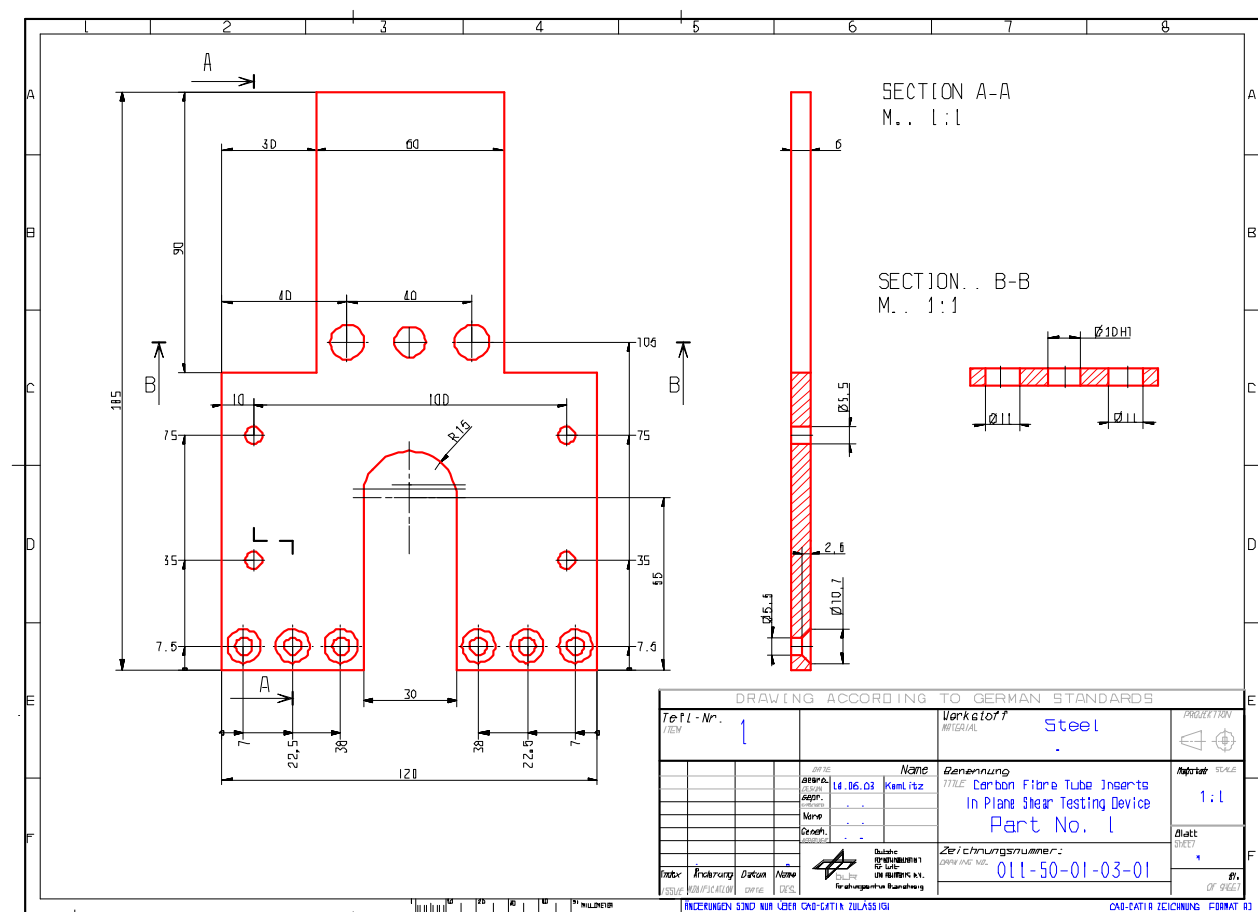
Figure H-10: Test fixture: In-plane shear load – part 1
