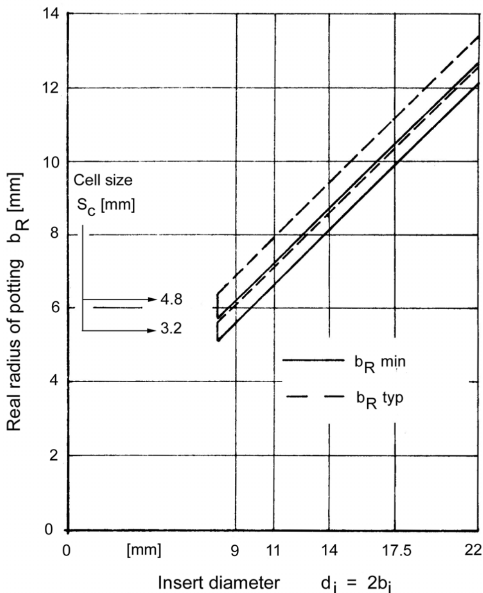
Figure 7-3: Real potting radius as a function of insert diameter
