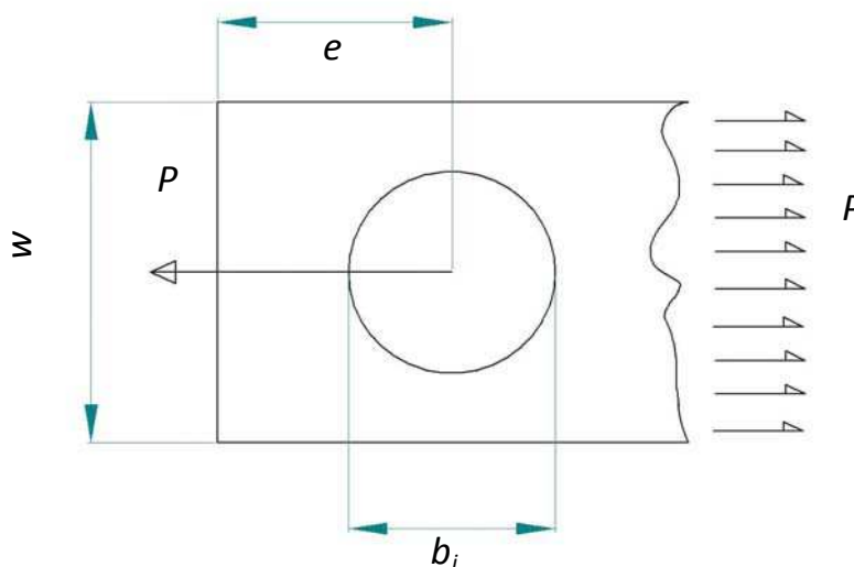
Figure 14-4: Nomenclature: Ultimate in-plane load against failure in tension
