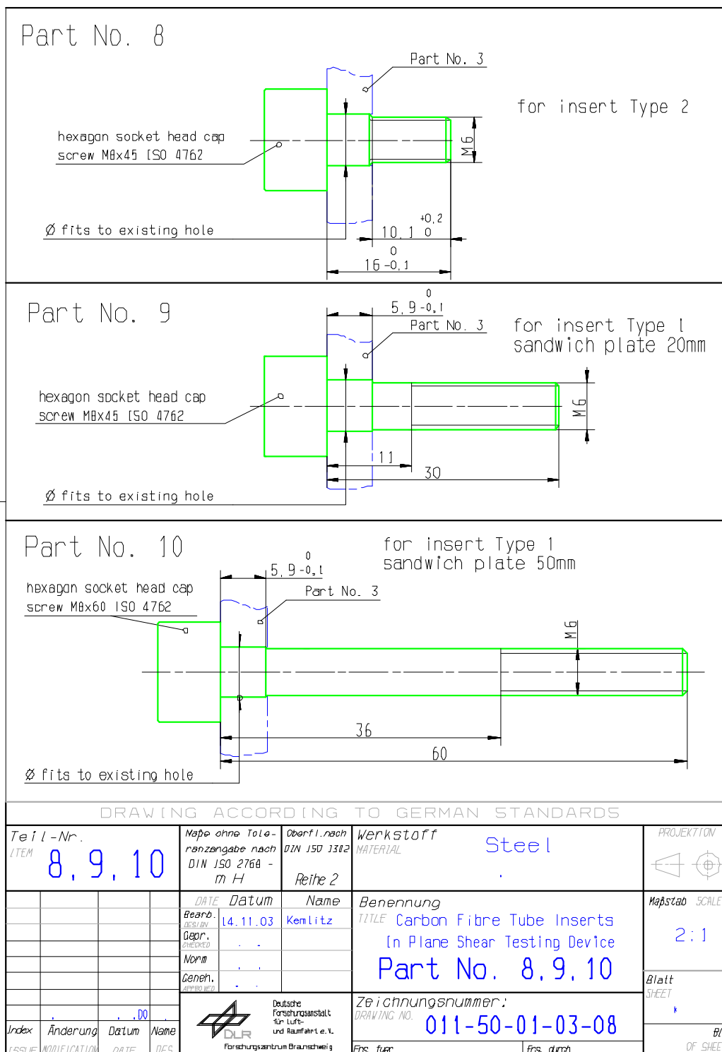
Figure H-17: Test fixture: In-plane shear load – part 8
