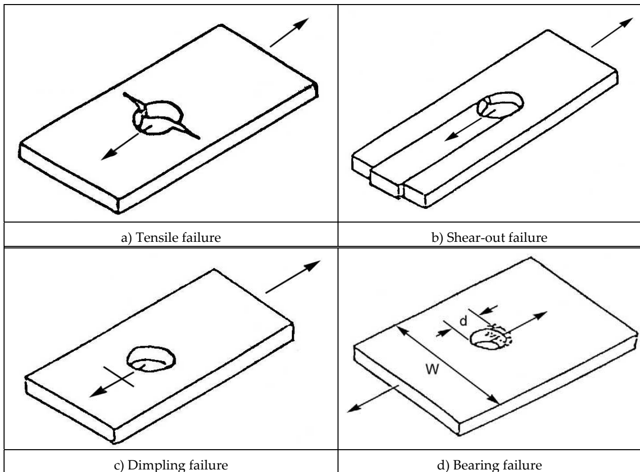
Figure 6-3: Possible failures modes: Anisotropic face sheets under shear-loading
