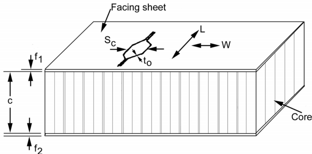
Figure 6-1: Sandwich and core: designation
