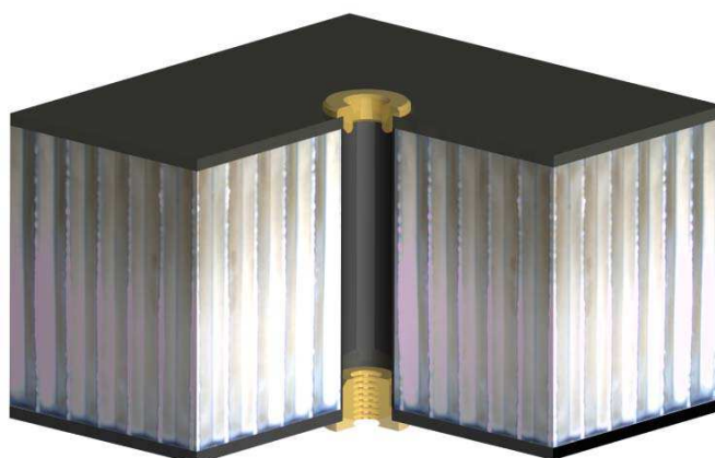
Figure A-3: Carbon fibre tube insert: Type 1 cap
