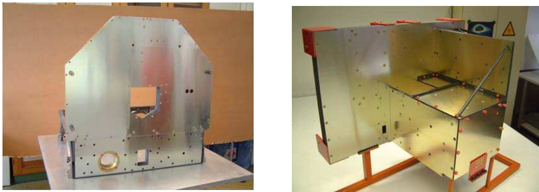
Figure F-11: ROSETTA Lander: Two structural components
