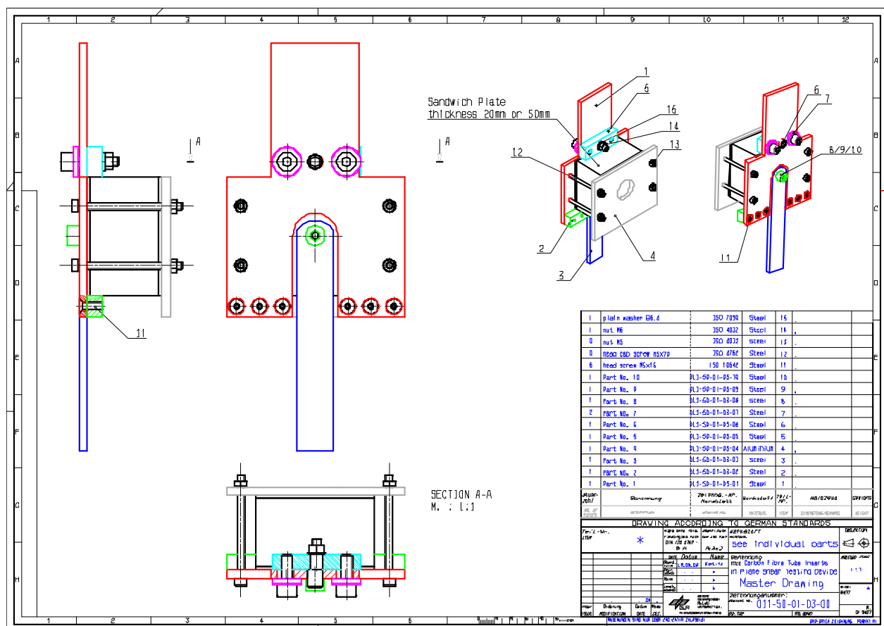
Figure H-9: Test fixture: In-plane shear load – master drawing
