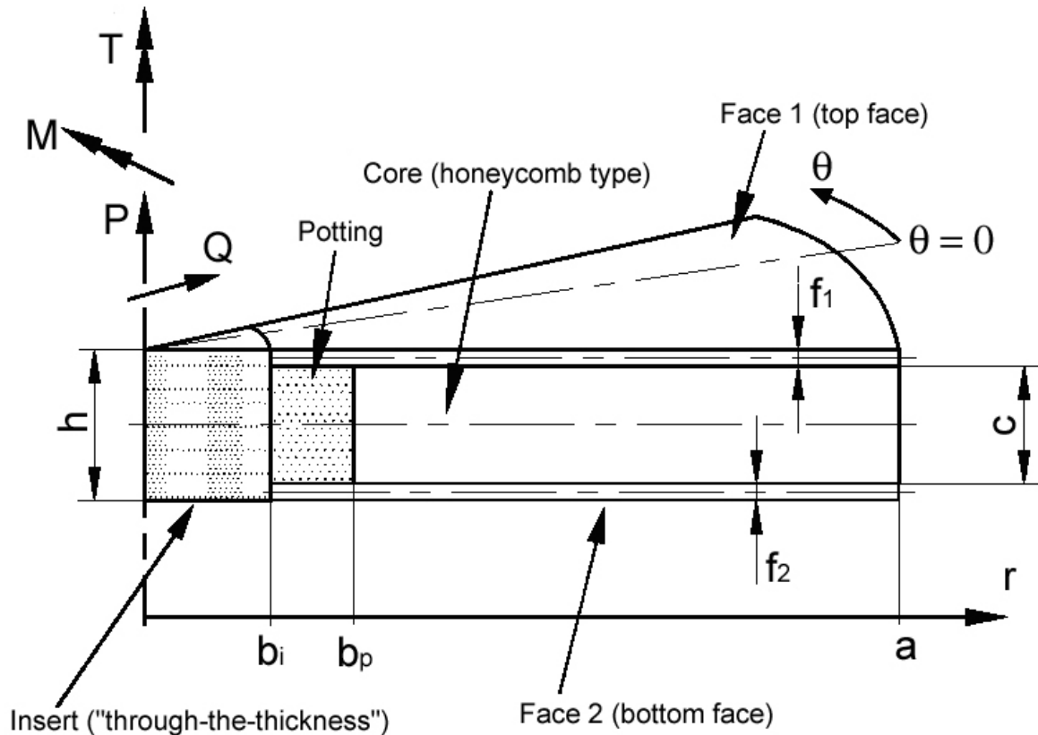
Figure 8-8: Model definition of sandwich plate with 'through-the-thickness' insert
