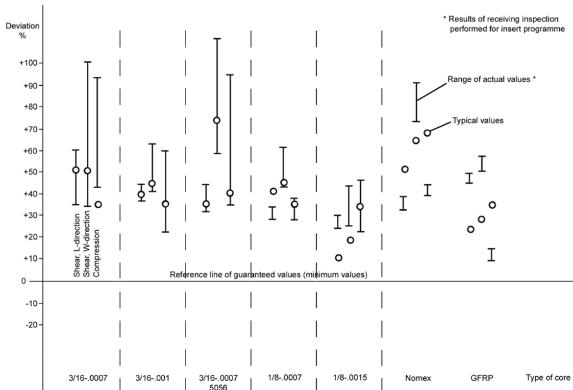
Figure 6-4: Core strength: Deviation (%) of actual strength from guaranteed values
