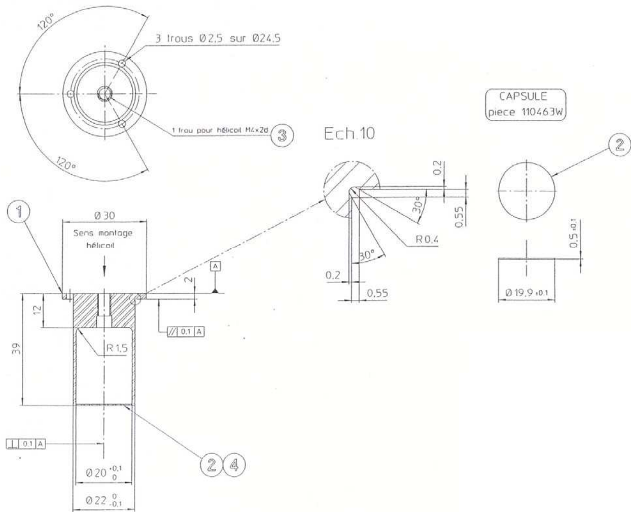
Figure F-21: Case study: HRG - Insert
