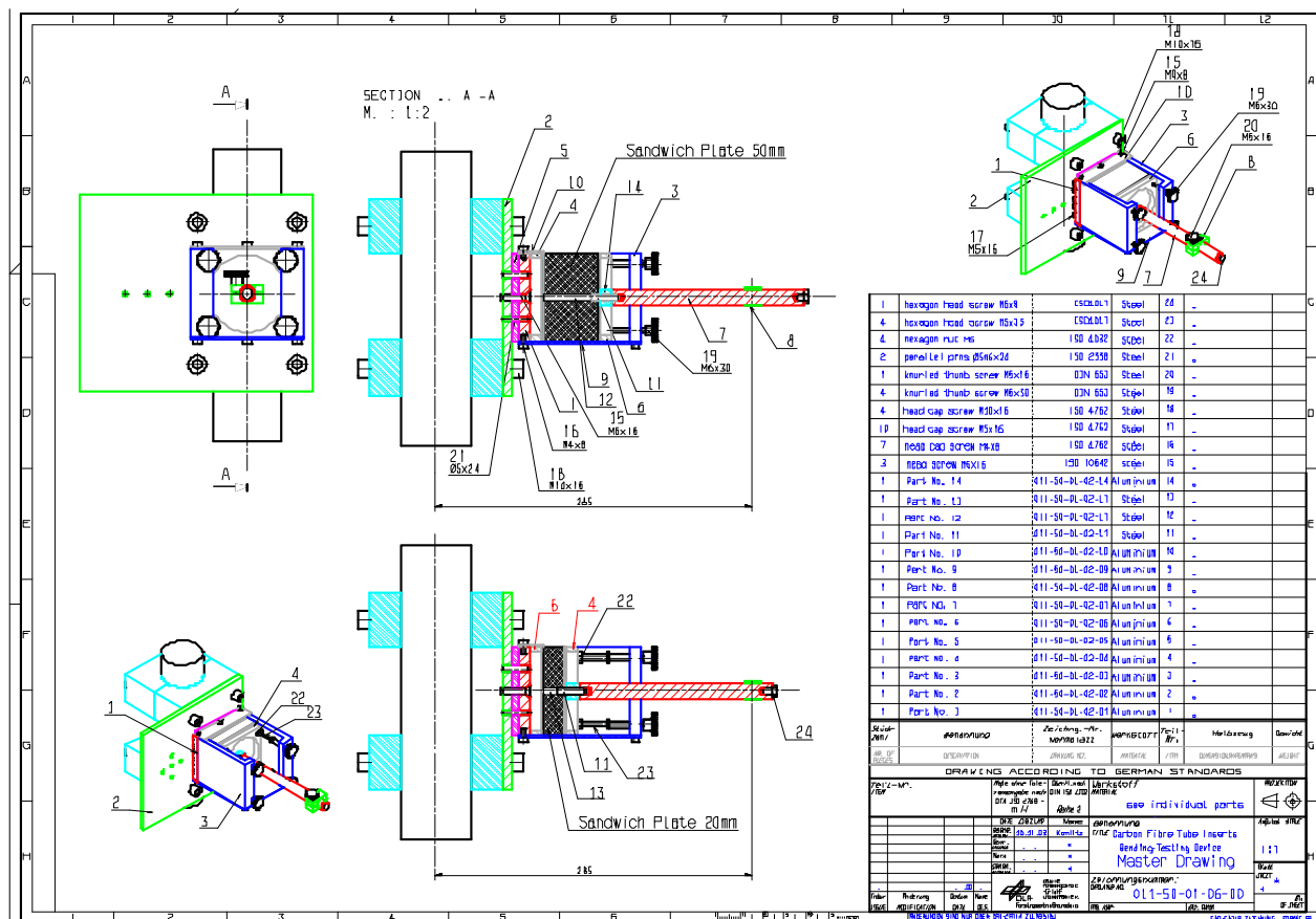
Figure H-18: Test fixture: Bending – master drawing
