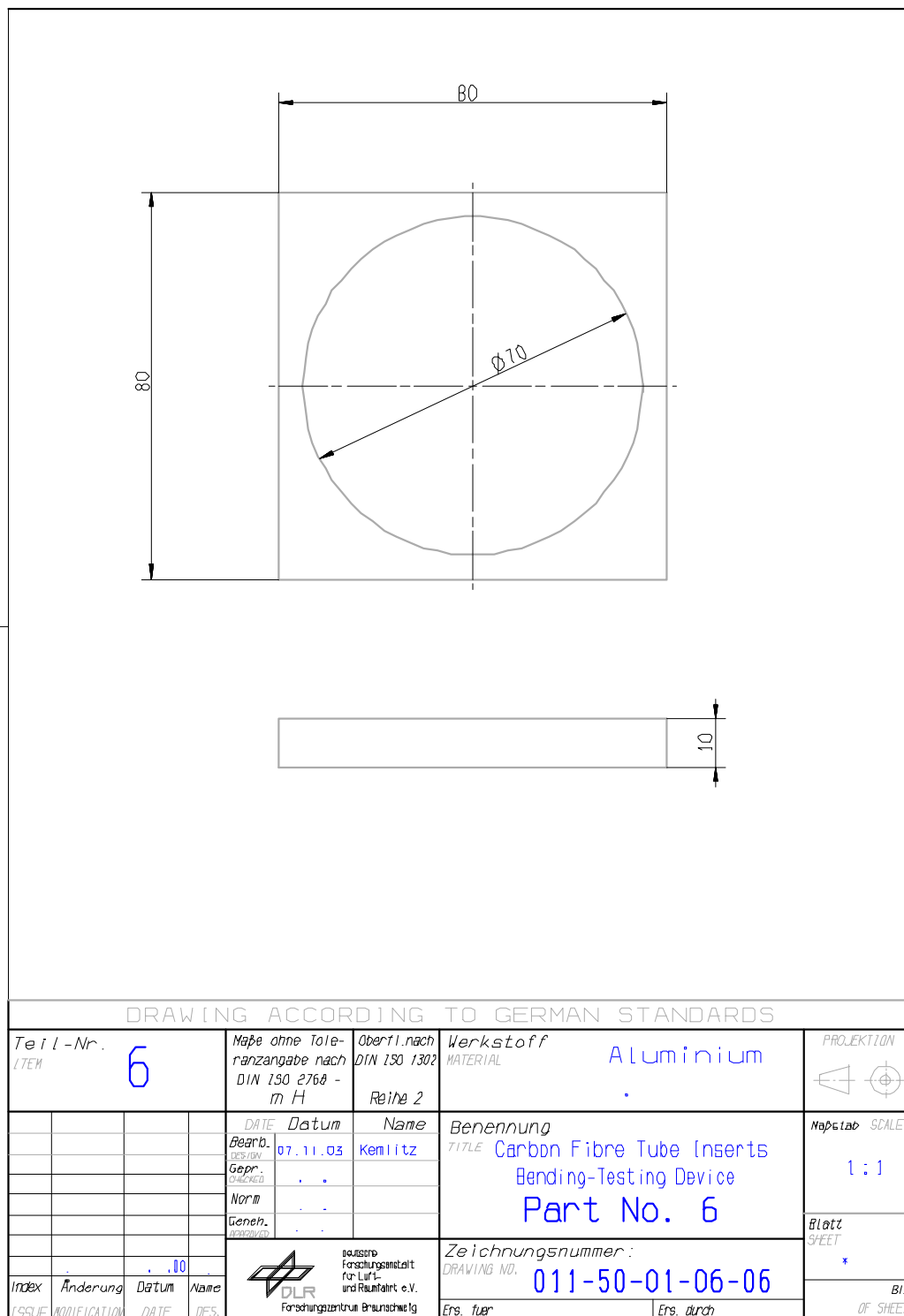
Figure H-24: Test fixture: Bending – part 6
