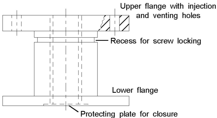
A – Typical standard-type insert
