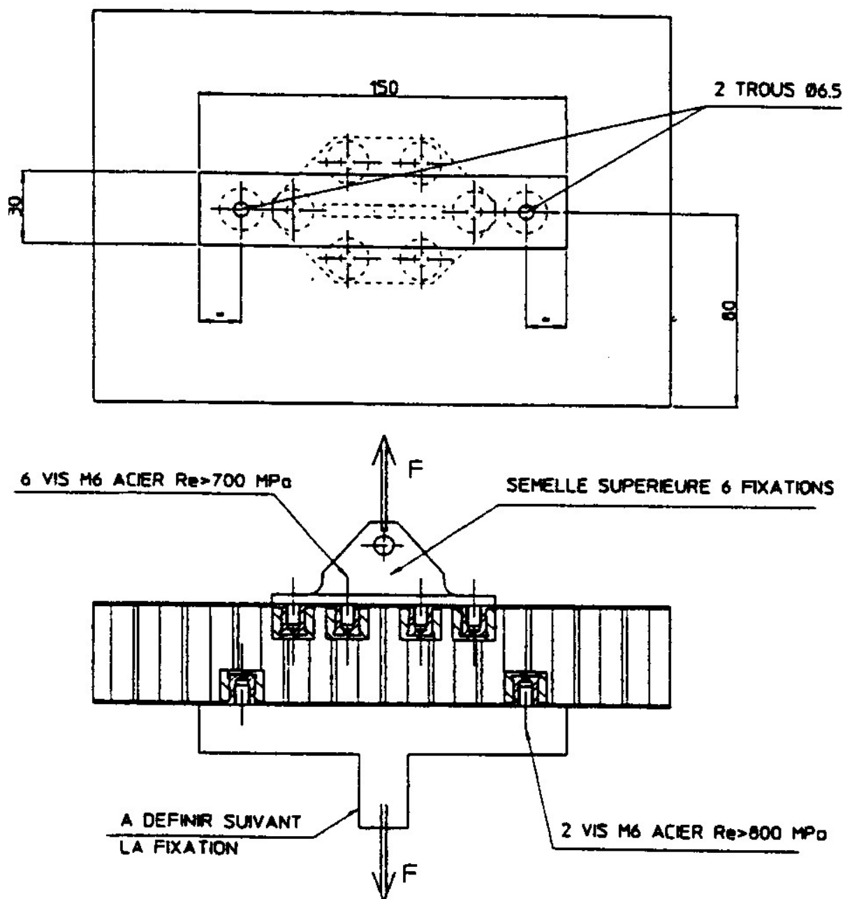
Figure F-8: Case study: ASAP 4 (AR4) - tensile (pull-out) method A
