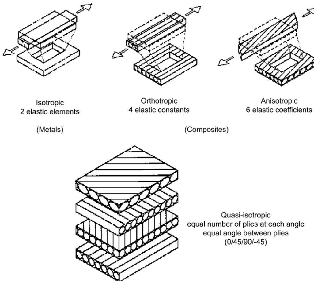
Figure 6-2: Face sheet properties: Isotropic, anisotropic and quasi-isotropic characteristics
