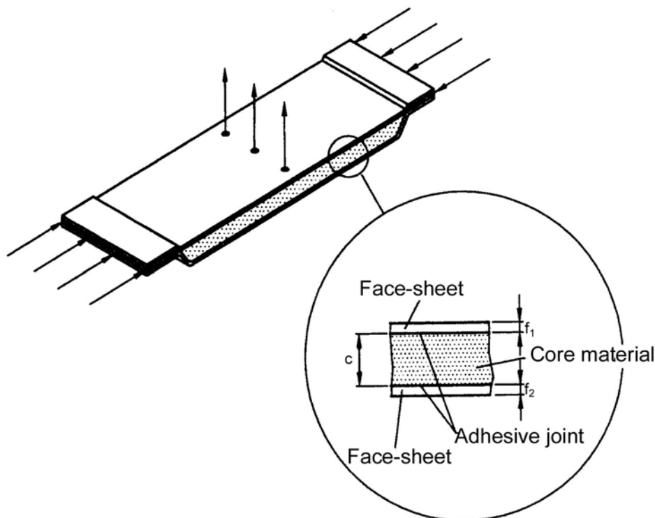
Figure 8-1: Schematic of structural sandwich panel subjected to both in-plane and out-of-plane external loading
