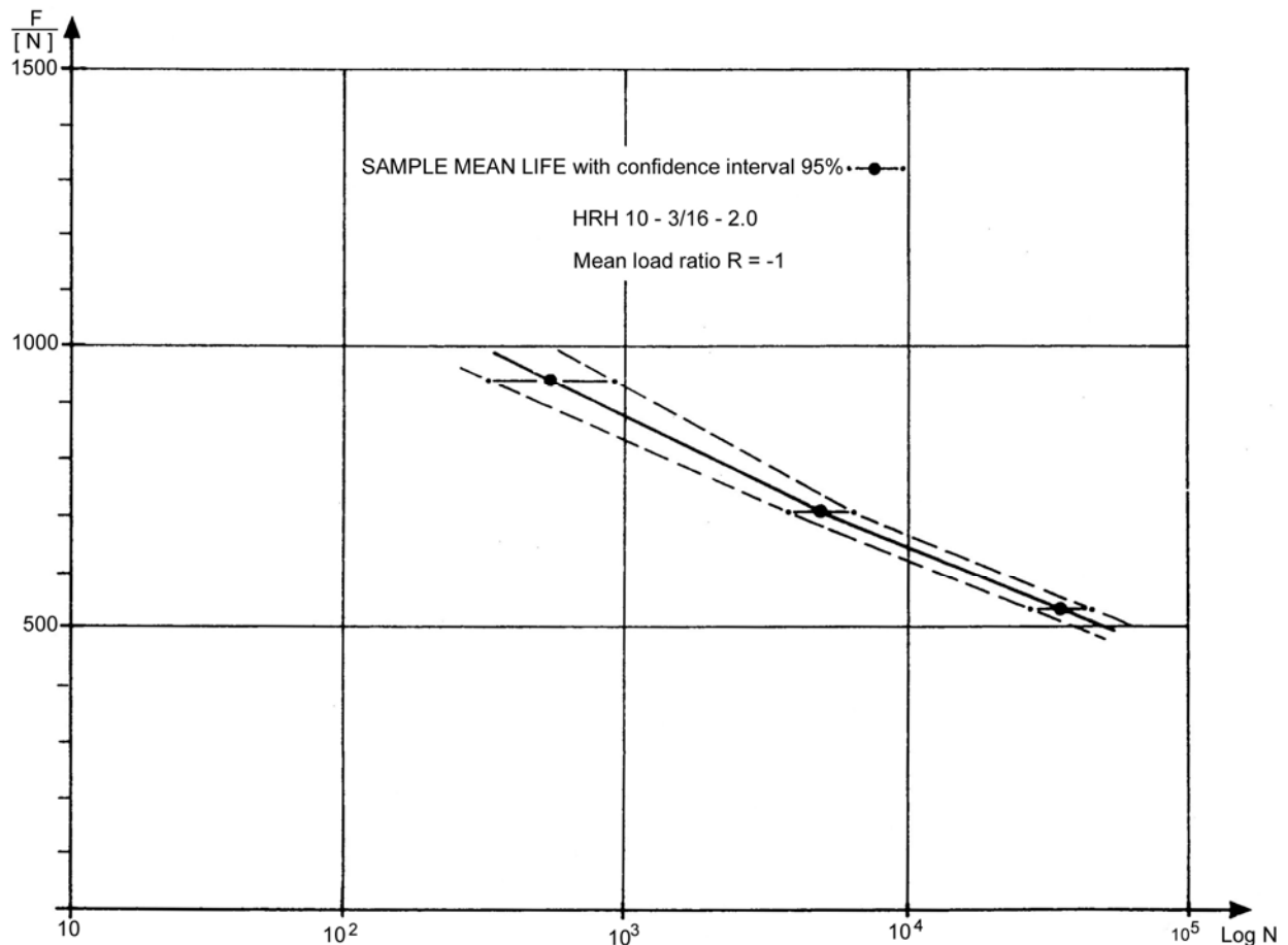
Figure 21-9: Fatigue life: Non-metallic Nomex® core
