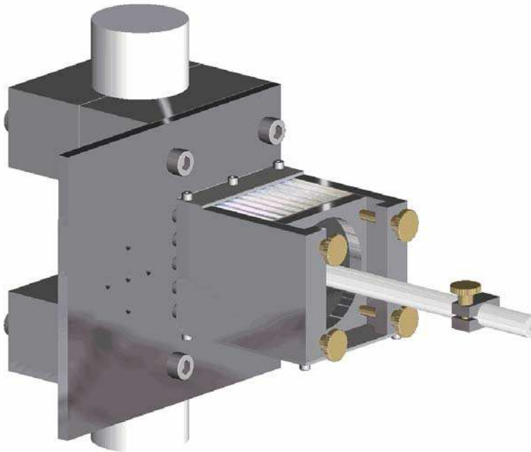
Figure 27-4: Manufacture control: Bending test fixture
