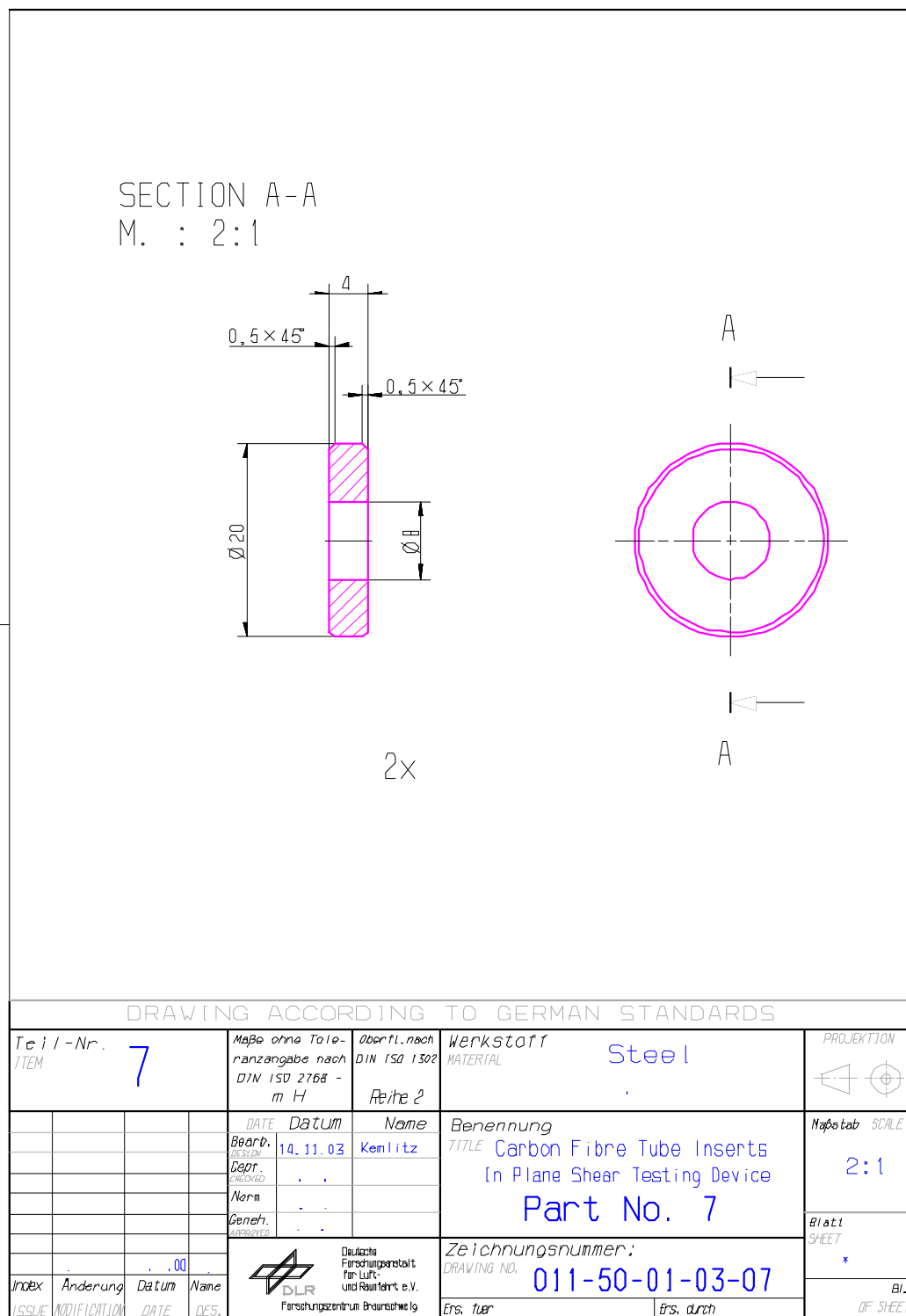
Figure H-16: Test fixture: In-plane shear load – part 7
