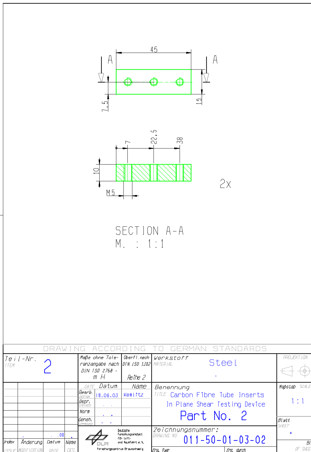
Figure H-11: Test fixture: In-plane shear load – part 2
