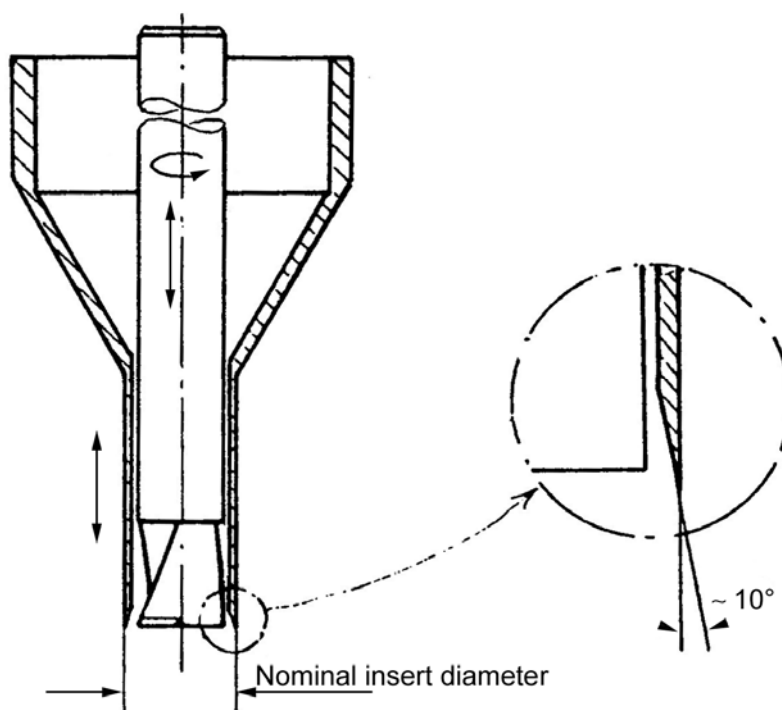
Figure 24-1: Sandwich panel machining: Combined drill and punch tool
