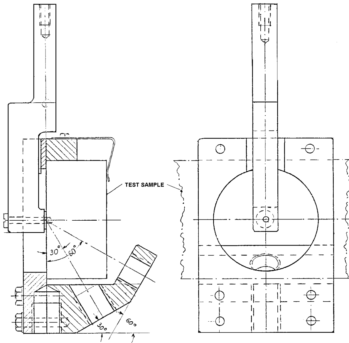
Figure 29-2: Testing: Insert static in-plane strength fixture
