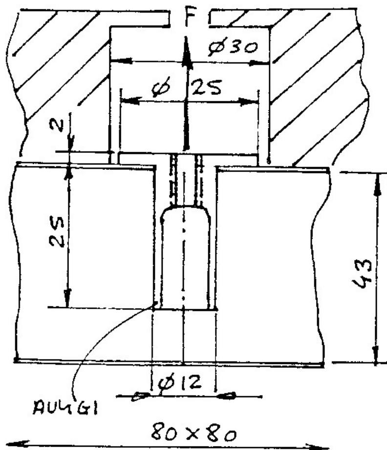
Figure F-22: Case study: HRG - Test method
