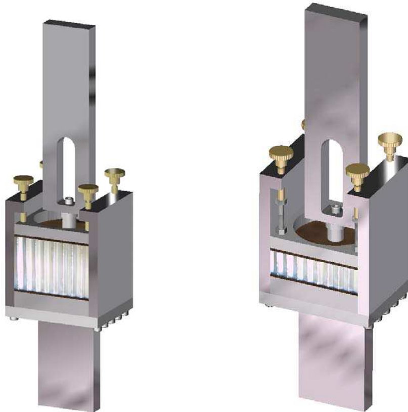
Figure 27-2: Manufacture control: Out-of-plane test fixture for compression or fatigue tests
