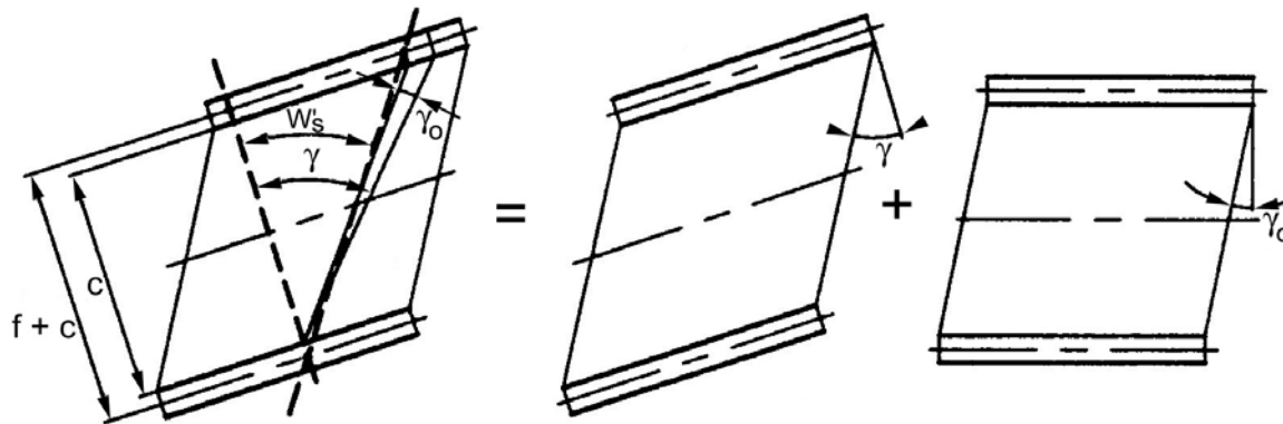
Figure 8-4 Shearing deformation of sandwich beam element
