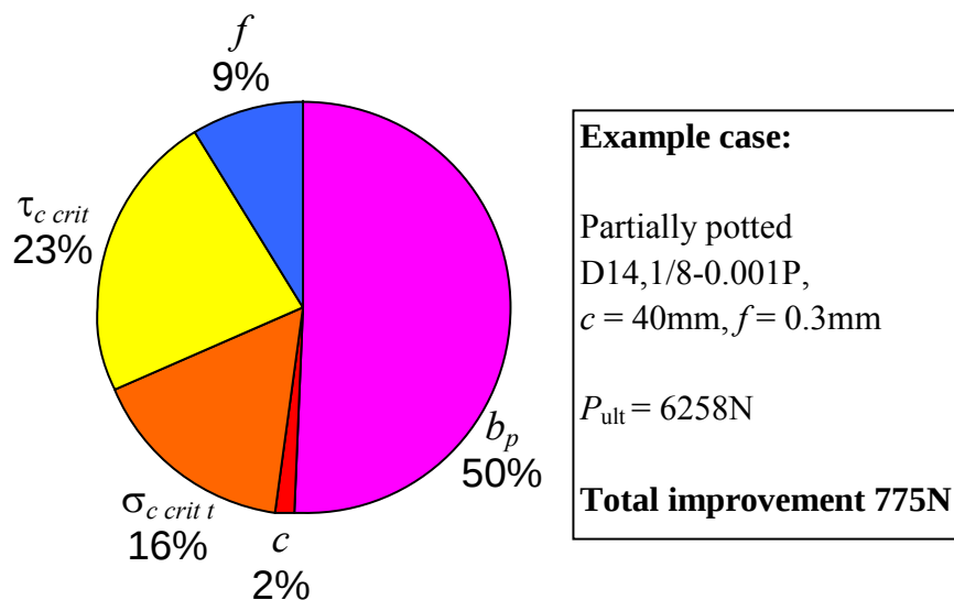
Figure 12-3: Out-of-plane capability: Contributions of the main components on improved core tension
