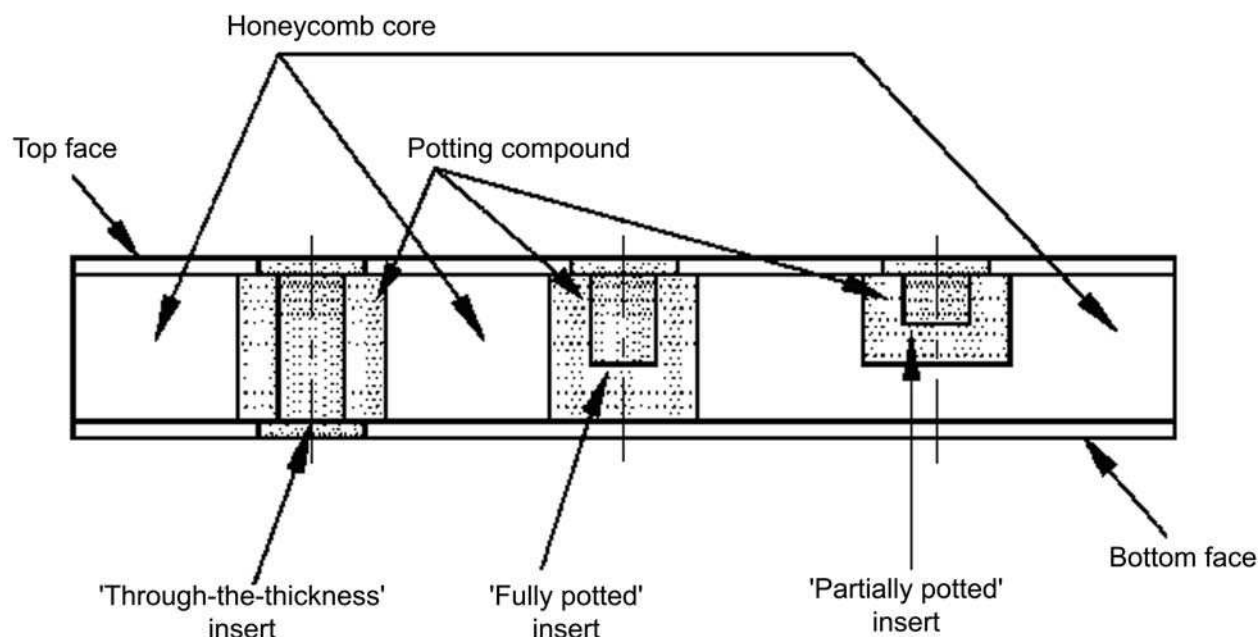
Figure 8-7: Schematic of potted insert types for sandwich panels used for spacecraft applications
