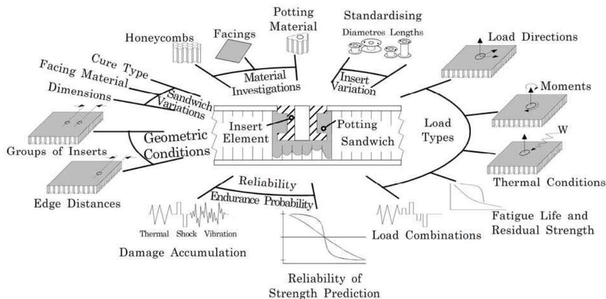
Figure 9-1: Basic aspects of insert design, analysis and testing
