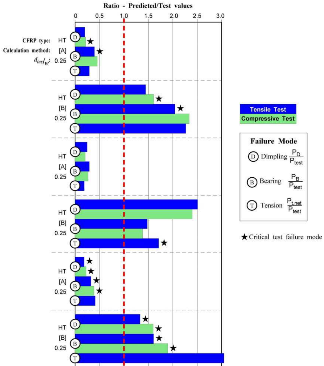
Figure 14-3: Correlation between calculated and tested in-plane capabilities with fibre strength
