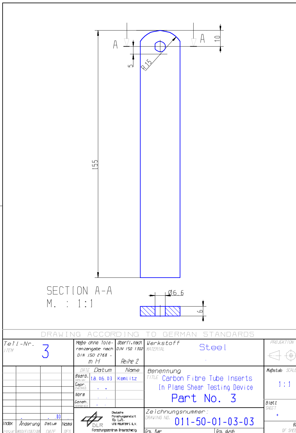
Figure H-12: Test fixture: In-plane shear load – part 3
