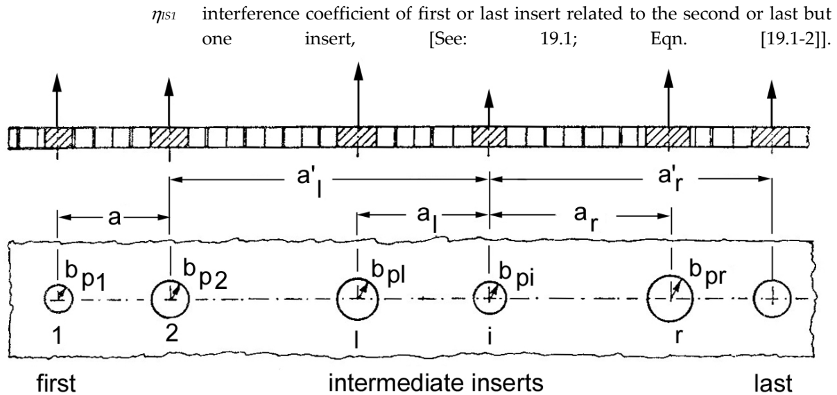
Figure 19-2: Insert groups: Series of inserts loaded in same direction
