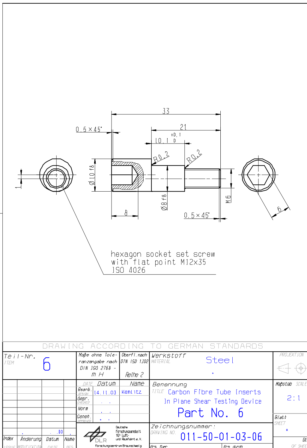
Figure H-15: Test fixture: In-plane shear load – part 6
