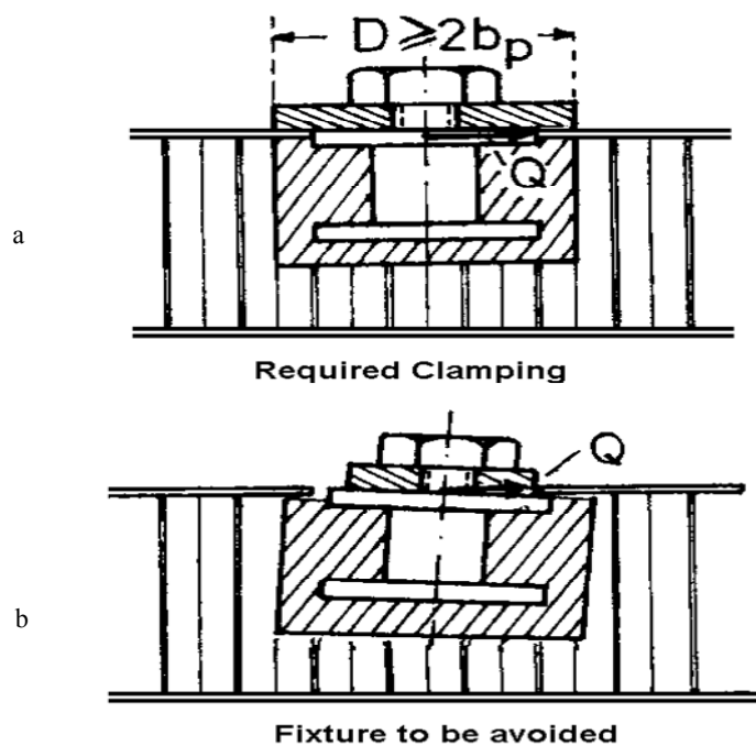
Figure 10-4: Insert design under in-plane load
