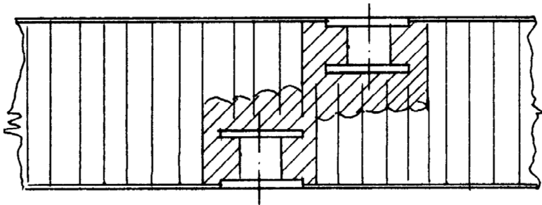
Figure 23-2: Inserts with connected potting mass
