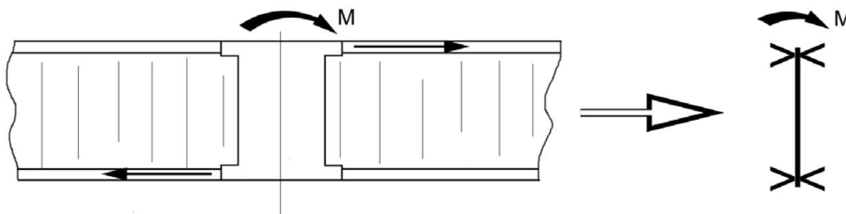
Figure 10-11: Pre-design: Through-the-thickness insert under bending
