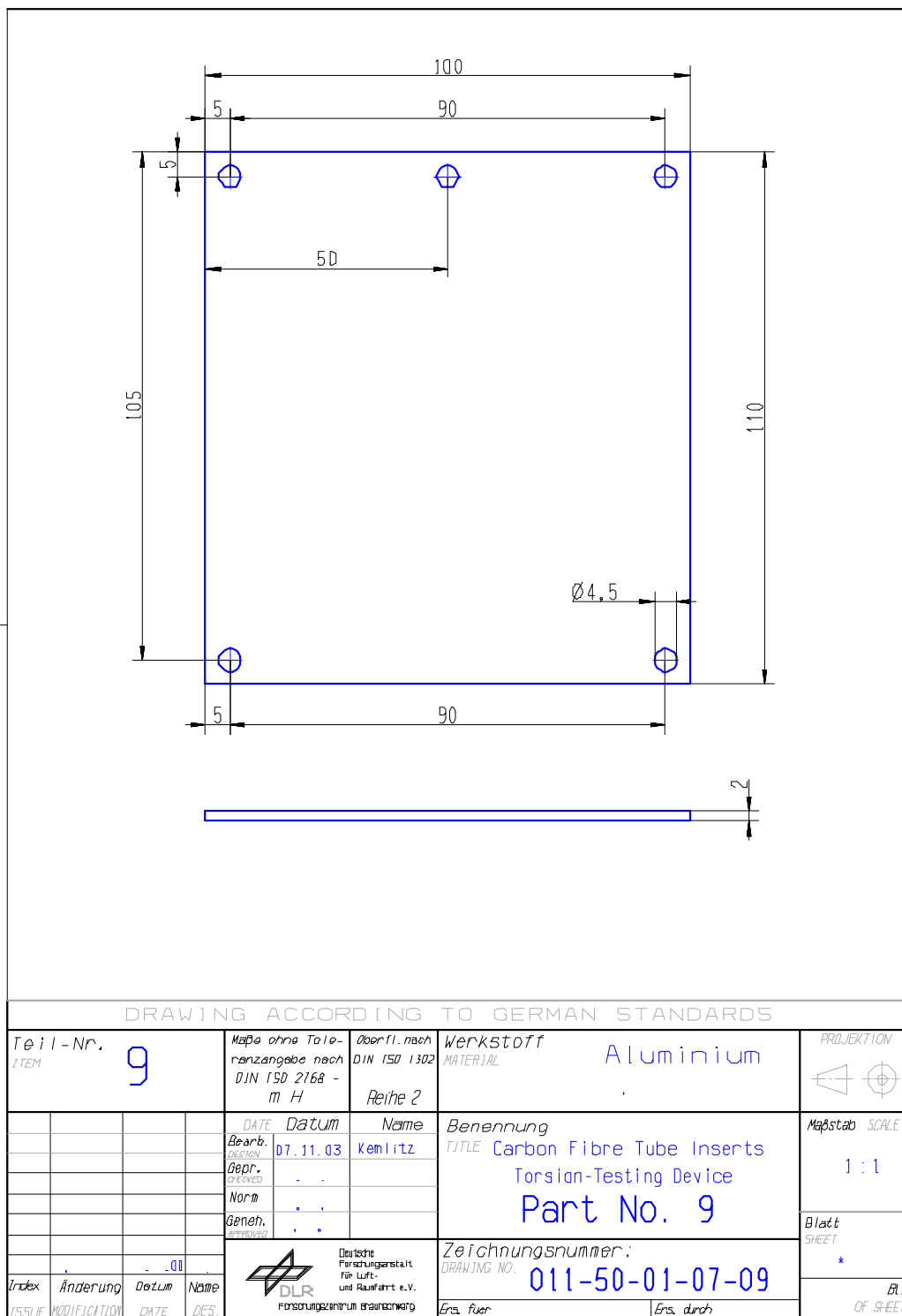
Figure H-40: Test fixture: Torsion – part 9
