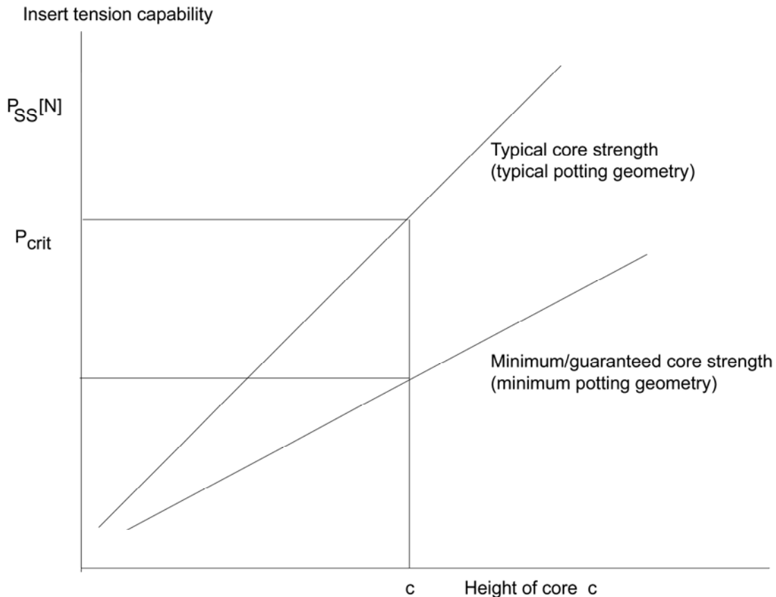
Figure 21-1: Static strength values with core height
