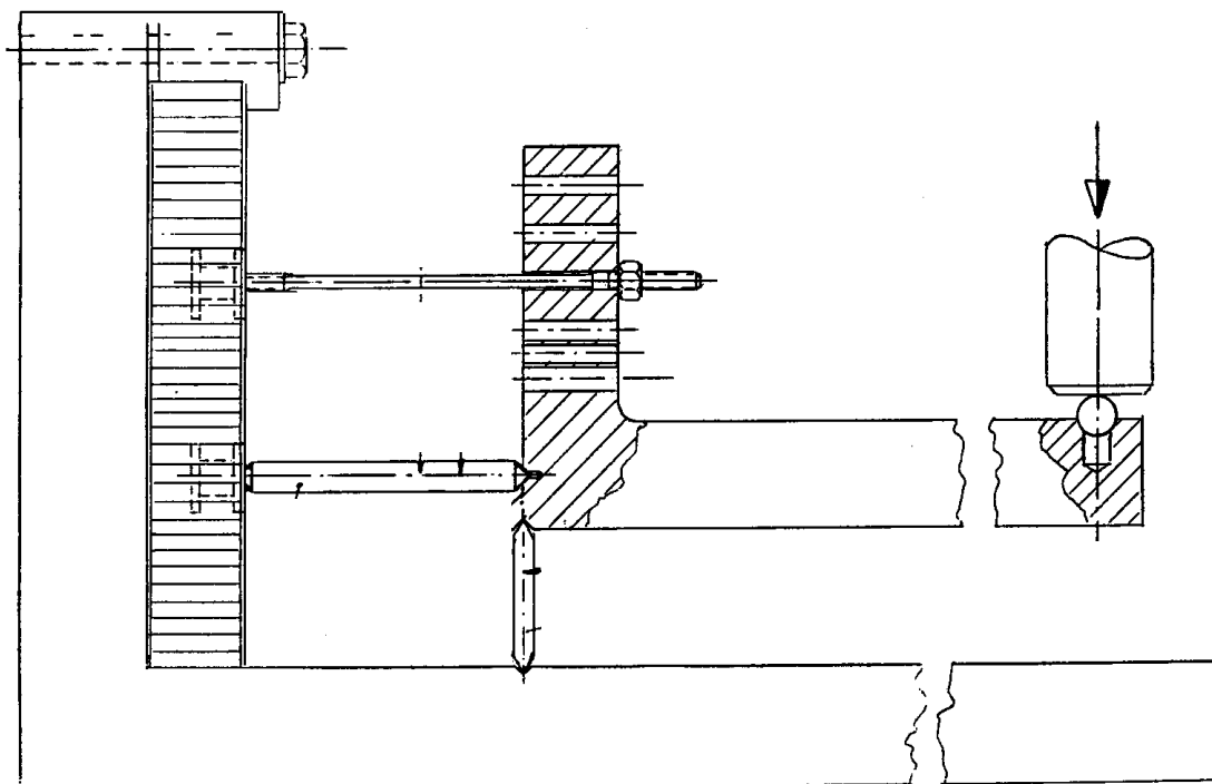
Figure 29-7: Testing: Insert proximity tensile-compression fixture
