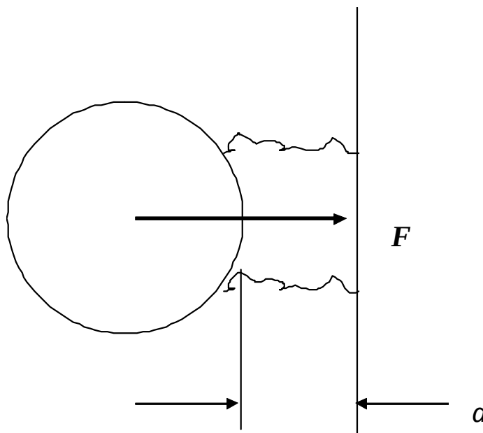
Figure 10-12: Pre-design: Face sheet shear-out failure mode
