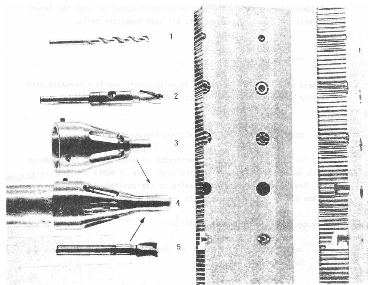
Figure 24-2 Sandwich panel machining: Series of single tools and their uses
