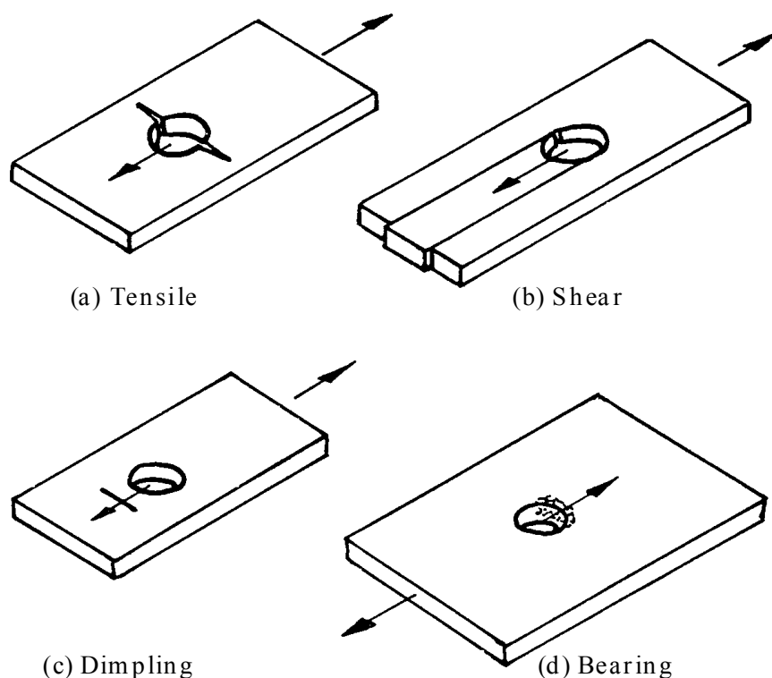
Figure 10-20: Failure modes: CFRP face sheets
