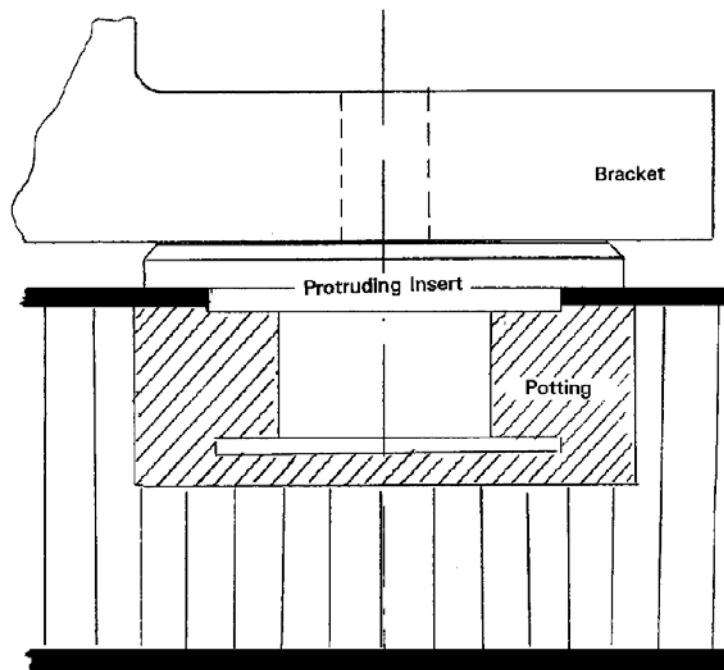
Figure 13-1: Compressive strength: Protruding insert
