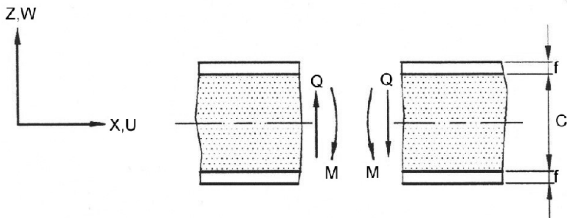
Figure 8-2: Sign conventions for sandwich beam element
