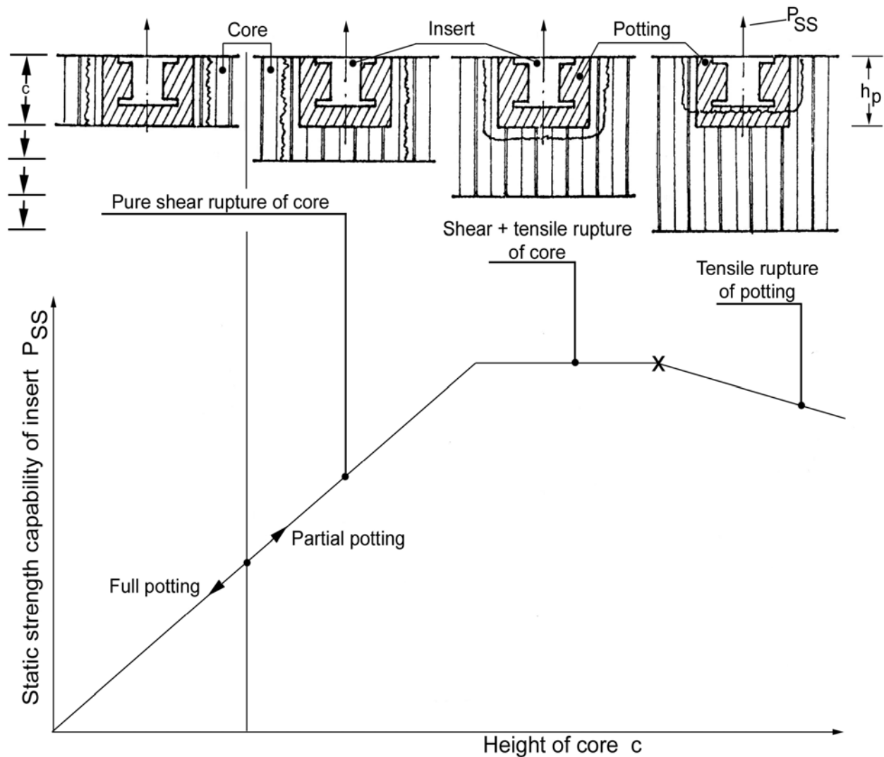
Figure 12-1: Failure modes in relation to the core height
