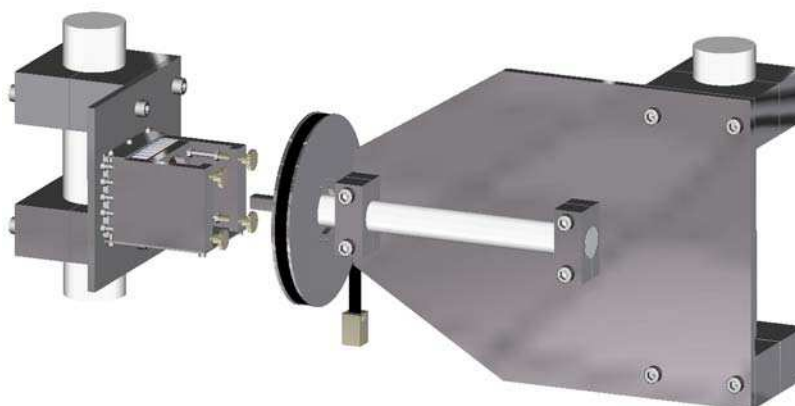
Figure 27-5: Manufacture control: Torsion test fixture
