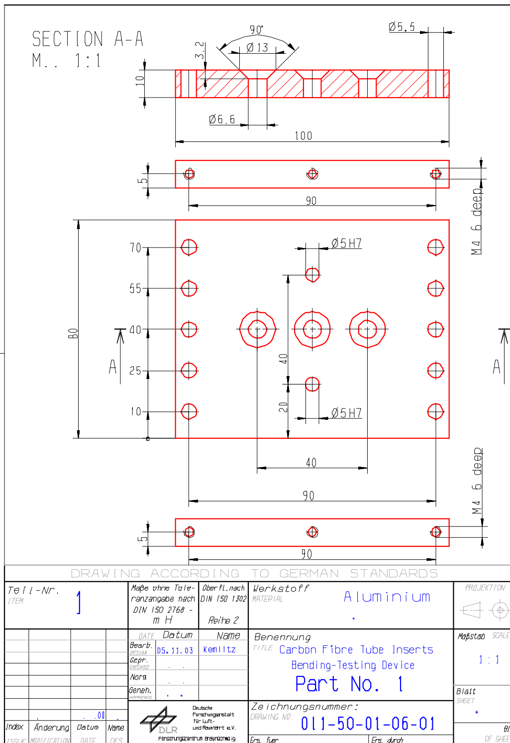
Figure H-19: Test fixture: Bending – part 1
