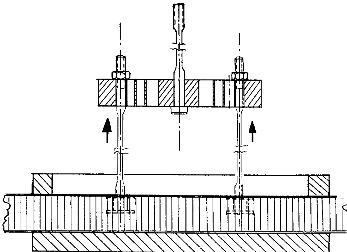
Figure 29-6: Testing: Insert proximity tensile fixture
