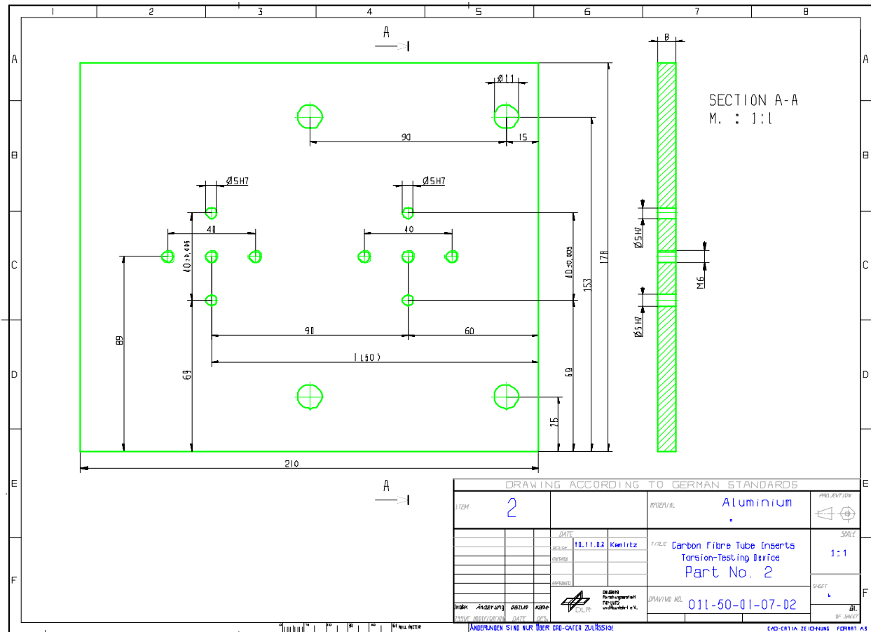
Figure H-33: Test fixture: Torsion – part 2
