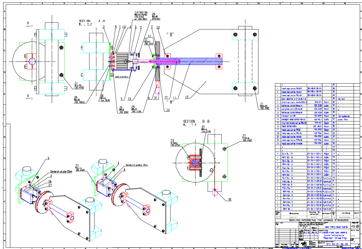
Figure H-31: Test fixture: Torsion – master drawing
