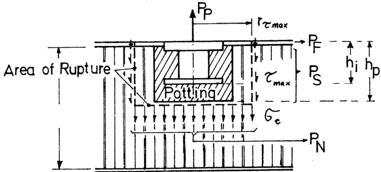
Figure C-2: Partially potted insert
