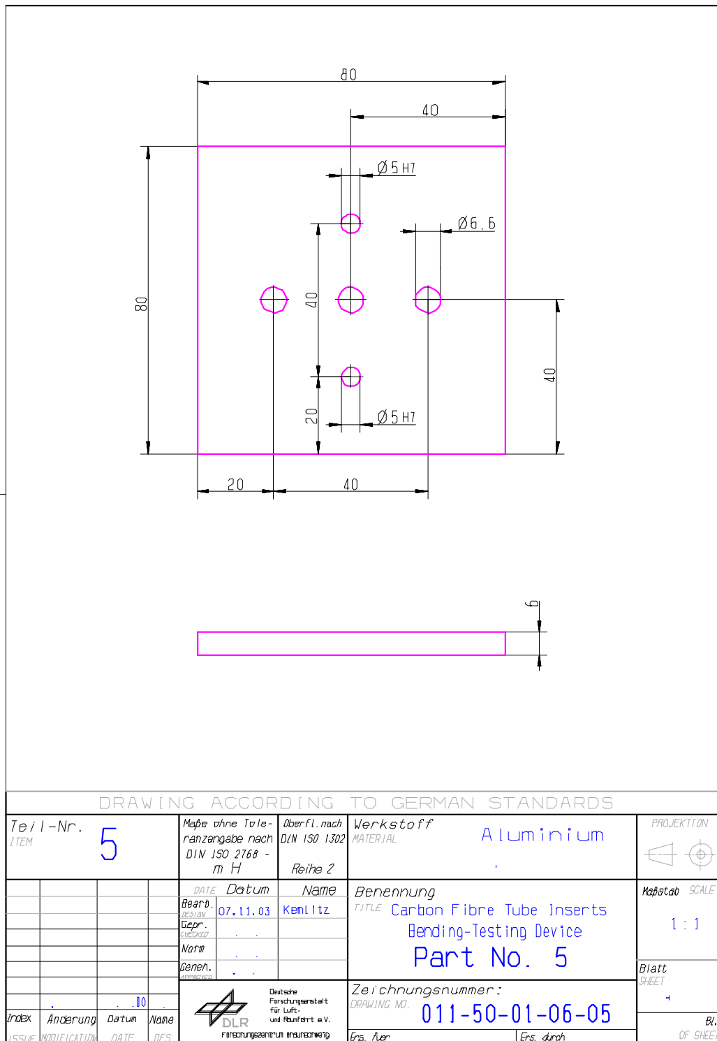
Figure H-23: Test fixture: Bending – part 5
