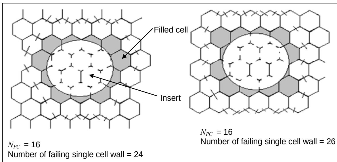
Figure 10-17: Failure modes: Non-correlation between number of the filled cells and number of the failing cell walls
