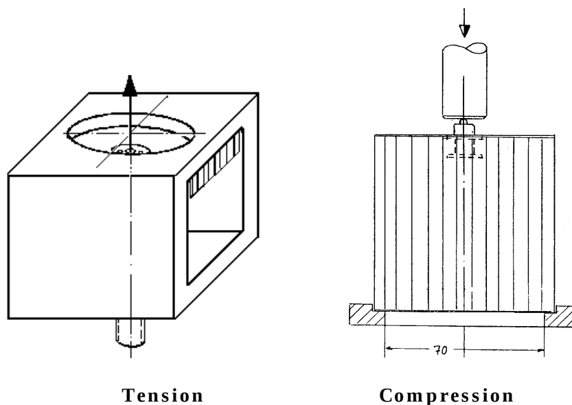
Figure 29-1: Testing: Insert static out-of-plane strength fixture
