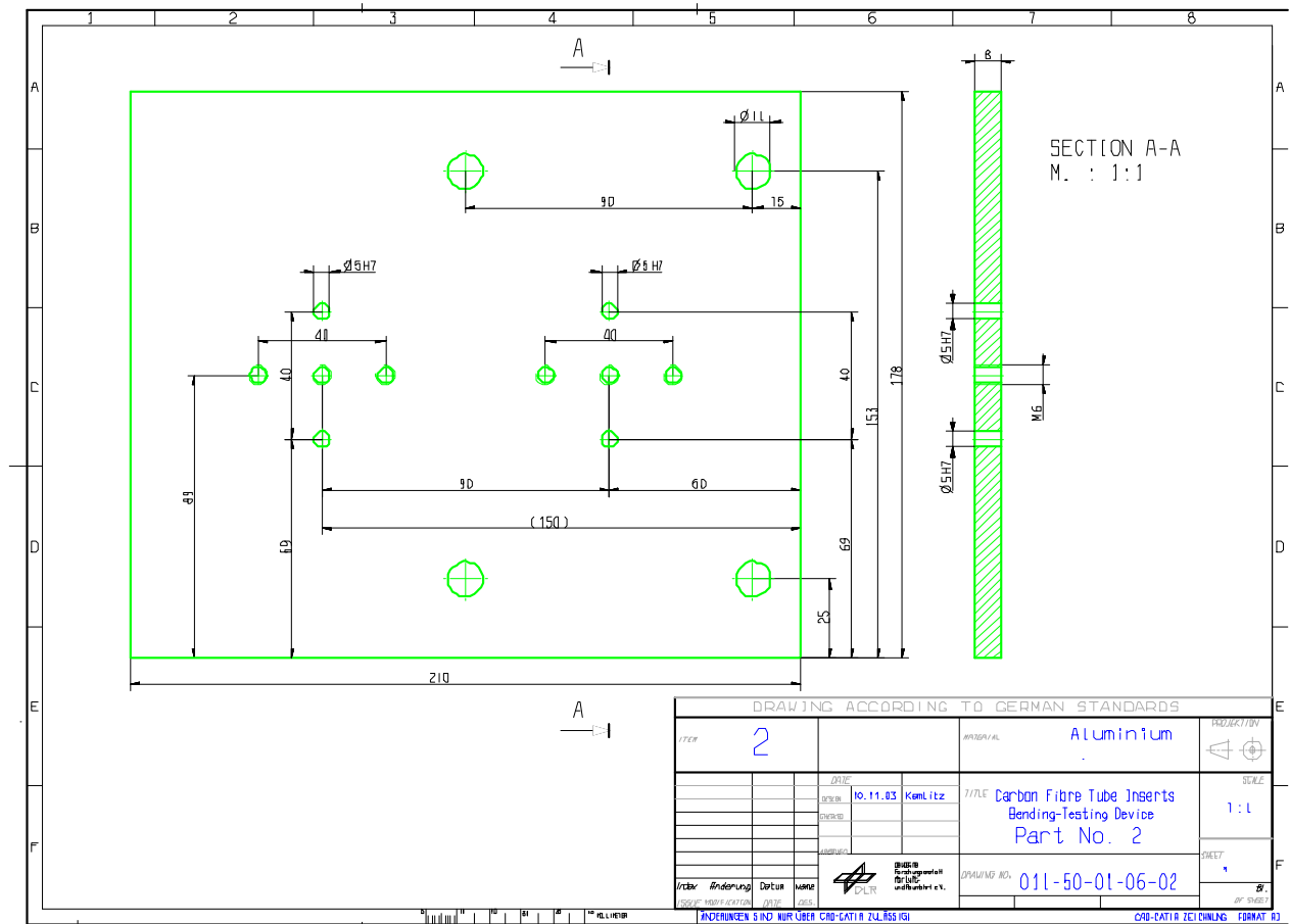
Figure H-20: Test fixture: Bending – part 2
