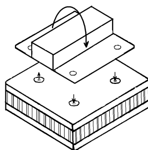
Figure 9-3: Insert out-of-plane load
