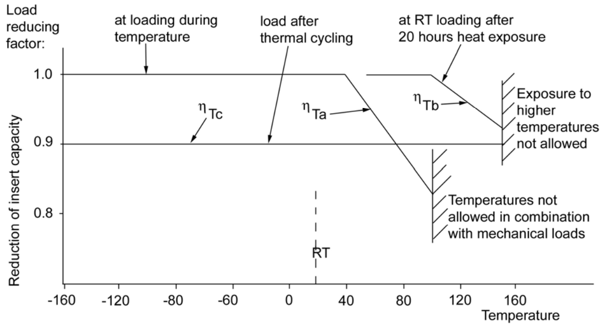
Figure 22-1: Thermal effects: Reduction of insert capability
