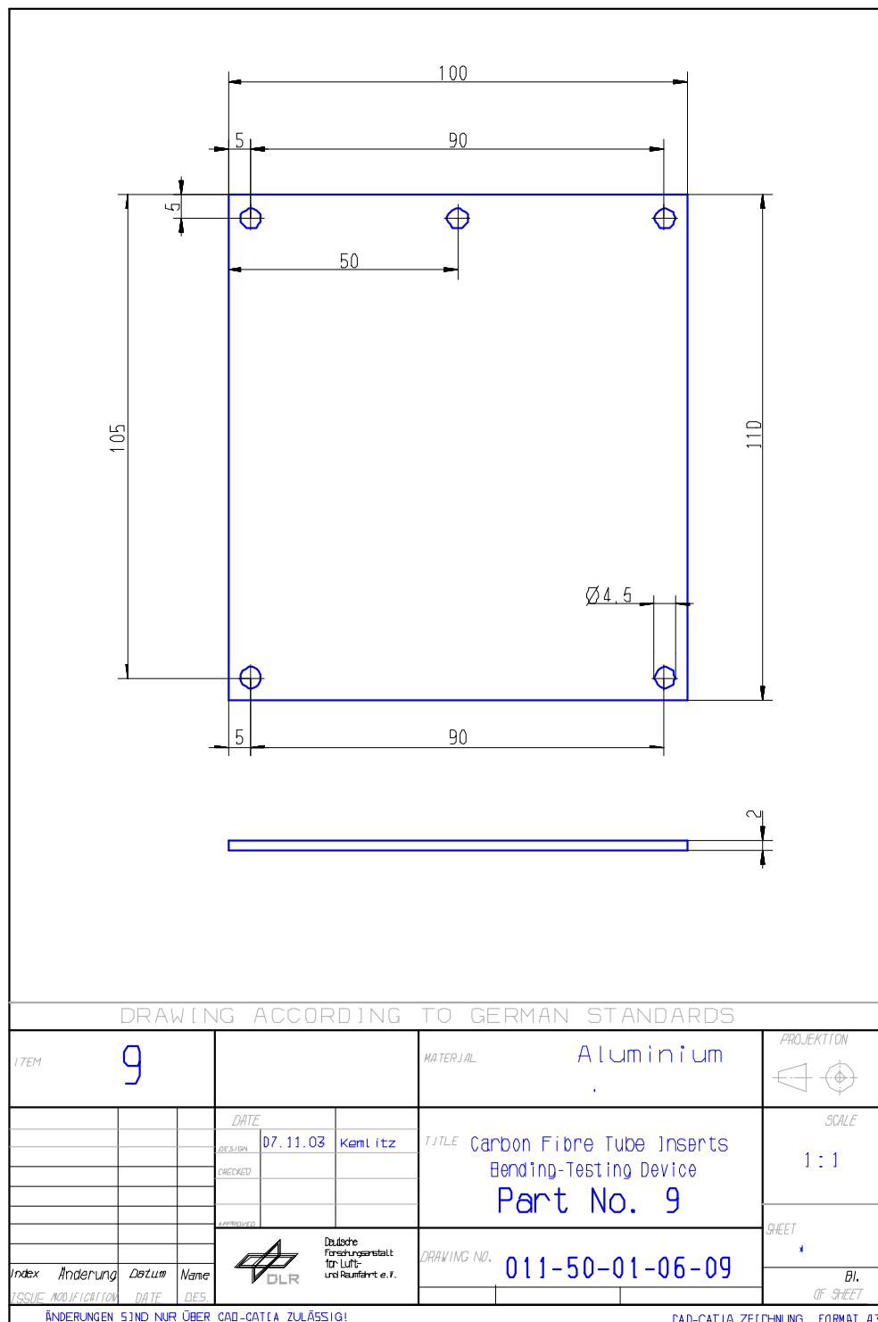
Figure H-27: Test fixture: Bending – part 9
