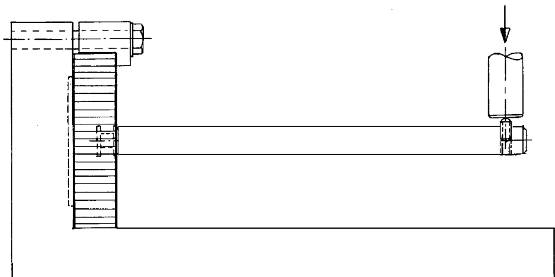
Figure 29-4: Testing: Bending fixture
