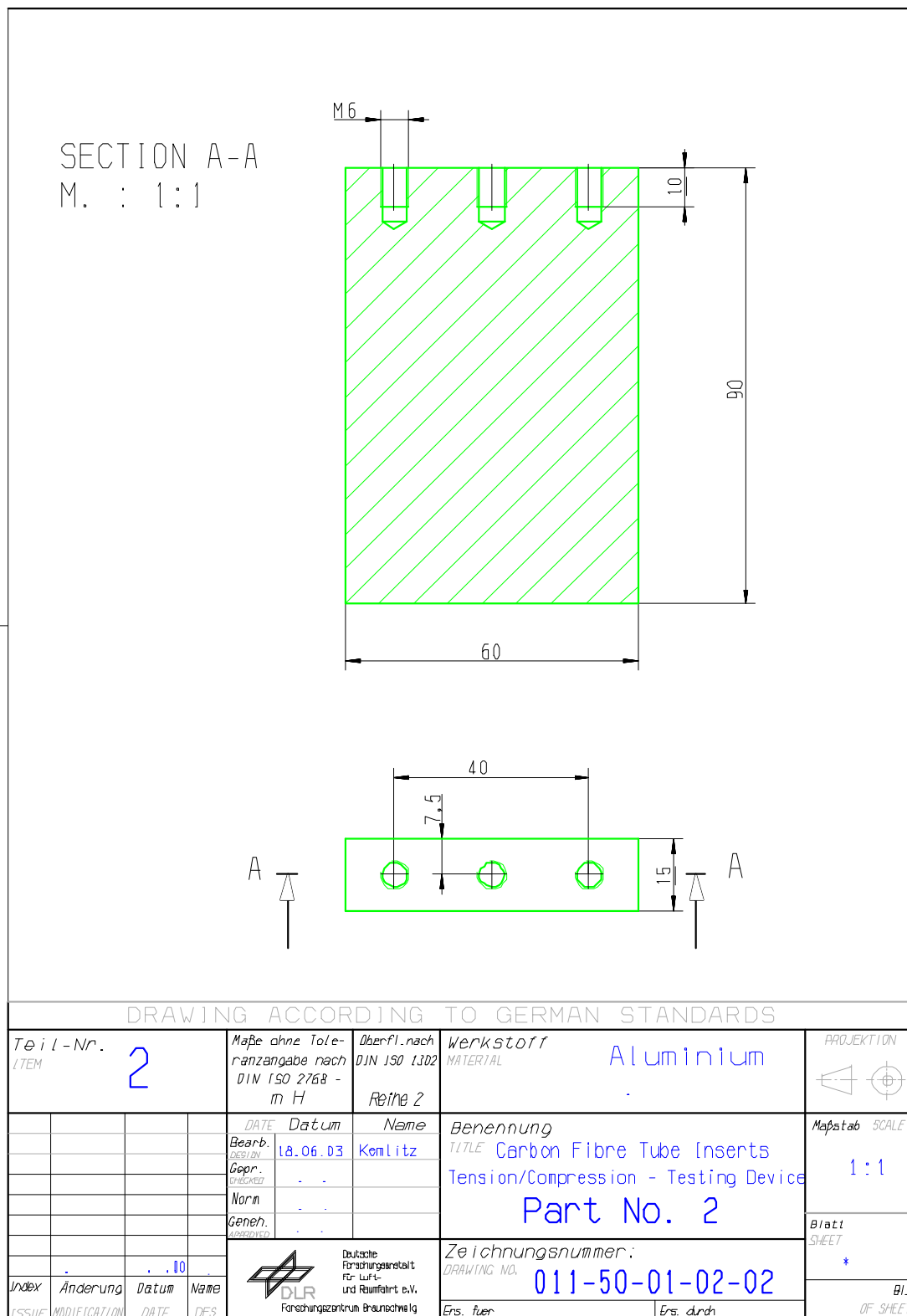
Figure H-3: Test fixture: Tension-compression load – part 2
