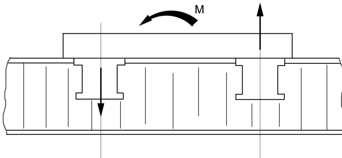
re 10-9: Selection of inserts: Partially potted
