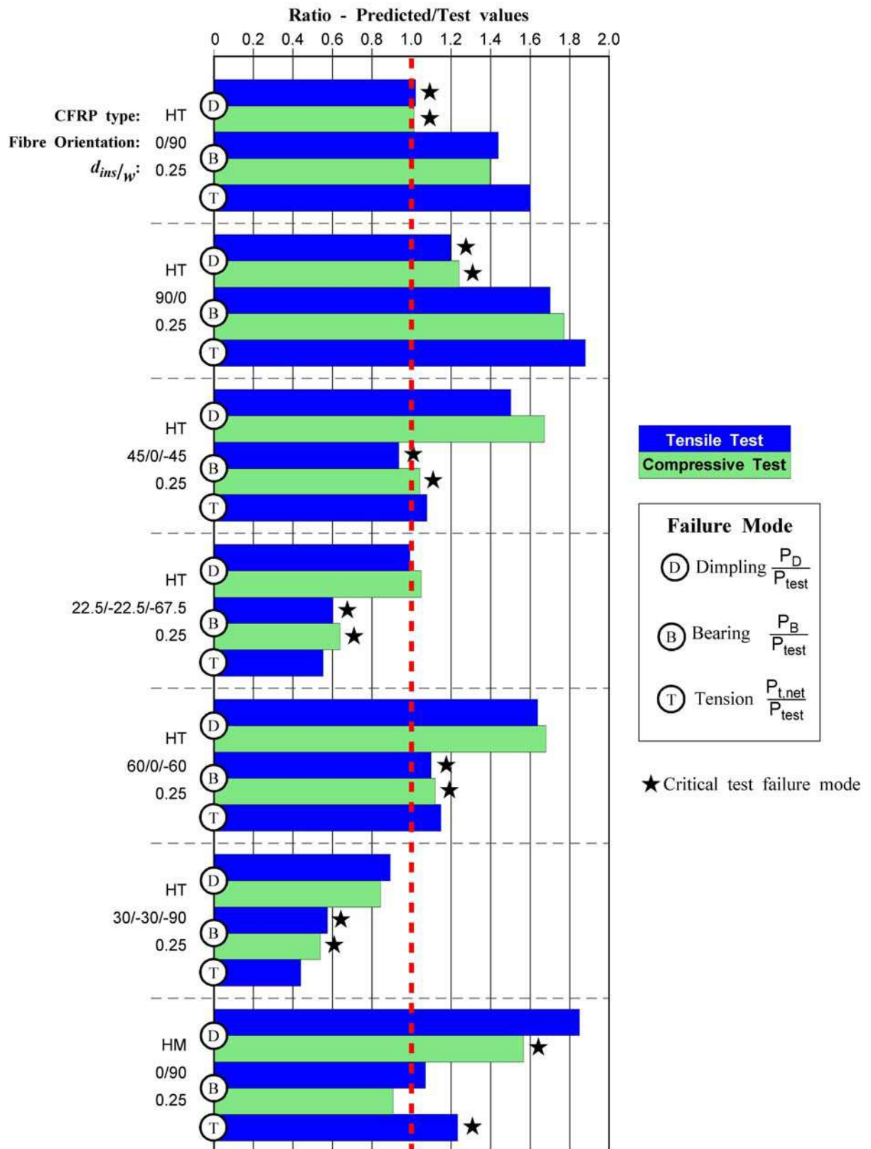
Figure 14-2: Correlation between calculated and tested in-plane capabilities with fibre orientation
