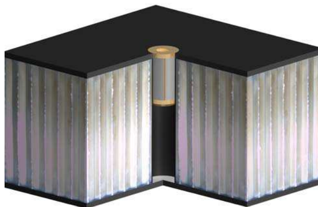
Figure F-13: Carbon fibre tube insert (type 2): With cap for unilateral fixing
