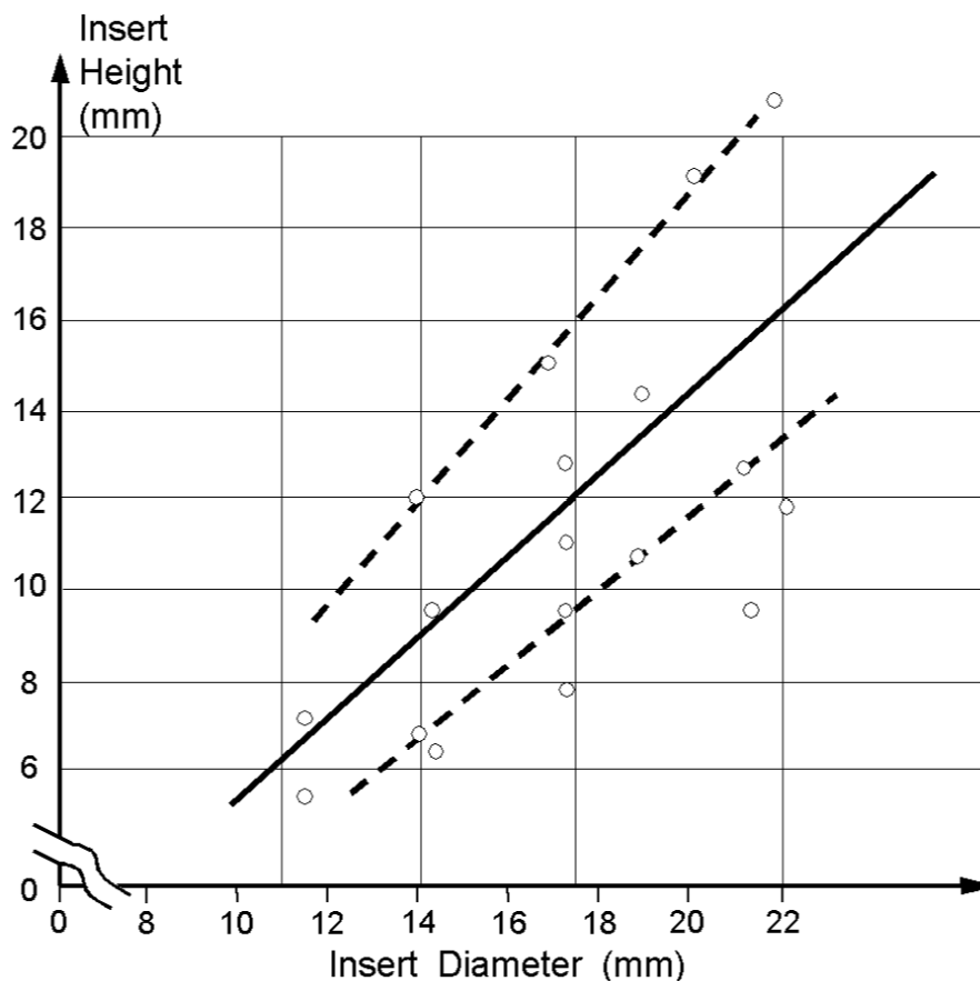
Figure 5-4 Preferred set of insert heights
