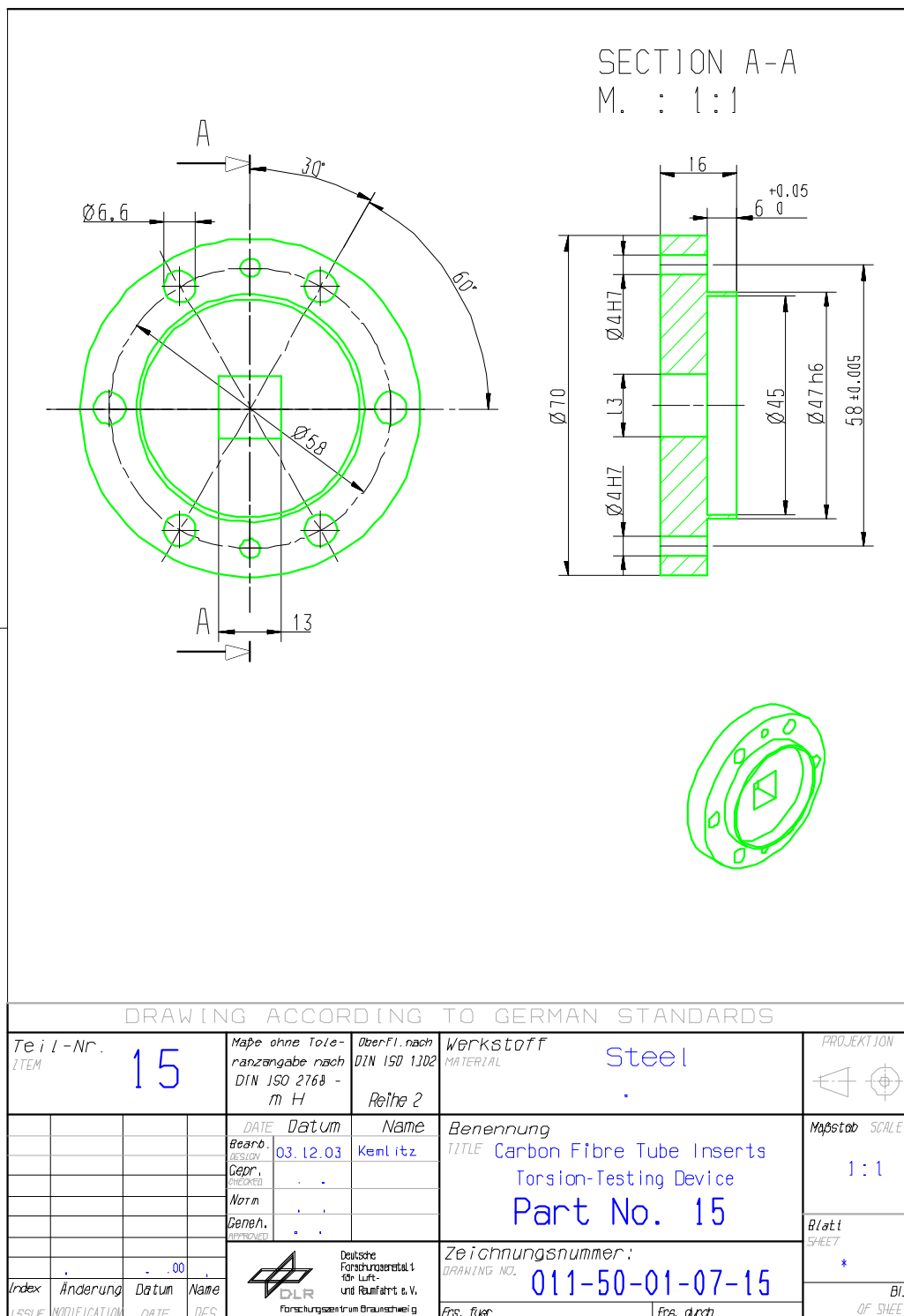
Figure H-46: Test fixture: Torsion – part 15
