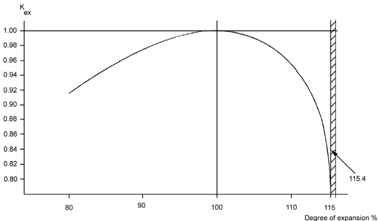
Figure 28-3: QA: Core density correction factor for degree of expansion
