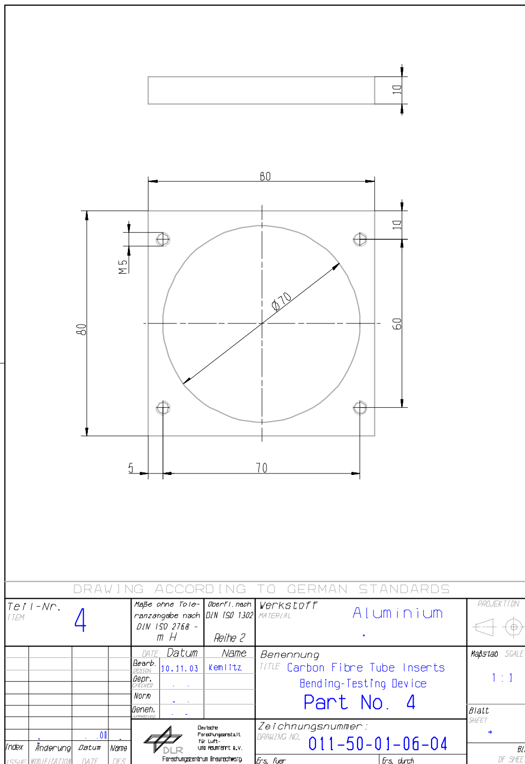
Figure H-22: Test fixture: Bending – part 4
