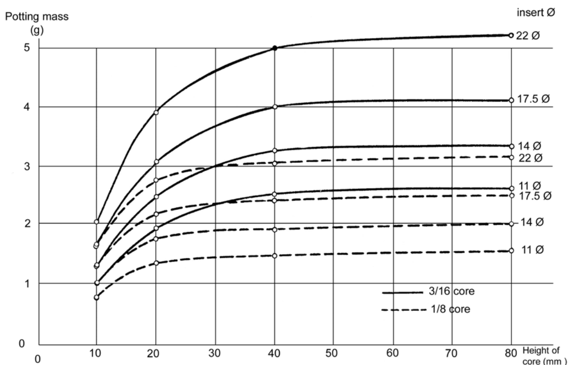
Figure 7-5: Mean weight of potting masses versus core height and insert diameter
