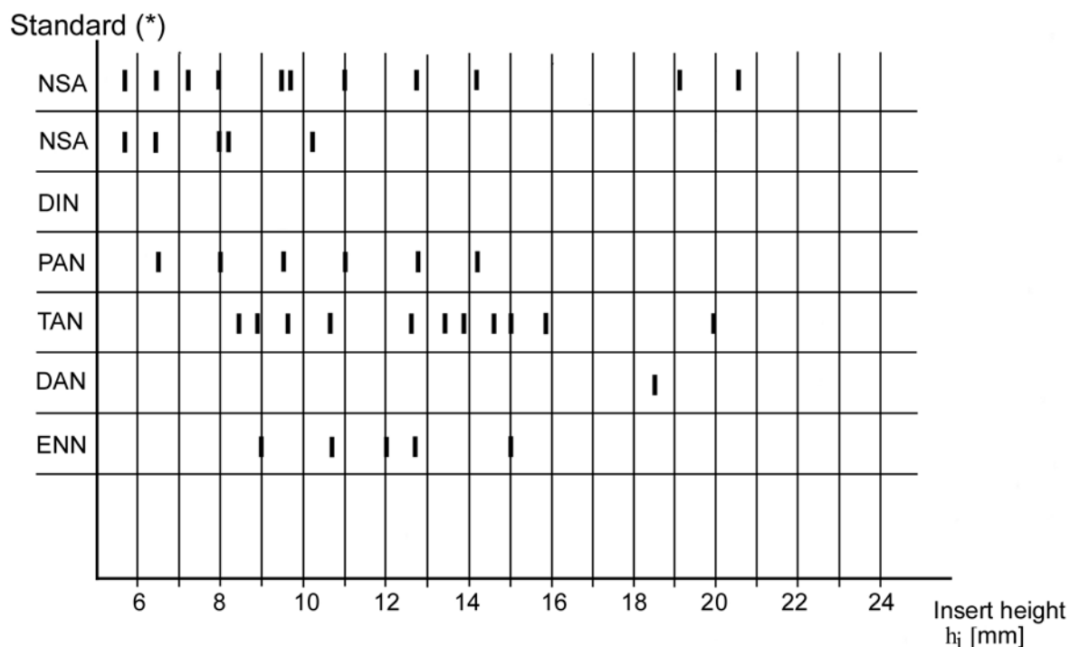
Figure 5-3: Standardised insert height
