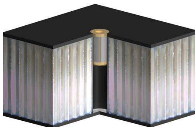
Figure A-4: Carbon fibre tube insert: Type 2 cap
