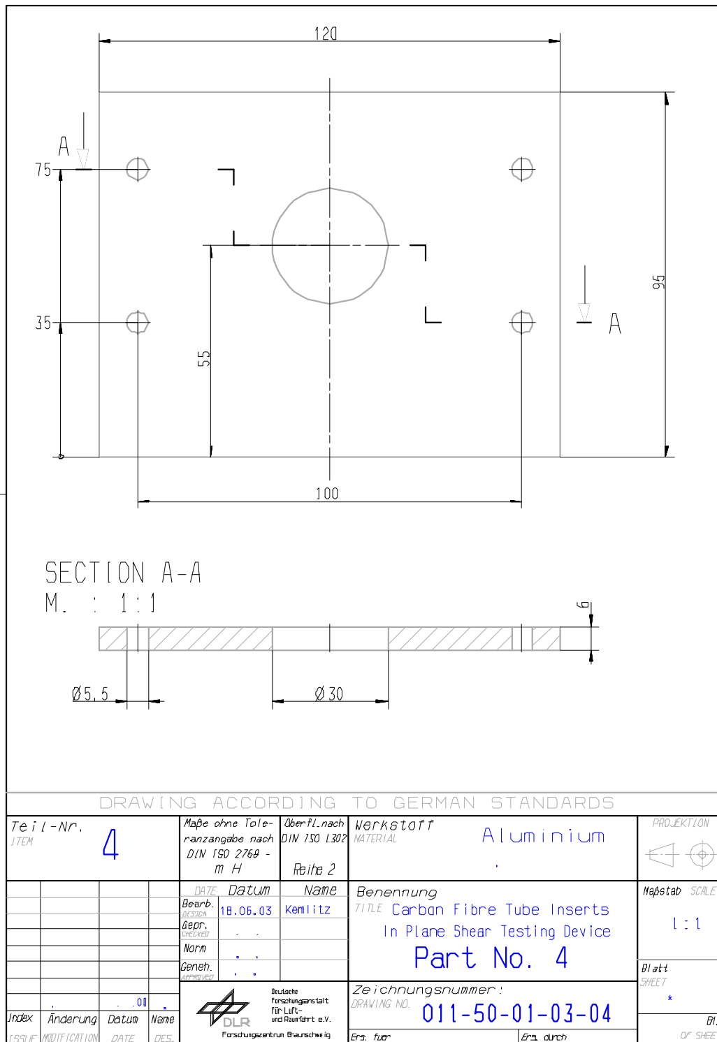
Figure H-13: Test fixture: In-plane shear load – part 4
