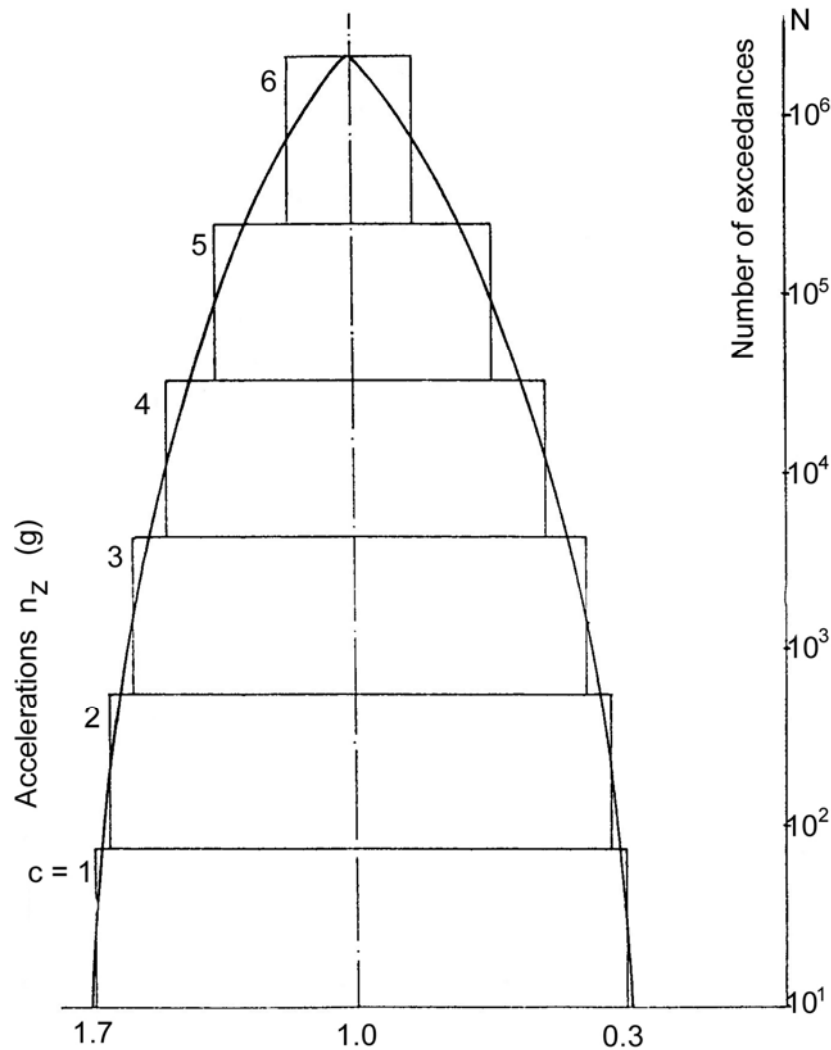
Figure 21-2: Schematic: Design load spectrum
