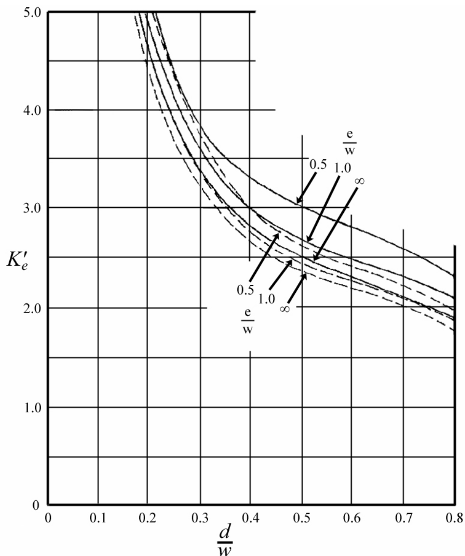
Figure 14-5: Shear strength: Stress concentration factor
