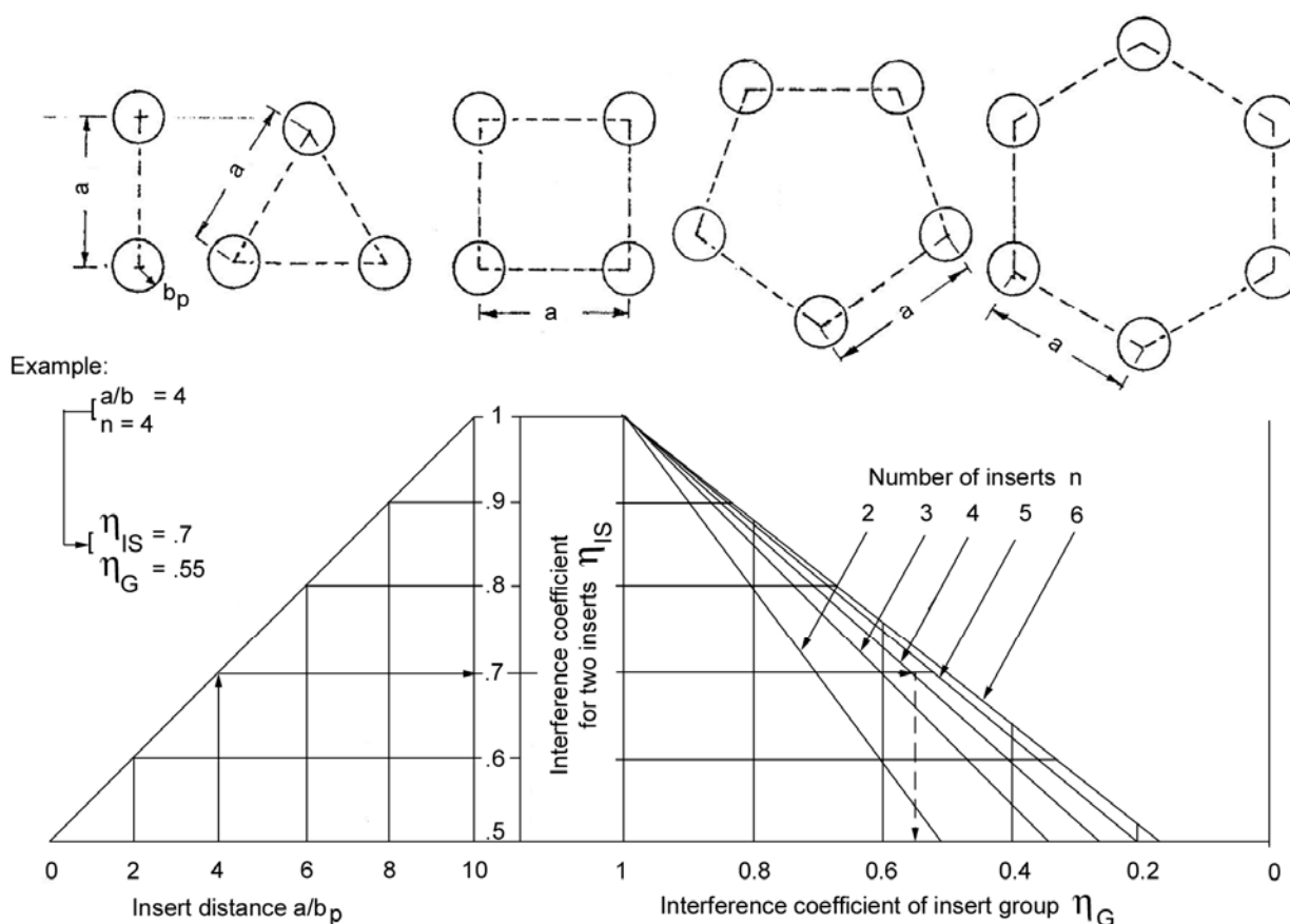
Figure 19-4: Insert groups: Interference coefficient for a group of equal and equidistant inserts
