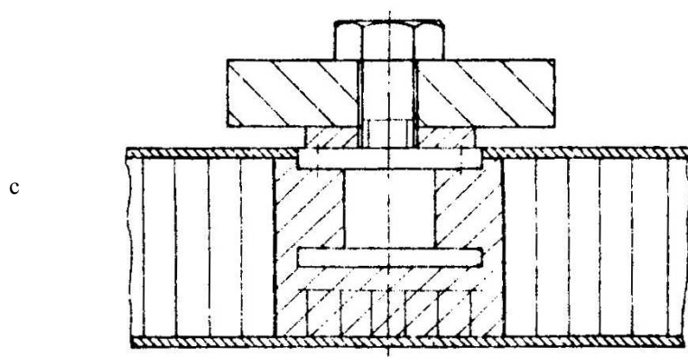
Figure 10-8: Connections
