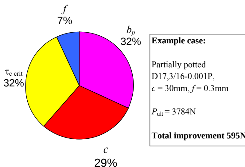
Figure 12-2: Out-of-plane capability: Contributions of the main components on improved core shear
