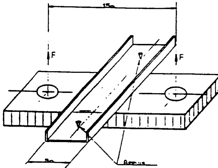
Figure F-4: Case study: ARIANE 4 - tensile (pull-out) test method
