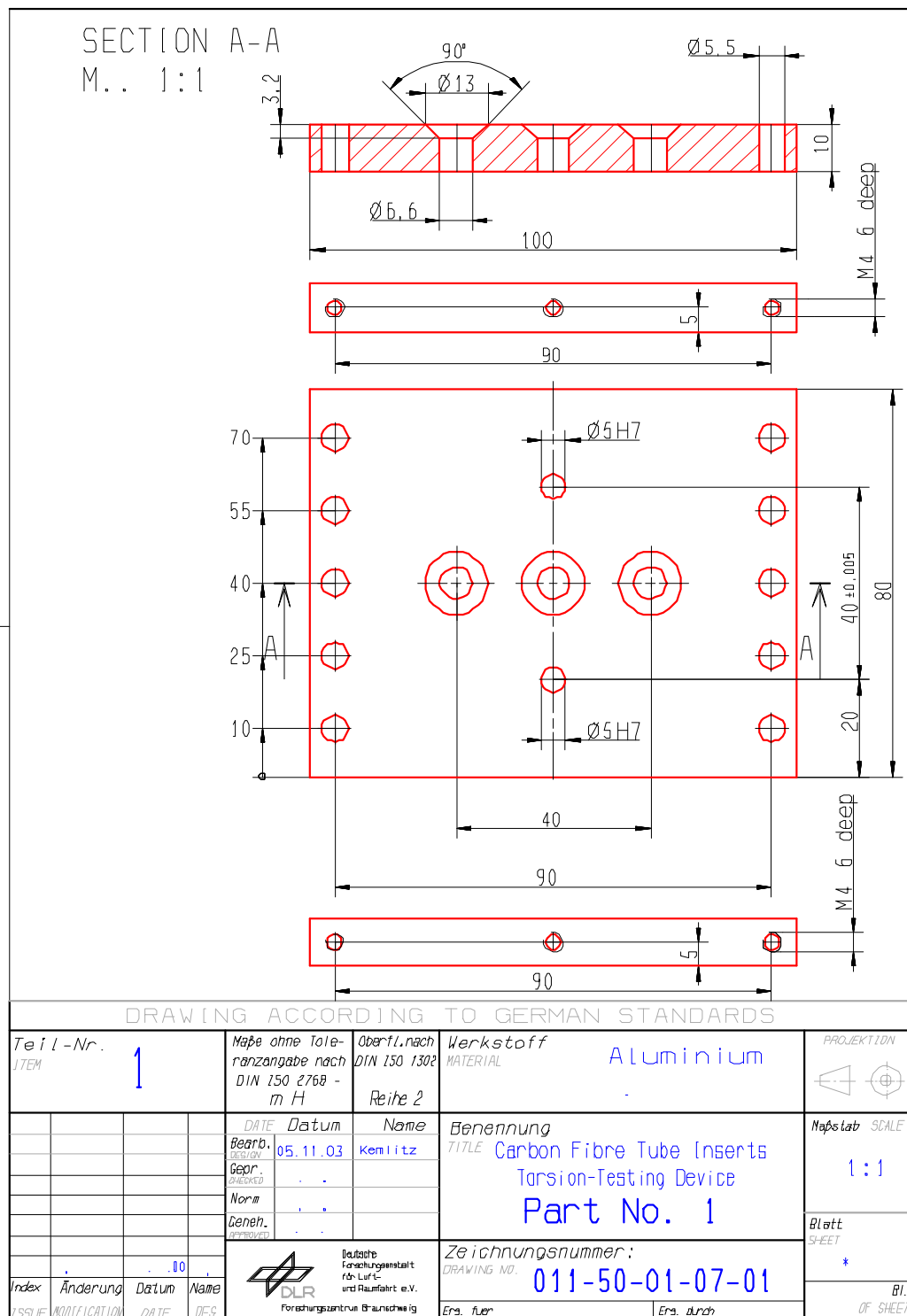
Figure H-32: Test fixture: Torsion – part 1
