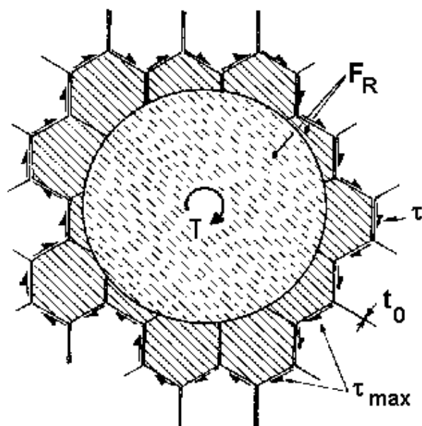
Figure 16-1: Torsional load: Nomenclature
