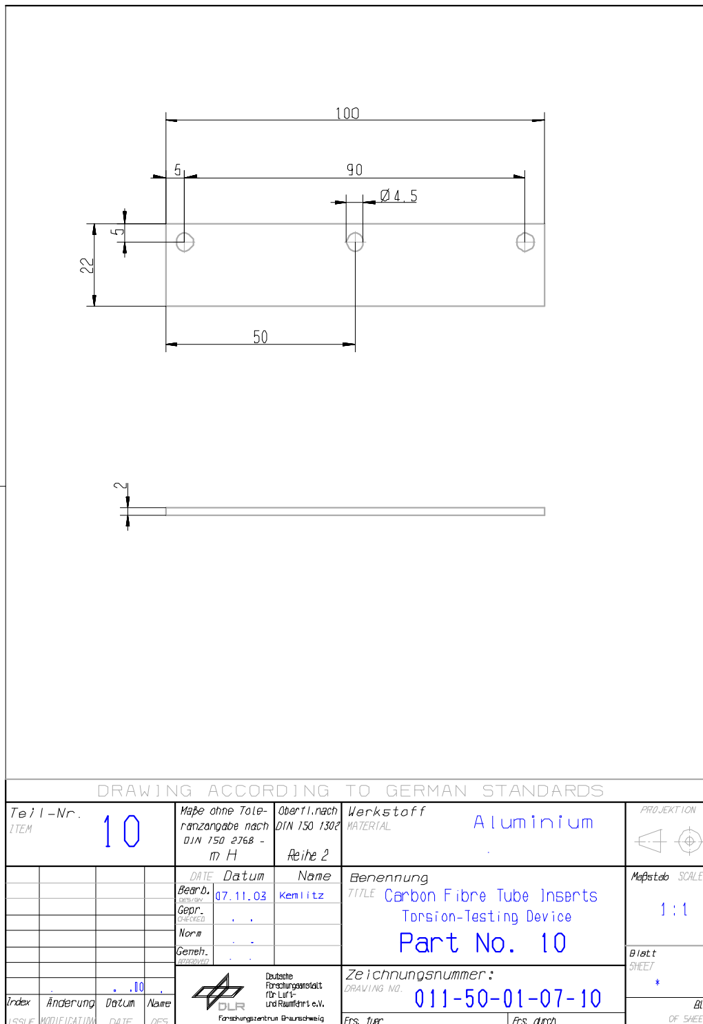
Figure H-41: Test fixture: Torsion – part 10
