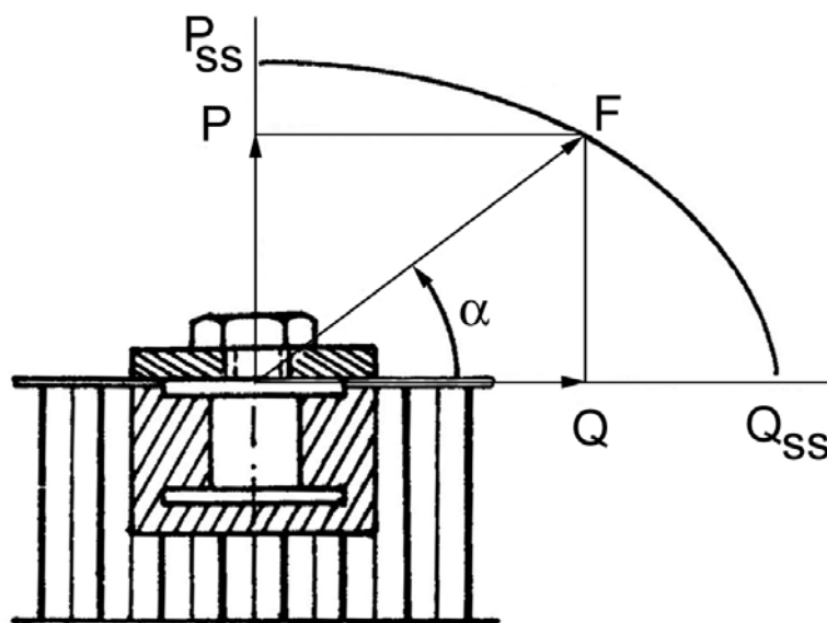
Figure 17-1: Insert submitted to an inclined load
