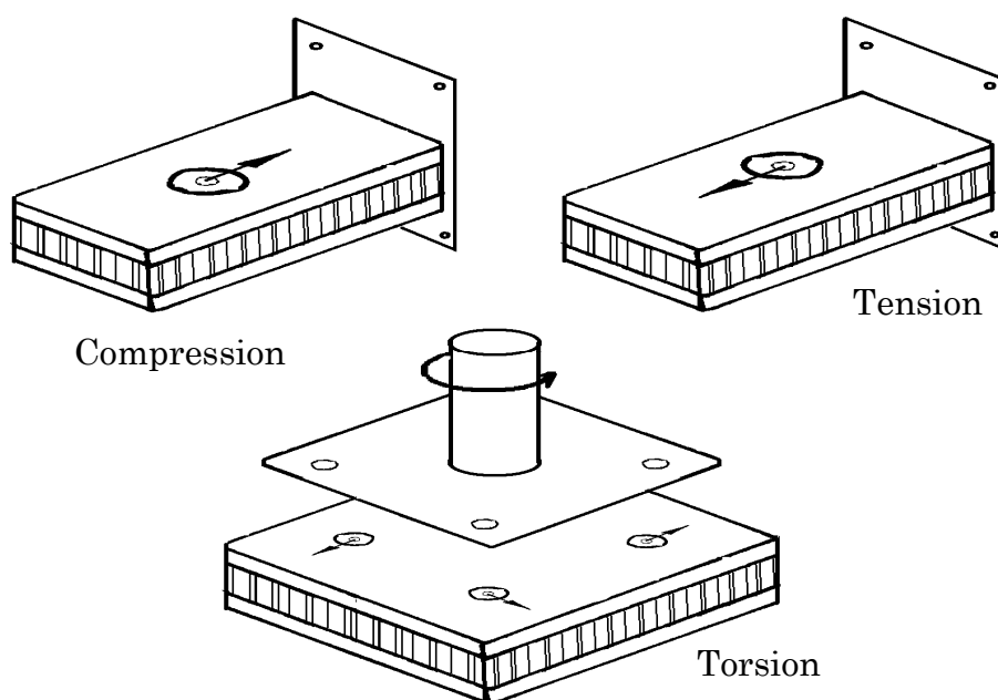
Figure 10-19: Failure modes: In-plane and torsion loads
