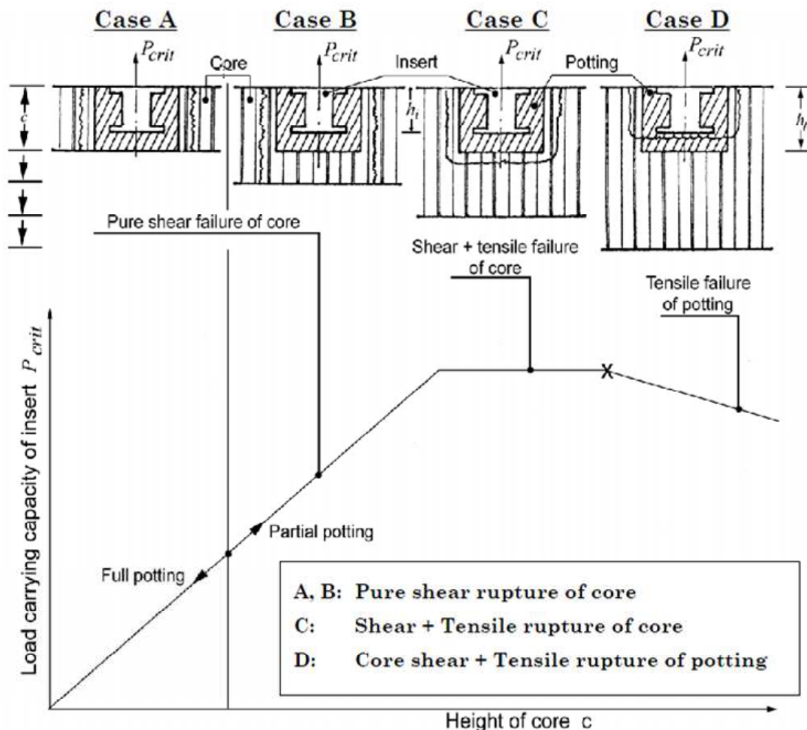
Figure 10-16: Failure modes: Insert as a function of core height
