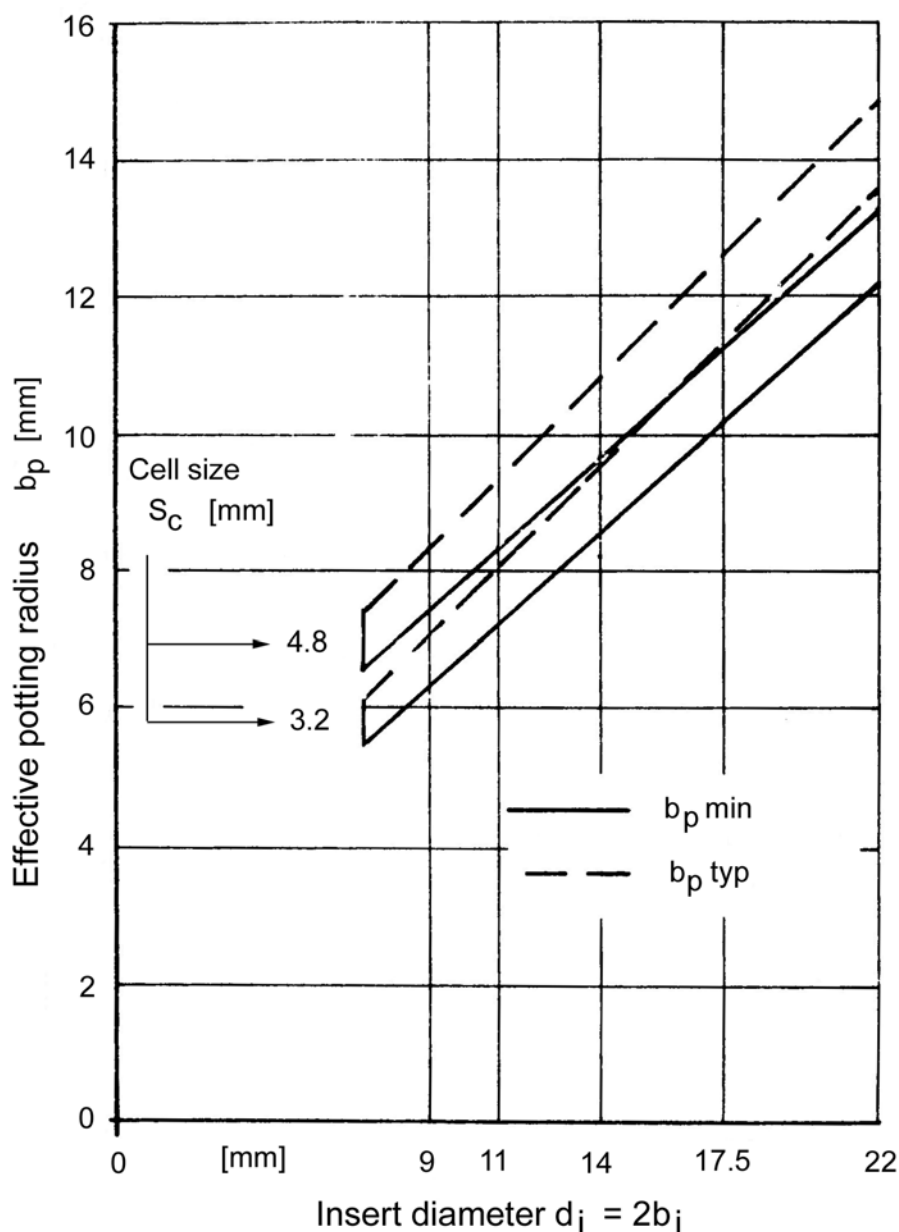
Figure 7-2: Effective potting radius as a function of insert diameter
