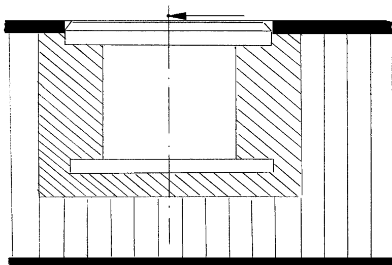
Figure 10-6: CFRP face sheets: Effect of small chamfer on insert flange on load transfer to face sheet
