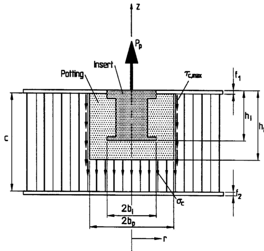
Figure D-2: Partially potted insert: out-of-plane loading
