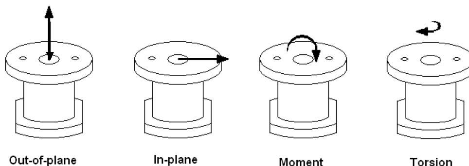
Figure 9-2: Insert load cases
