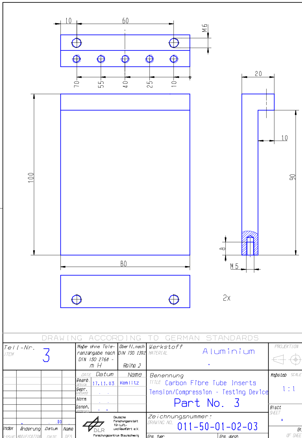
Figure H-4: Test fixture: Tension-compression load – part 3
