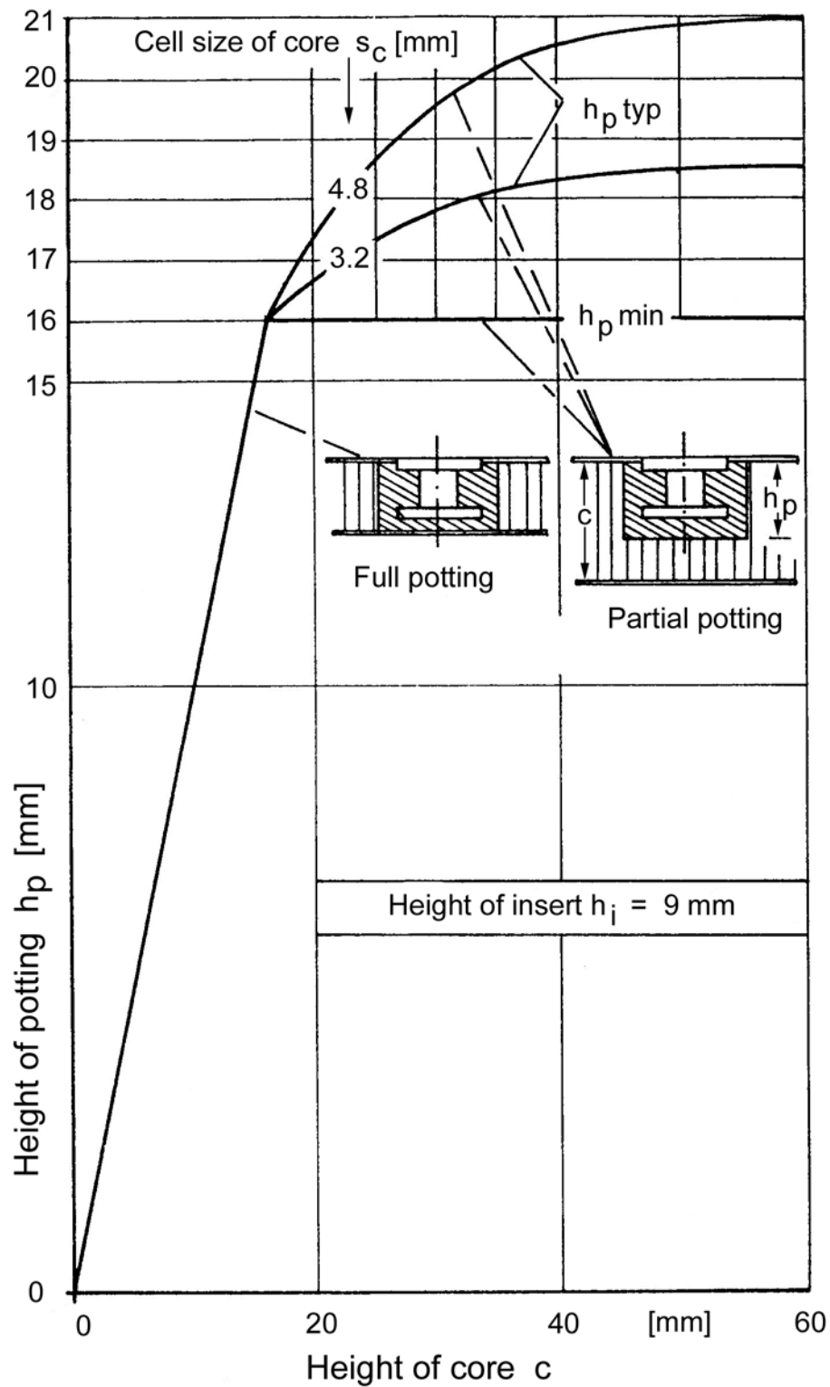
Figure 7-4: Potting height as a function of the honeycomb core height
