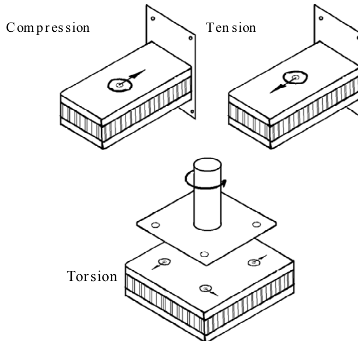
Figure 9-4: Insert in-plane load
