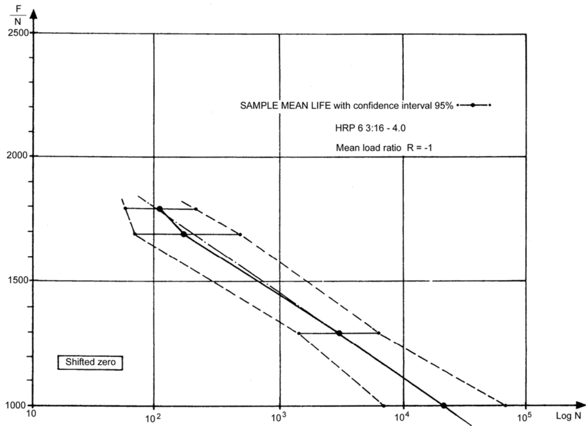
Figure 21-8: Fatigue life: Non-metallic GFRP core
