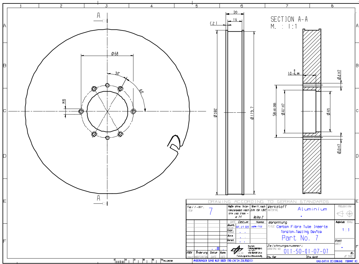
Figure H-38: Test fixture: Torsion – part 7
