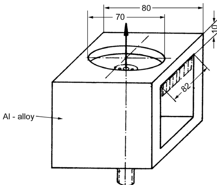
Figure E-1: Manufacture control: Insert tensile pull-out test fixture
