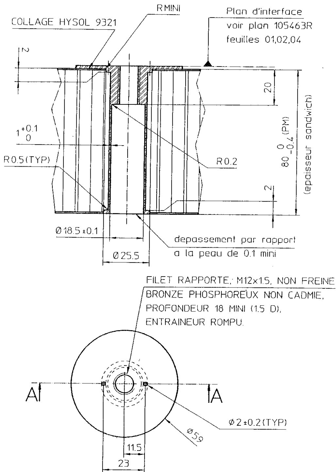
Figure F-16: Case study: SPOT 5 - Structure I/F platform
