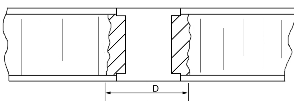
Figure 10-13: Pre-design: Through-the-thickness insert under transverse force
