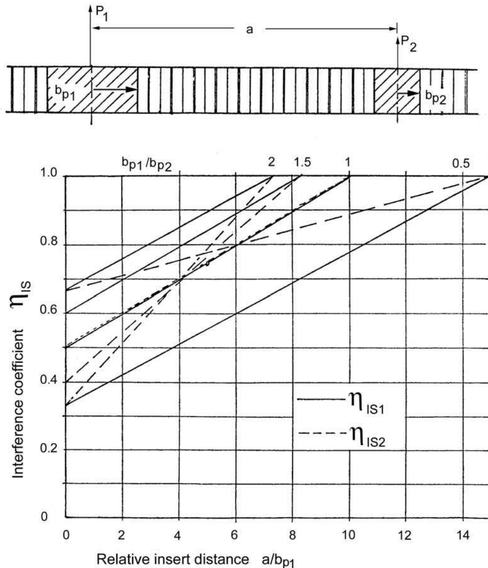
Figure 19-1: Insert groups: Reduced insert capability - two adjacent inserts loaded in the same direction
