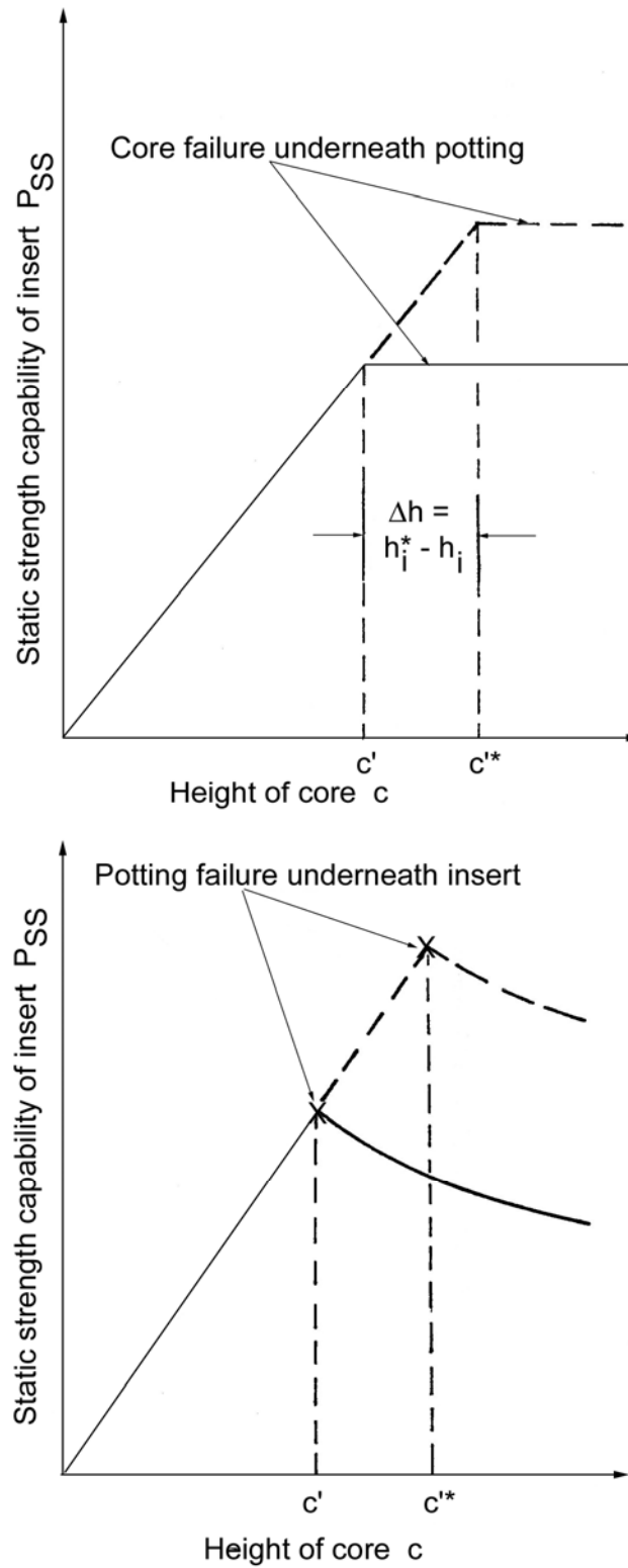
Figure 12-4: Influence of insert height on insert capability
