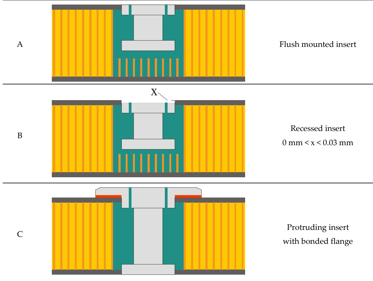
Figure 10-7: Insert mounting modes
