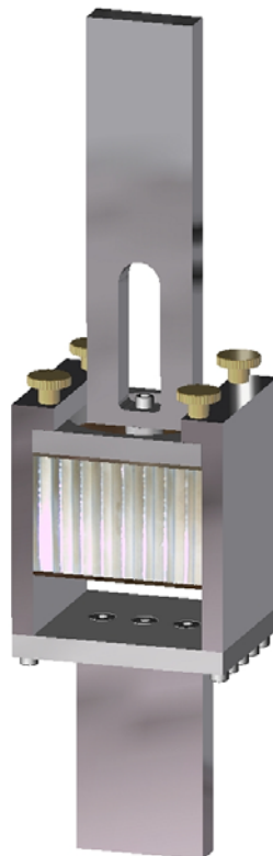
Figure 27-1: Manufacture control: Out-of-plane test fixture for tension (pull-out) tests
