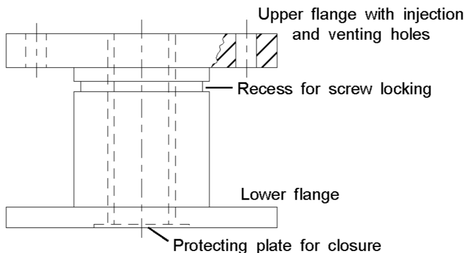
Figure 5-1: Typical insert
