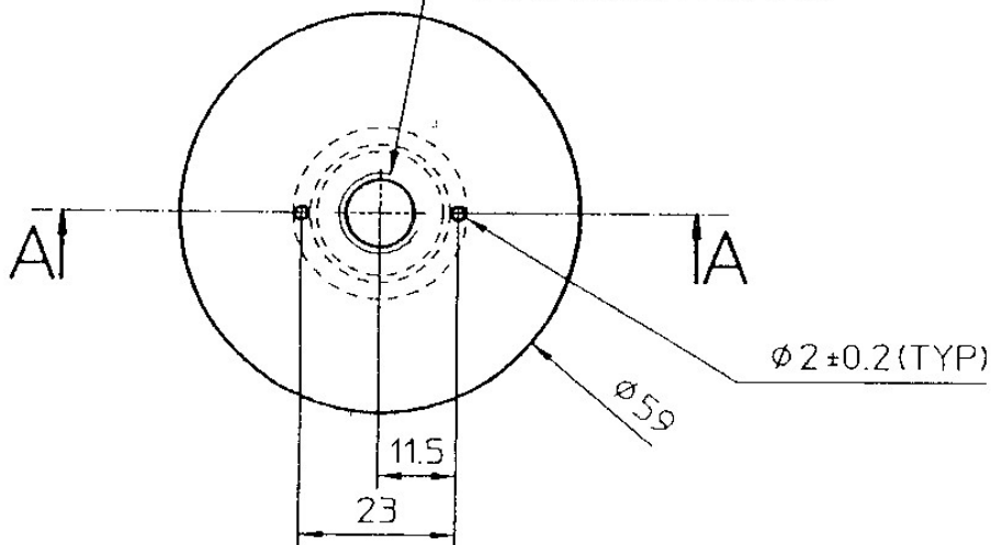
Figure F-16: Case study: SPOT 5 - Structure I/F platform
