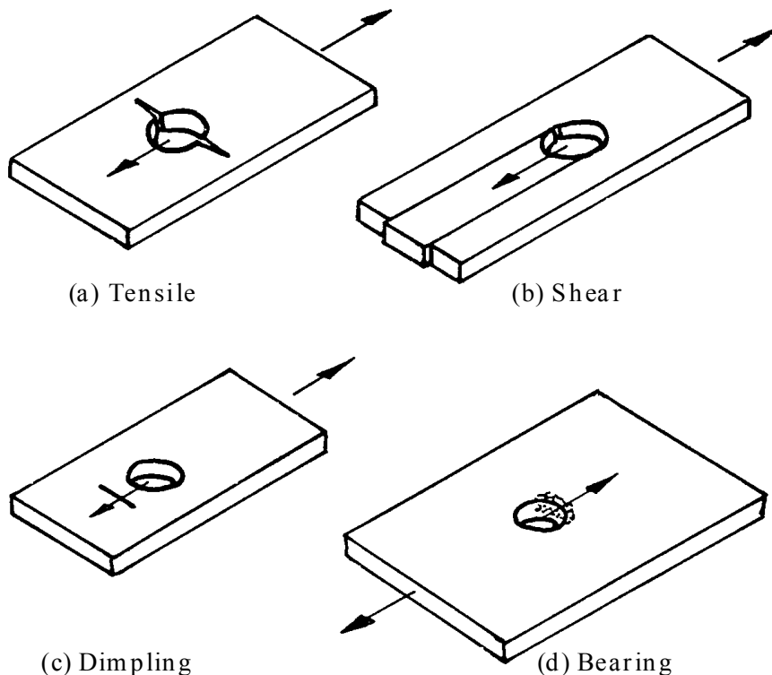
Figure 10-20: Failure modes: CFRP face sheets
