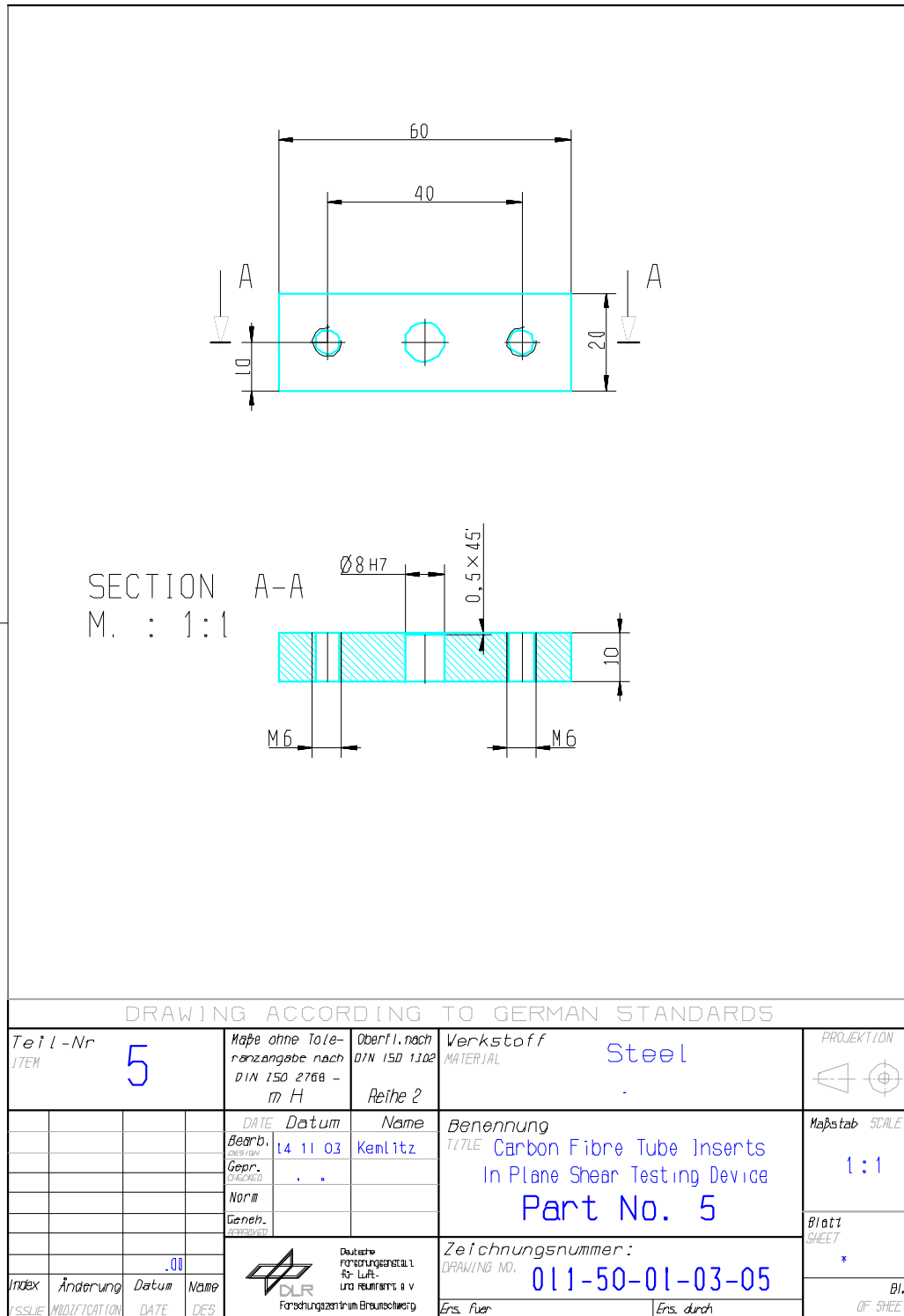
Figure H-14: Test fixture: In-plane shear load – part 5
