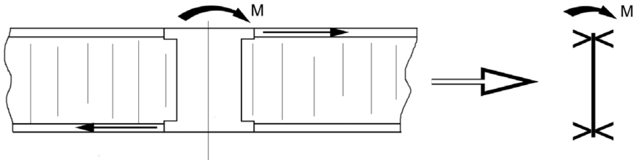
Figure 10-11: Pre-design: Through-the-thickness insert under bending
