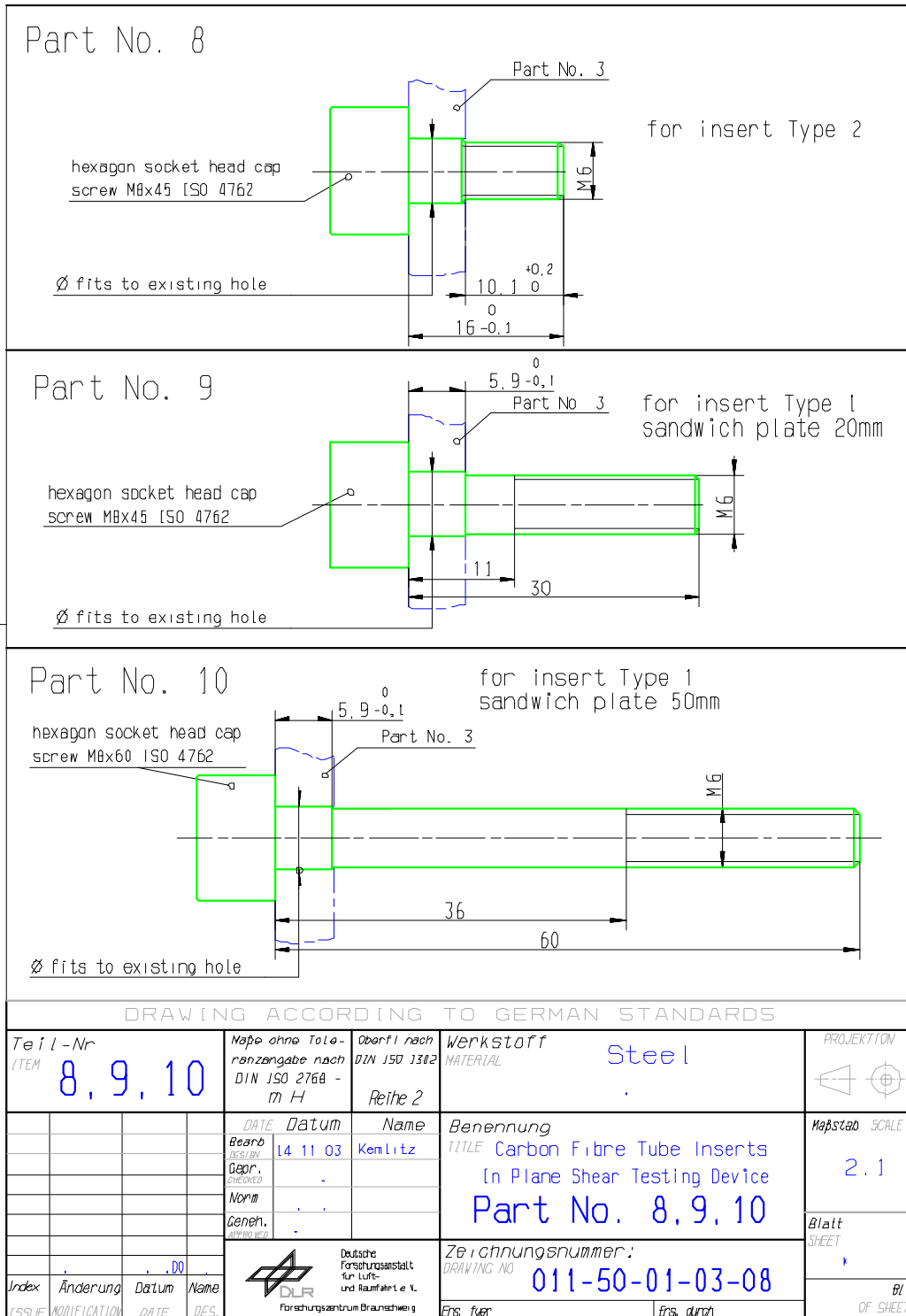
Figure H-17: Test fixture: In-plane shear load – part 8
