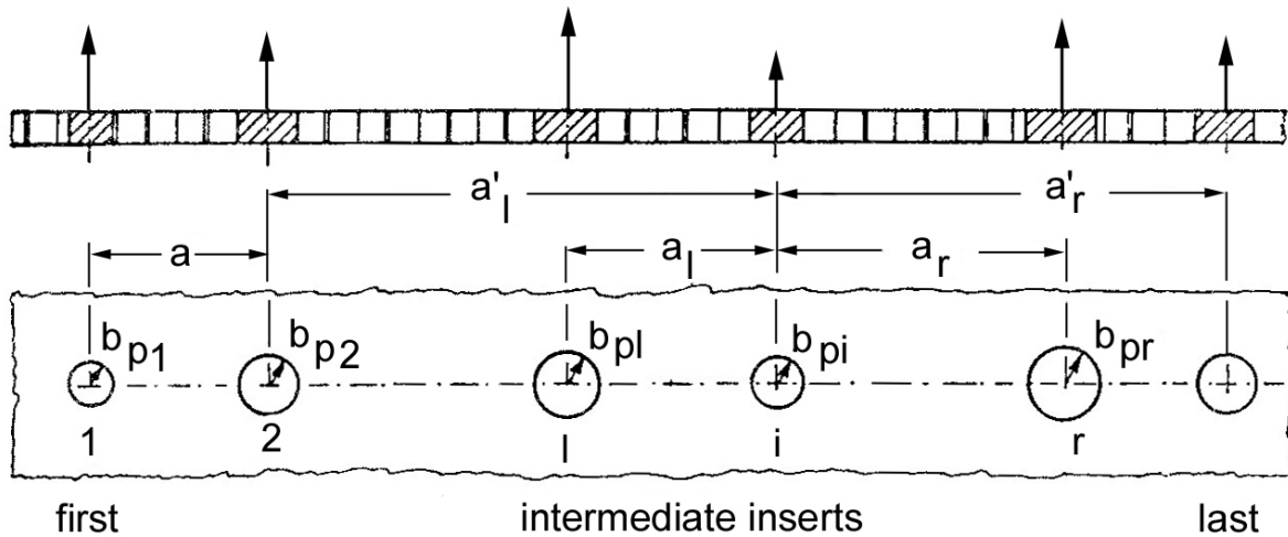
Figure 19-2: Insert groups: Series of inserts loaded in same direction
