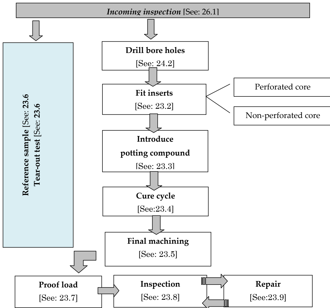
Figure 23-1: Basic manufacturing sequence Fit inserts
