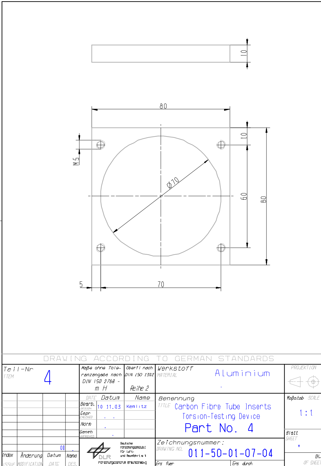
Figure H-35: Test fixture: Torsion – part 4
