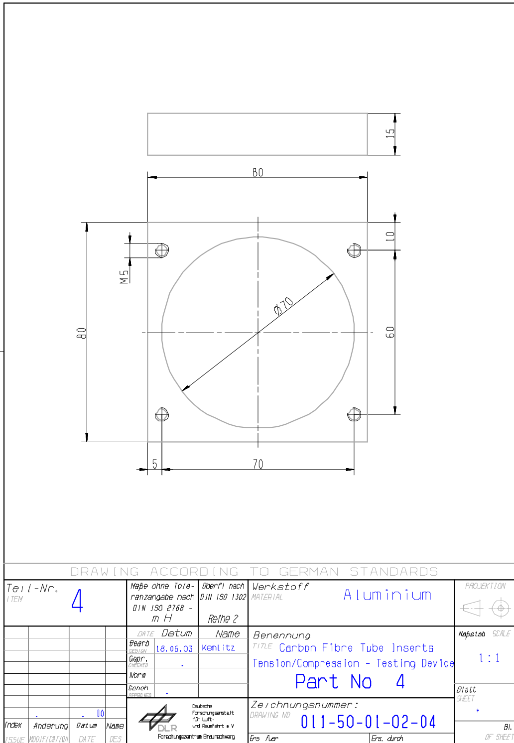
Figure H-5: Test fixture: Tension-compression load – part 4
