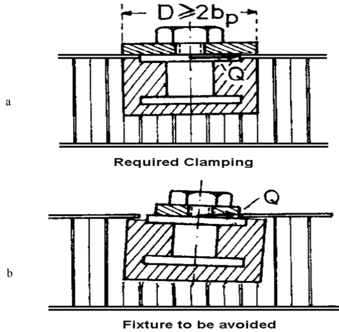
Figure 10-4: Insert design under in-plane load
