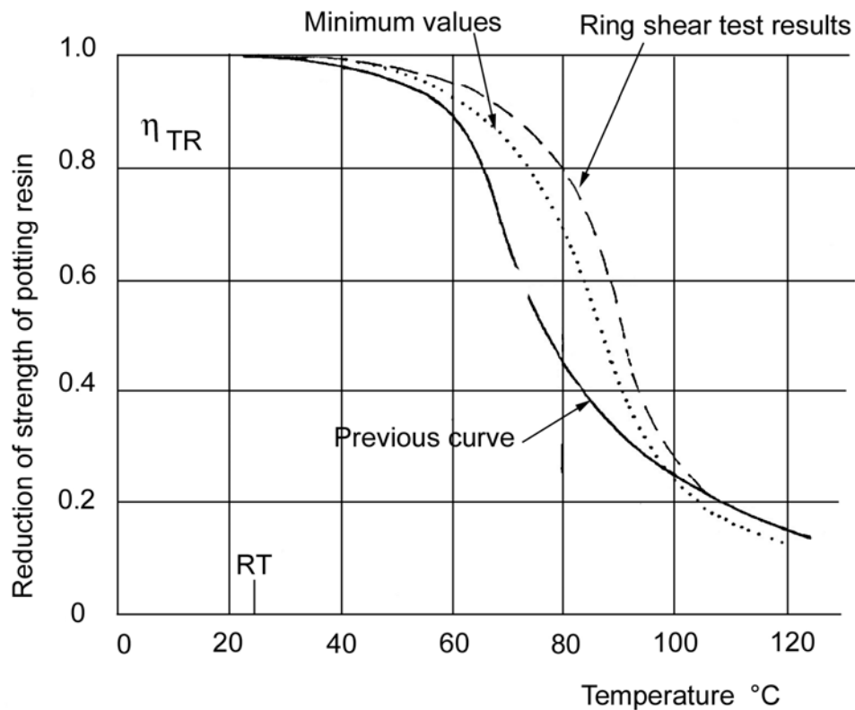
Thermal effects: Reduction of potting resin strength
