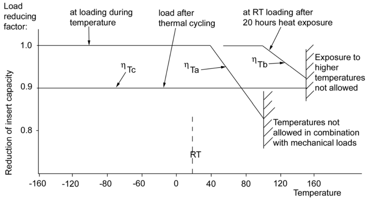
Figure 22-1: Thermal effects: Reduction of insert capability
