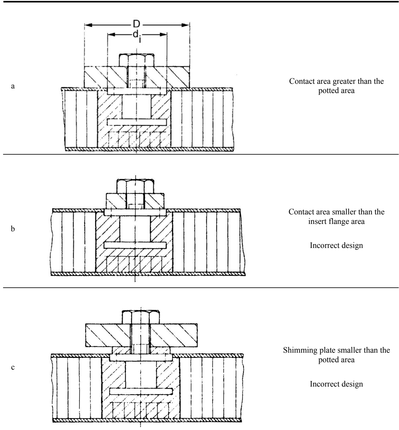
Figure 10-8: Connections
