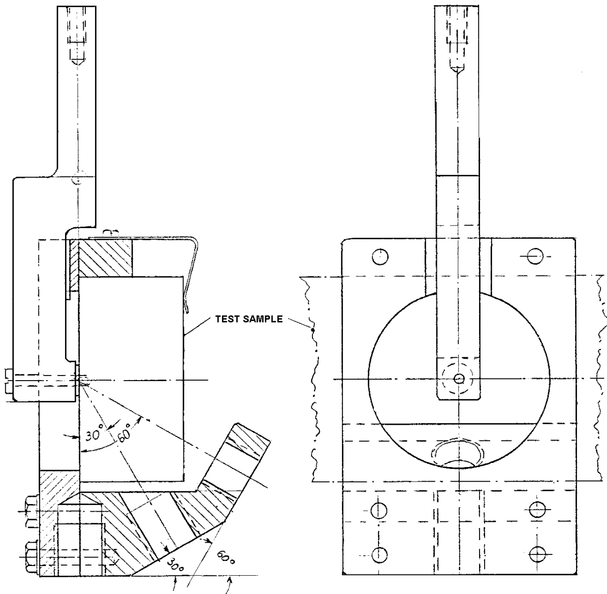
Figure 29-2: Testing: Insert static in-plane strength fixture
