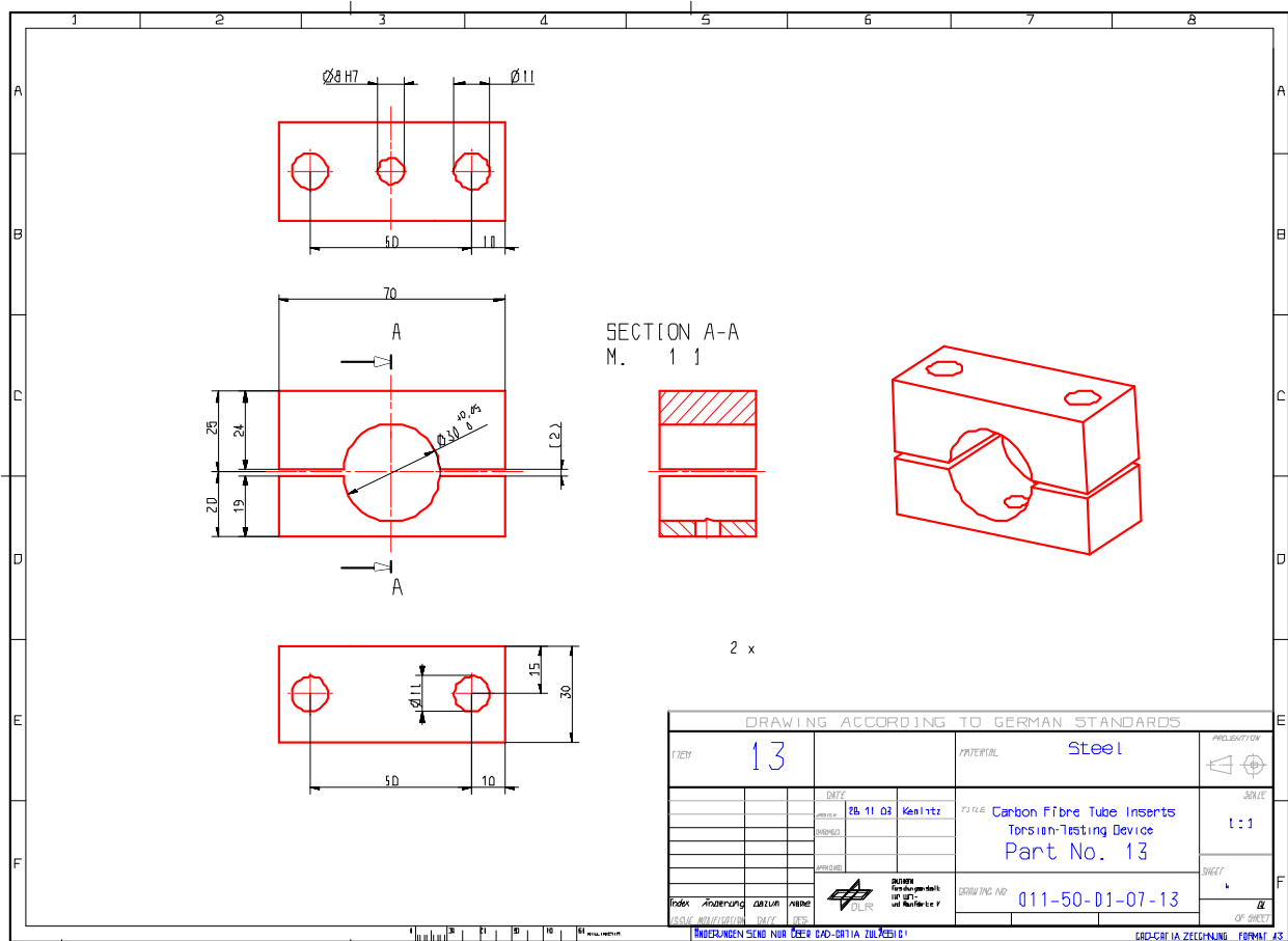
Figure H-44: Test fixture: Torsion – part 13
