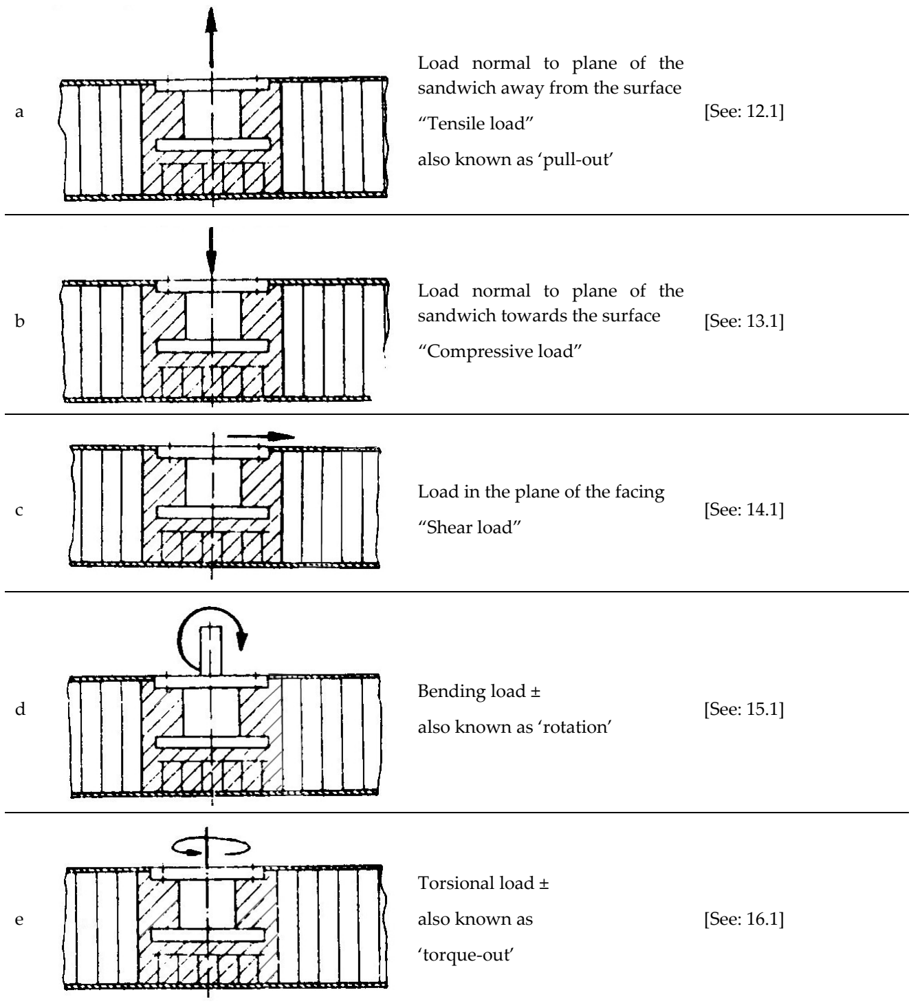
Figure 10-2: Insert load conditions
