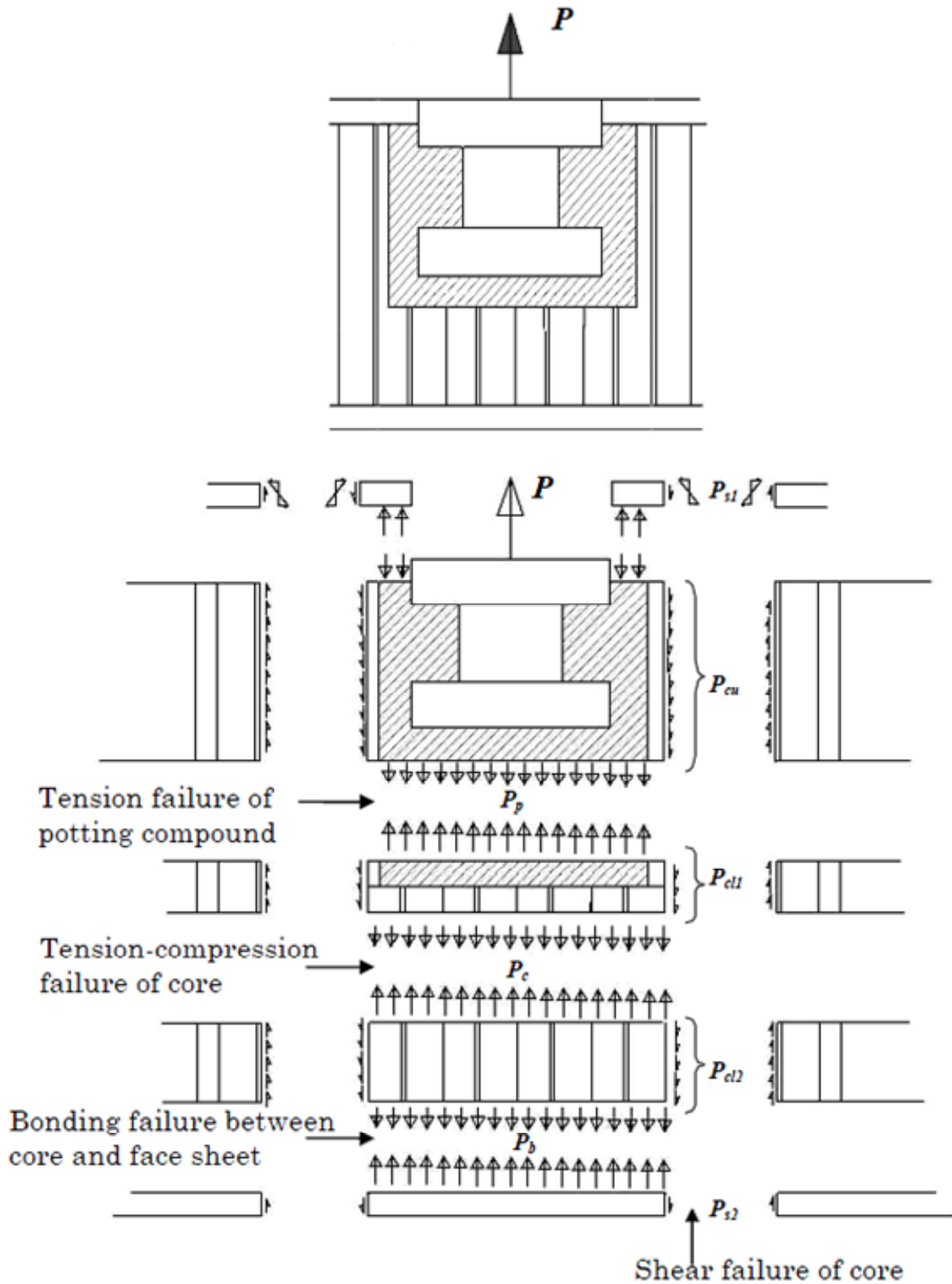
Figure 10-15: Failure modes: Load transfer in out-of-plane case
