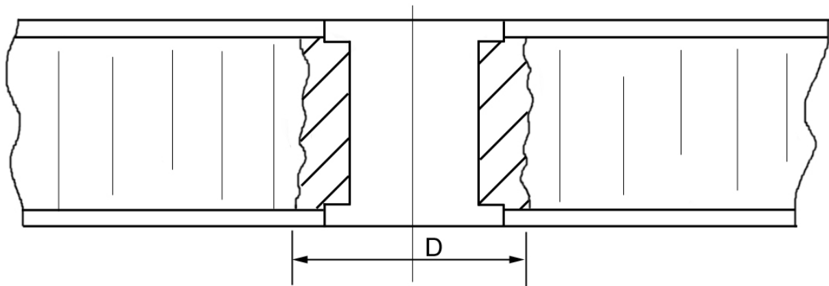
Figure 10-13: Pre-design: Through-the-thickness insert under transverse force
