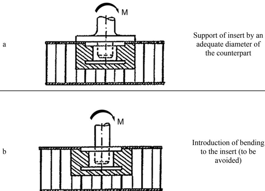
Figure 10-5: Insert design loaded by moments
