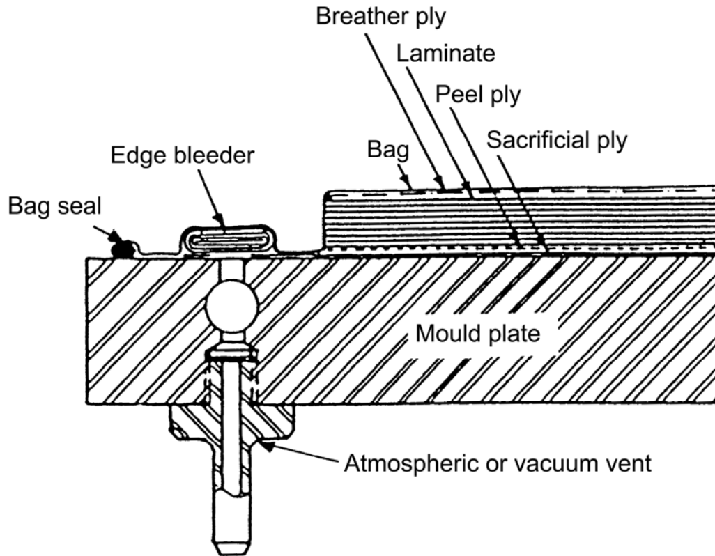
Figure 38.4-5 - Bag moulding: Edge bleed out system
