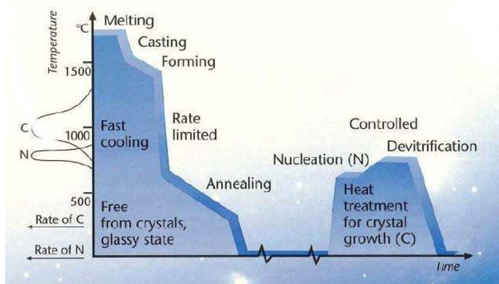
Figure 43.15-3 - Zerodur®: Annealing process
