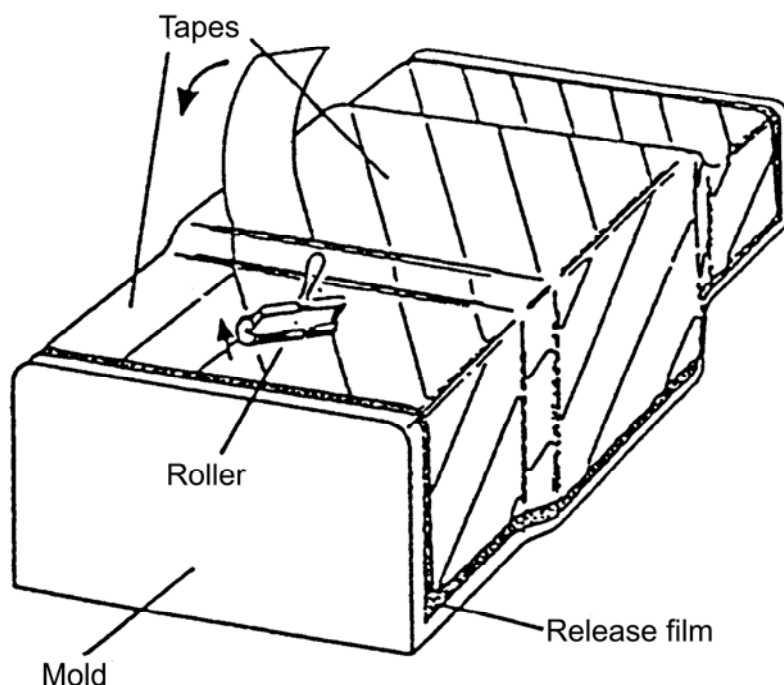
Figure 38.3-2 - Prepreg: Direct lay-up
