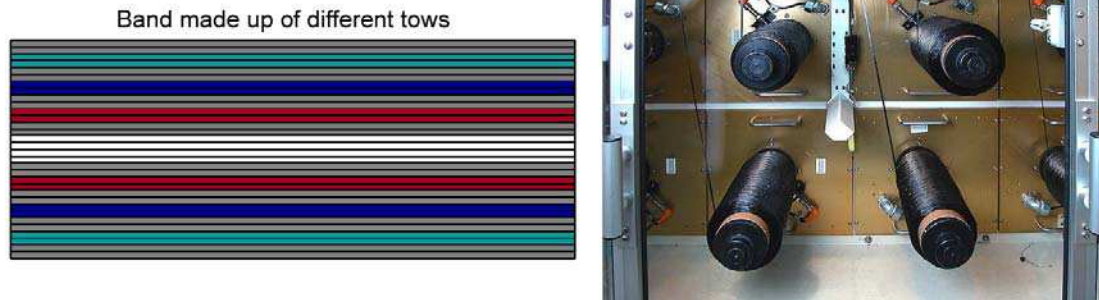
Figure 38.14-8 – Fibre placement: Mixed-material lay-up
