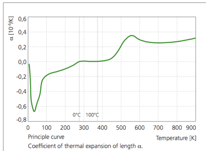
Figure 43.15-6 - Zerodur®: Thermal expansion – cryogenic behaviour
