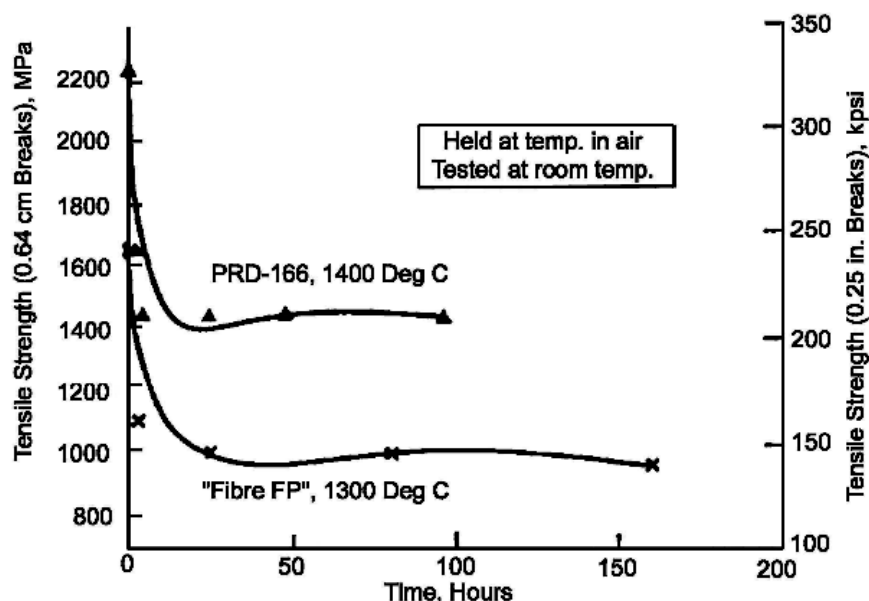
Figure 42.6-11 - Alumina fibres: tensile strength against exposure time
