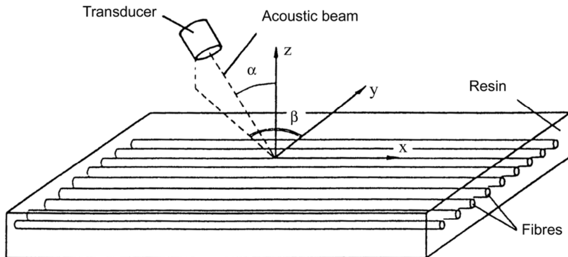
Figure 34.10-2 - Detection of fibre orientation by backscattering measurement
