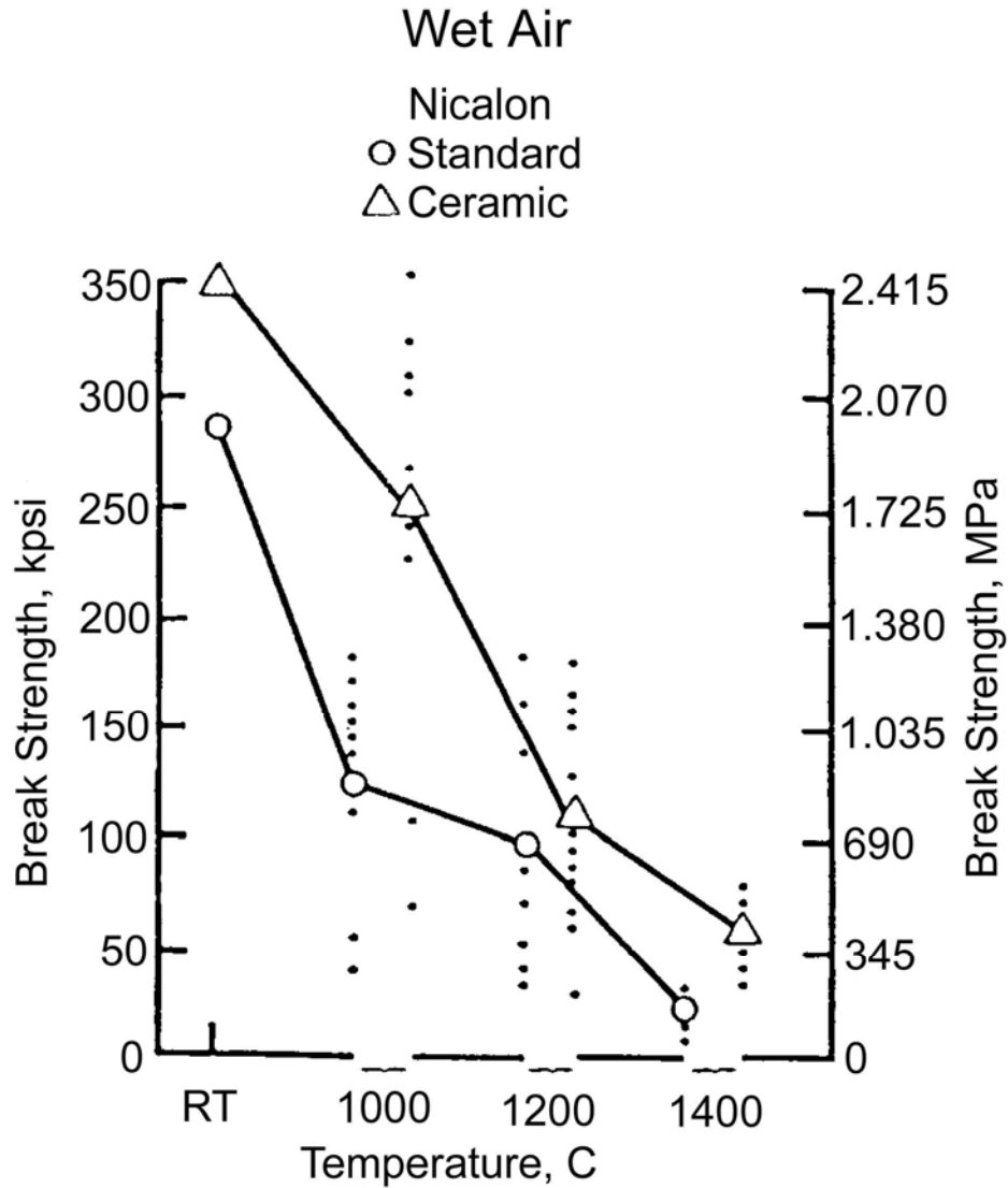
Figure 42.6-1 - SiC Nicalon fibre tensile strength at elevated temperature
