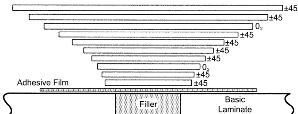
Figure 41.6-2 - External repair: Cured in place
