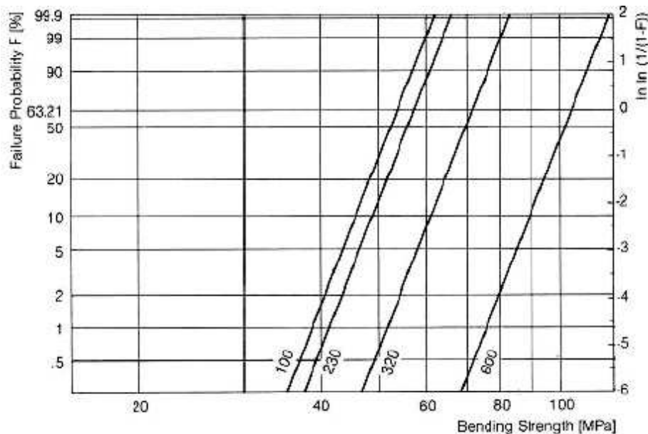
Figure 43.15-11 - Zerodur®: Failure probability of Zerodur for test surfaces processed with loose grit of different sizes
