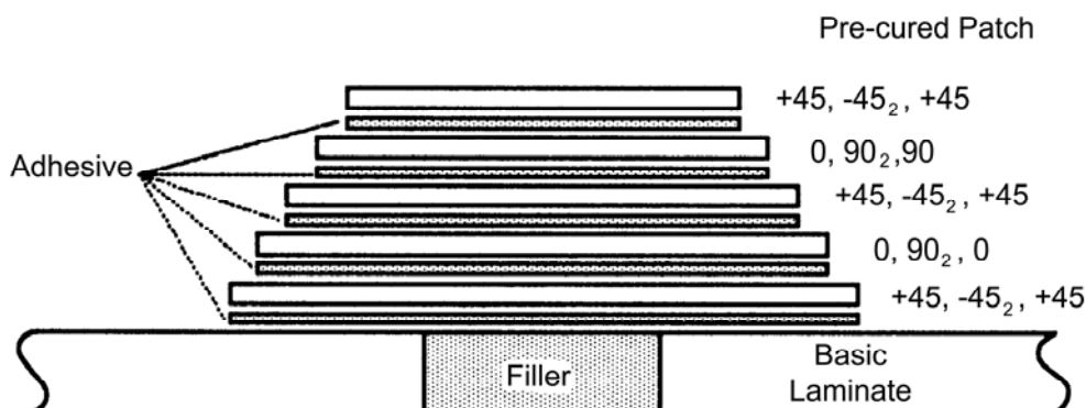
Figure 41.6-1 - External repair: Pre-cured patches
