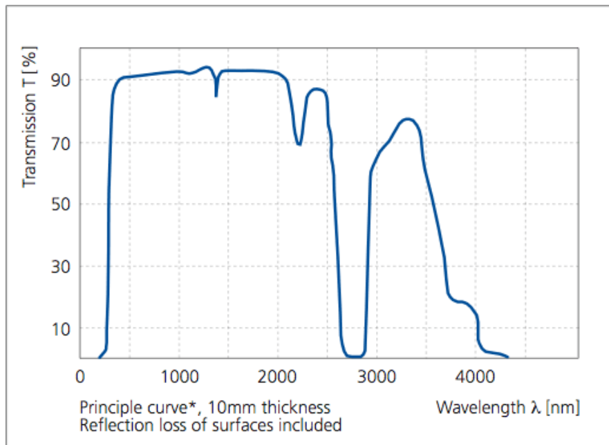
Figure 43.15-14 - ULE®: Transmission curve
