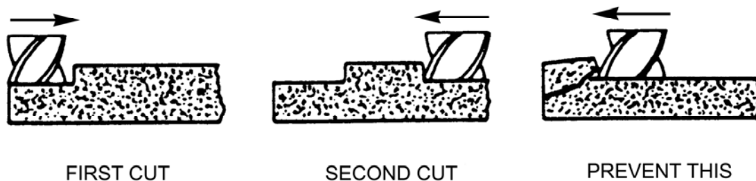
Figure 39.8-1 - Proper milling technique
