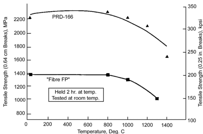
Figure 42.6-10 - Alumina fibres: tensile strength against exposure to elevated temperature
