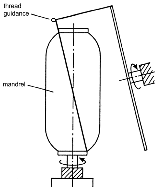
Figure 38.6-1 - Filament winding: Polar vertical
