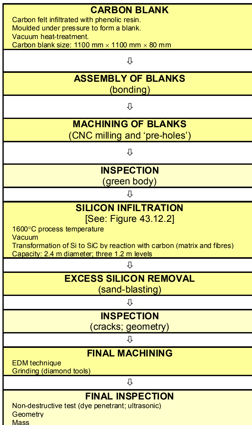
Figure 43.12-1 – Cestic®: Basic processing sequence
