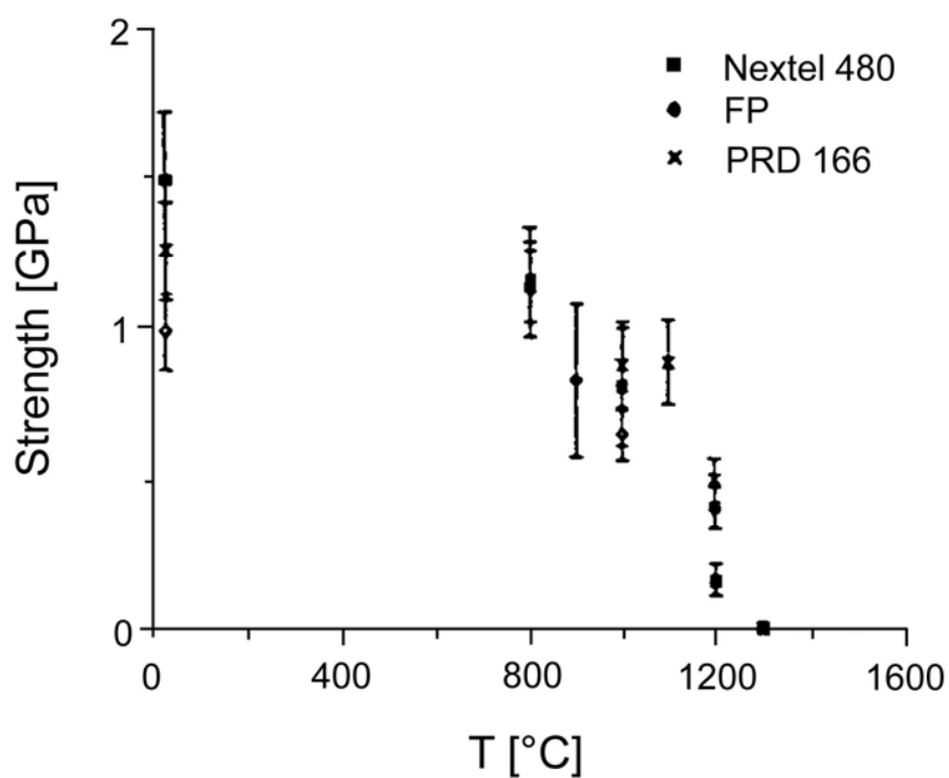
Figure 42.6-8 - Alumina fibres: tensile strength at elevated temperature
