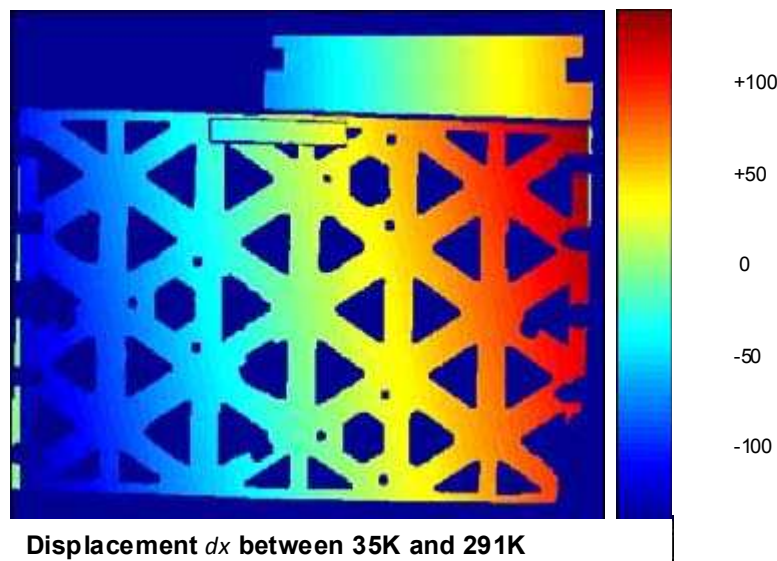
Figure 43.18-6 – NIRSspec optical bench development: Thermal contraction under cryogenic test
