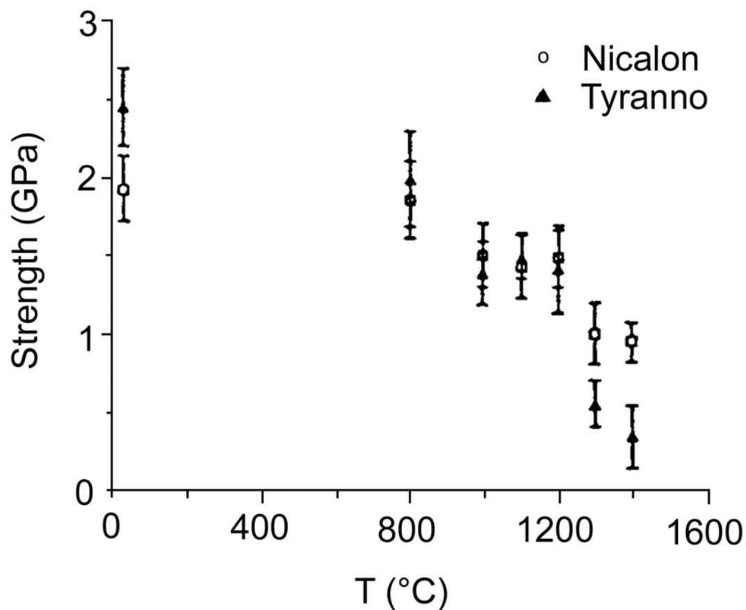
Figure 42.6-6 - SiC fibres Nicalon and Tyranno: tensile strength at elevated temperature
