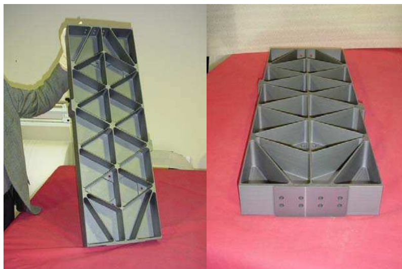
Figure 43.12-13 – SiC-100®: NIRSpec Optical Bench Breadboard
