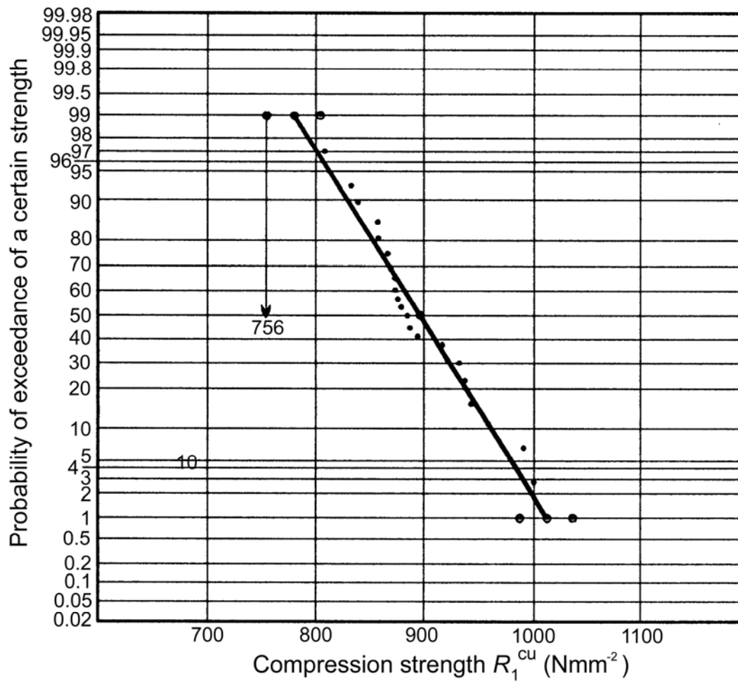
Figure 37.5-3 - Probability of exceedance: Compressive strength 90°
