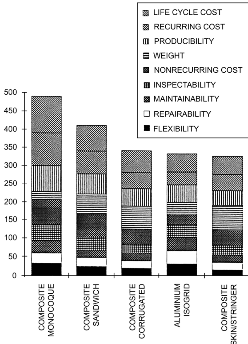
Figure 40.6-3 - Launcher fairing cylinder: Kepner-Tregoe evaluation scores for the section designs
