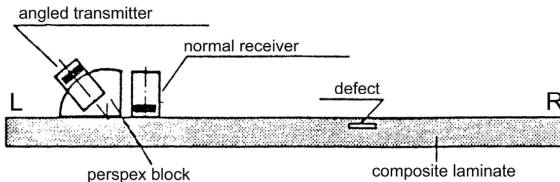
Figure 34.10-1 - Leaky-Lamb-wave technique for composites
