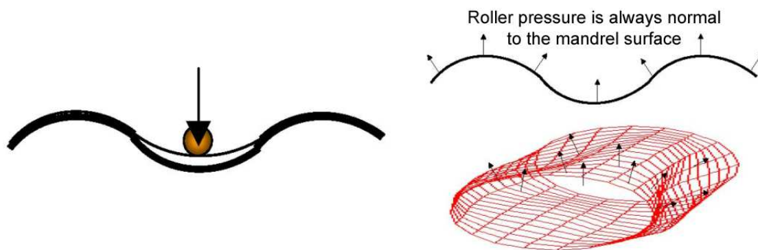
Figure 38.14-4 – Fibre placement: Complex curvature
