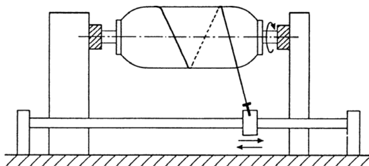
Figure 38.6-4 - Filament winding: Helical
