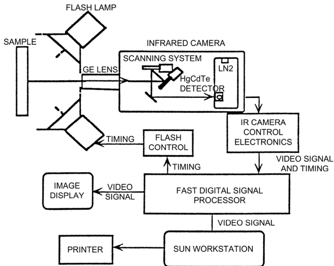
Figure 34.15-1 - Basic thermographic technique
