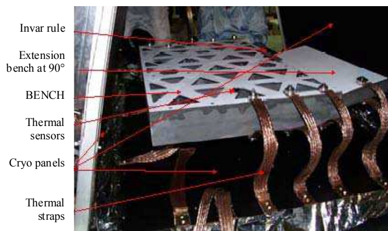
Figure 43.18-5 – NIRSpec optical bench development: Test set-up for cryogenic temperature test
