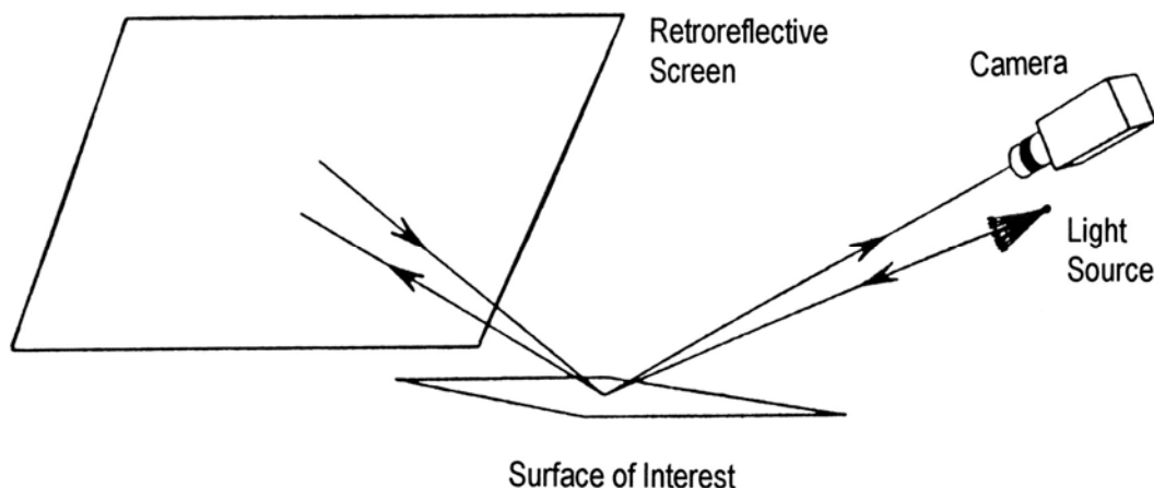
Figure 34.19-1 - D sight - Diffracto sight schematic
