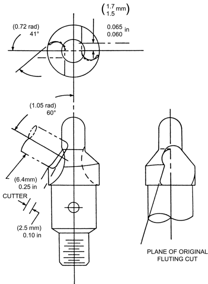
Figure 39.6-1 - Countersink for aramid/epoxy composite
