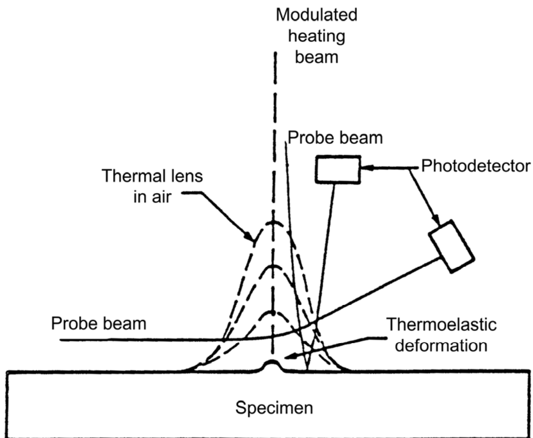
Figure 34.15-2 - Thermal-wave imaging: Photo-optical detection
