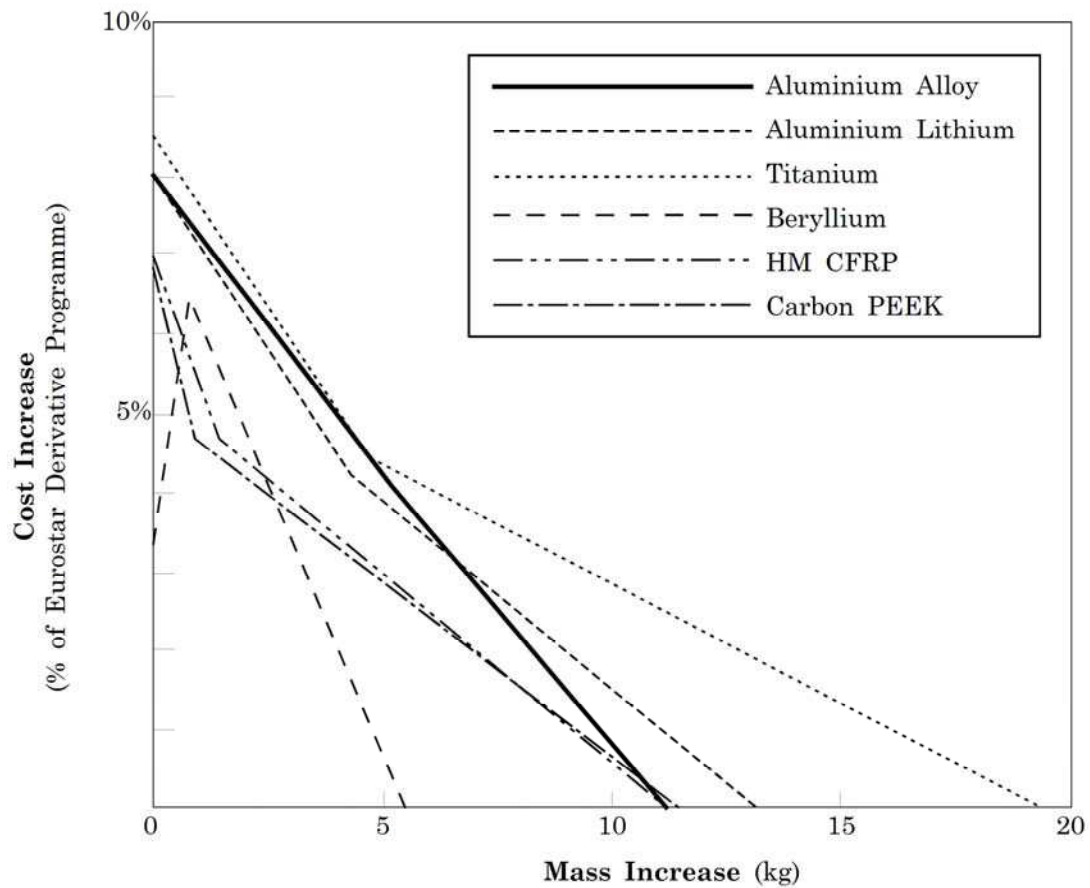
Figure 40.3-1 - Mass/cost sensitivity for central thrust structure
