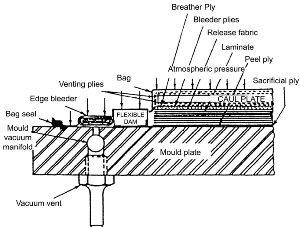
Figure 38.4-1 - Vacuum bag moulding method, with vertical bleeder
