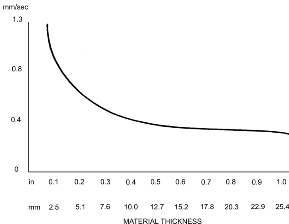
Figure 39.5-2 - Circular sawing: Feed rate versus thickness of composite materials
