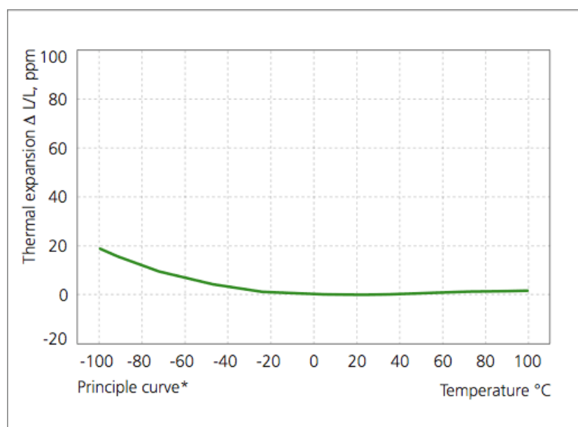
Figure 43.15-15 - ULE®: Thermal expansion characteristics
