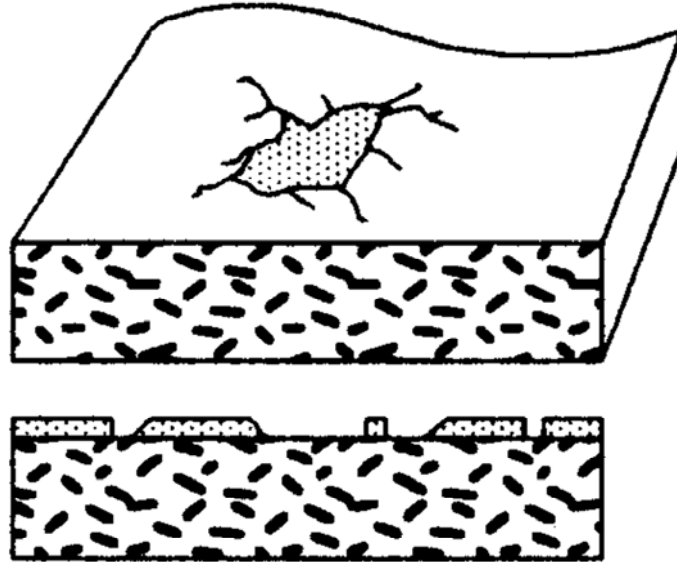
Figure 41.3-3 - Damage categories: Chipping
