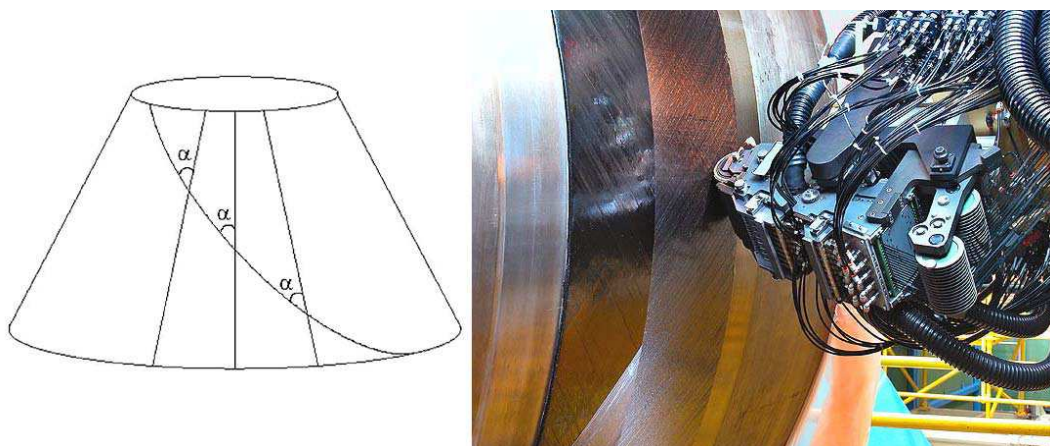
Figure 38.14-6 – Fibre placement: Complex trajectories
