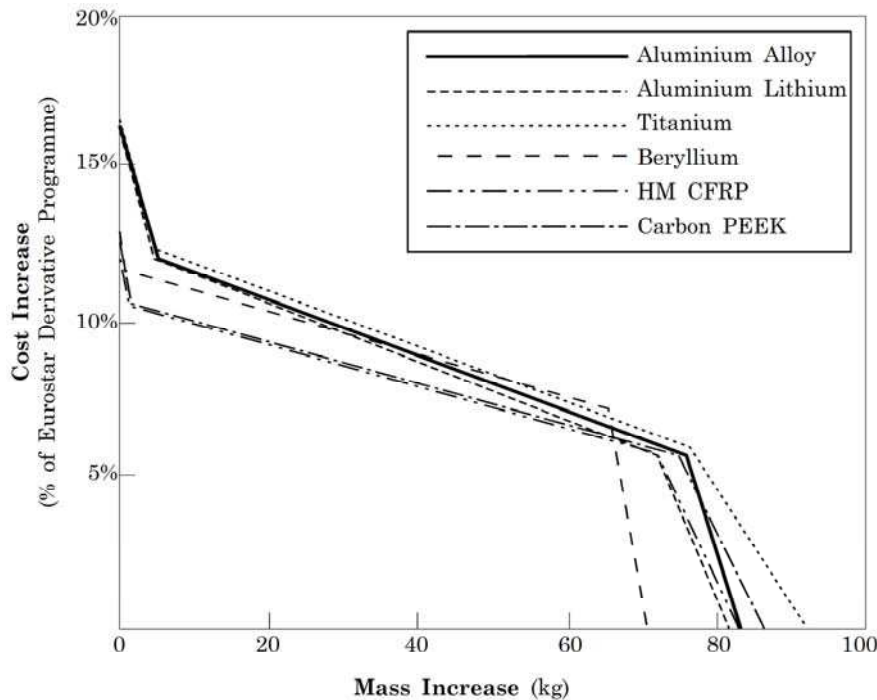
Figure 40.3-2 - Mass/cost sensitivity for complete structure
