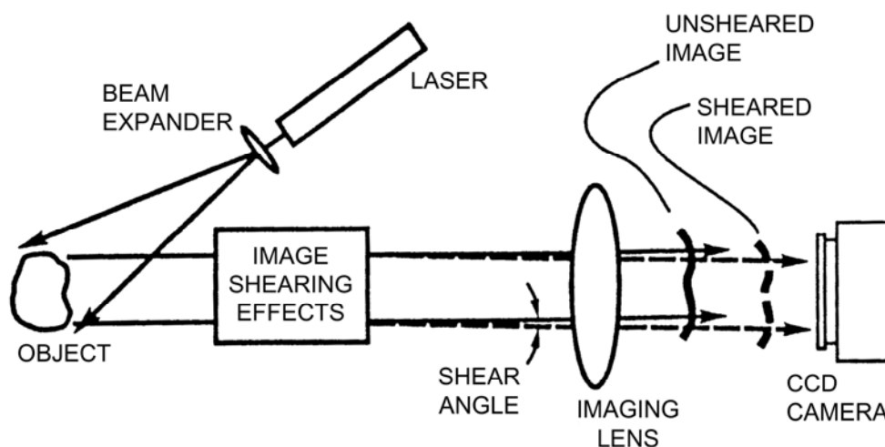
Figure 34.14-1 - Electronic shearographic system: Schematic diagram
