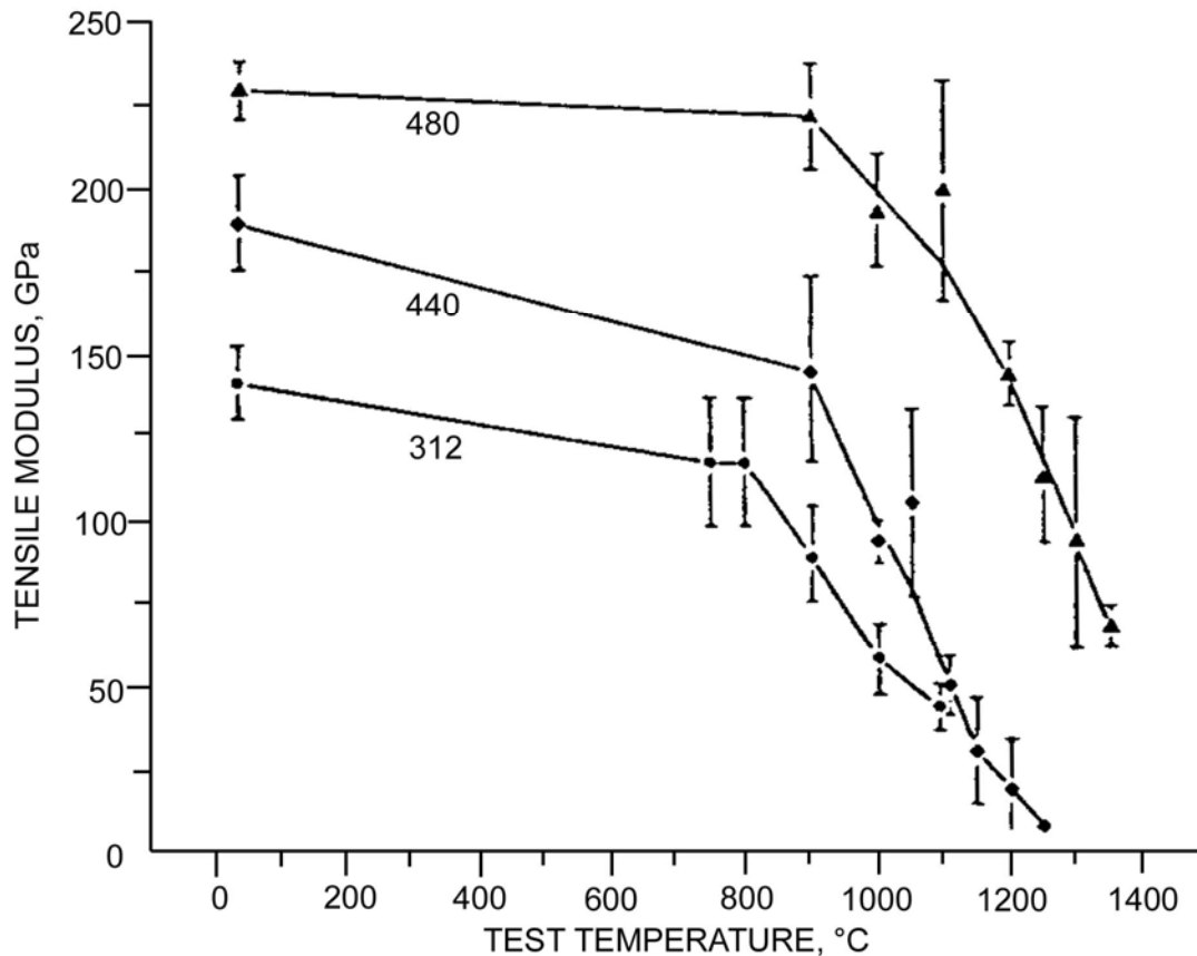
Figure 42.6-13 - Alumina-boria-silica single filament: tensile modulus at elevated temperature in air
