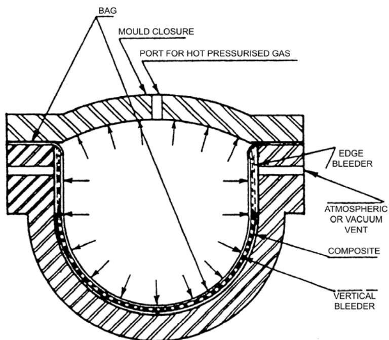
Figure 38.4-2 - Pressure bag moulding
