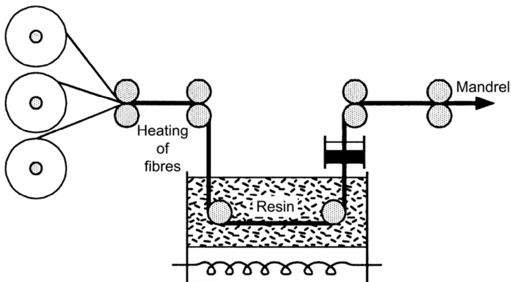
Figure 38.5-1 - Filament winding: Impregnation of fibres
