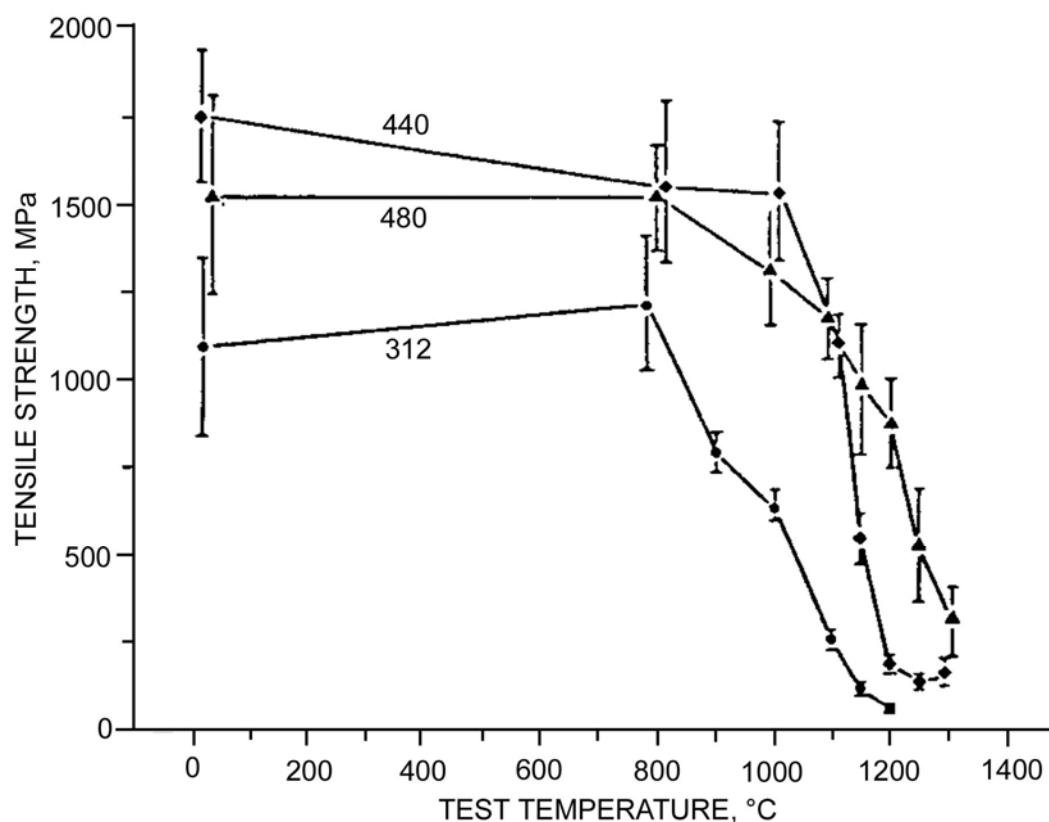
Figure 42.6-12 - Alumina-boria-silica single filament: tensile strength at elevated temperature in air
