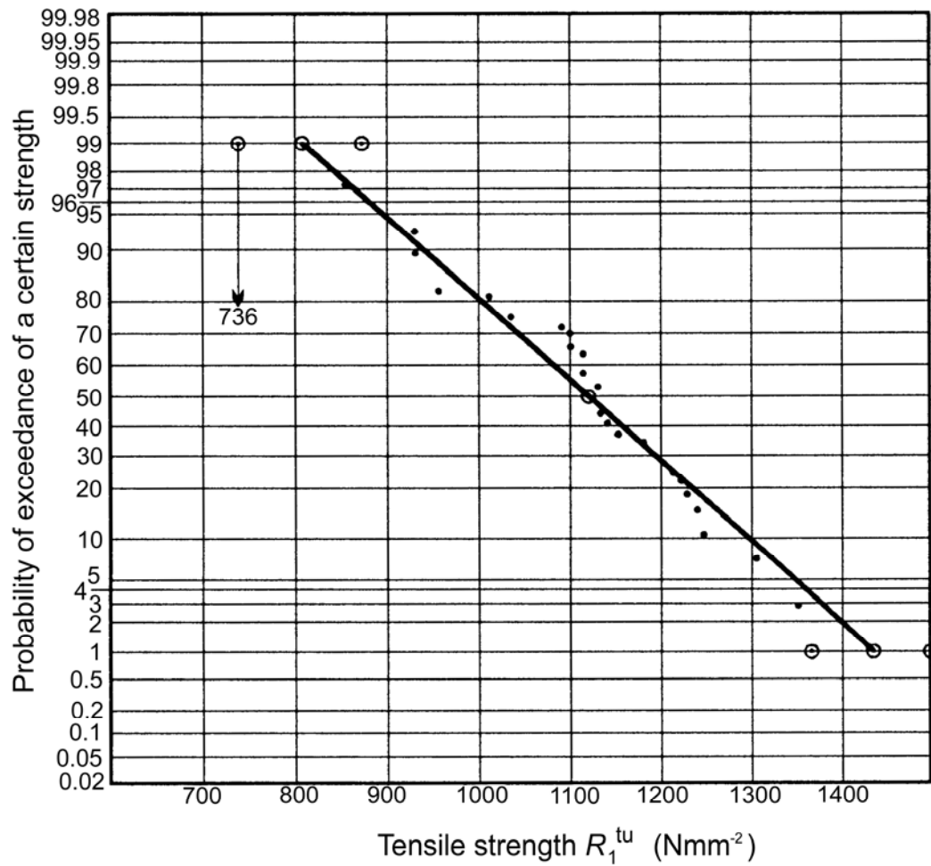
Figure 37.5-1 - Probability of exceedance: Tensile strength 0°
