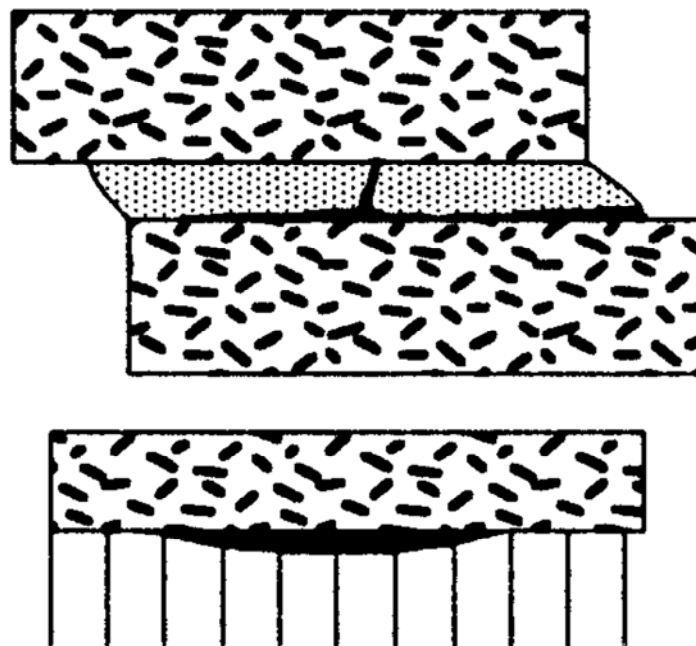
Figure 41.3-4 - Damage categories: Debonding
