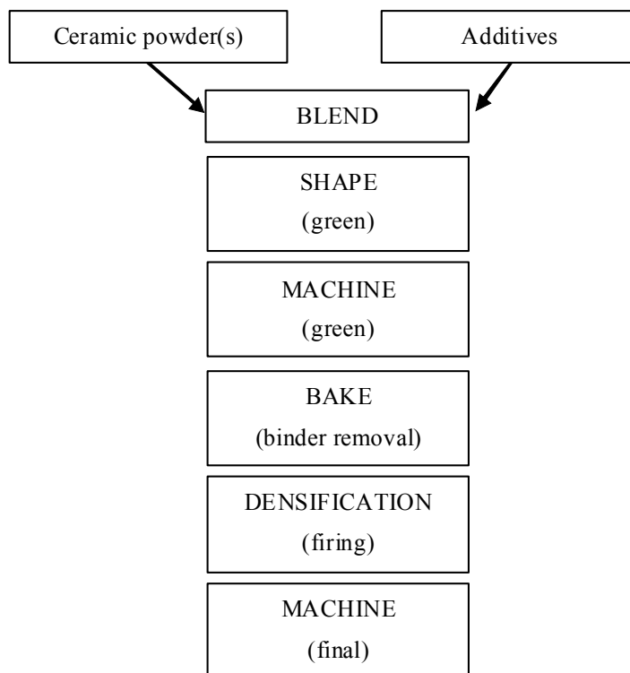
Figure 43.4-1 – Technical ceramics: Manufacturing processes
