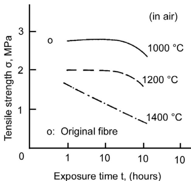
Figure 42.6-5 - SiC Nicalon fibre: tensile strength after high temperature exposure in argon
