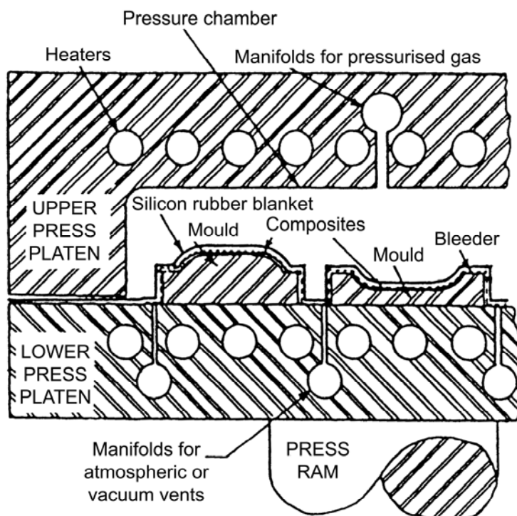
Figure 38.4-3 - Pressure bag moulding: Press modifications
