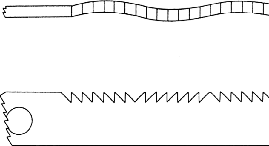
Figure 39.5-3 - Sabre sawing: Alternating tooth blade for aramid/epoxy
