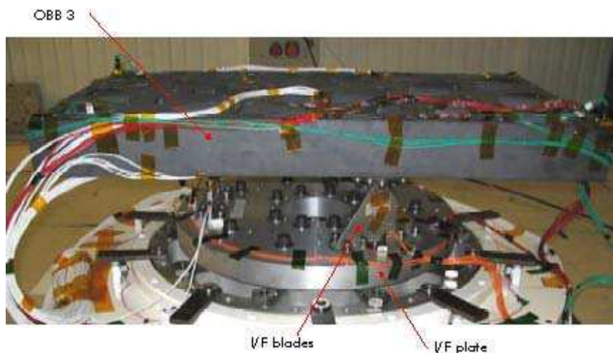
Figure 43.18-4 – NIRSpec optical bench development: Test set-up for 'shaker' vibration tests
