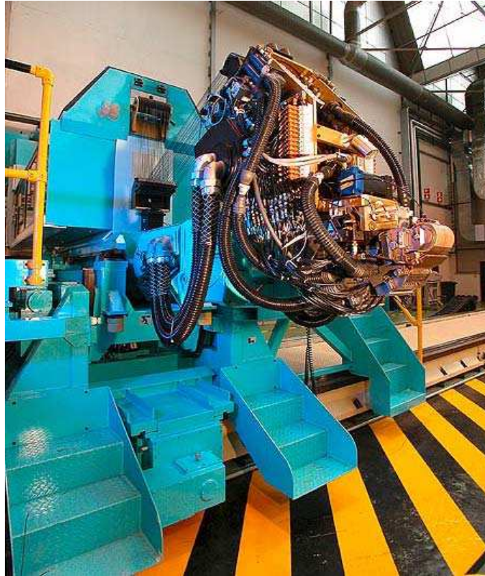
Figure 38.14-2 – Fibre placement: Head
