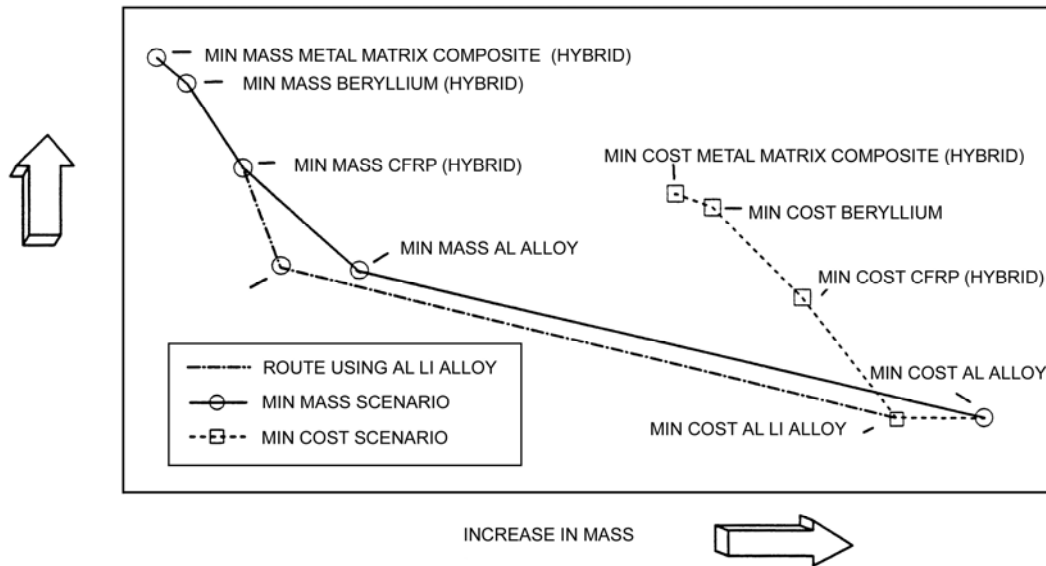
Figure 40.3-3 - Mass to cost envelope for material improvements
