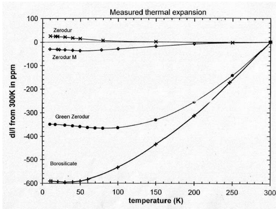
Figure 43.15-8 - Zerodur®: Thermal expansion of different glass ceramics
