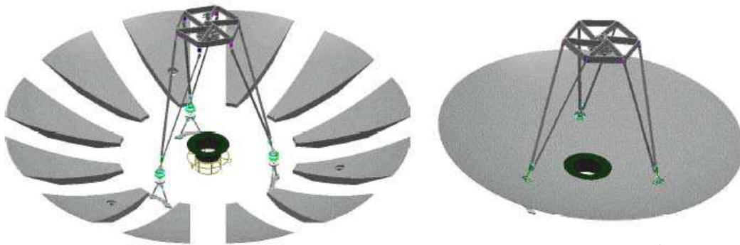
Figure 43.12-11 – SiC-100®: 3.5 m diameter HERSCHEL Primary Mirror – manufactured by brazing 12 SiC segments
