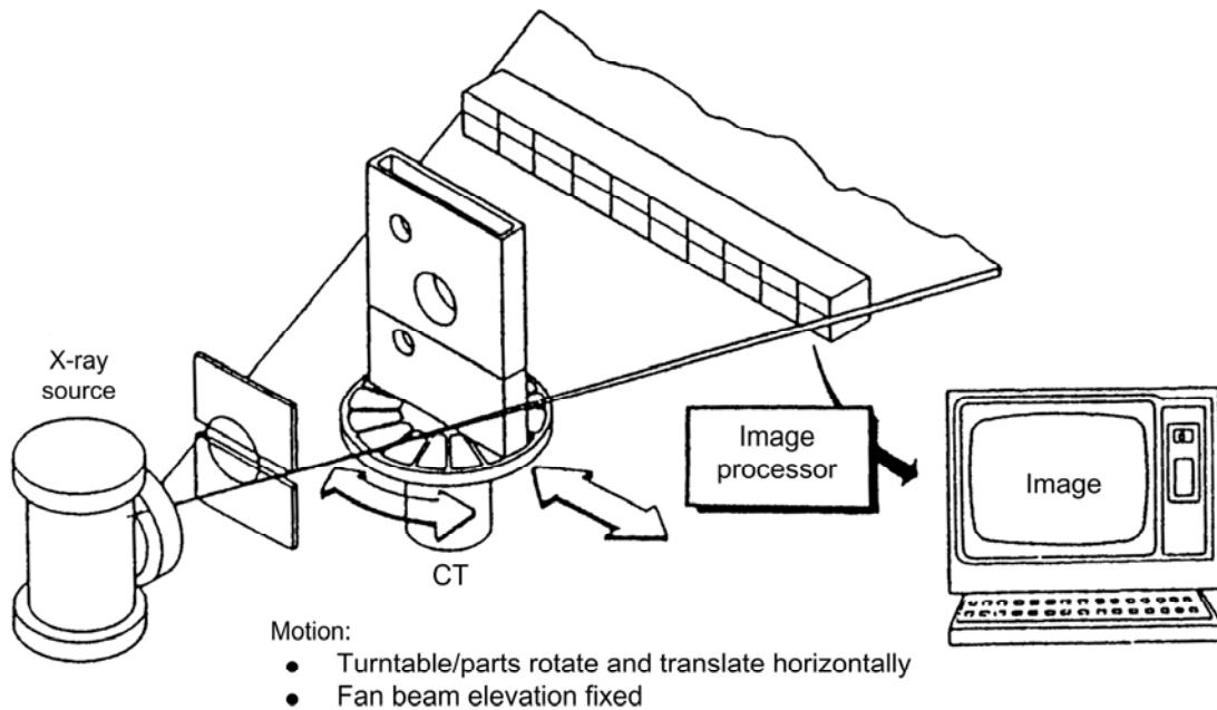
Figure 34.17-1 - Computer tomography facility
