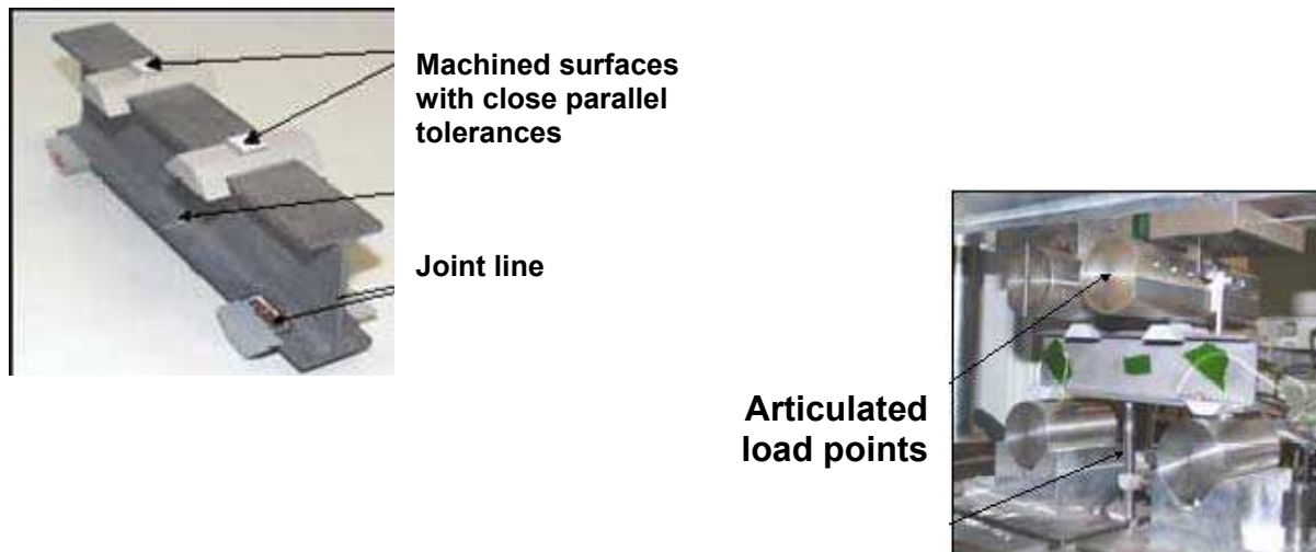
Figure 43.18-2 – NIRSpec optical bench development: Test set-up and I-beam sample with joint line
