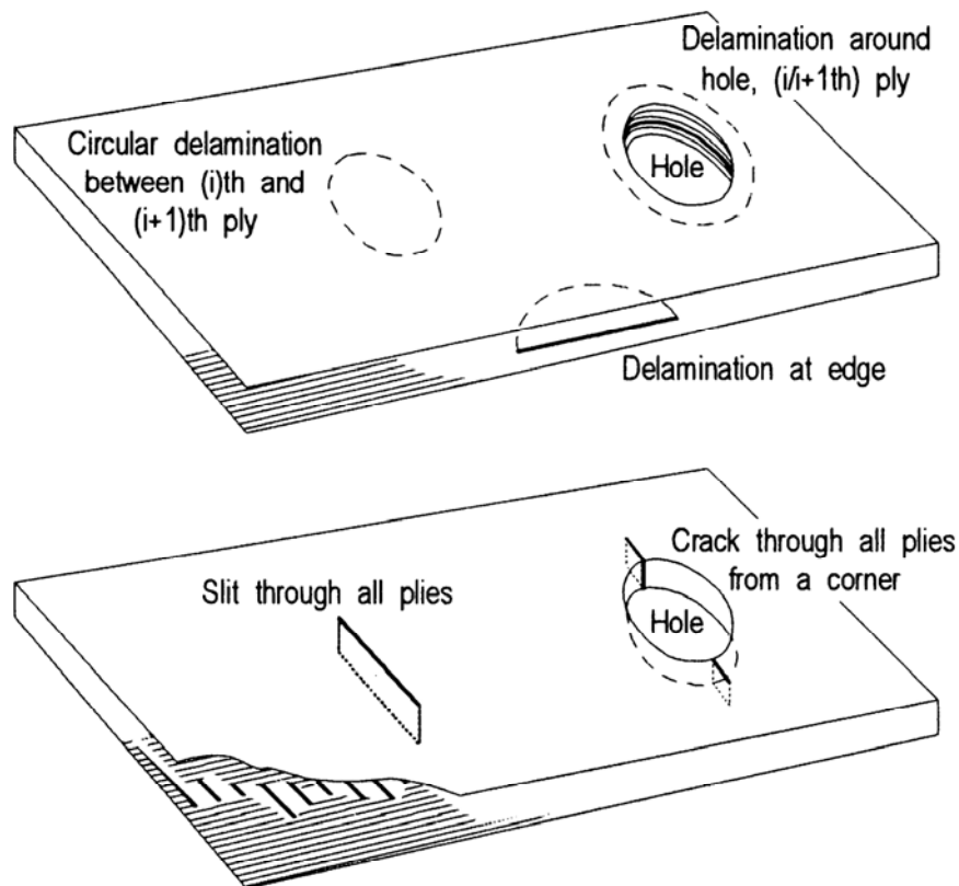
Figure 33.4-2 - Composite structures: Idealisation of defects by standard circular defect
