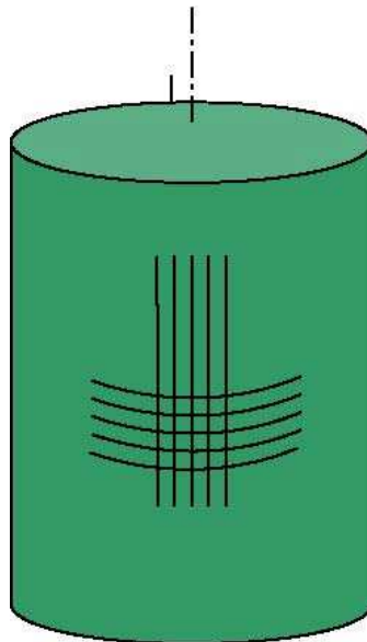
Figure 38.14-5 – Fibre placement: Specific orientations
