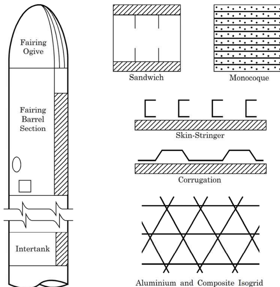
Figure 40.6-1 - Candidate fairing and intertank constructions
