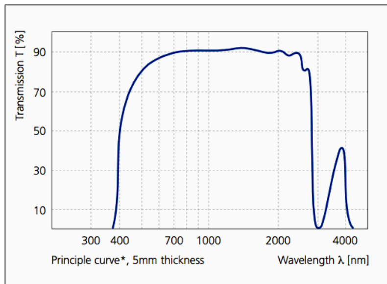
Figure 43.15-5 - Zerodur®: Optical transmission curve
