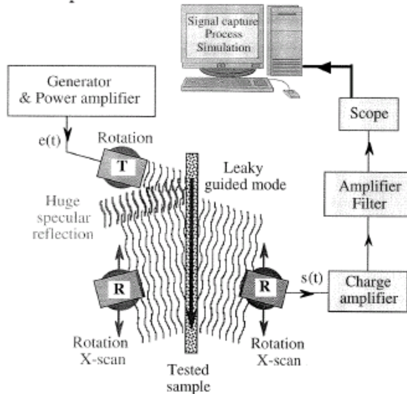
Figure 34.10-6 - Non-contact ultrasonics: Capacitive sensors in plate wave configuration set-up
