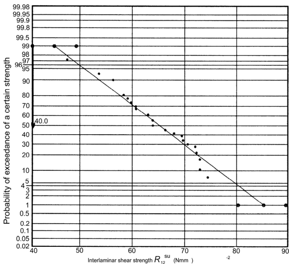
Figure 37.5-4 - Probability of exceedance: Interlaminar shear strength
