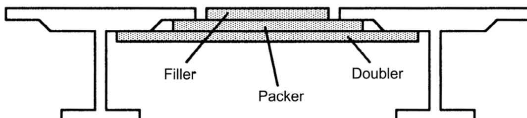
Figure 41.7-1 - Bolted and bonded repair using a composite patch
