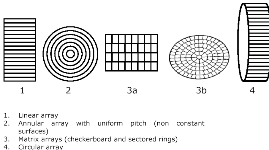
Figure 34.10-3 – Phased-array transducers: Element configurations
