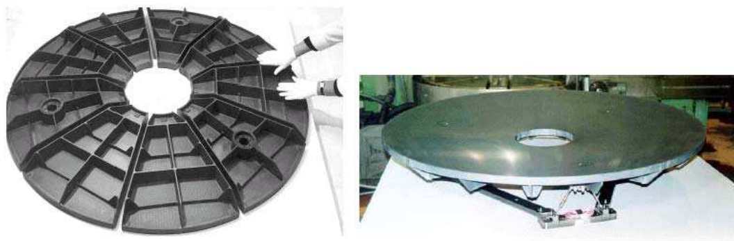
Figure 43.12-10 – SiC-100 ® : 1.35 m diameter HERSCHEL Demonstrator Breadboard – before and after brazing
