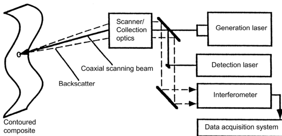
Figure 34.12-1 - Laser ultrasonic test system: Diagrammatic representation
