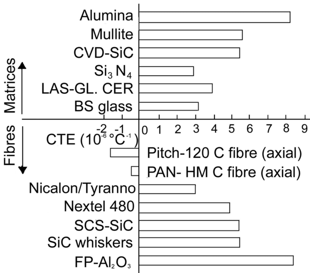
Figure 42.6-15 - Coefficients of thermal expansion for various fibres and matrix materials
