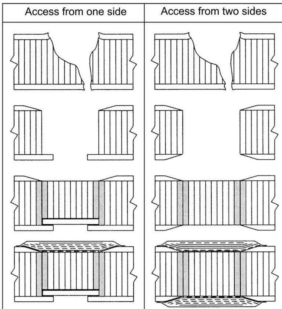
Figure 41.8-1 - Sandwich repair
