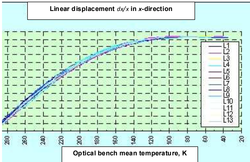
Figure 43.18-7 – NIRSspec optical bench development: Linear displacement under cryogenic test
