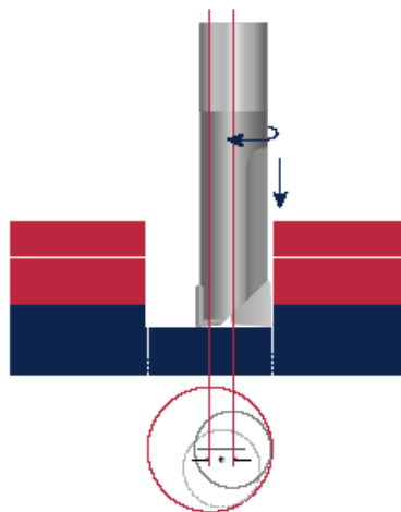
Figure 39.10-1 – Orbital drilling principle
