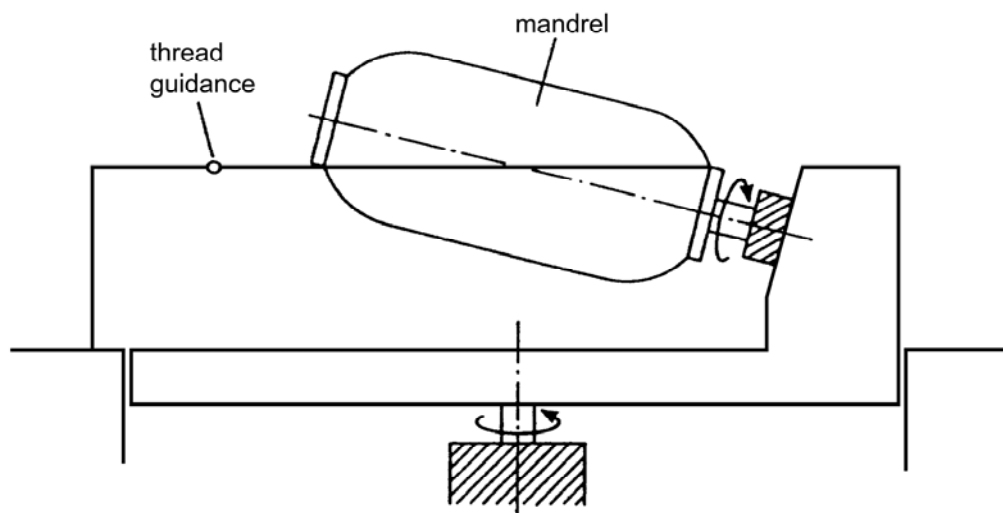
Figure 38.6-3 - Filament winding: Polar tumbling
