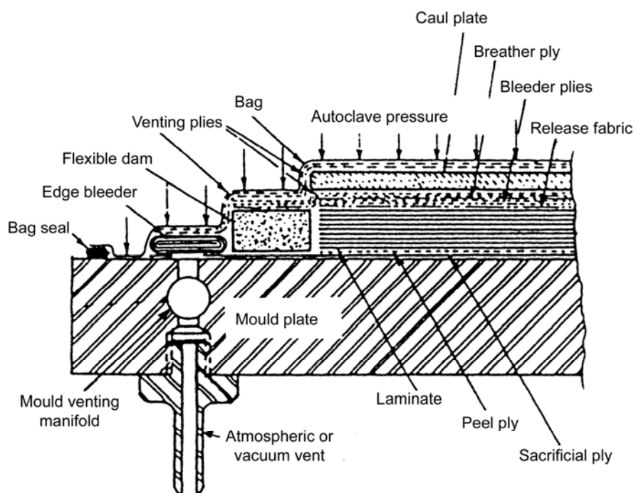
Figure 38.4-4 - Autoclave moulding method, with vertical bleeder
