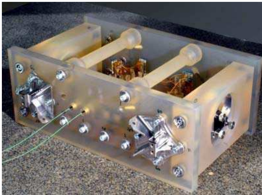
Figure 43.19-1 – Zerodur®: Optical bench for LISA pathfinder mission
