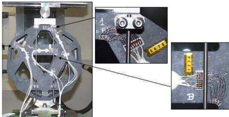
Figure 43.18-3 – NIRSpec optical bench development: Test set-up for instrumented bench cells
