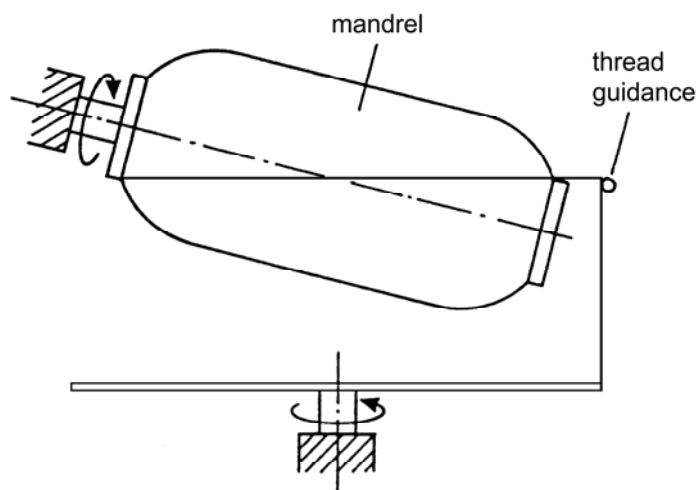
Figure 38.6-2 - Filament winding: Polar horizontal
