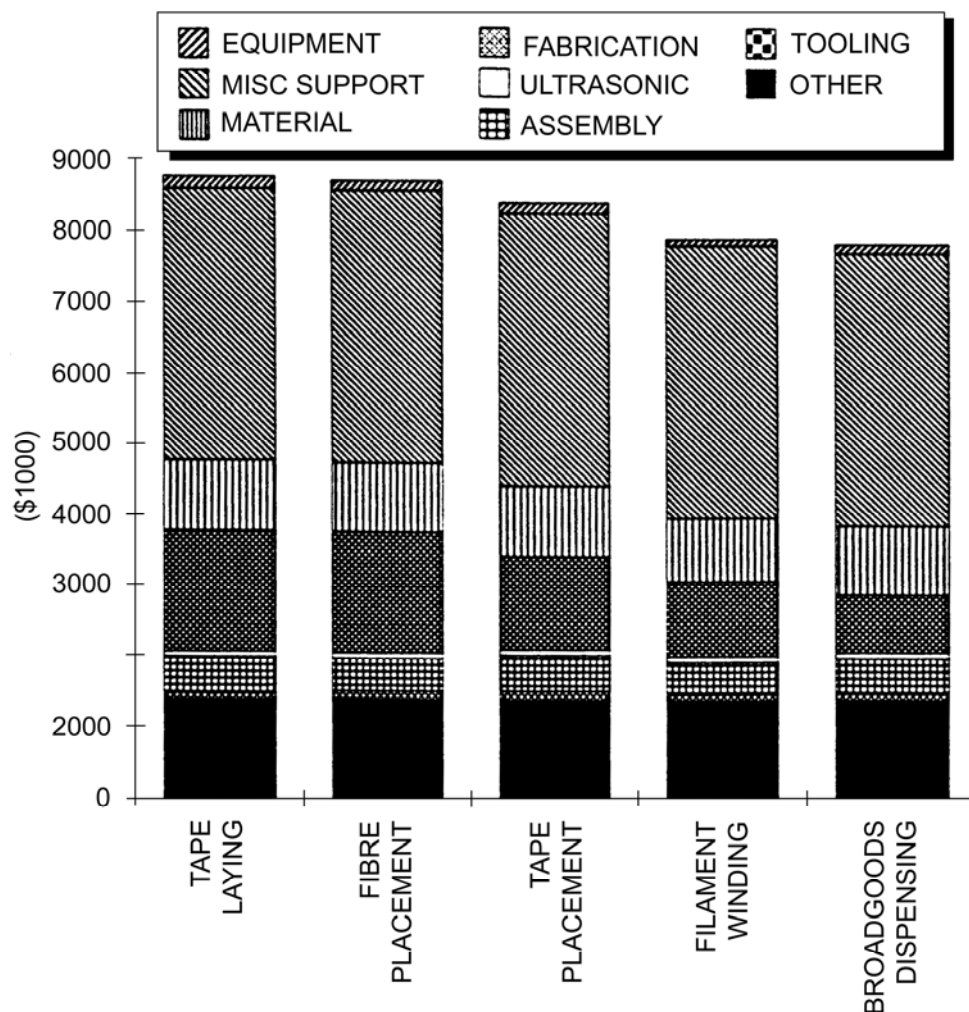
Figure 40.6-4 - Launcher fairing: Unit life cycle costs for sandwich fairing cylinder designs for different fabrication processes
