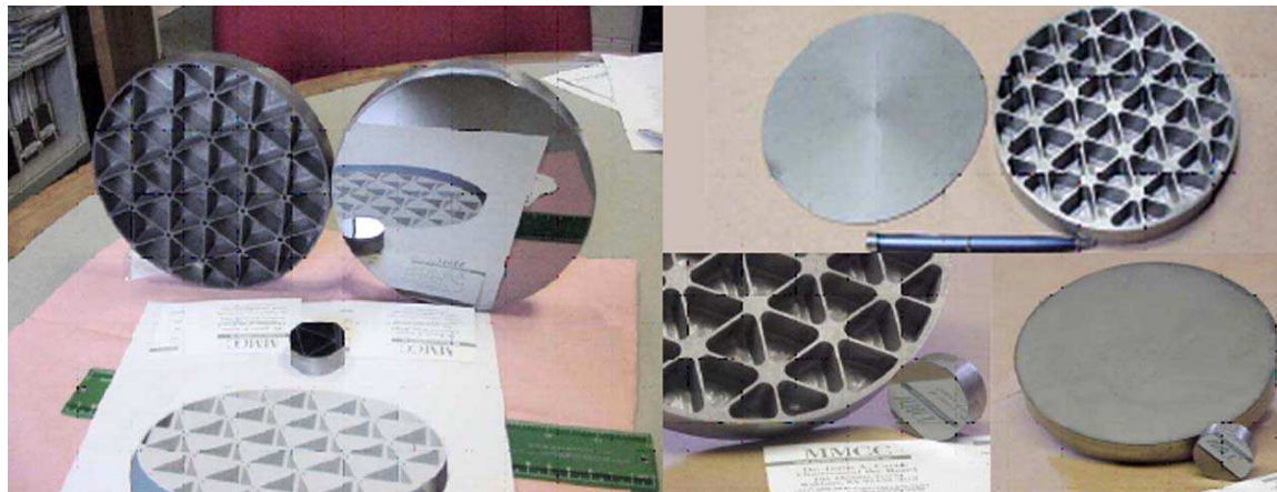
Pre-polished Si membrane bonded to lightweighted substrate. Areal density = 9.7 \text{ kg/m}^2
