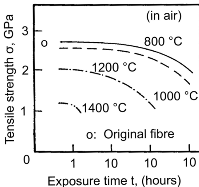
Figure 42.6-4 - SiC Nicalon fibre: tensile strength after high temperature exposure in air
