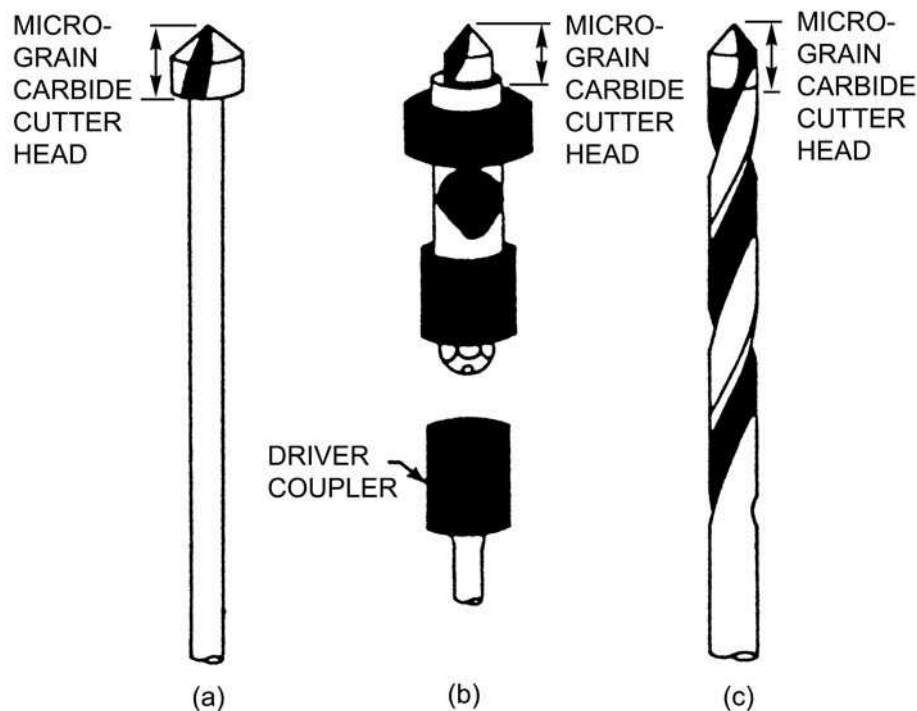
(a) Solid shank drill, (b) Drill guide system, (c) Fluted twist drill
