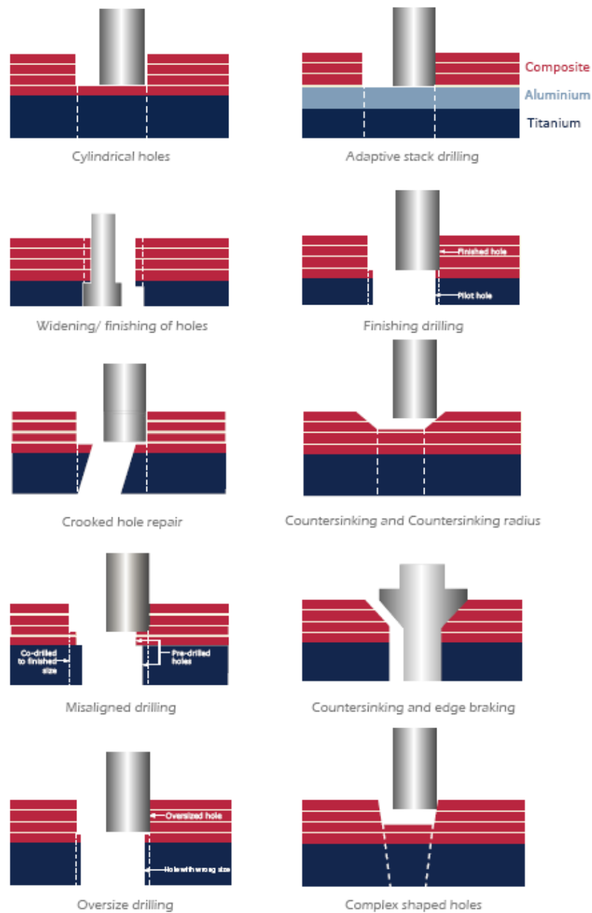
Figure 39.10-3 – Orbital drilling: Application examples
