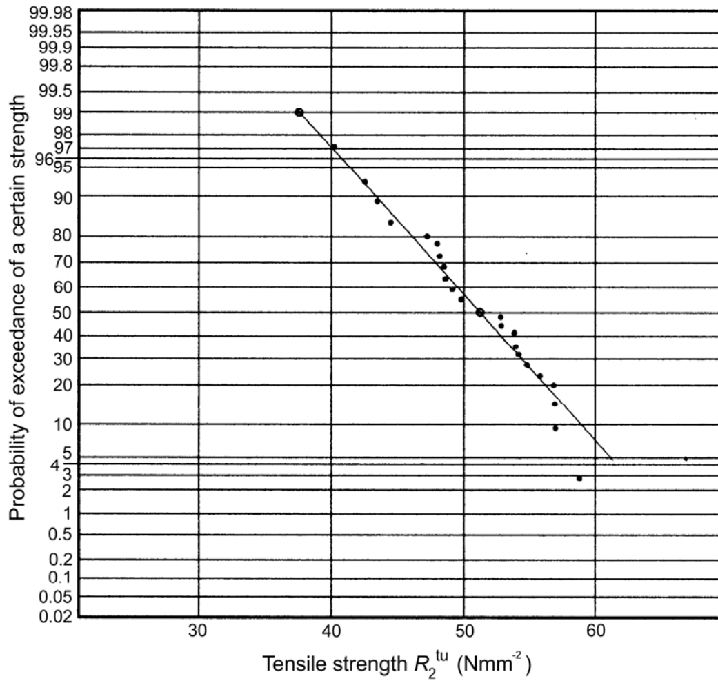
Figure 37.5-2 - Probability of exceedance: Tensile strength 90°
