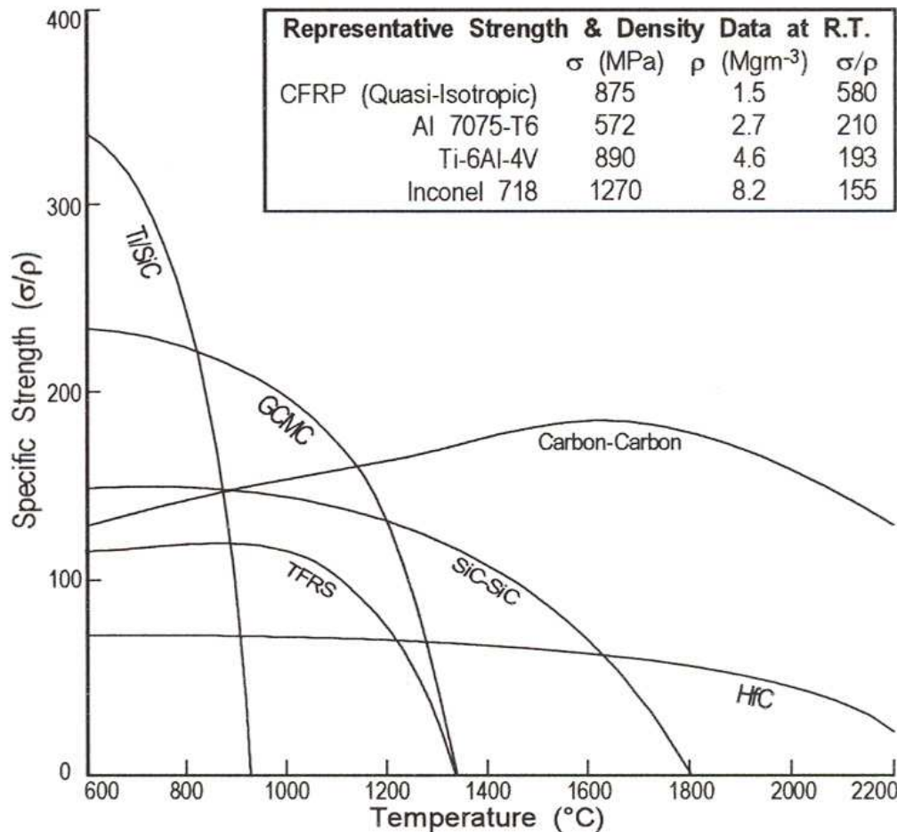
Figure 42.2-2 - Specific strength against temperature for advanced materials
