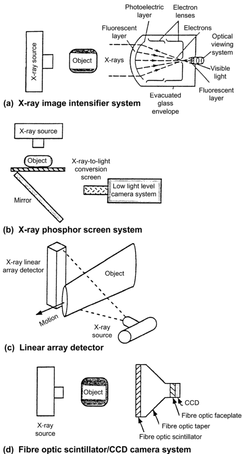
Figure 34.16-1 - Typical digital radiography systems
