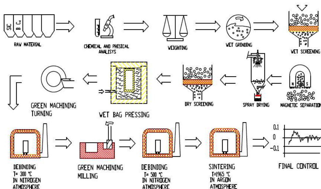
Figure 43.12-5 – SiC 54S® ceramic: Process sequence
