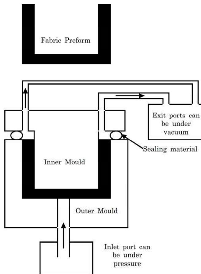
Figure 38.7-1 - Resin transfer moulding (RTM): Process
