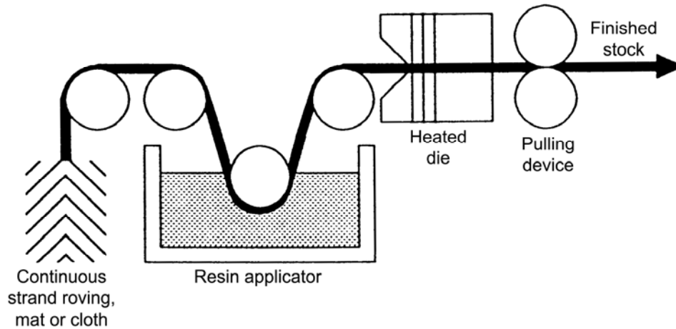
Figure 38.8-1 - Pultrusion: Basic process
