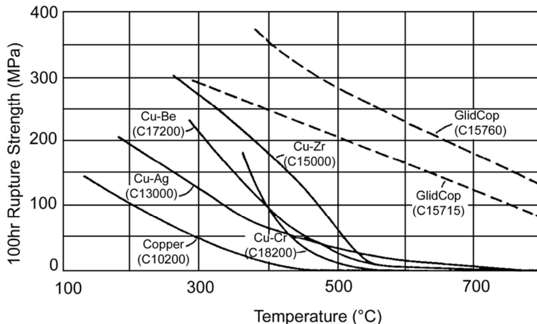
Figure 45.3-1 - Copper ODS alloys: Elevated temperature stress-rupture properties of Glidcop ODS alloys compared with some high conductivity copper alloys
