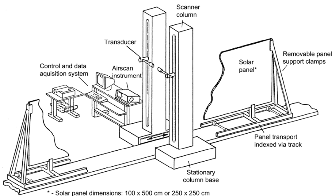
Figure 34.10-7 – Airscan™ (air-coupled ultrasonics) system: Non-contact NDI of Fokker solar panel substrates
