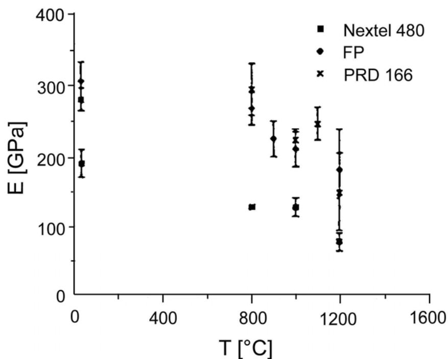
Figure 42.6-9 - Alumina fibres: modulus at elevated temperature
