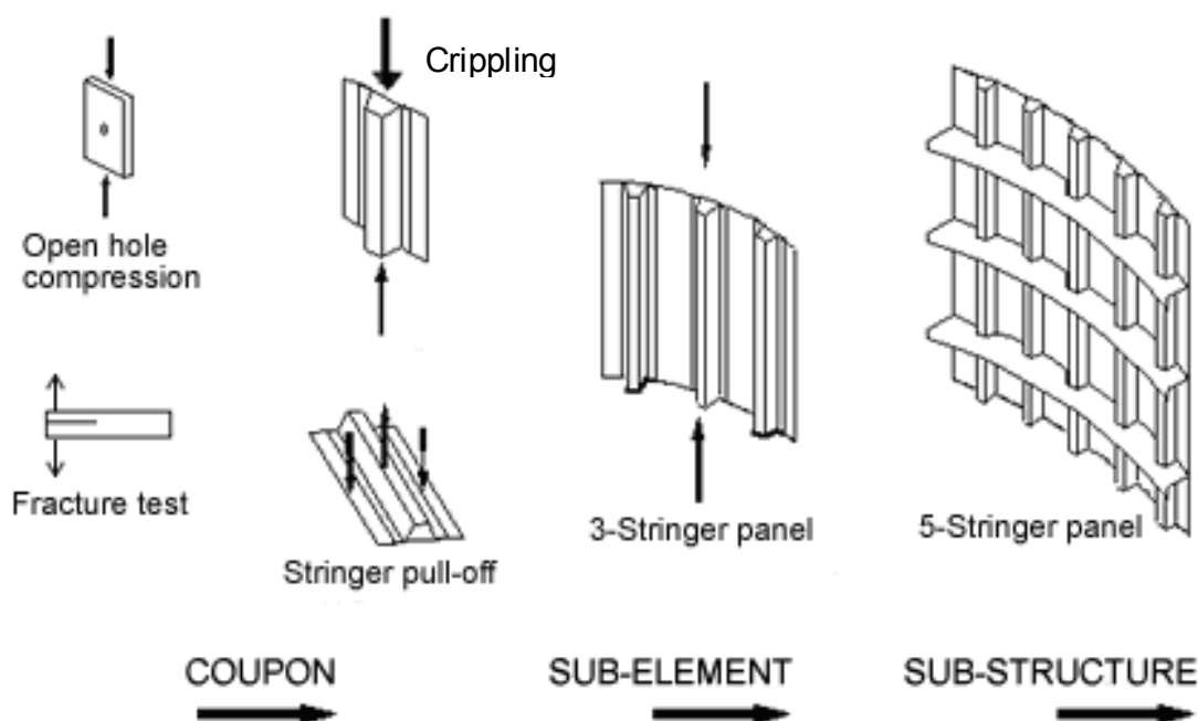
Figure 33.6-1 - Building block approach: Test programme development
