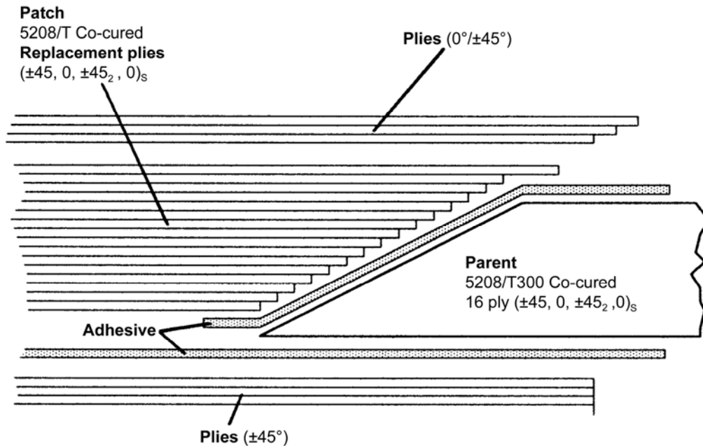
Figure 41.5-3 - Flush repair with adhesive film and cover plies
