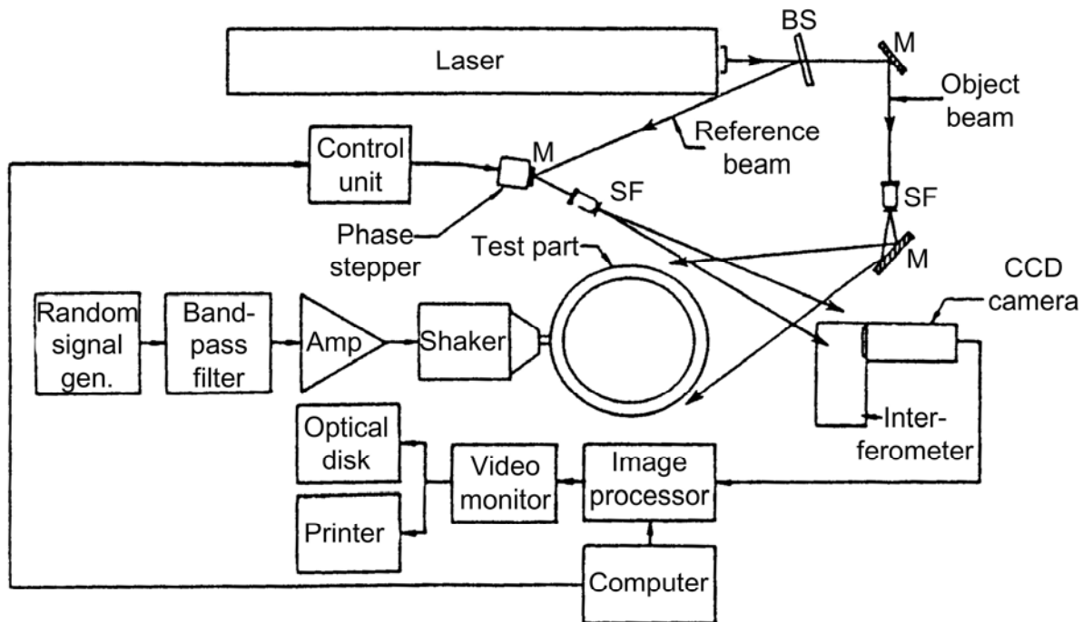
Figure 34.13-1 - Holography by electronic imaging with random vibration excitation
