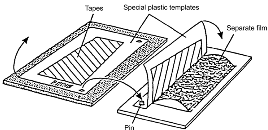
Figure 38.3-3 - Prepreg: Indirect lay-up
