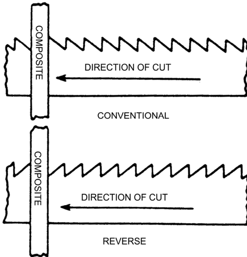
Figure 39.5-1 - Reverse bandsawing aramid/epoxy laminates
