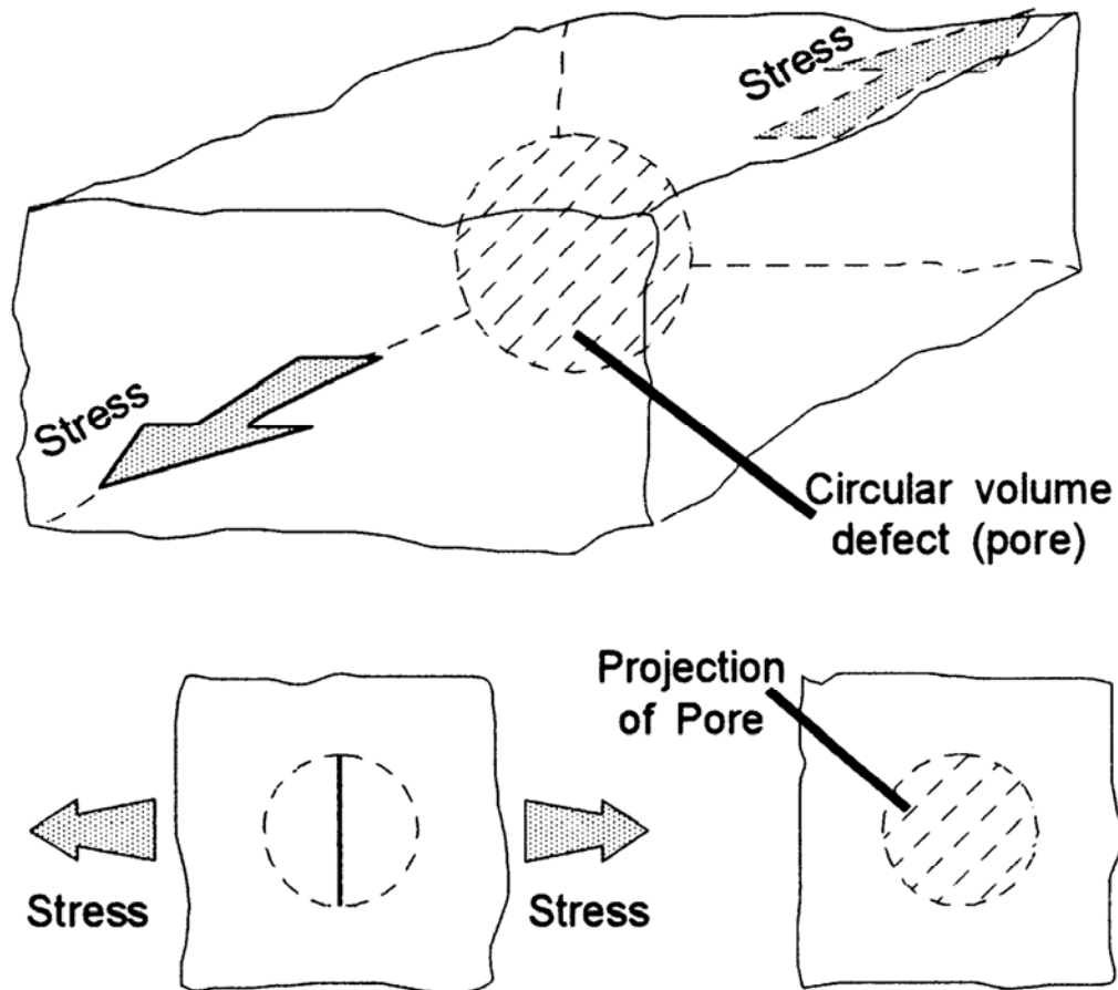
Figure 33.4-1 - Metal structures: Idealisation of a volumetric defect
