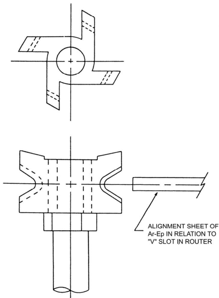
Figure 39.3-2 - Router for trimming aramid/epoxy composites
