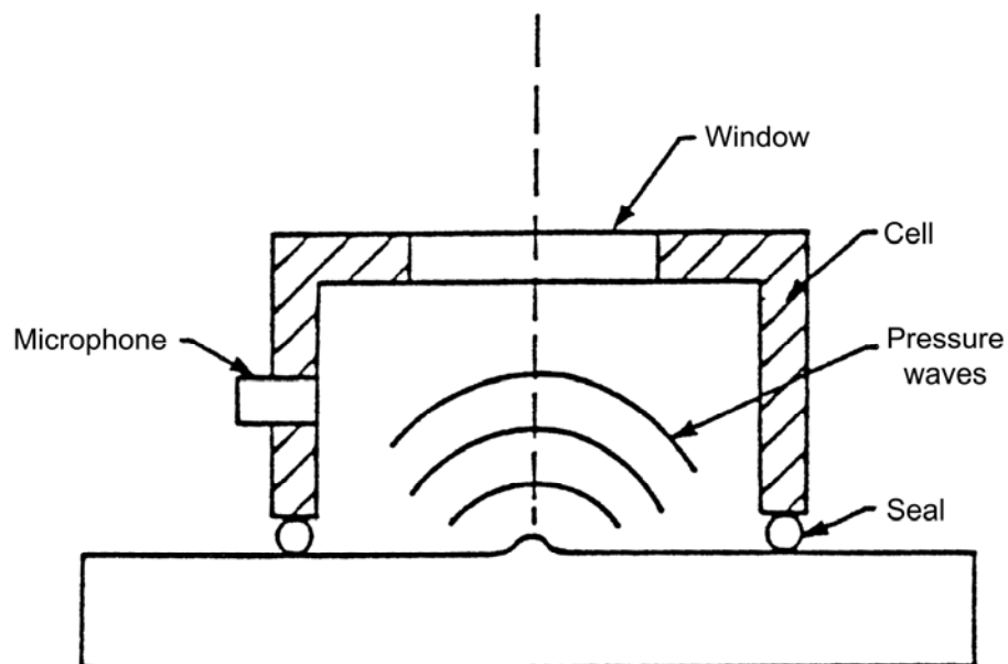
Figure 34.15-4 - Thermal-wave imaging: Photoacoustic gas cell
