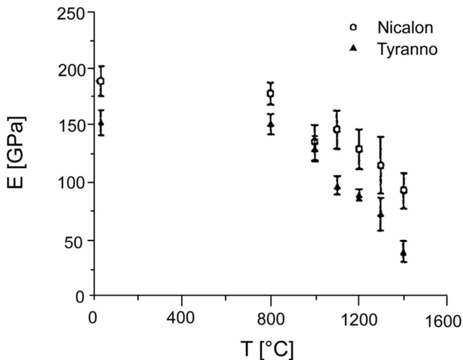
Figure 42.6-7 - SiC fibres Nicalon and Tyranno: modulus at elevated temperature
