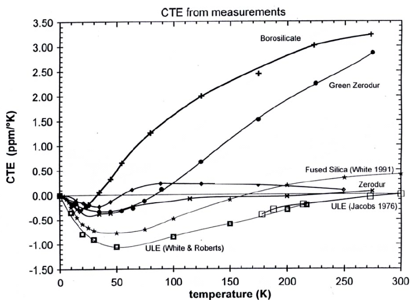
Figure 43.15-7 - Zerodur®: Coefficient of thermal expansion – different glass ceramics
