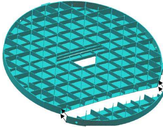
Figure 43.12-9 – SiC-100 ® : 1m diameter ‘Demonstration Mirror’ – green part joining by ceramic bonding
