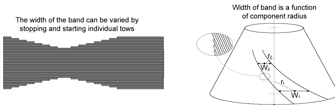
Figure 38.14-7 – Fibre placement: Variation of band width
