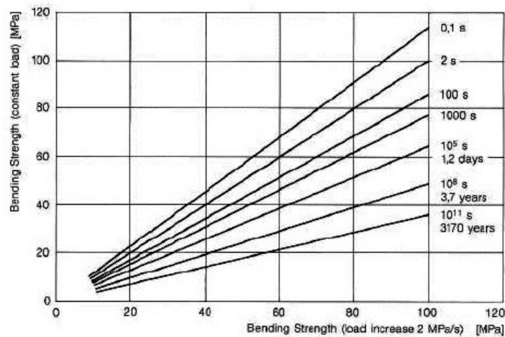
Figure 43.15-13 - Zerodur®: Bending strength under constant load
