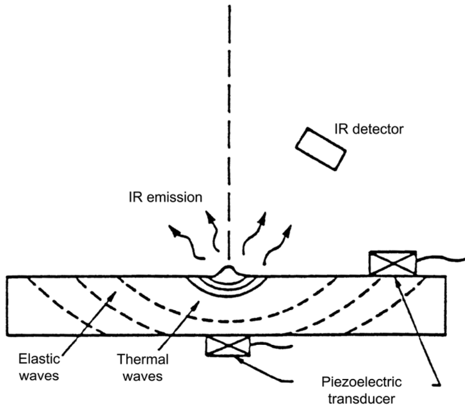
Figure 34.15-3 - Thermal-wave imaging: Photothermal and piezoelectric detection
