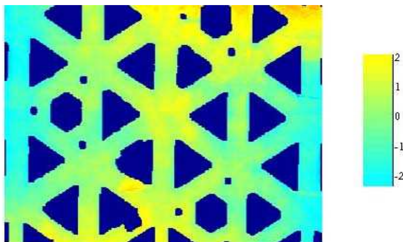
Figure 43.18-8 – NIRSspec optical bench development: Out-of-plane displacement under cryogenic test
