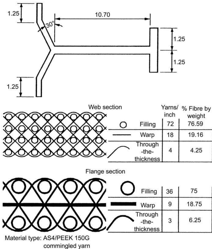
Figure 38.13-1 - Preform technology: Architecture of woven commingled AS4/PEEK 150g 0°/90°
