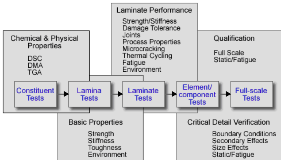
Figure 33.6-2 - Building block approach: Composite materials
