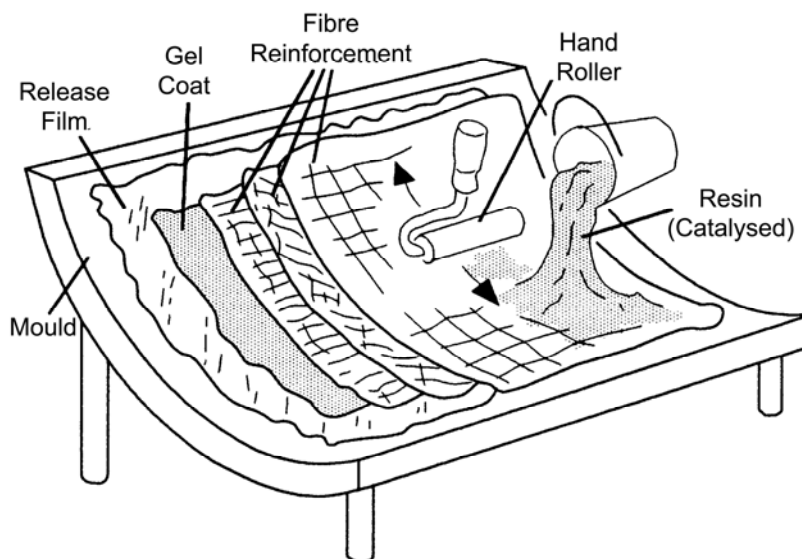
Figure 38.3-1 - Hand lay-up process for mat or cloth
