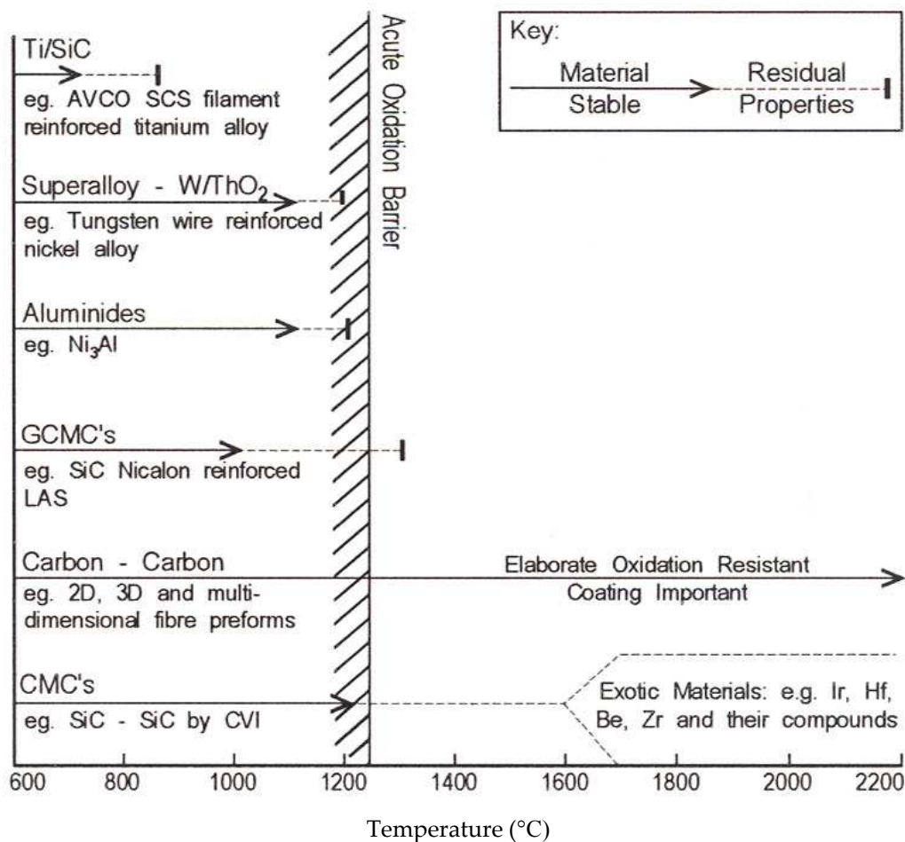
Figure 42.2-1 - Classification of advanced metallic and ceramic materials with temperature
