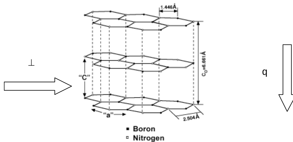
Figure 43.9-1 – Technical ceramics: pyrolytic boron nitride – structure
