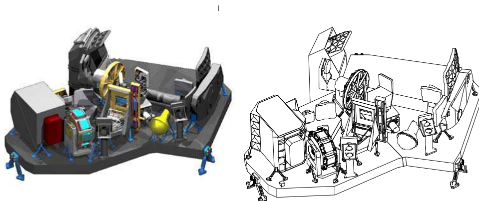
Figure 43.12-14 – SiC-100®: Optical Assembly of NIRSpec for James Webb Space Telescope
