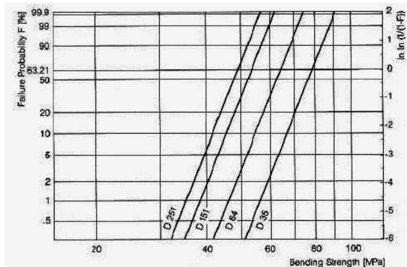
Figure 43.15-10 - Zerodur®: Failure probability for test surfaces processed with bonded grit of different sizes
