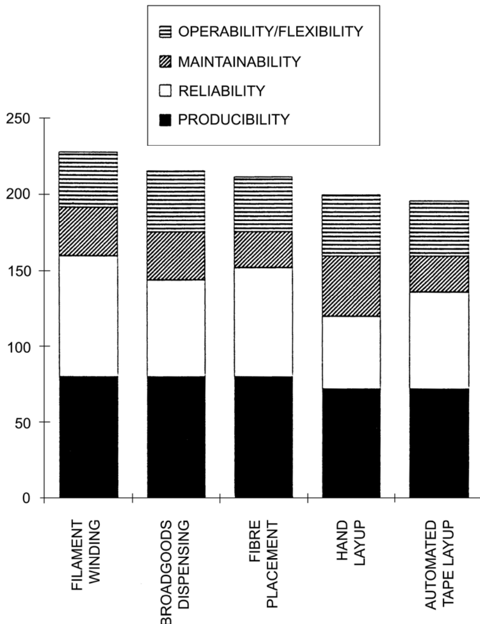
Figure 40.6-5 - Launcher fairing: Kepner-Tregoe evaluation scores for processes to fabricate the monocoque and sandwich cylinder
