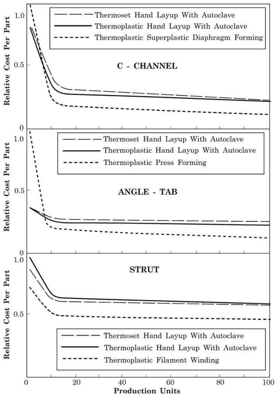
Figure 40.7-1 - Thermoplastic components: Manufacturing unit costs as a function of production volumes
