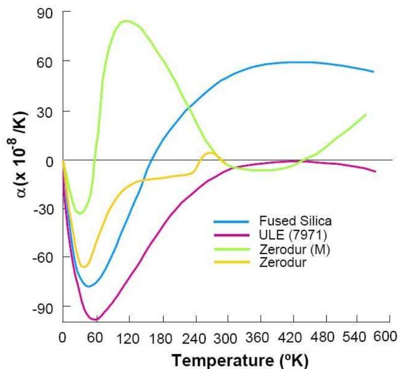
Figure 43.15-1 - Glass ceramics: Coefficient of thermal expansion with temperature - materials for optical instruments in space
