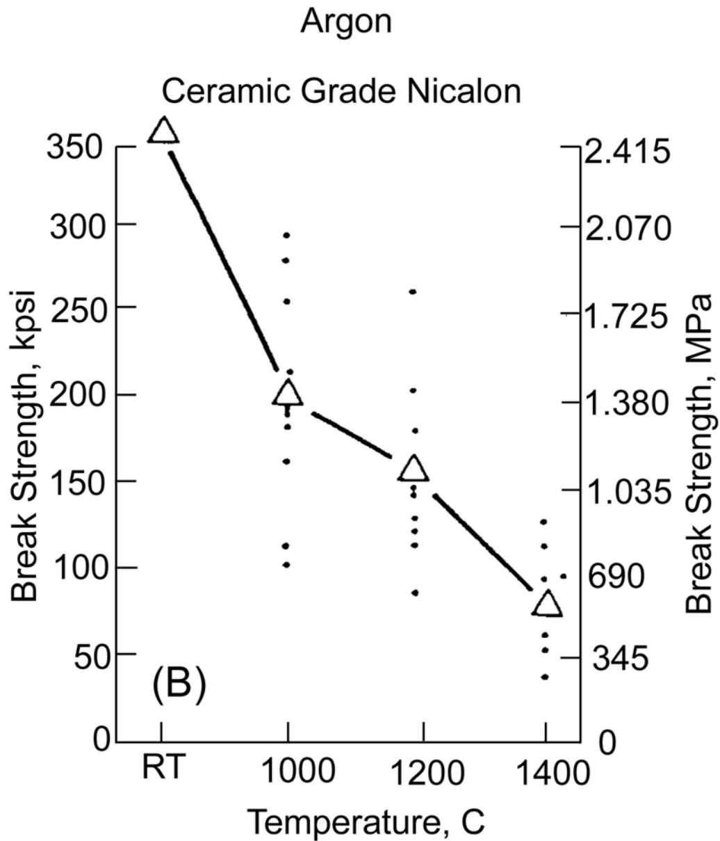
Figure 42.6-3 - SiC Nicalon ceramic grade fibre: tensile strength at elevated temperature
