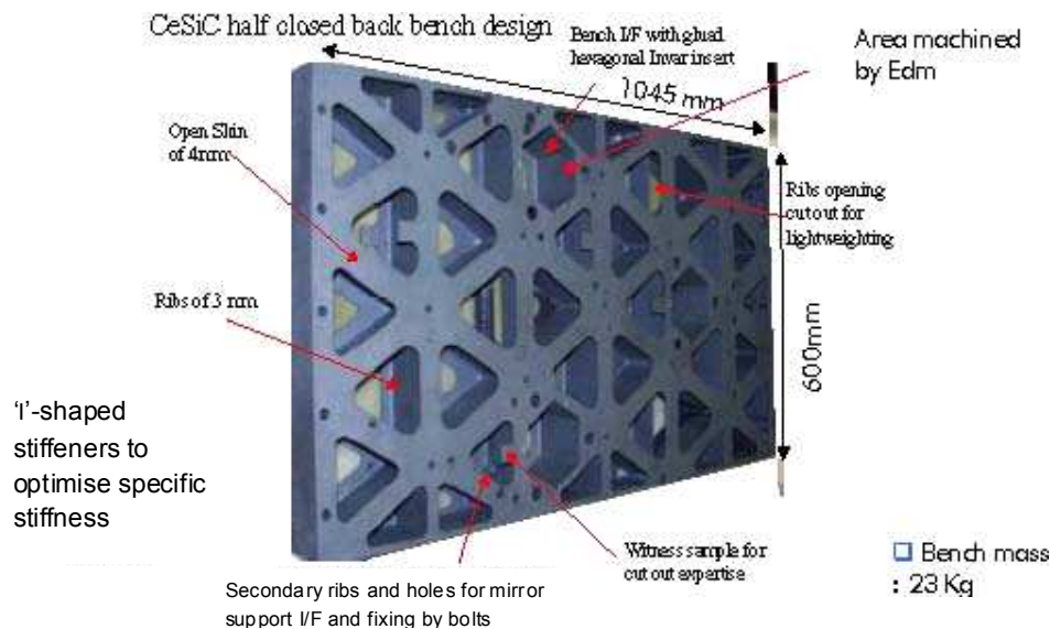
Figure 43.18-1 – NIRSpec optical bench development: Ceric® ceramic demonstrator structure
