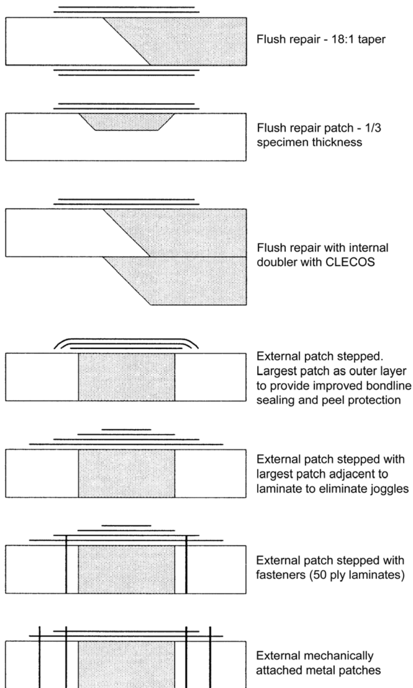
Figure 41.4-1 - Basic repair concepts
