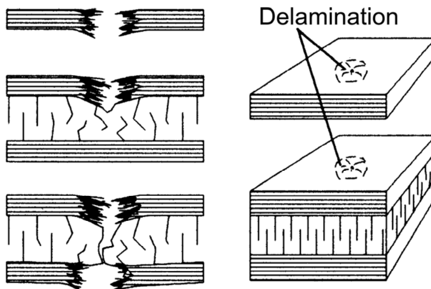
Figure 41.3-6 - Damage categories: Perforation
