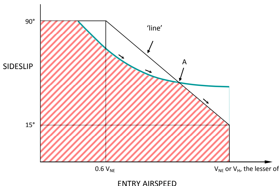
Figure 1 — YAW/FORWARD SPEED DIAGRAM
