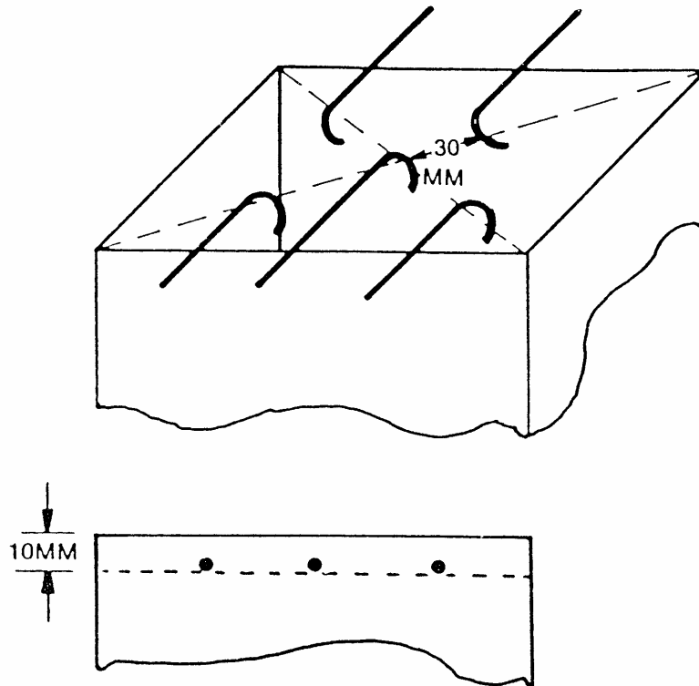
FIGURE 5. THERMOCOUPLE POSITION
