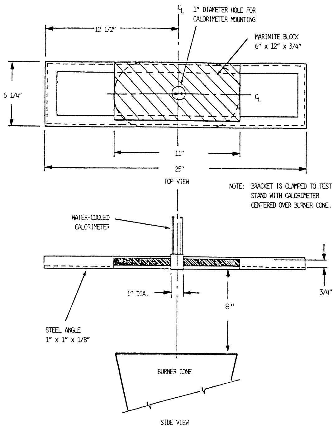
FIGURE 2 CALORIMETER BRACKET
