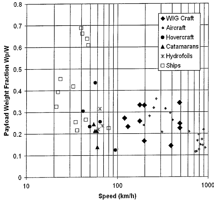
Figure 17 Payload Fraction versus Speed [24]
