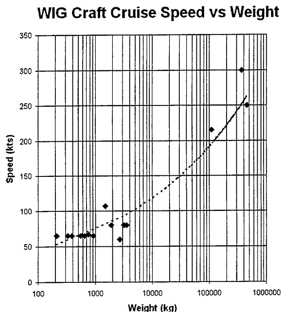
Figure 20 Cruise Speed versus WIG Craft Weight.
