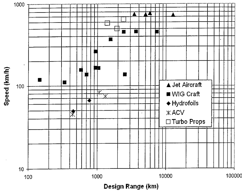
Figure 16 Range and Speed of WIG craft [25]
