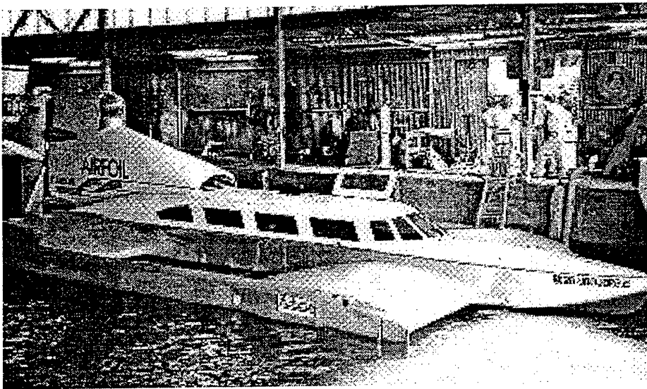
Figure 10 Tandem Wing Craft by Jorg
