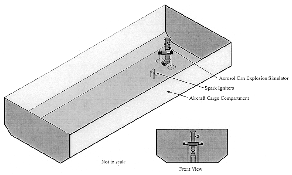
Figure 10. Aerosol Can Explosion Simulation Test Setup (Short Version)
