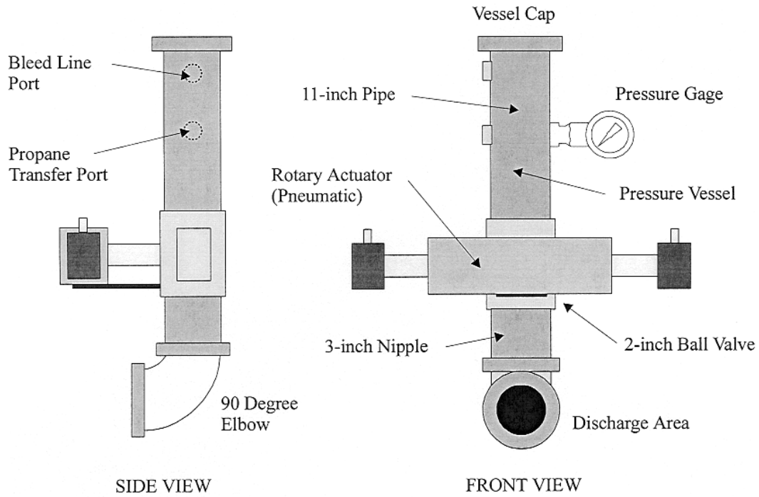
Figure 8. Aerosol Can Explosion Simulator
