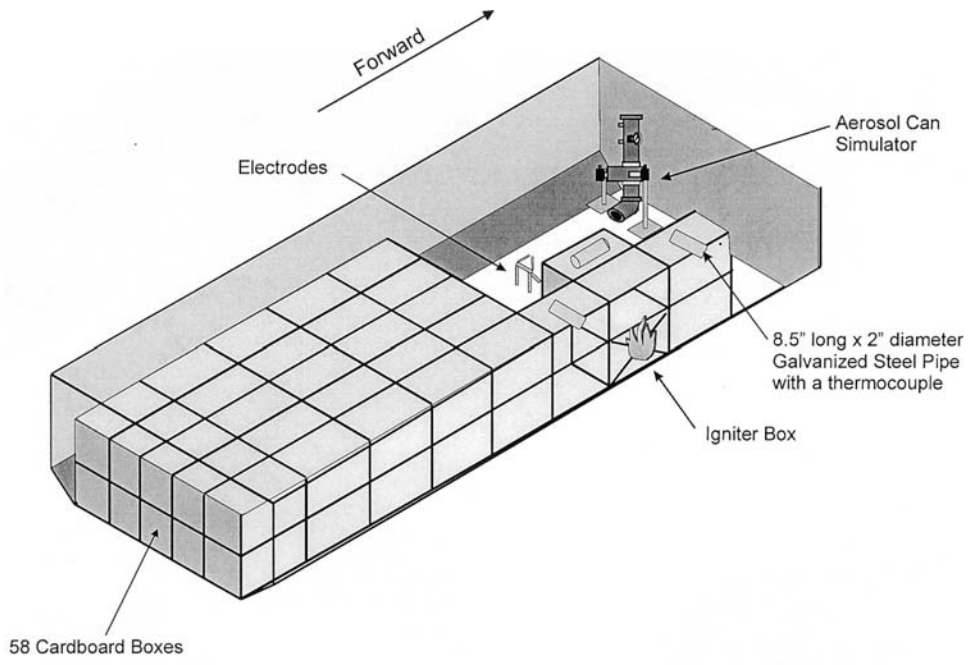
Figure 9. Aerosol Can Explosion Simulation Test Setup
