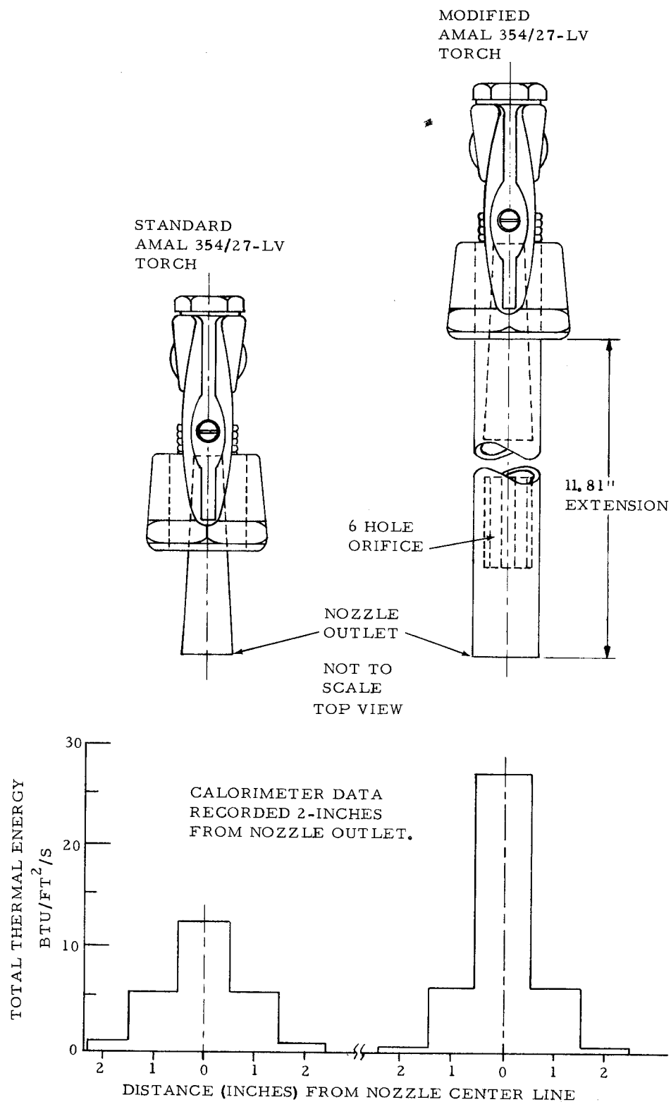
FIGURE 23. AMAL PERIPHERY Btu/ft 2 /s PROFILE
