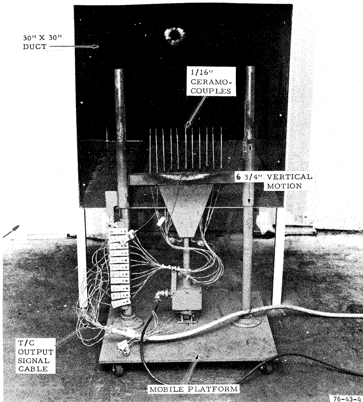
FIGURE 5. THERMOCOUPLE RAKE
