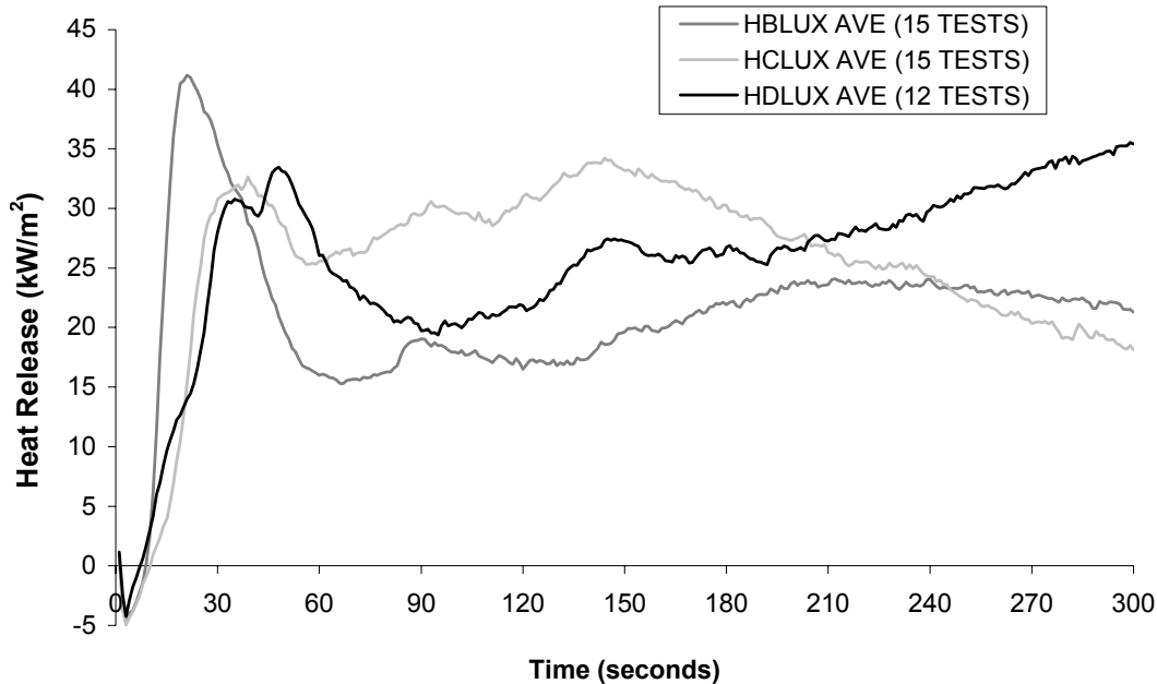
FIGURE 10. HEAT RELEASE AVERAGE (POINT-BY-POINT)—COMPARISON OF PANELS B, C, AND D FINISHED WITH LAMINATE U
