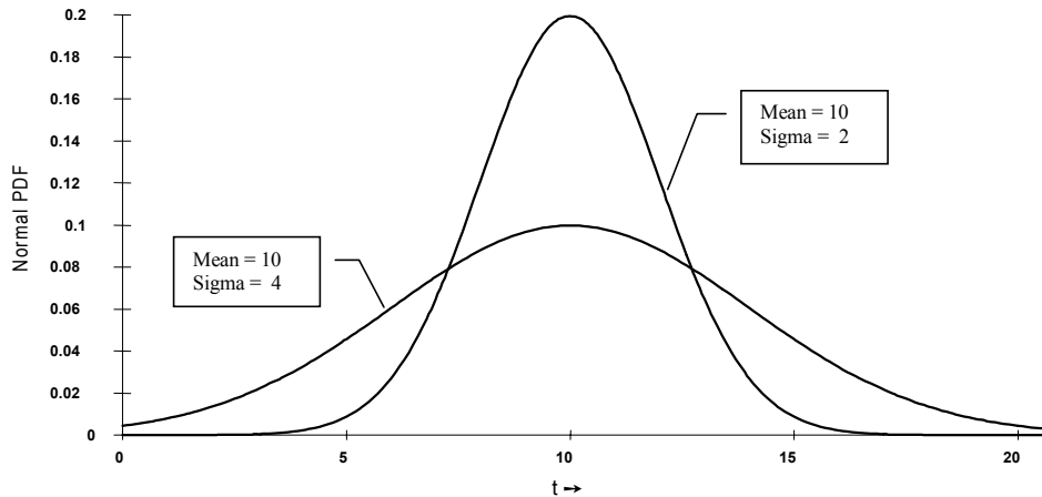
FIGURE 3-2. THE NORMAL DISTRIBUTION
