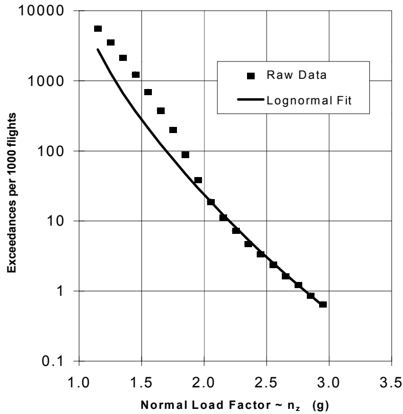
(a) Positive Maneuver n_z -Exceedance Data and Lognormal Fit
