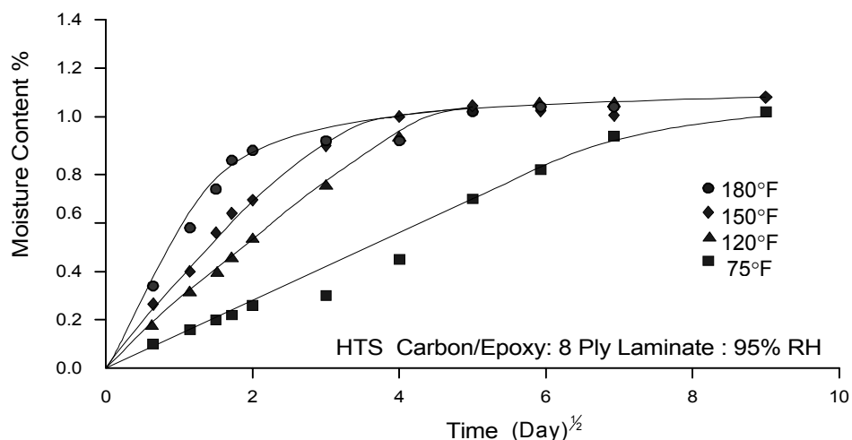
FIGURE 5-4. TYPICAL MOISTURE ABSORPTION RESPONSE [90]
