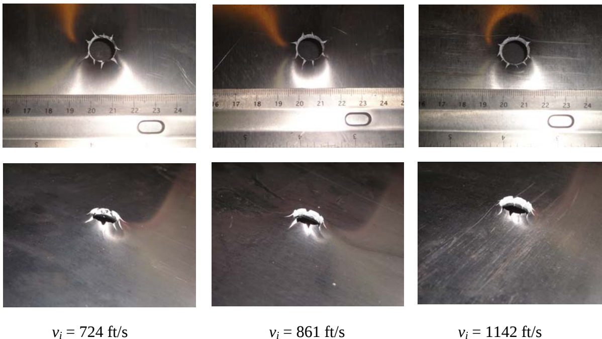
FIGURE 30. VIEWS OF PLATES SHOT AT DIFFERENT INITIAL VELOCITIES, SHOWING THE CONSISTENCY IN PETAL DEFORMATION WITH INCREASING PROJECTILE VELOCITY
