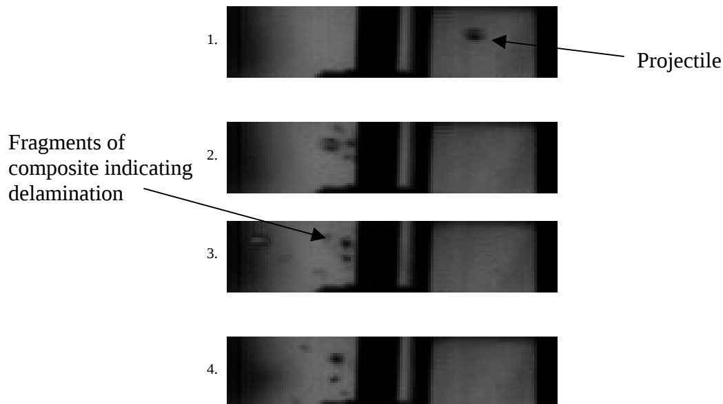
FIGURE 52. IMAGE SEQUENCE SHOWING DELAMINATION OF PETALS
