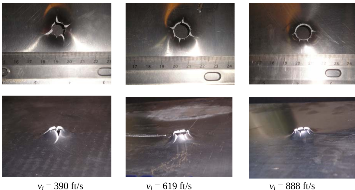
FIGURE 24. BACK AND ANGLED BACK VIEWS OF PLATES SHOT AT DIFFERENT INITIAL VELOCITIES, SHOWING THE INCREASE IN THE NUMBER OF PETALS AND DECREASE IN PETAL SIZE WITH INCREASING PROJECTILE VELOCITY
