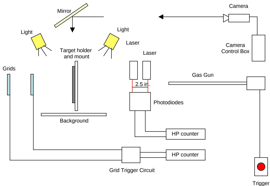
FIGURE 3. SCHEMATIC OF EXPERIMENTAL ARRANGEMENT USING THE GAS GUN
