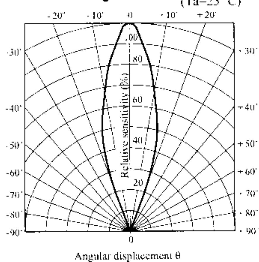
Fig. 6 Radiation Diagram
