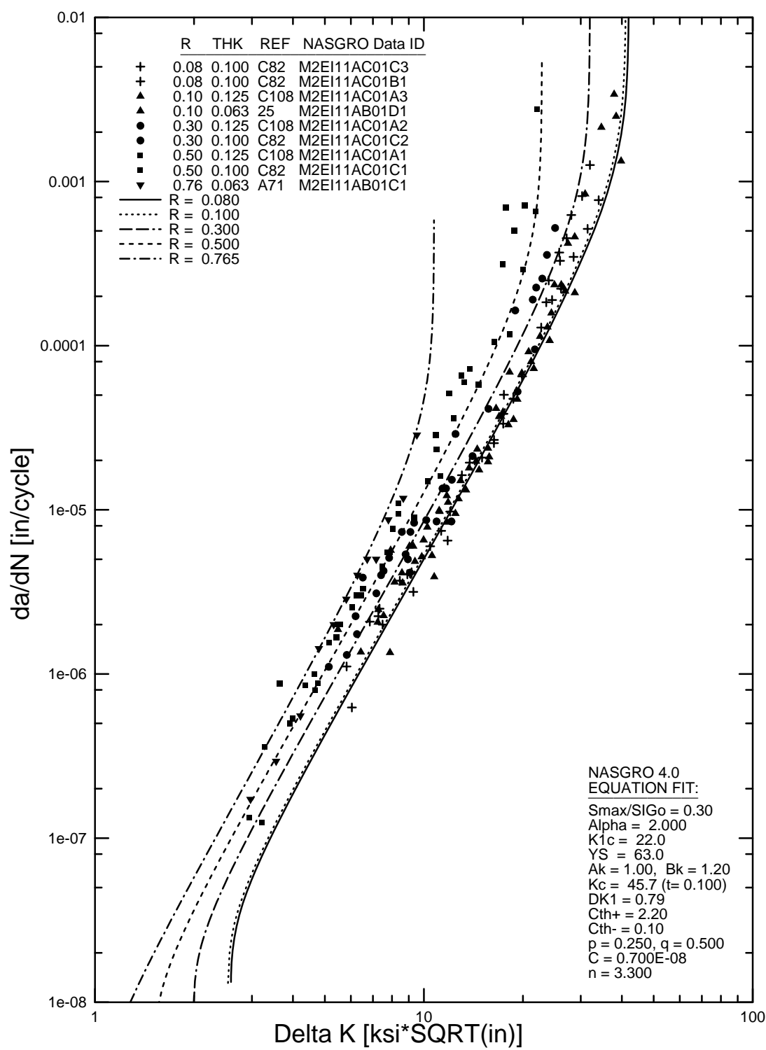
FIGURE B-19. NASGRO EQUATION FIT FOR 2024-T81 SHEET, L-T (M2EI11AB1)
