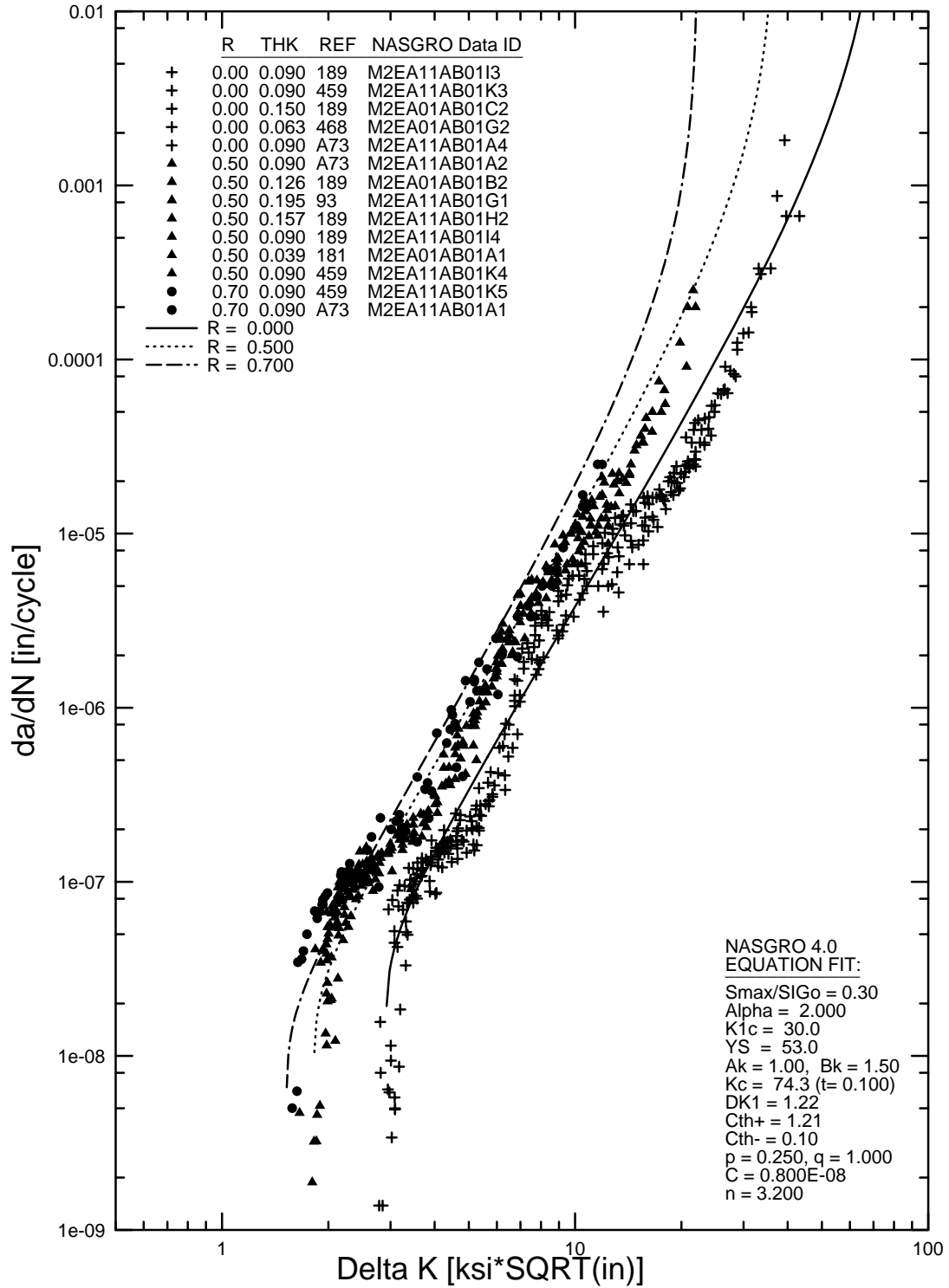
FIGURE B-4a. NASGRO EQUATION FIT FOR 2024-T3 CLAD AND BARE SHEET, L-T (M2EA11AB1) WITH POSITIVE R VALUES
