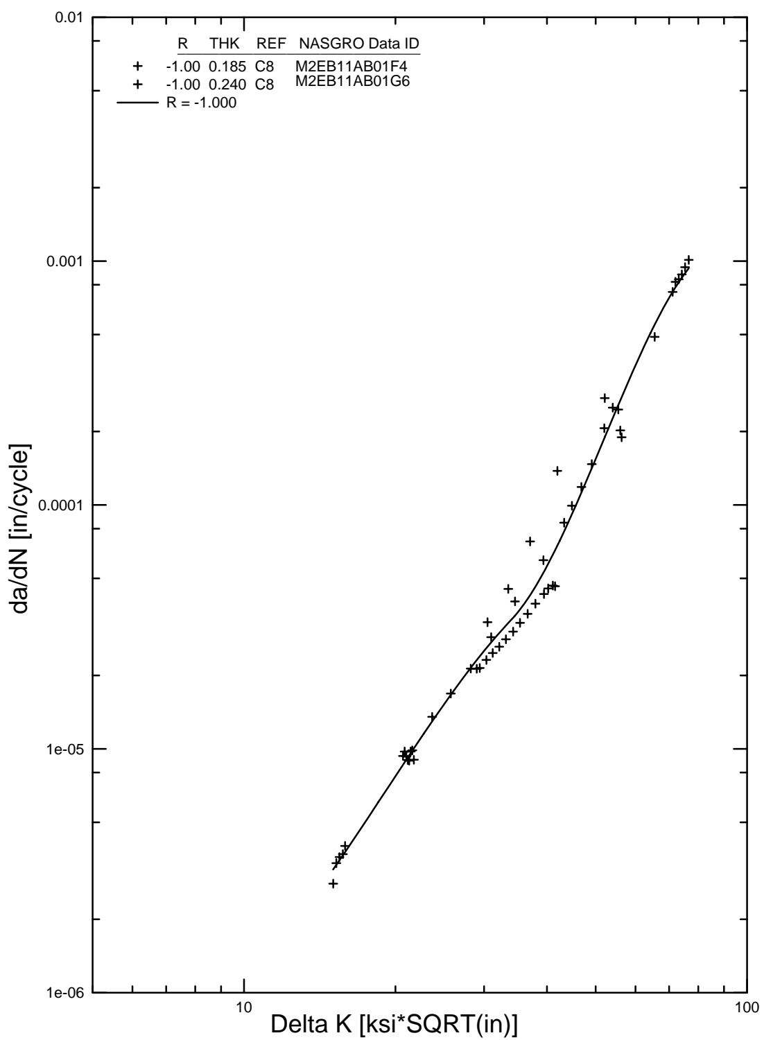
FIGURE B-12b. SPLINE FIT FOR 2024-T351 PLATE, L-T (M2EB11AB1) WITH NEGATIVE R VALUE
