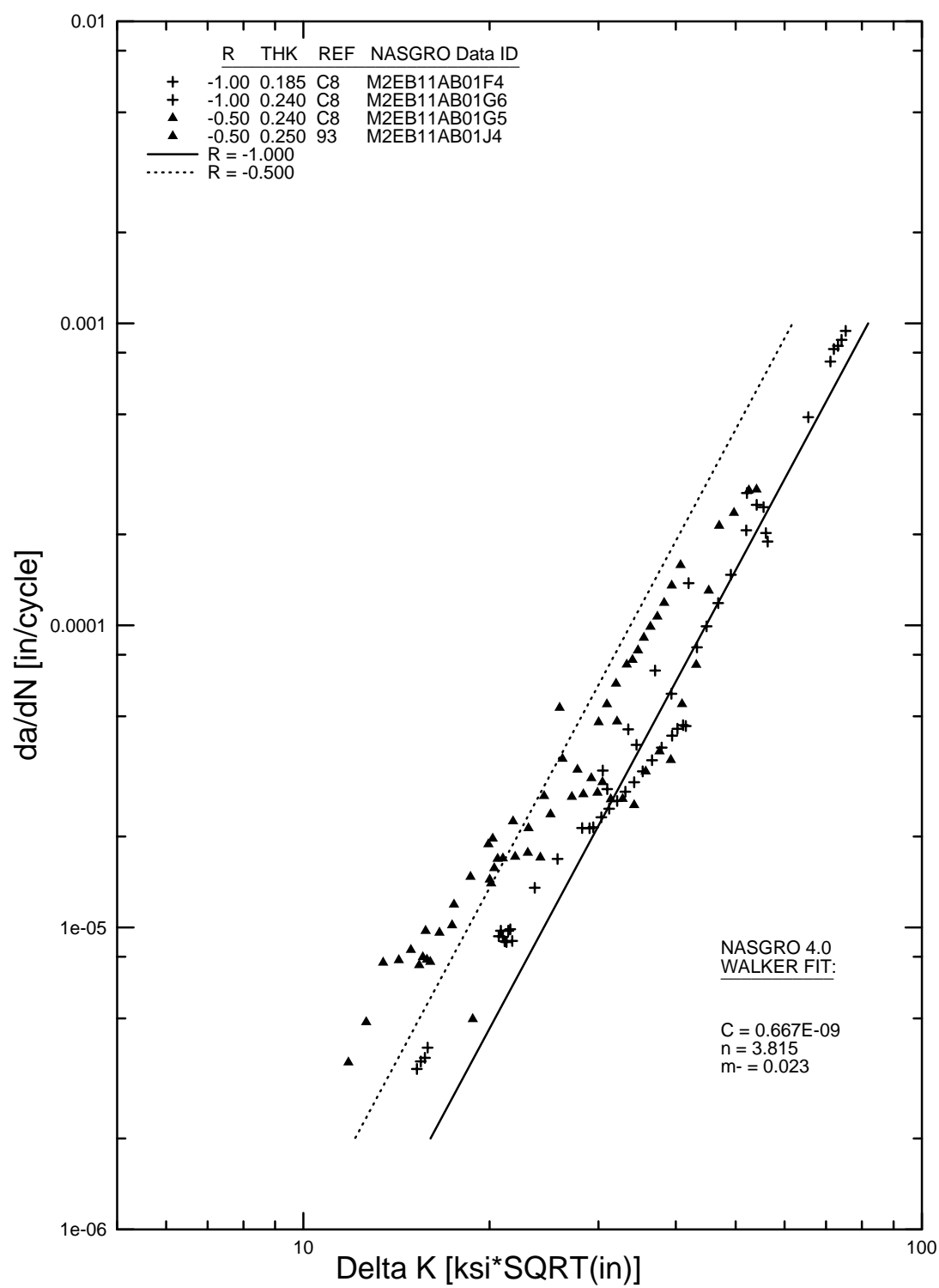
FIGURE B-11b. WALKER EQUATION FIT FOR 2024-T351 PLATE, L-T (M2EB11AB1) WITH NEGATIVE R VALUES
