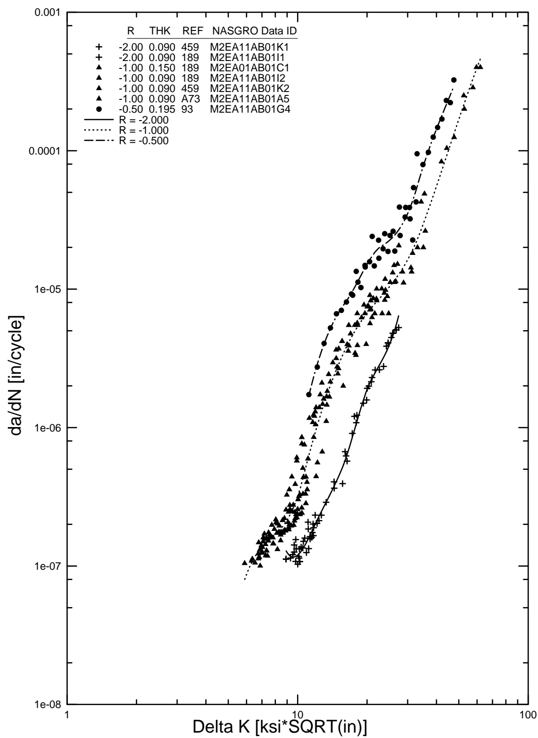
FIGURE B-6b. SPLINE FIT FOR 2024-T3 CLAD AND BARE SHEET, L-T (M2EA11AB1) WITH NEGATIVE R VALUES
