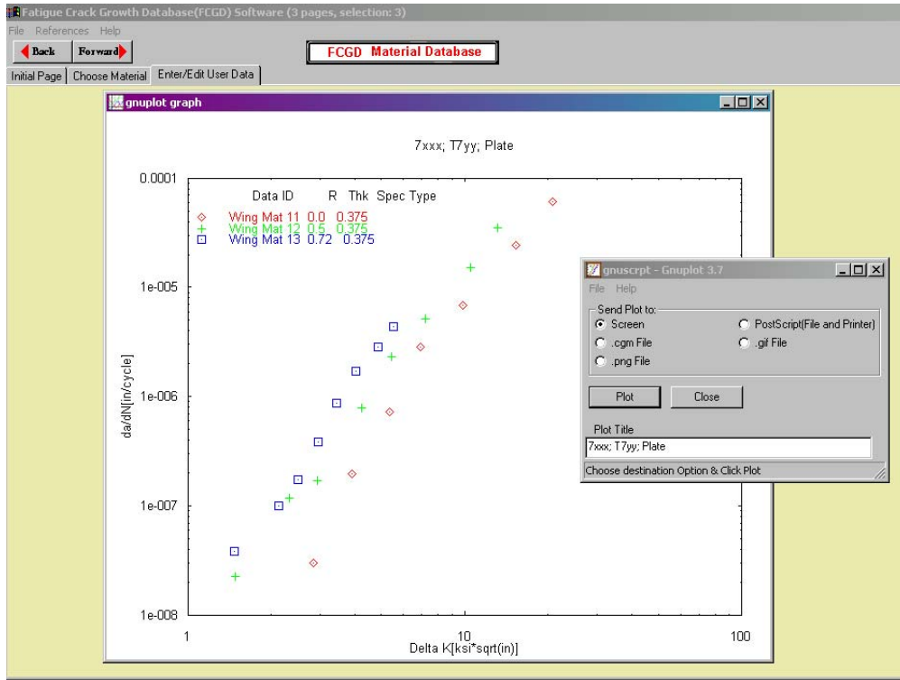
FIGURE D-2. DISPLAY OF USER-ENTERED DATA
