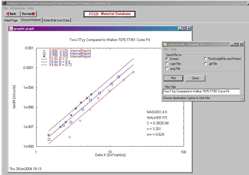
FIGURE D-5. COMPARISON OF USER-ENTERED DATA WITH 7075-T7351 WALKER CURVE FIT AT R = 0, 0.5, AND 0.72
