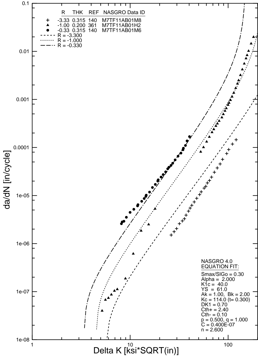
FIGURE B-31b. NASGRO EQUATION FIT FOR 7475-T7351 PLATE, L-T (M7TF11AB1) WITH NEGATIVE R VALUES
