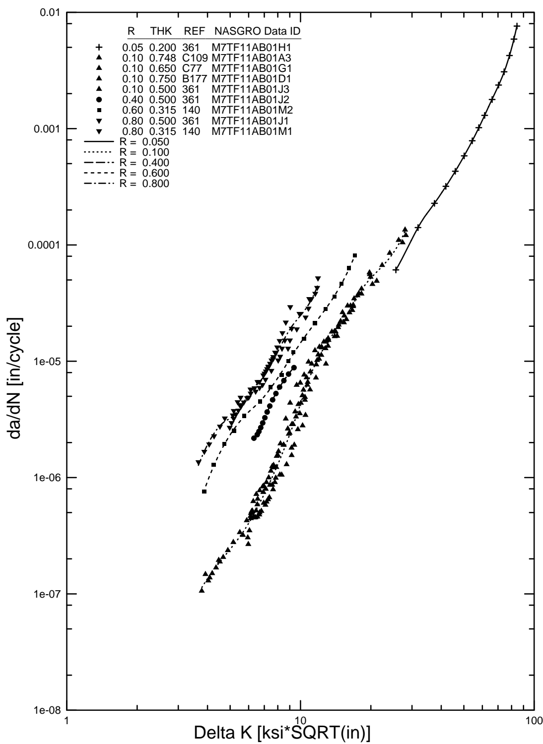
FIGURE B-33a. SPLINE FIT FOR 7475-T7351 PLATE, L-T (M7TF11AB1) WITH POSITIVE R VALUES
