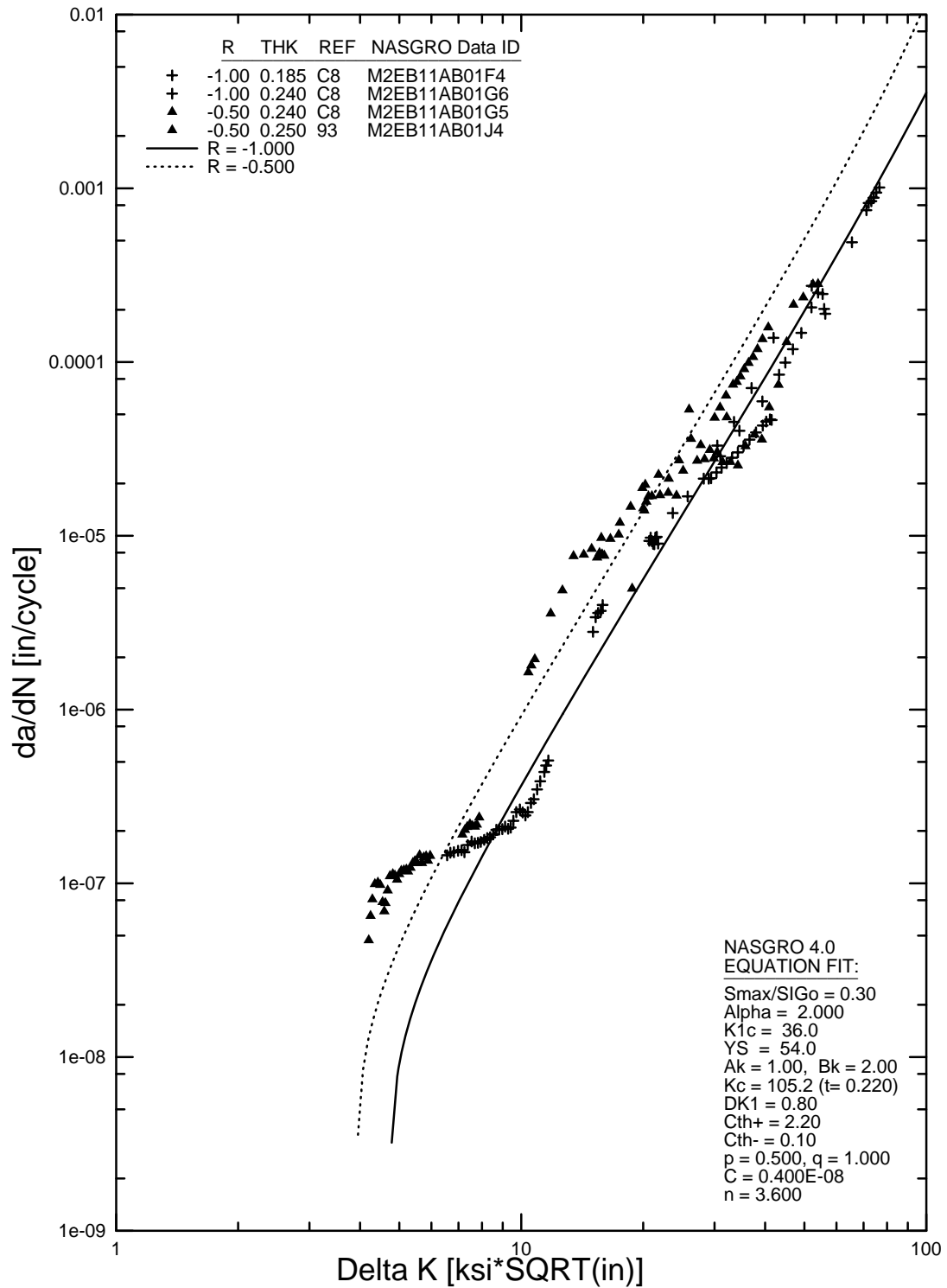
FIGURE B-10b. NASGRO EQUATION FIT FOR 2024-T351 CLAD AND BARE SHEET, L-T (M2EB11AB1) WITH NEGATIVE R VALUES
