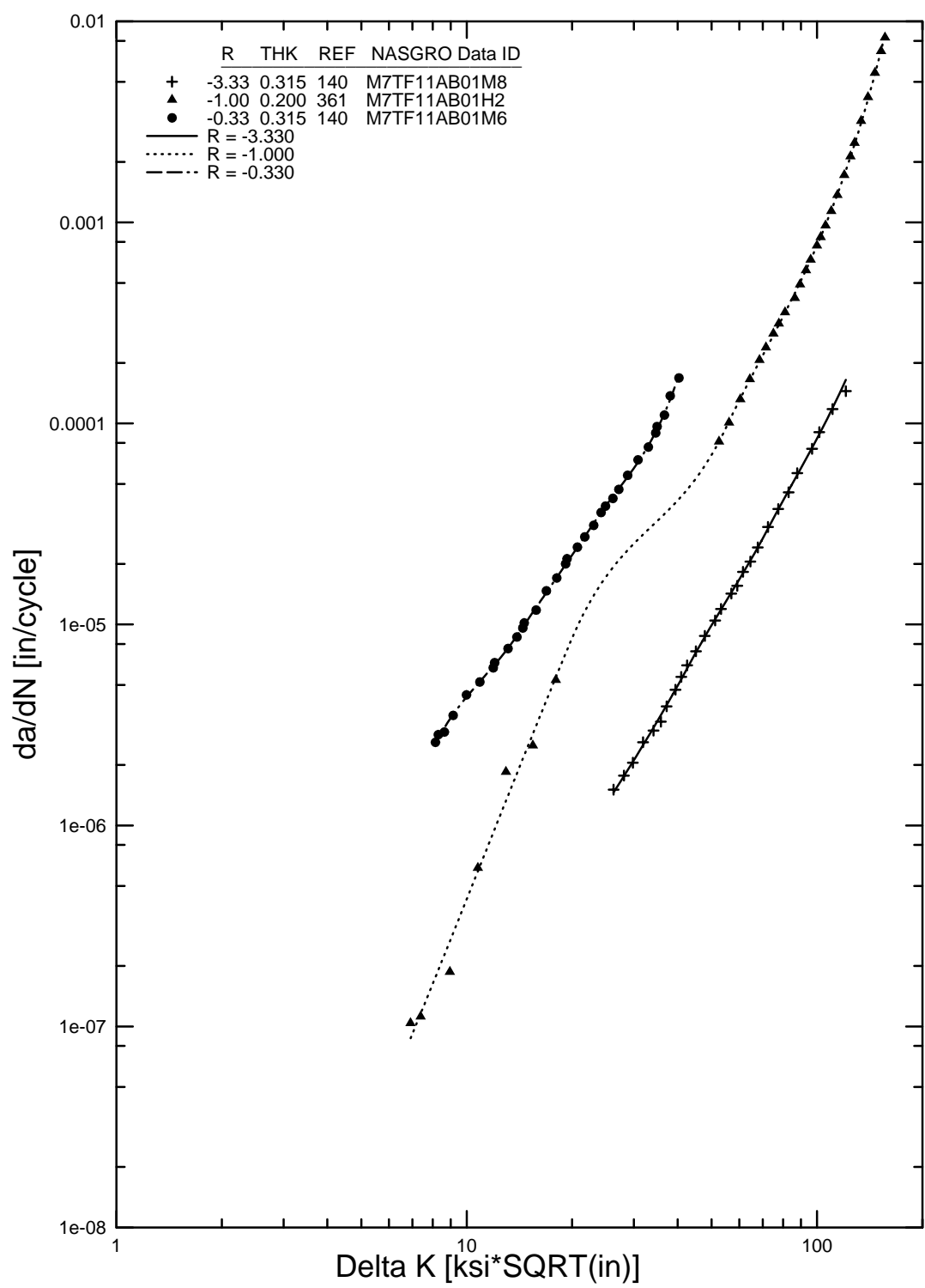
FIGURE B-33b. SPLINE FIT FOR 7475-T7351 PLATE, L-T (M7TF11AB1) WITH NEGATIVE R VALUES
