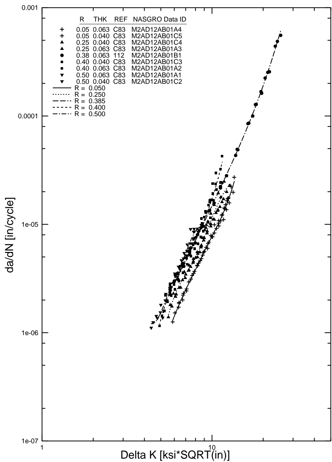
FIGURE B-3. SPLINE FIT FOR 2014-T6 SHEET, T-L (M2AD12AB1)
