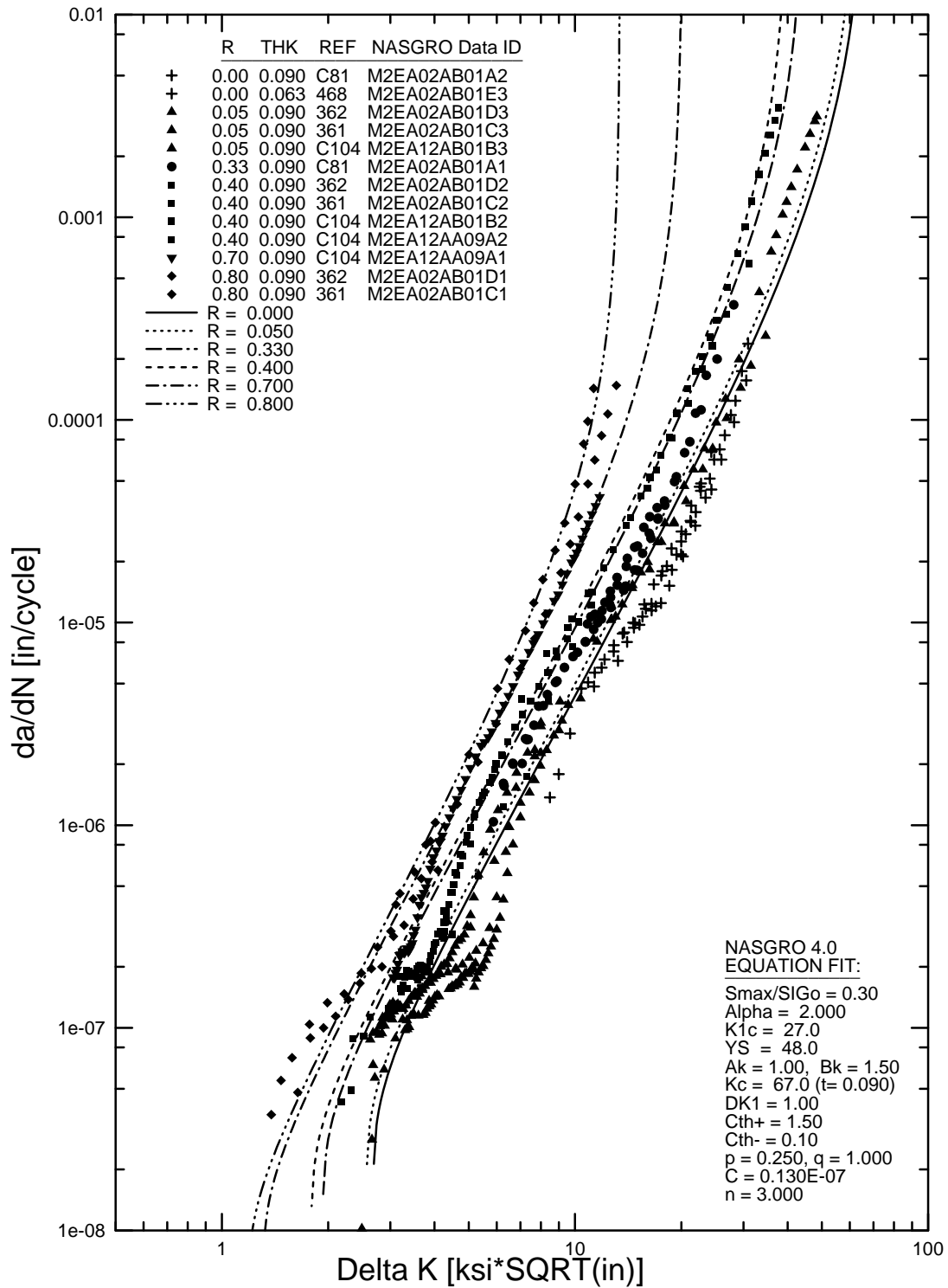
FIGURE B-7. NASGRO EQUATION FIT FOR 2024-T3 CLAD AND BARE SHEET, T-L (M2EA02AB1)
