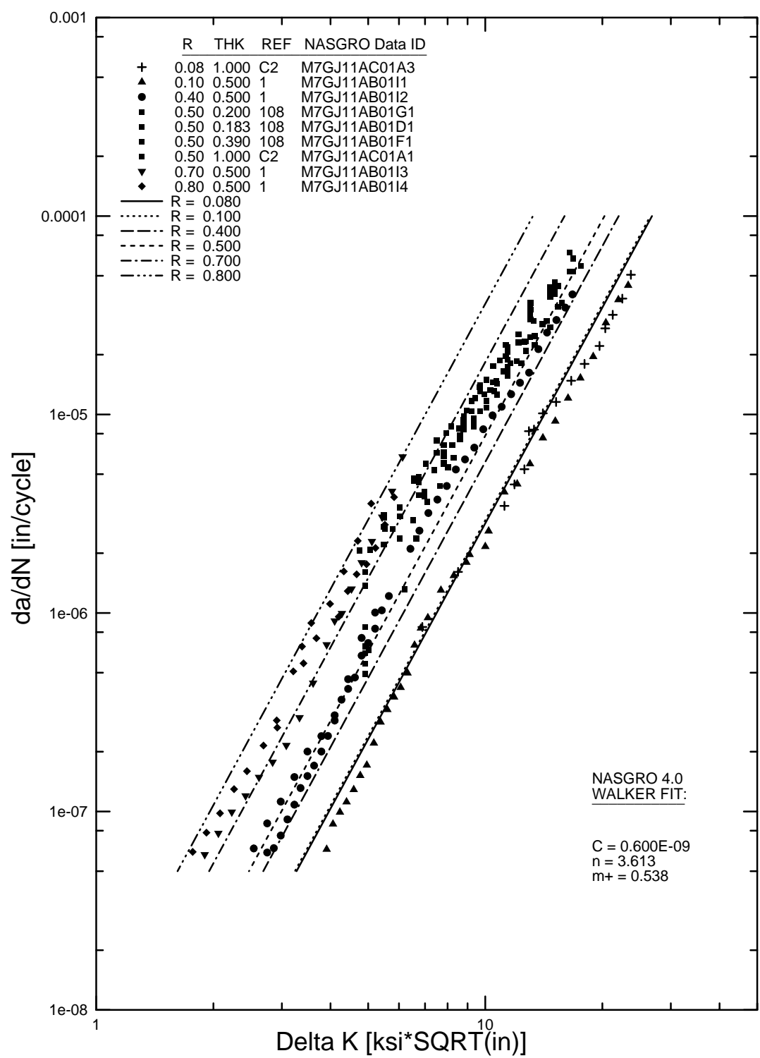
FIGURE B-23. WALKER EQUATION FIT FOR 7050-T7451 PLATE, L-T (M7GJ11AB1)
