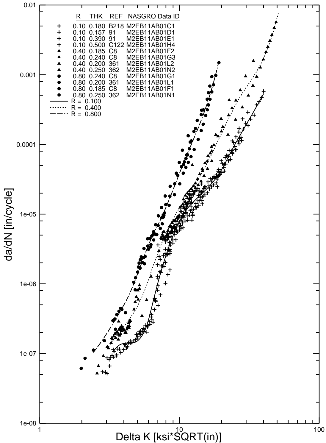
FIGURE B-12a. SPLINE FIT FOR 2024-T351 PLATE, L-T (M2EB11AB1) WITH POSITIVE R VALUES
