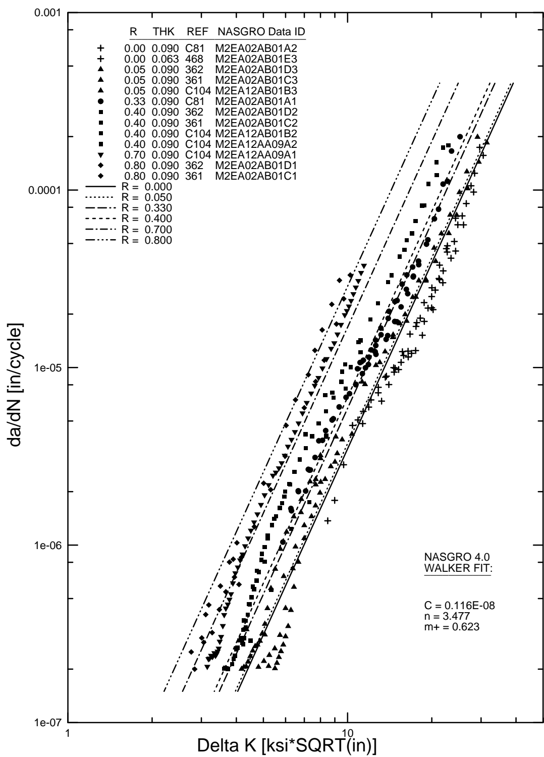
FIGURE B-8. WALKER EQUATION FIT FOR 2024-T3 CLAD AND BARE SHEET, T-L (M2EA02AB1)
