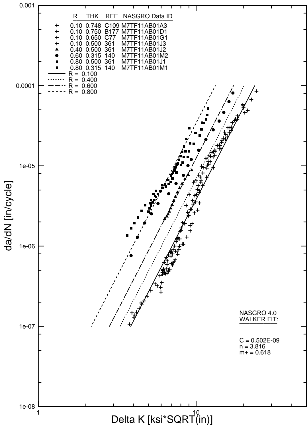
FIGURE B-32a. WALKER EQUATION FIT FOR 7475-T7351 PLATE, L-T (M7TF11AB1) WITH POSITIVE R VALUES
