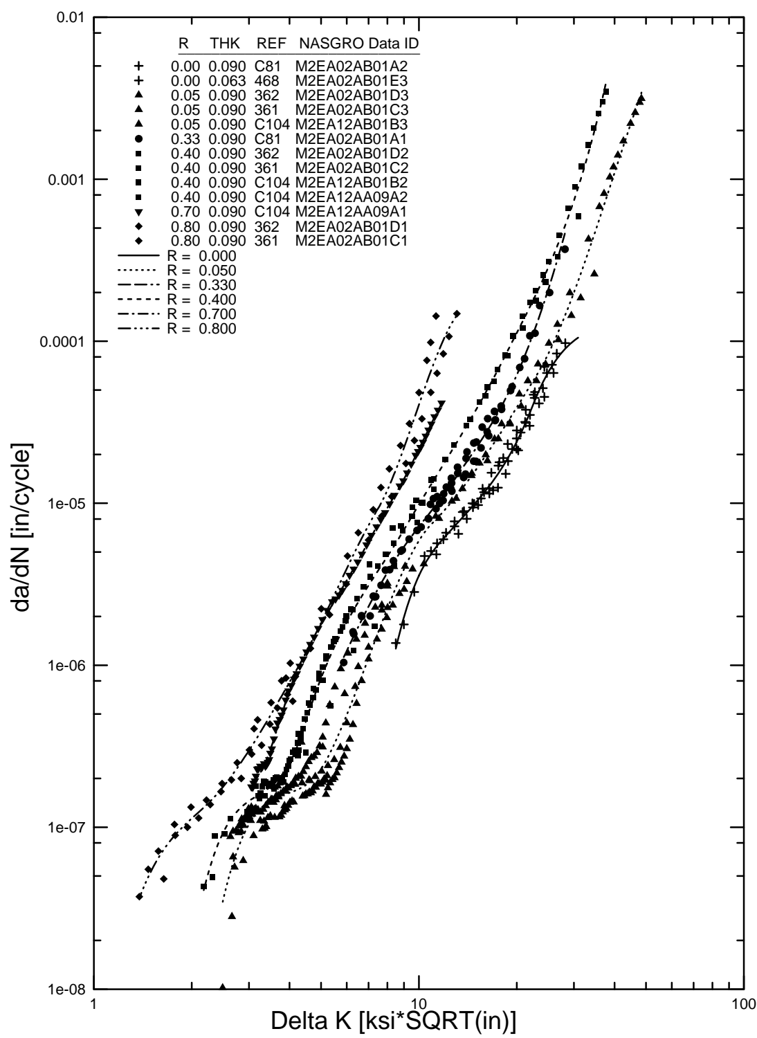
FIGURE B-9. SPLINE FIT FOR 2024-T3 CLAD AND BARE SHEET, T-L (M2EA02AB1)
