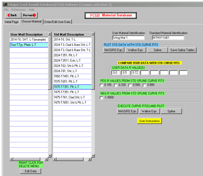
FIGURE D-3. SELECTION OF USER MATERIAL AND FCGD MATERIAL FOR COMPARISON PLOTTING
