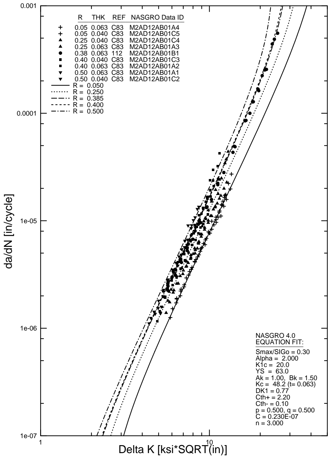
FIGURE B-1. NASGRO EQUATION FOR FIT 2014-T6 SHEET, T-L (M2AD12AB1)
