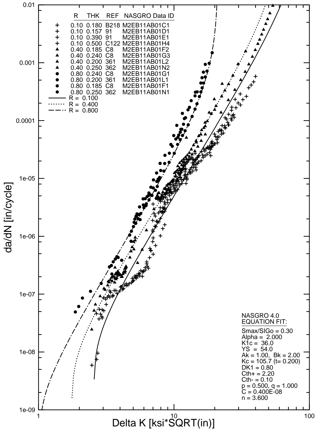
FIGURE B-10a. NASGRO EQUATION FIT FOR 2024-T351 PLATE, L-T (M2EB11AB1) WITH POSITIVE R VALUES
