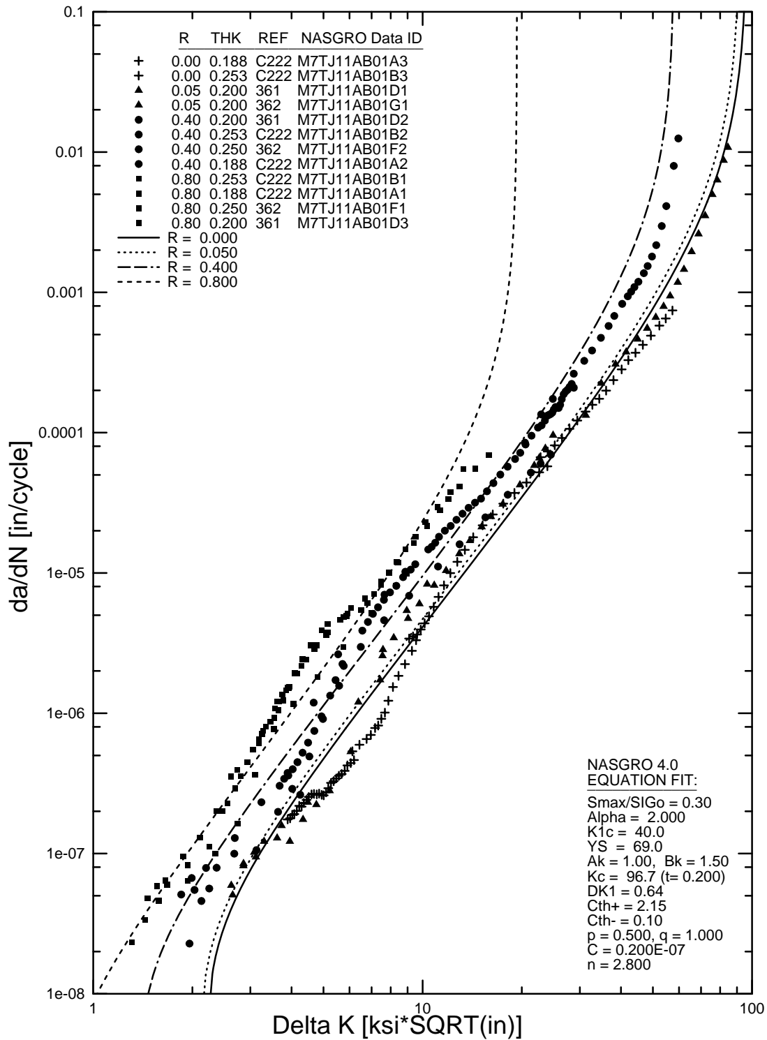
FIGURE B-37. NASGRO EQUATION FIT FOR 7475-T7651 SHEET AND PLATE, L-T (M7TJ11AB1)
