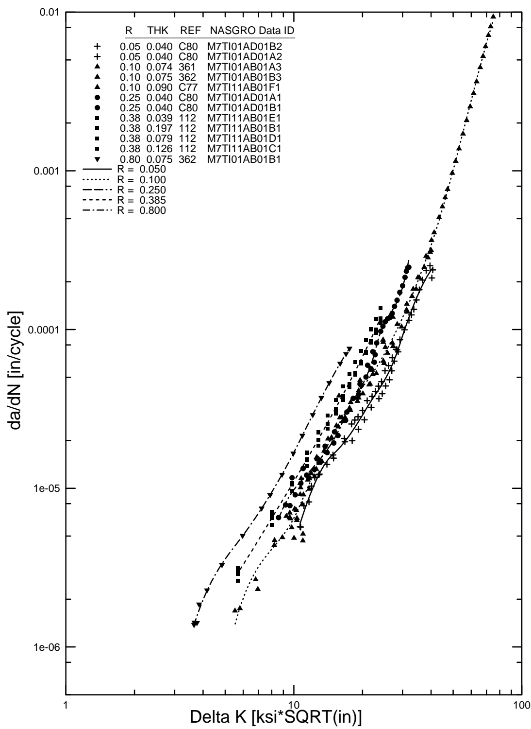
FIGURE B-36. SPLINE FIT FOR 7475-T761 CLAD SHEET, L-T (M7TI01AB1)
