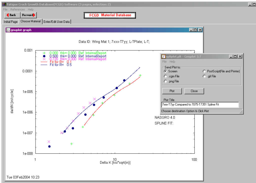
FIGURE D-6. COMPARISON OF USER-ENTERED DATA WITH 7075-T7351 SPLINE CURVE FIT AT R = 0.1 and 0.5
