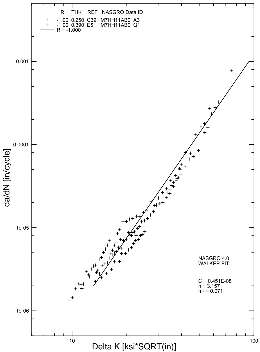
FIGURE B-29b. WALKER EQUATION FIT FOR 7075-T7351 PLATE, L-T (M7HH11AB1) WITH NEGATIVE R VALUE
