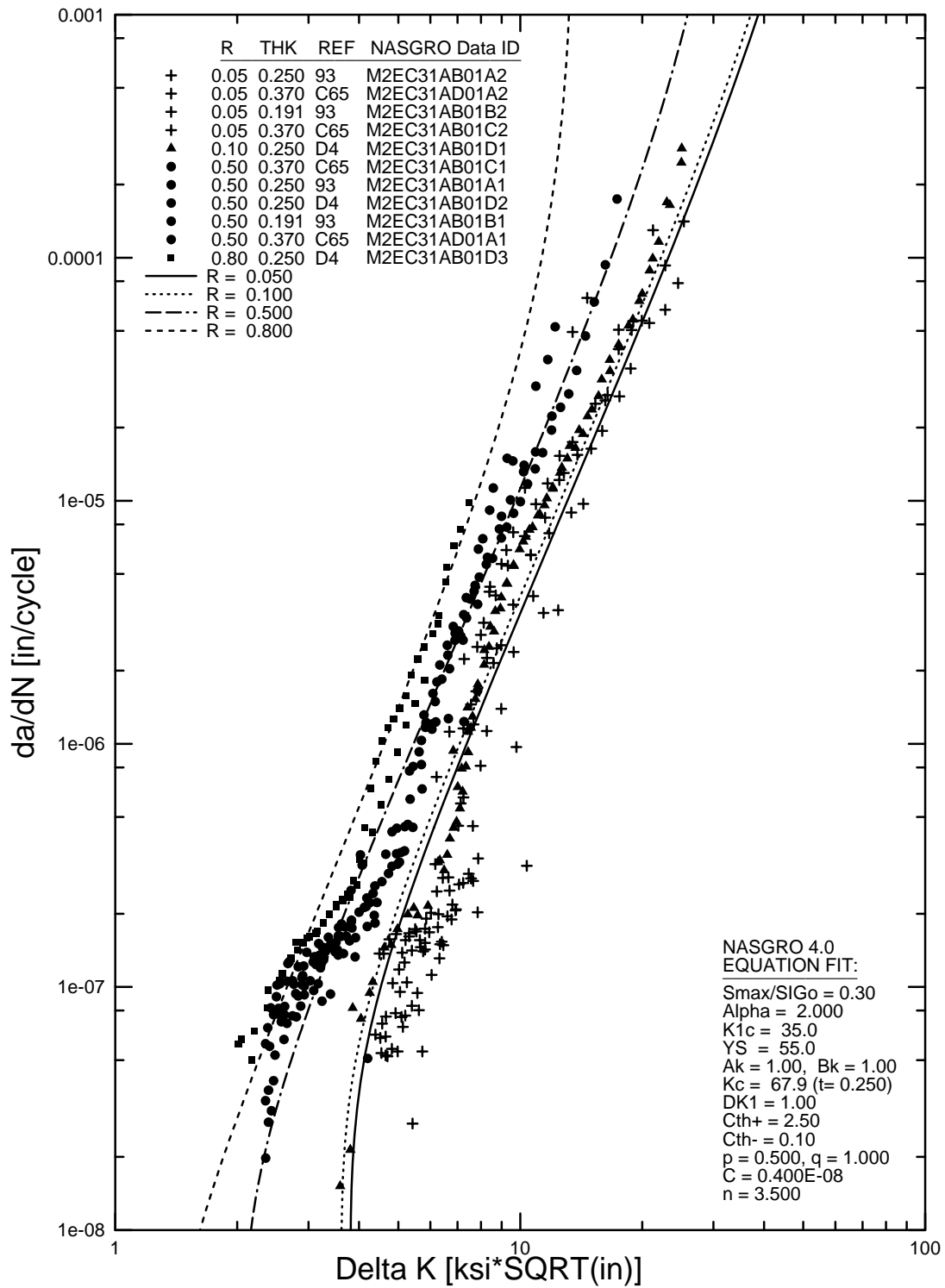
FIGURE B-13. NASGRO EQUATION FIT FOR 2024-T3511 EXTRUSION, L-T (M2EC31AB1)
