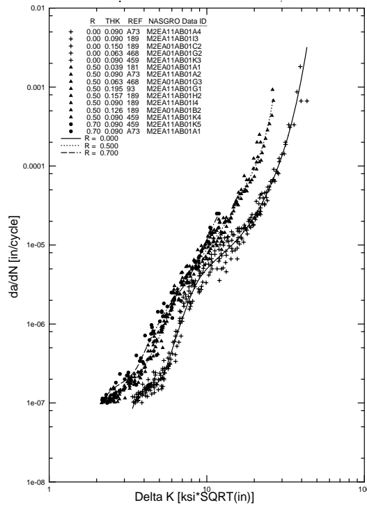
FIGURE 4. SPLINE CURVE FITS FOR 2024-T3 CLAD AND BARE SHEET, L-T (M2EA11AB1)
