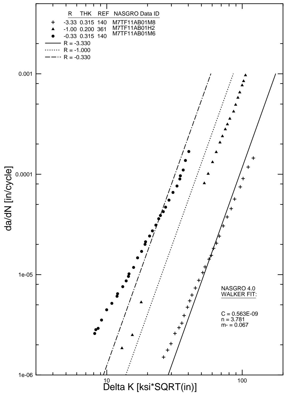
FIGURE B-32b. WALKER EQUATION FIT FOR 7475-T7351 PLATE, L-T (M7TF11AB1) WITH NEGATIVE R VALUES
