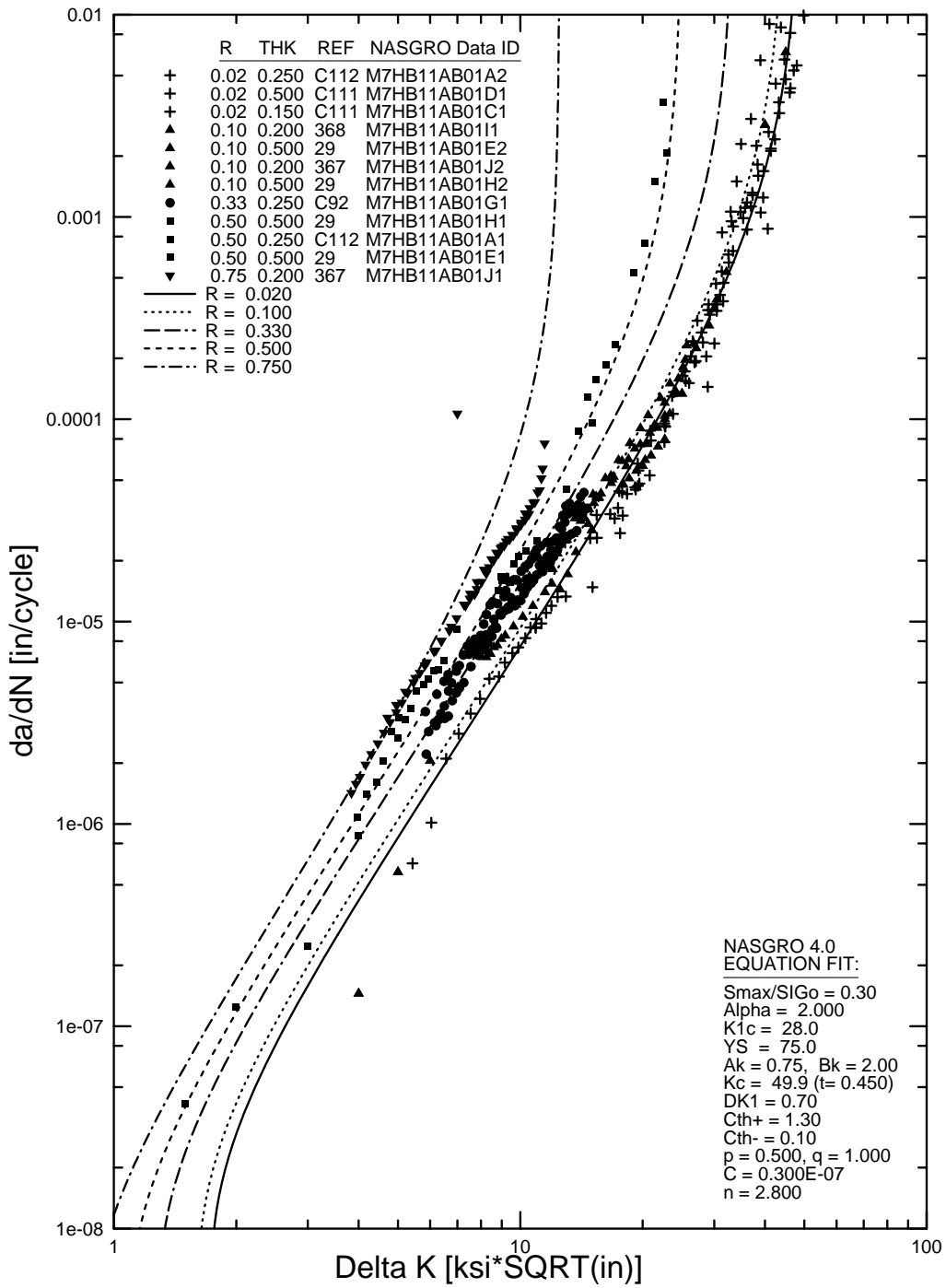
FIGURE B-25. NASGRO EQUATION FIT FOR 7075-T651 PLATE, L-T (M7HB11AB1)
