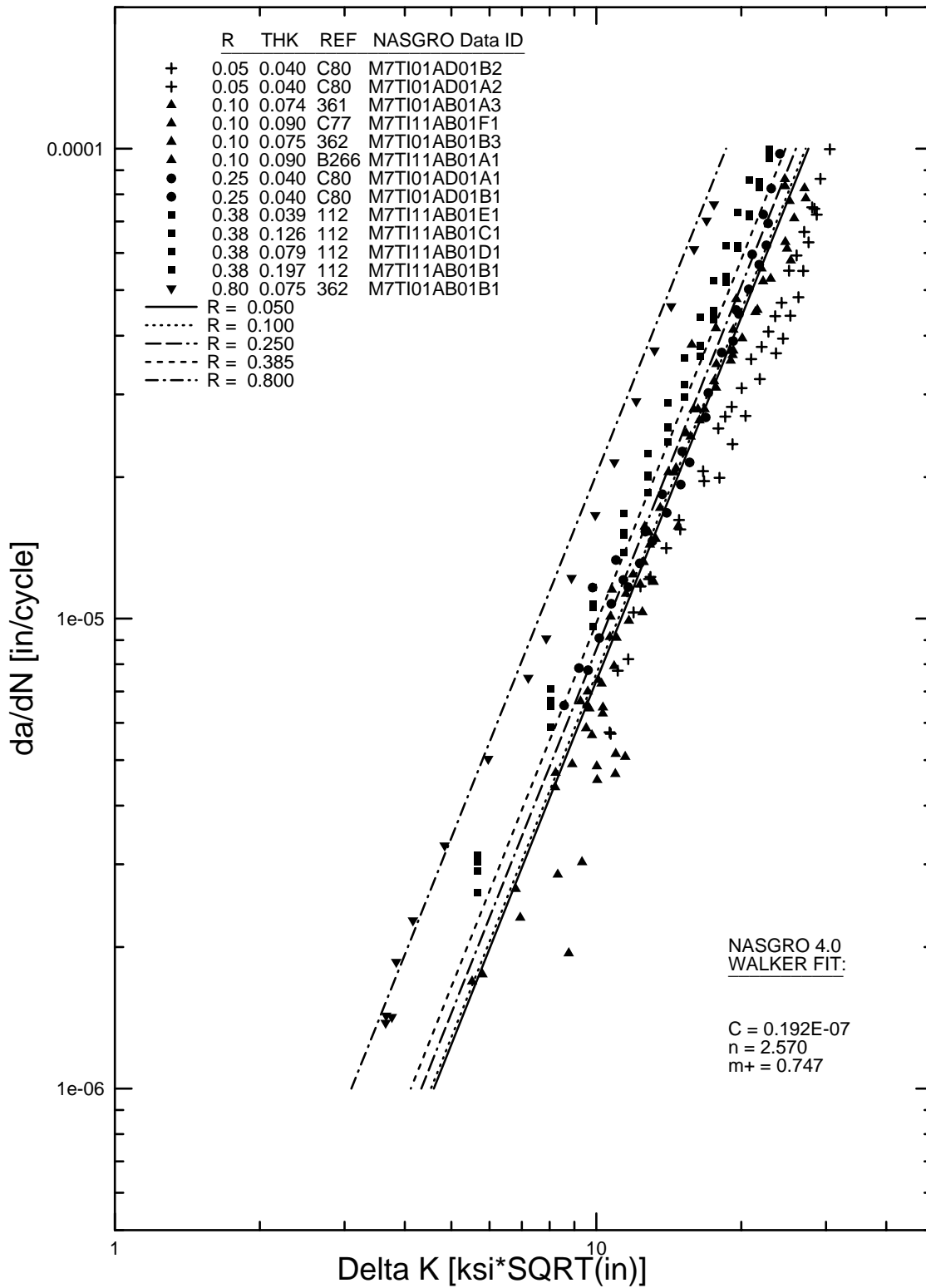
FIGURE B-35. WALKER EQUATION FIT FOR 7475-T761 CLAD SHEET, L-T (M7TI01AB1)
