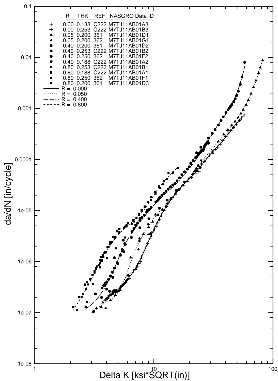
FIGURE B-39. SPLINE FIT FOR 7475-T7651 SHEET AND PLATE, L-T (M7TJ11AB1)
