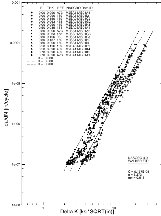
FIGURE 3. WALKER EQUATION FIT FOR 2024-T3 CLAD AND BARE SHEET, L-T (M2EA11AB1)
