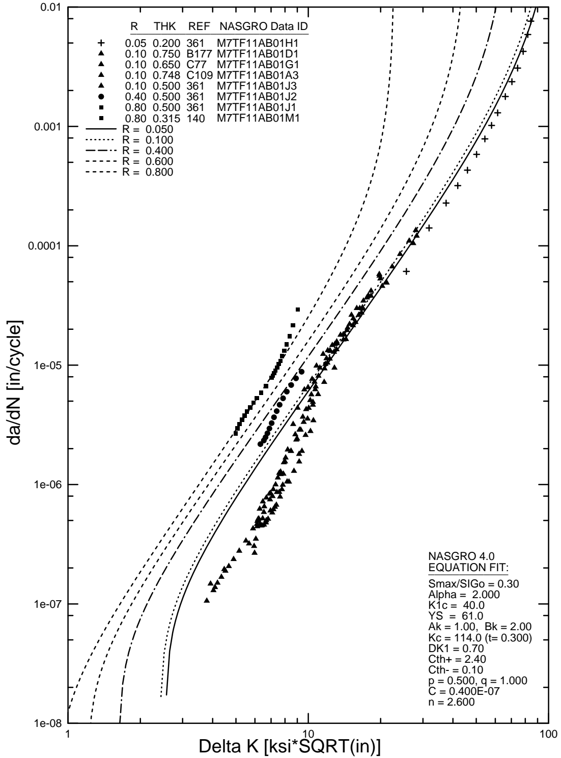
FIGURE B-31a. NASGRO EQUATION FIT FOR 7475-T7351 PLATE, L-T (M7TF11AB1) WITH POSITIVE R VALUES
