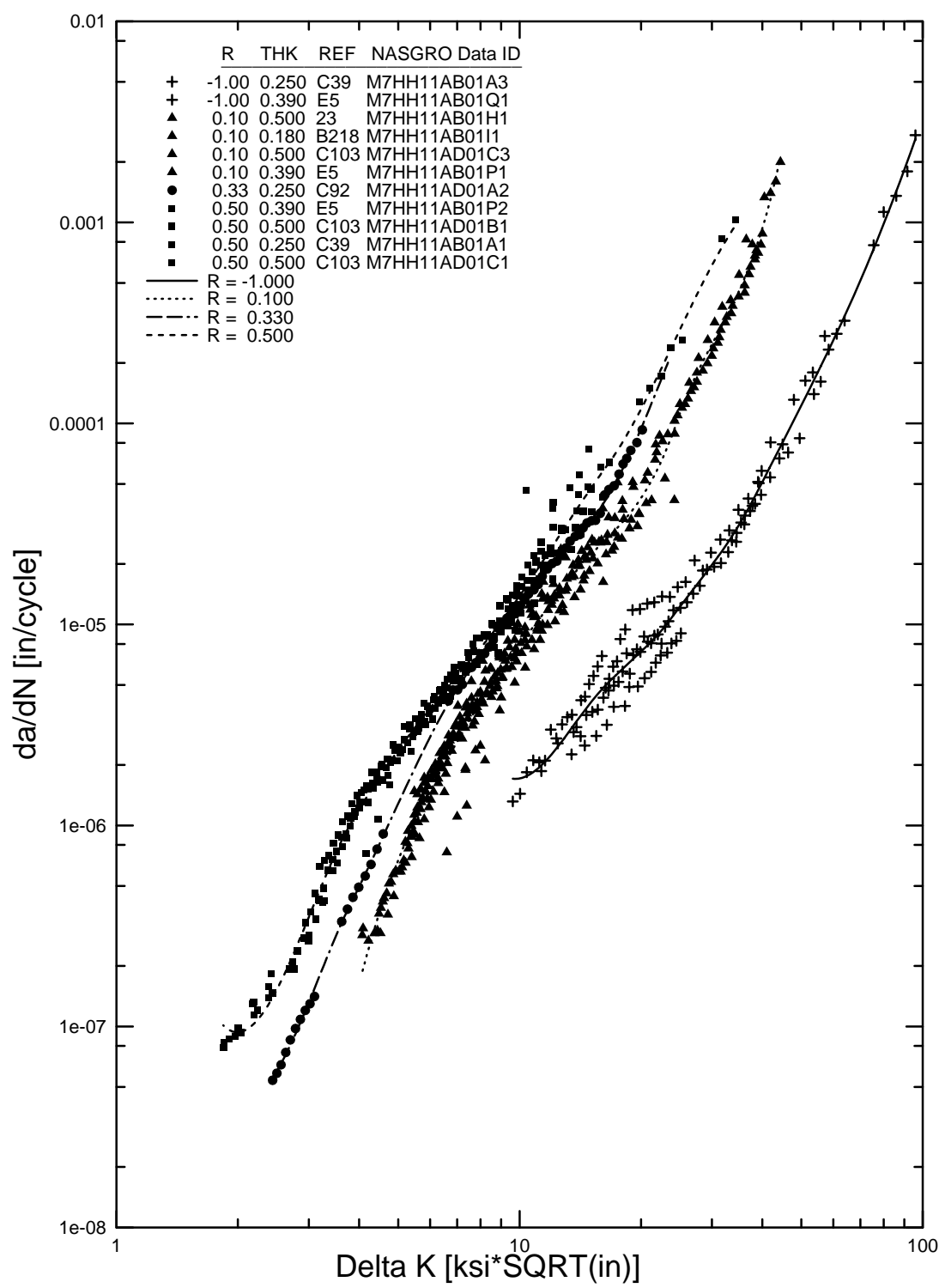
FIGURE B-30. SPLINE FIT FOR 7075-T7351 PLATE, L-T (M7HH11AB1) WITH POSITIVE AND NEGATIVE R VALUES
