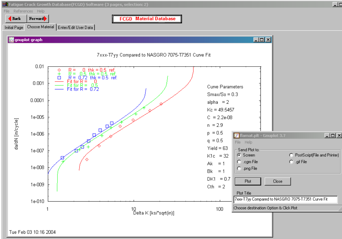
FIGURE D-4. COMPARISON OF USER-ENTERED DATA WITH 7075-T7351 NASGRO CURVE FIT AT R = 0, 0.5, AND 0.72
