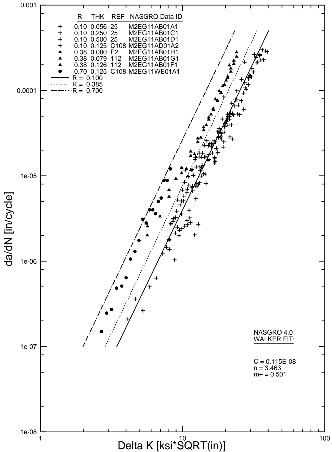
FIGURE B-17. WALKER EQUATION FIT FOR 2024-T62 SHEET AND PLATE, L-T (M2EG11AB1)
