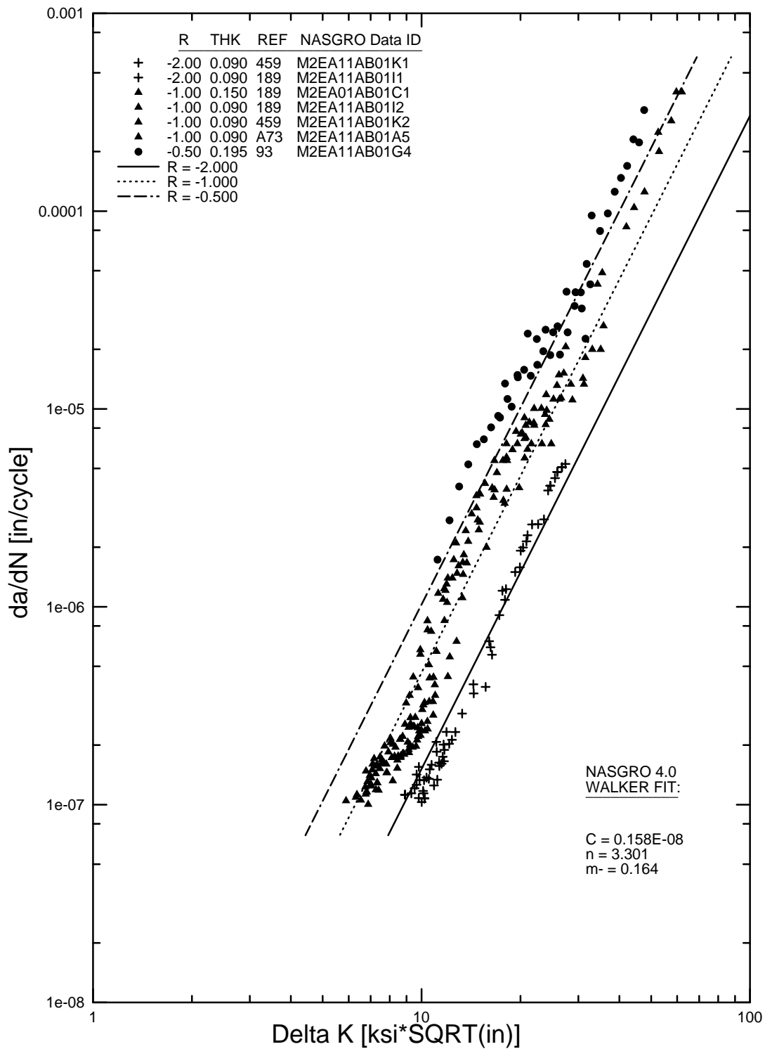
FIGURE B-5b. WALKER EQUATION FIT FOR 2024-T3 CLAD AND BARE SHEET, L-T (M2EA11AB1) WITH NEGATIVE R VALUES
