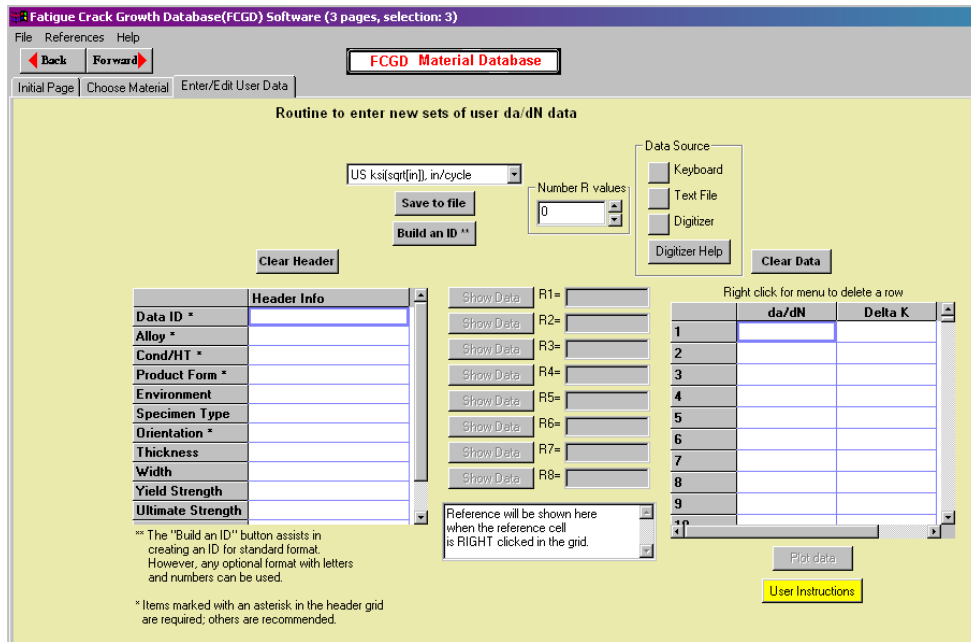
FIGURE C-3. INPUT WINDOW FOR USER-DEFINED FATIGUE CRACK GROWTH DATA
