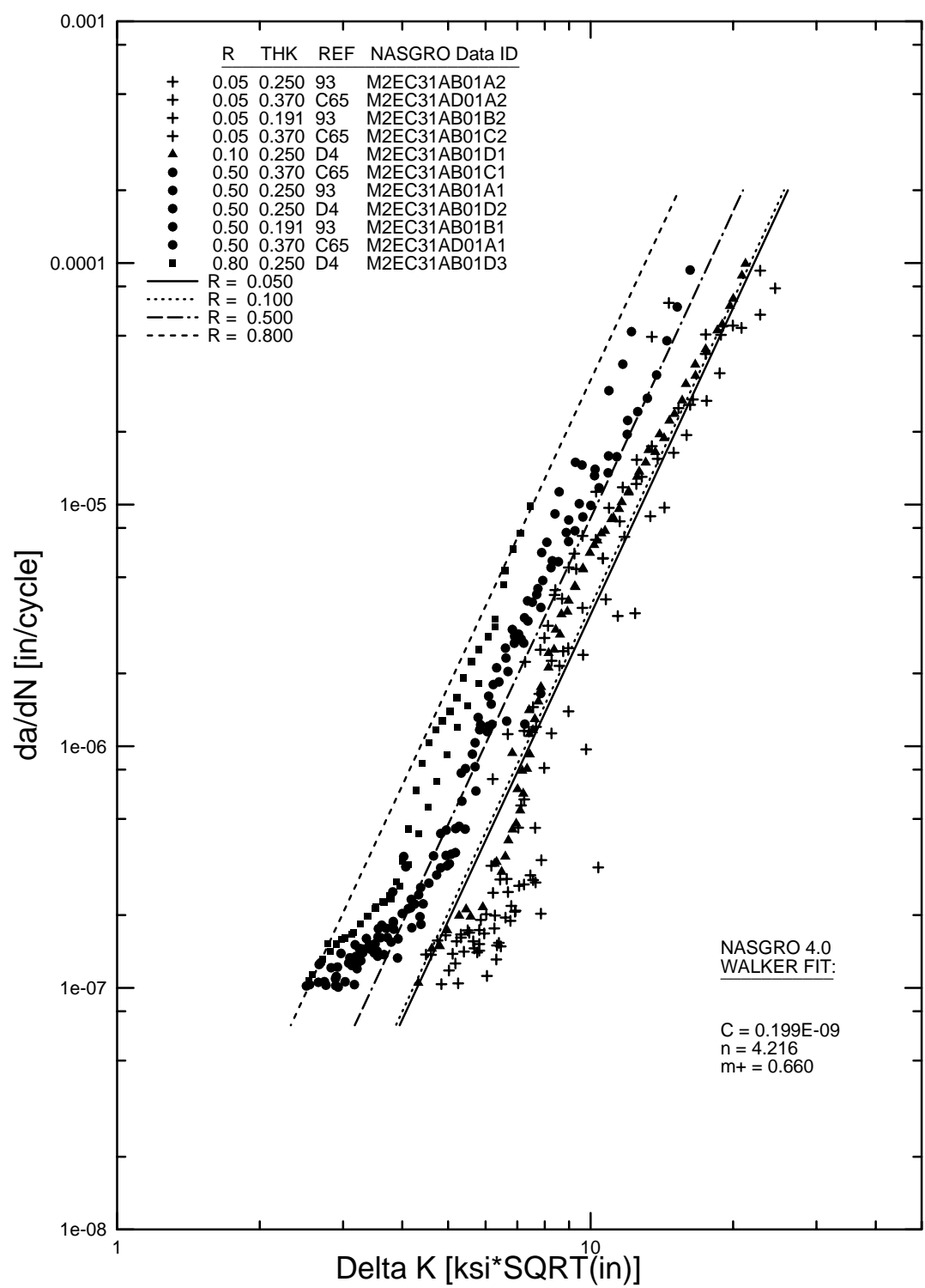
FIGURE B-14. WALKER EQUATION FIT FOR 2024-T3511 EXTRUSION, L-T (M2EC31AB1)
