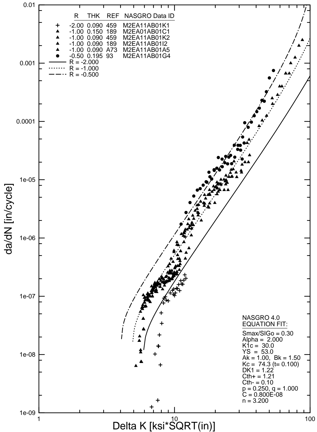
FIGURE B-4b. NASGRO EQUATION FIT FOR 2024-T3 CLAD AND BARE SHEET, L-T (M2EA11AB1) WITH NEGATIVE R VALUES
