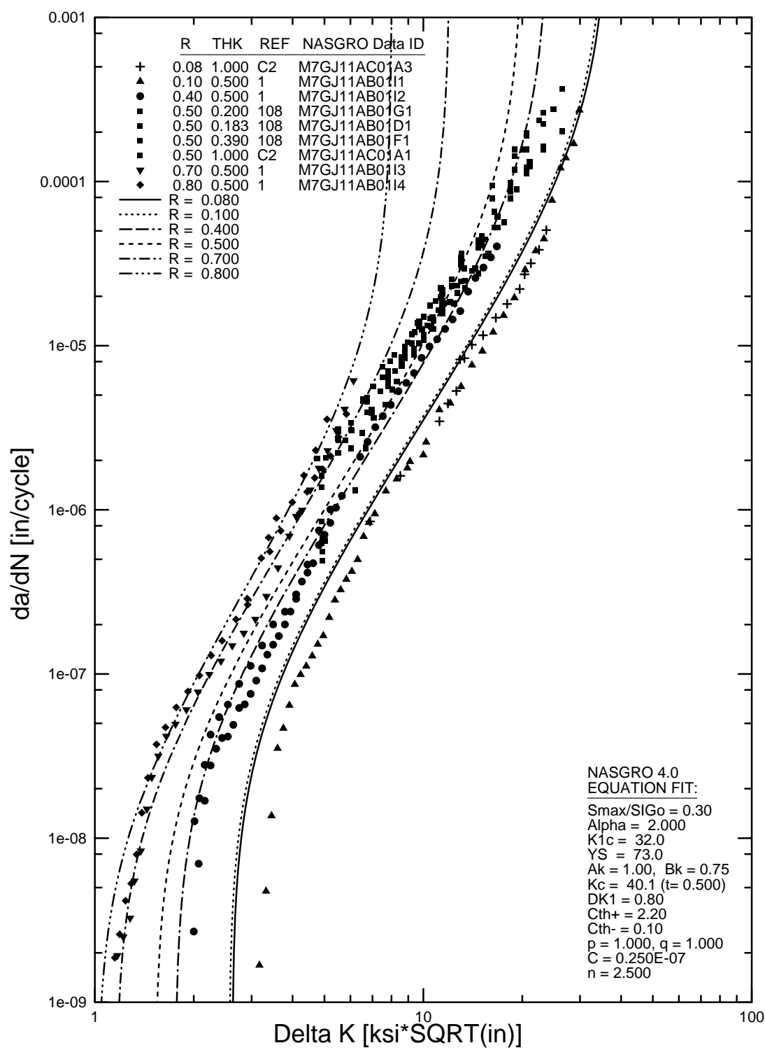
FIGURE B-22. NASGRO EQUATION FIT FOR 7050-T7451, L-T (M7GJ11AC1)
