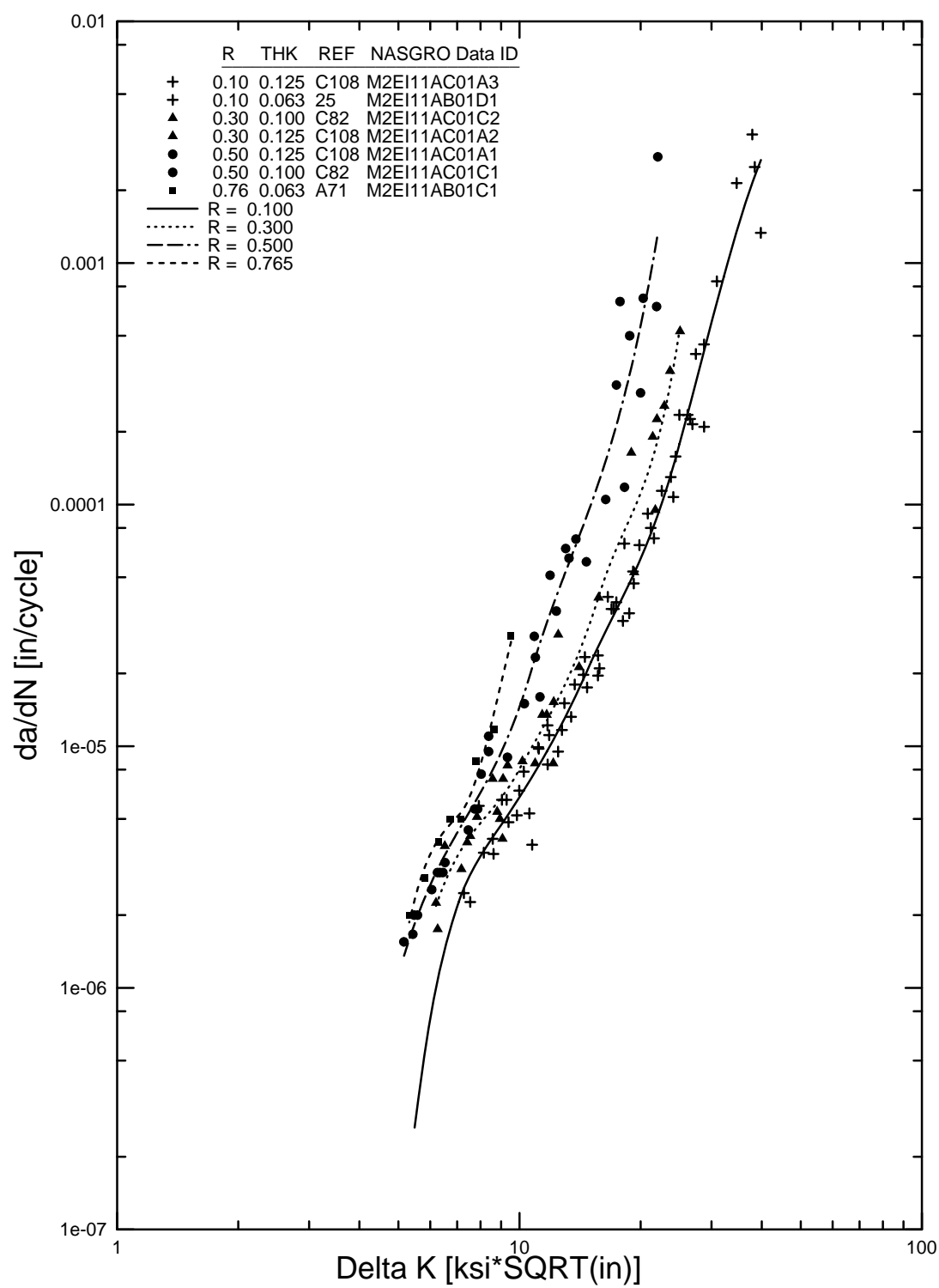
FIGURE B-21. SPLINE FIT FOR 2024-T81 SHEET, L-T (M2E111AB1)
