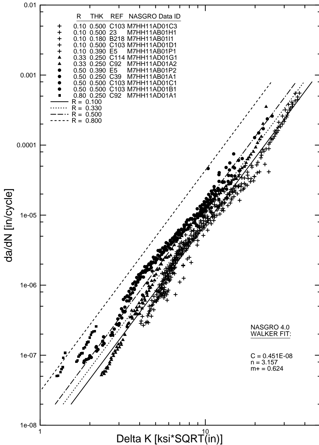
FIGURE B-29a. WALKER EQUATION FIT FOR 7075-T7351 PLATE, L-T (M7HH11AB1) WITH POSITIVE R VALUES
