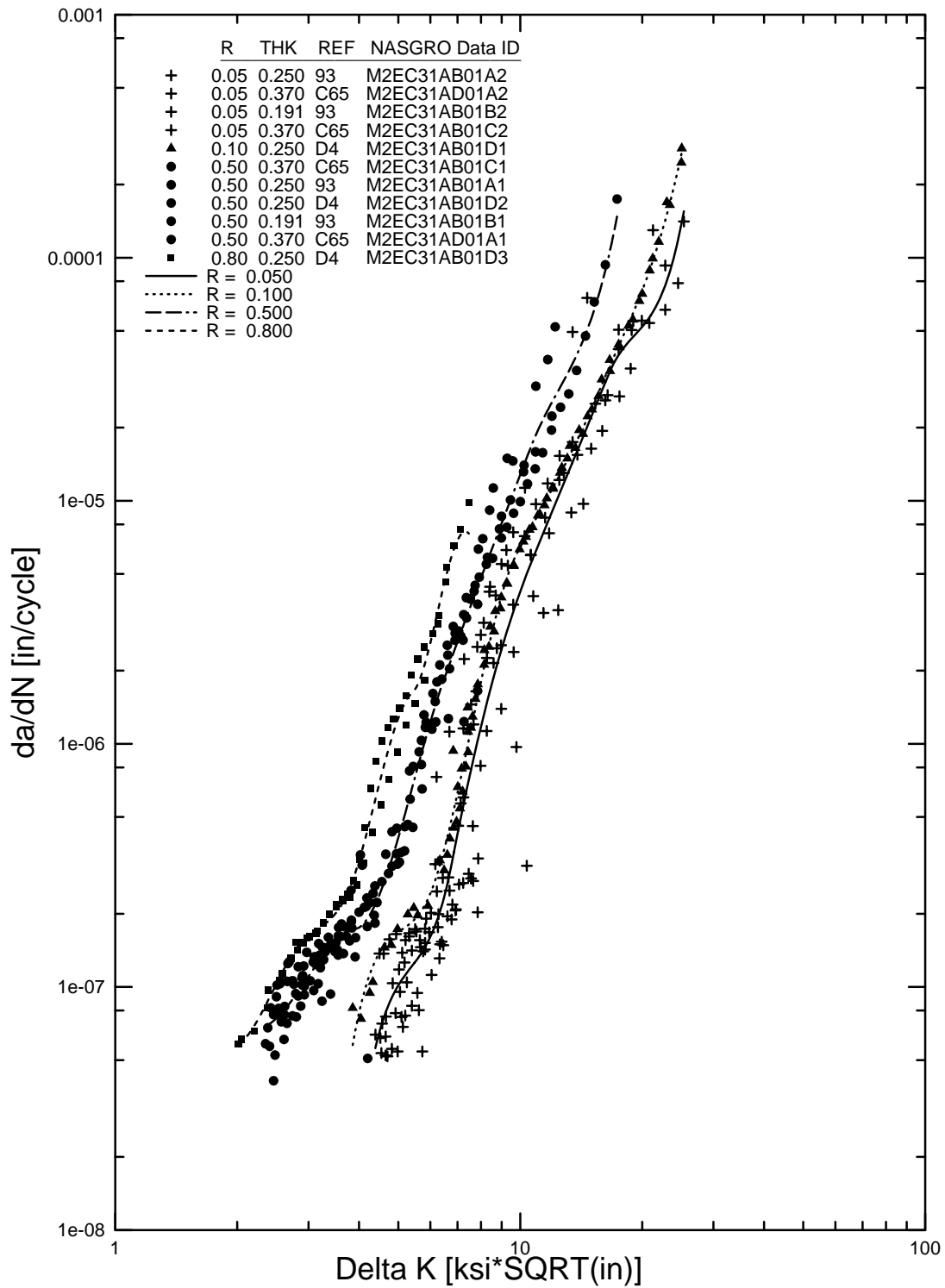
FIGURE B-15. SPLINE FIT FOR 2024-T3511 EXTRUSION, L-T (M2EC31AB1)
