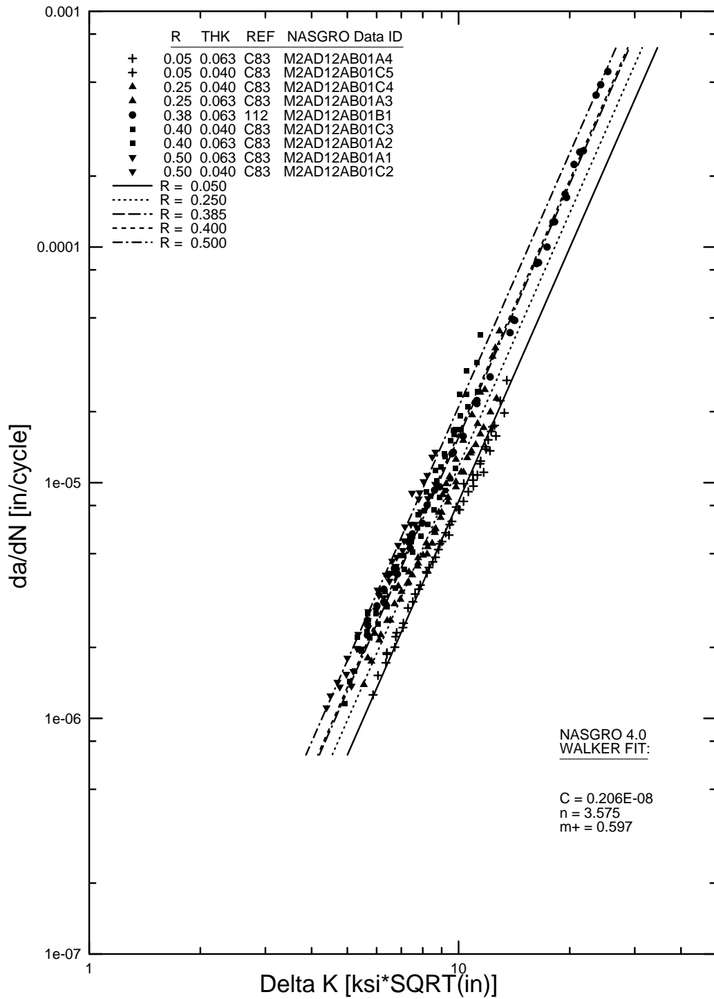
FIGURE B-2. WALKER EQUATION FIT FOR 2014-T6 SHEET, T-L (M2AD12AB1)
