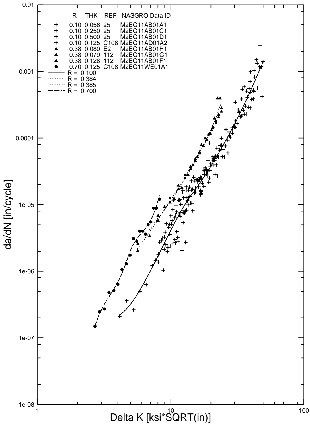
FIGURE B-18. SPLINE FIT FOR 2024-T62 SHEET AND PLATE, L-T (M2EG11AB1)
