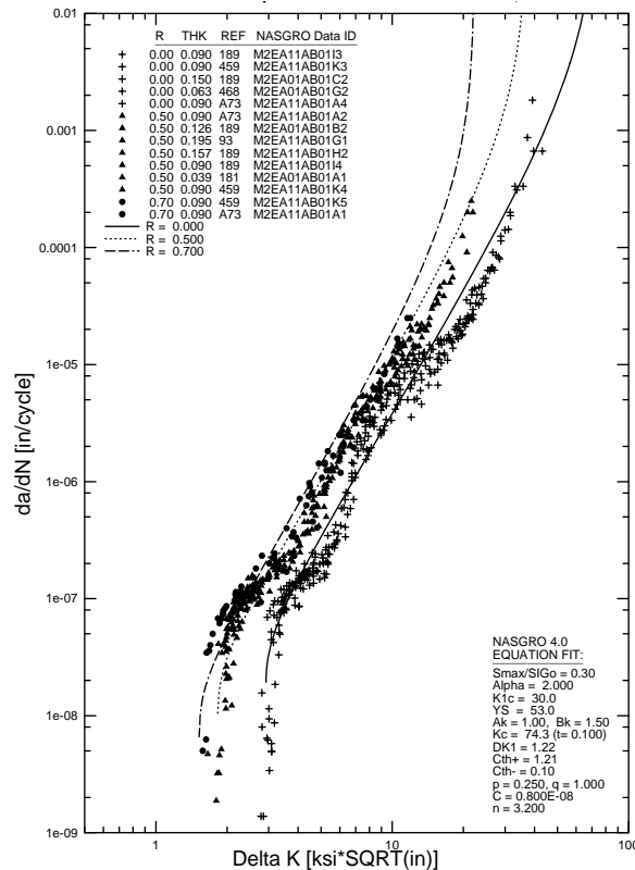
FIGURE 2. NASGRO EQUATION FIT FOR 2024-T3 CLAD AND BARE SHEET, L-T (M2EA11AB1)
