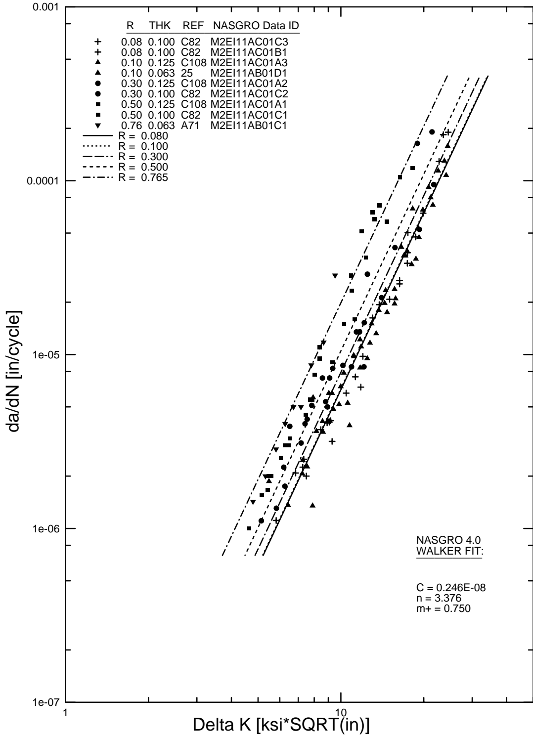
FIGURE B-20. WALKER EQUATION FIT FOR 2024-T81 SHEET, L-T (M2E111AB1)
