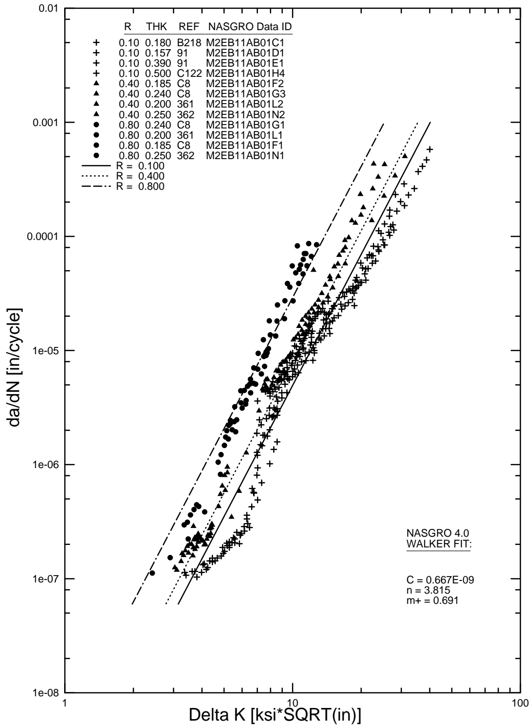
FIGURE B-11a. WALKER EQUATION FIT FOR 2024-T351 PLATE, L-T (M2EB11AB1) WITH POSITIVE R VALUES
