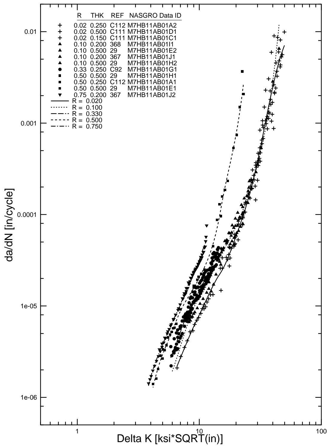
FIGURE B-27. SPLINE FIT FOR 7075-T651 PLATE, L-T (M7HB11AB1)
