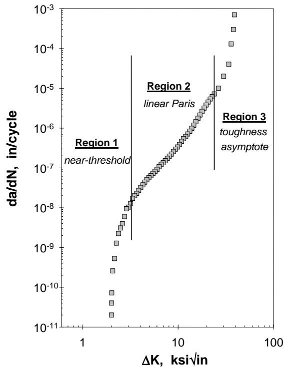
FIGURE 1. FATIGUE CRACK GROWTH RATE DATA ILLUSTRATING THE THREE REGIONS OF CRACK GROWTH BEHAVIOR
