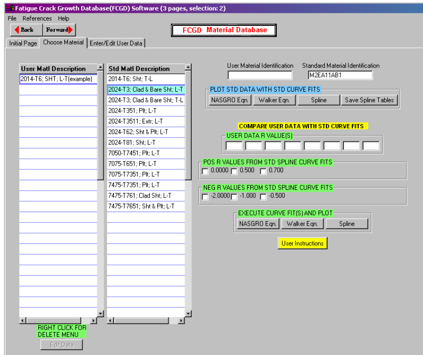
FIGURE C-2. MATERIAL SELECTION WINDOW FOR PLOTTING STANDARD DATA AND CURVE FITS
