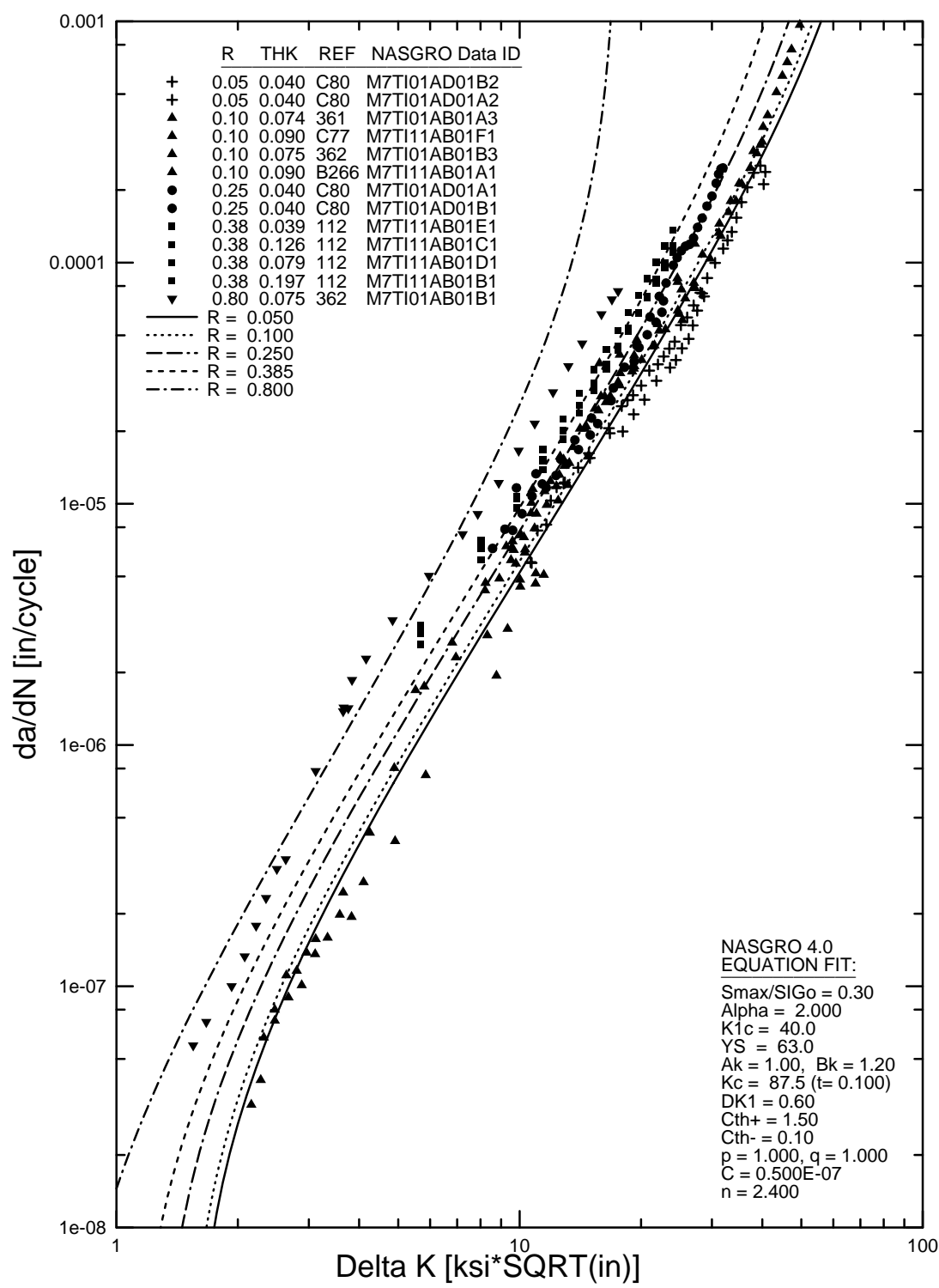
FIGURE B-34. NASGRO EQUATION FIT FOR 7475-T761 CLAD SHEET, L-T (M7TI01AB1)
