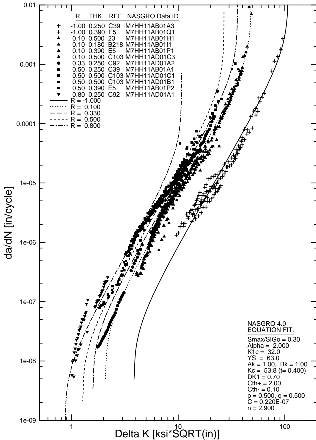
FIGURE B-28. NASGRO EQUATION FIT FOR 7075-T7351 PLATE, L-T (M7HH11AB1) WITH POSITIVE AND NEGATIVE R VALUES
