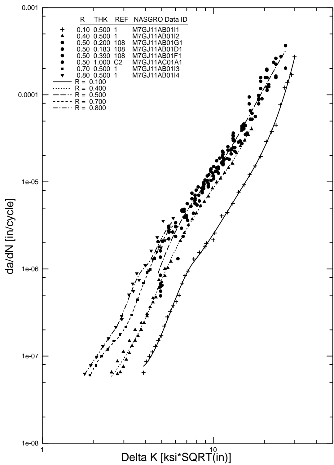
FIGURE B-24. SPLINE FIT FOR 7050-T7451 PLATE, L-T (M7GJ11AB1)
