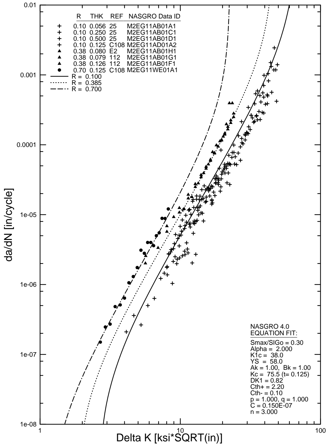
FIGURE B-16. NASGRO EQUATION FIT FOR 2024-T62 SHEET AND PLATE, L-T (M2EG11AB1)
