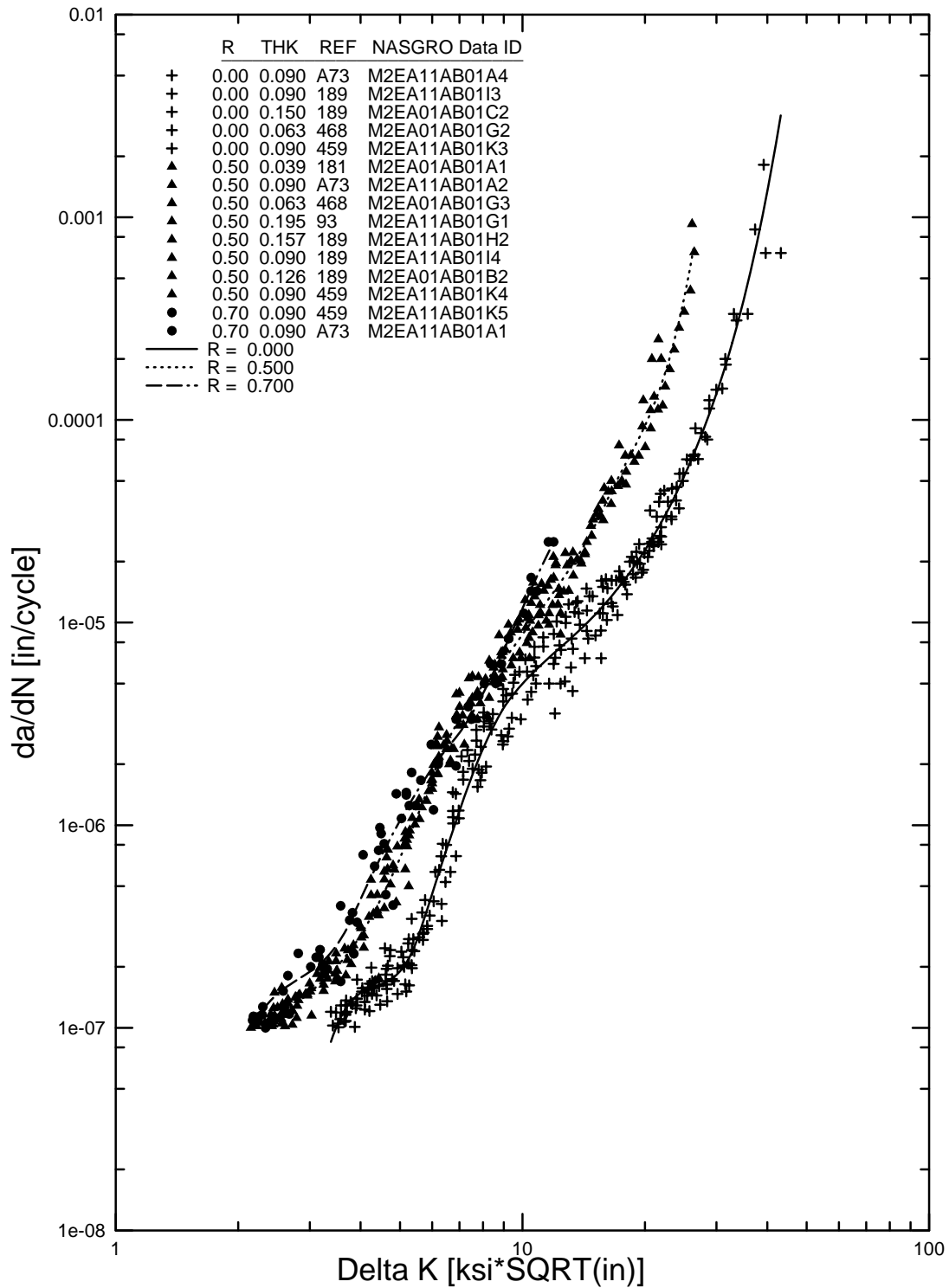
FIGURE B-6a. SPLINE FIT FOR 2024-T3 CLAD AND BARE SHEET, L-T (M2EA11AB1) WITH POSITIVE R VALUES
