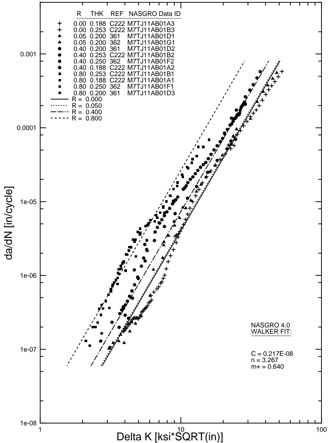
FIGURE B-38. WALKER EQUATION FIT FOR 7475-T7651 SHEET AND PLATE, L-T (M7TJ11AB1)
