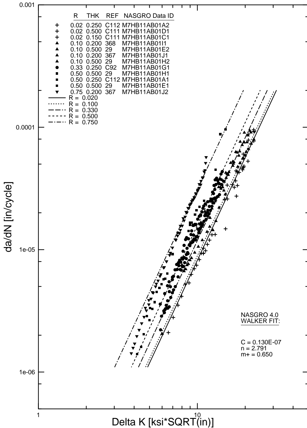
FIGURE B-26. WALKER EQUATION FIT FOR 7075-T651 PLATE, L-T (M7HB11AB1)
