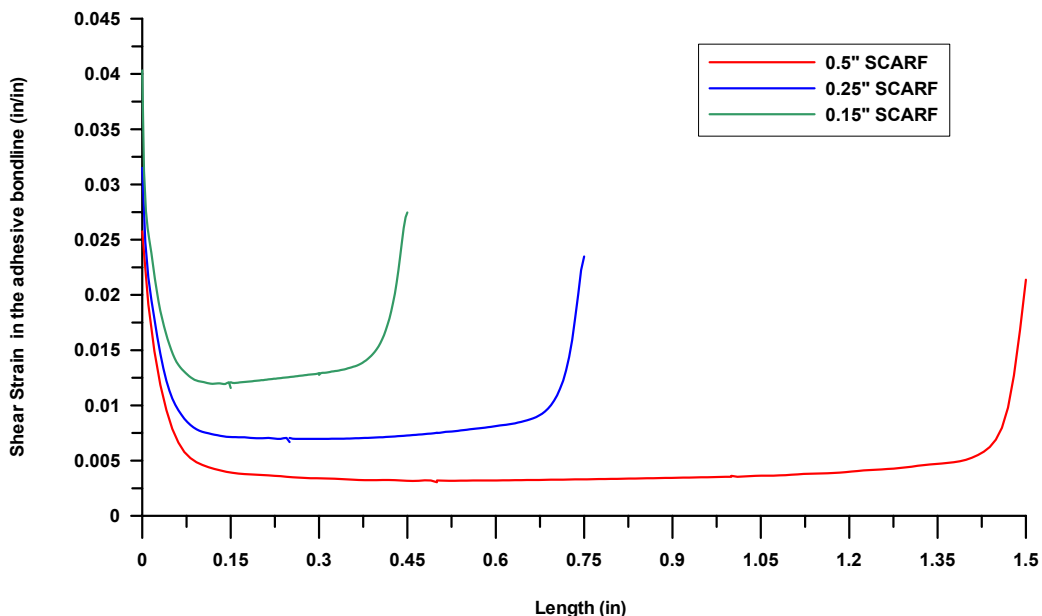
FIGURE 91. SHEAR STRAIN IN THE ADHESIVE BONDLINE FOR DIFFERENT SCARF REPAIRS ON THE 3/8-inch CORE UNIDIRECTIONAL TENSION COUPONS (WET LAY-UP REPAIR)
