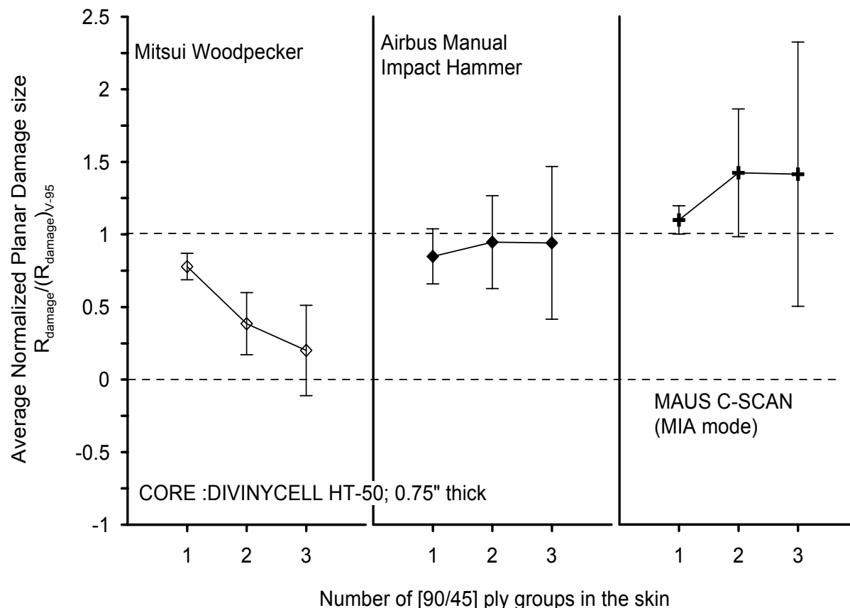
FIGURE 16. AVERAGE NORMALIZED DAMAGE SIZE FOR SANDWICH PANELS WITH DIFFERENT FACESHEET CONFIGURATIONS, WITH 0.75" THICK, 2.6 lb/ft 3 CORES ONLY
