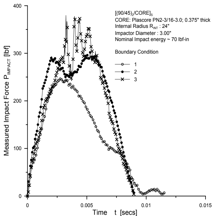
FIGURE 34. IMPACT RESPONSES OF [(90/45) 2 /CORE] s WITH R INT =24" AND DIFFERENT BOUNDARY CONDITIONS IMPACTED WITH 3.00" IMPACTOR WITH NOMINAL ENERGY OF 70 lbf-in
