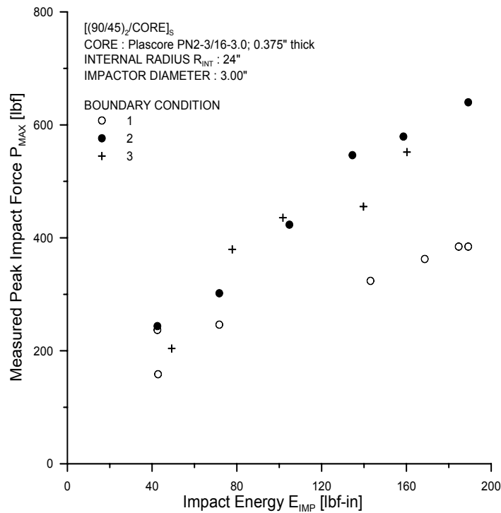
FIGURE 36. PEAK IMPACT FORCE AT VARIOUS ENERGY LEVELS FOR [(90/45) 2 /CORE] s SPECIMENS WITH DIFFERENT BOUNDARY CONDITIONS
