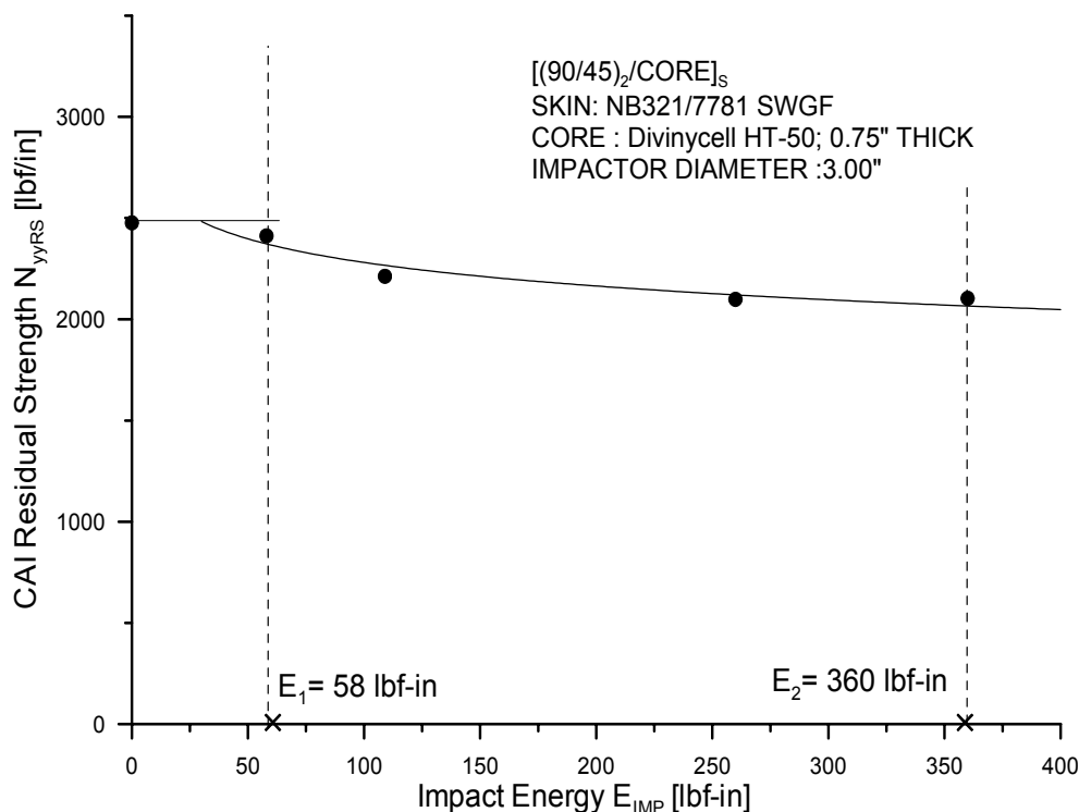
FIGURE 52. IMPACT ENERGY LEVELS FOR [(90/45)_2/CORE]_s SANDWICH PANELS (FOAM CORE) BASED ON CAI DATA
