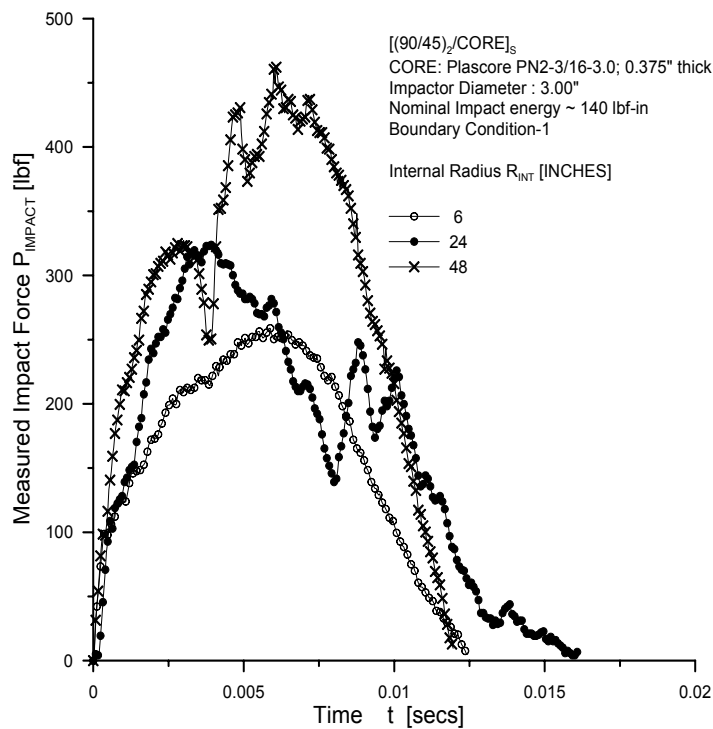
FIGURE 30. IMPACT RESPONSES OF [(90/45)_2/CORE]_s SANDWICH PANELS WITH DIFFERENT INTERNAL RADIUS R_{INT} AT NOMINAL IMPACT ENERGY OF 140 lbf-in
