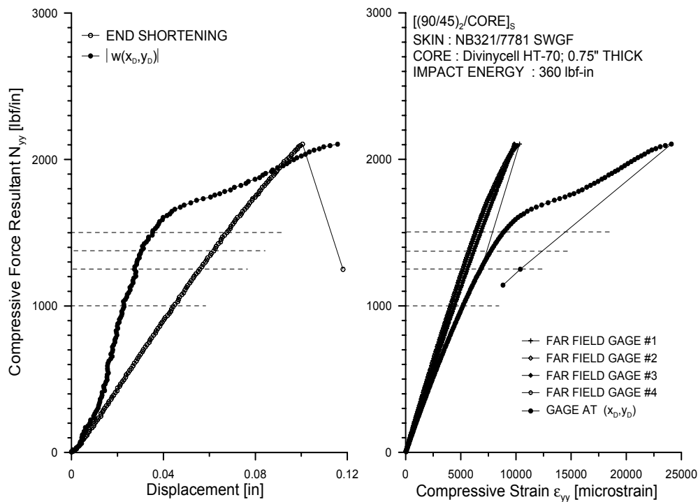
FIGURE 60. CAI TEST DATA FOR [(90/45)_2/CORE]_s SPECIMEN HONEYCOMB CORE IMPACTED WITH ENERGY LEVEL E_2=360 lbf-in
