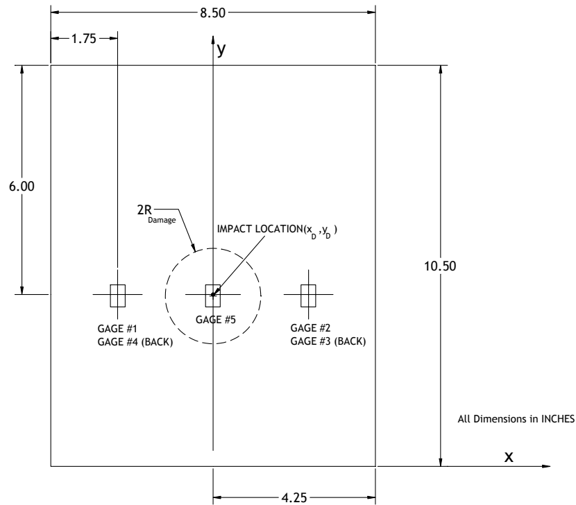
FIGURE 48. GEOMETRY OF TEST SPECIMEN AND LOCATION OF STRAIN GAGES
