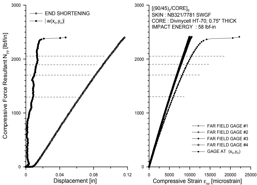
FIGURE 59. CAI TEST DATA FOR [(90/45)_2/CORE]_s SPECIMEN FOAM CORE IMPACTED WITH ENERGY LEVEL E_1=58 lbf-in
