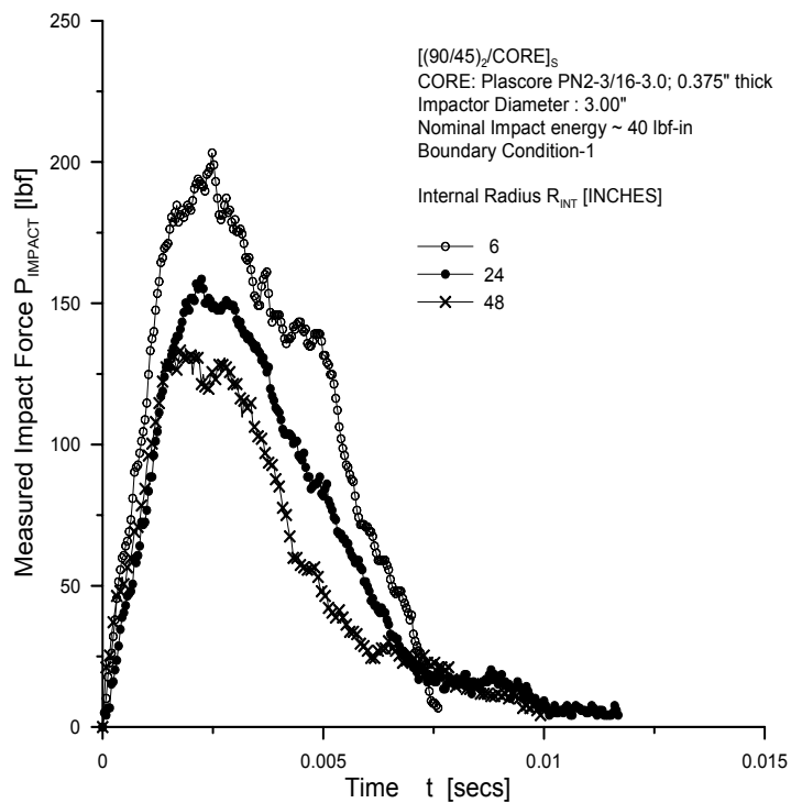
FIGURE 29. IMPACT RESPONSES OF [(90/45)_2/CORE]_s SANDWICH PANELS WITH DIFFERENT INTERNAL RADIUS R_{INT} AT NOMINAL IMPACT ENERGY OF 40 lbf-in
