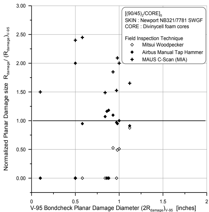
FIGURE 15. NORMALIZED DAMAGE SIZES FOR [(90/45)_3/\text{CORE}]_s FOAM CORE SANDWICH PANELS USING DIFFERENT FITs
