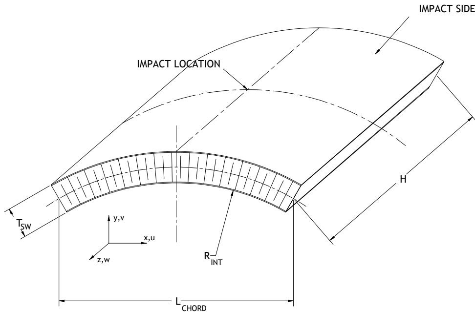
FIGURE 24. GEOMETRY OF CYLINDRICAL SANDWICH PANELS AND ASSOCIATED NOMENCLATURE
