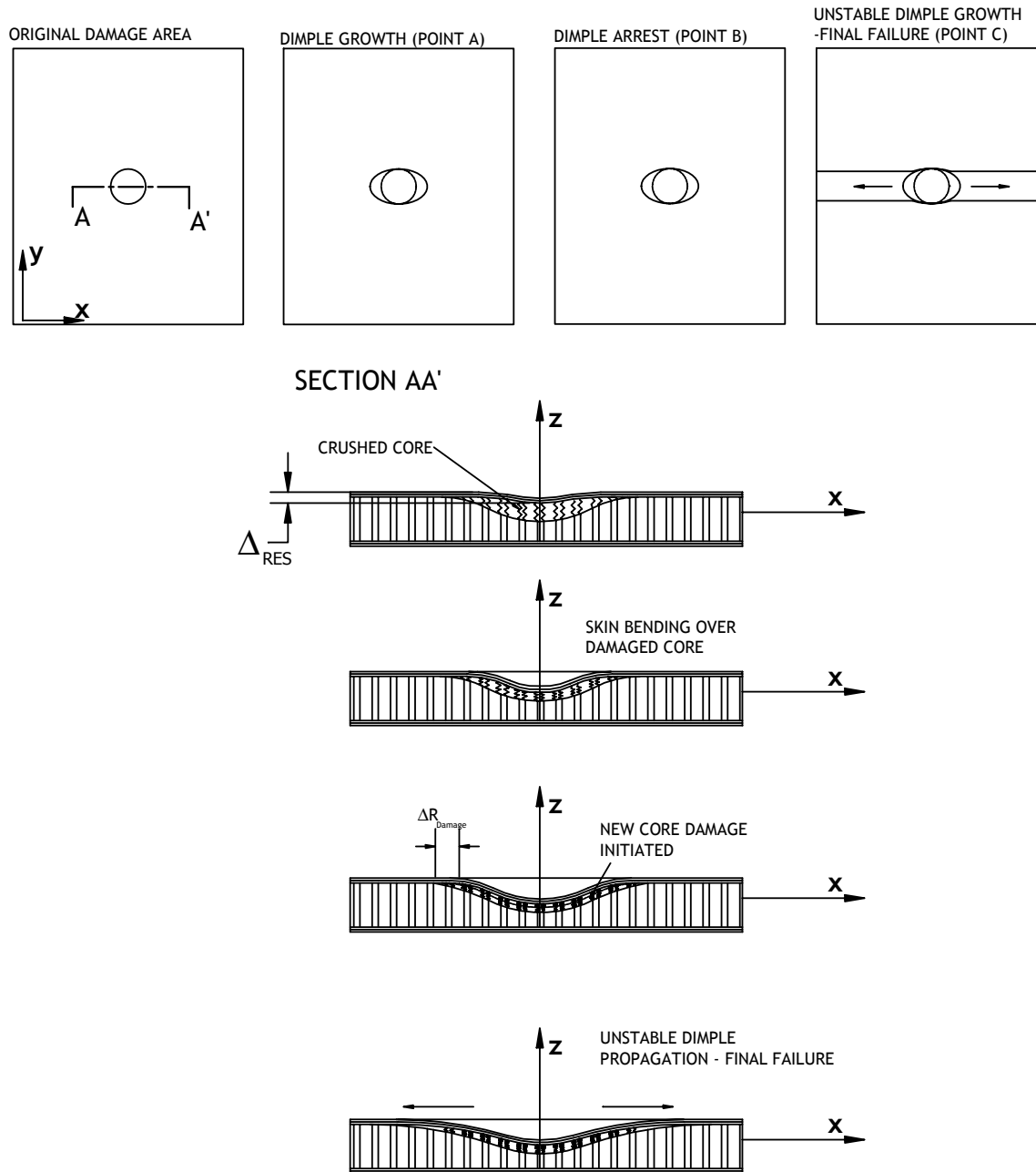
FIGURE 22. DAMAGE GROWTH MECHANISM AND FINAL FAILURE MODE OBSERVED IN [(90/45)_2/\text{CORE}]_s SANDWICH PANEL WITH HONEYCOMB CORE
