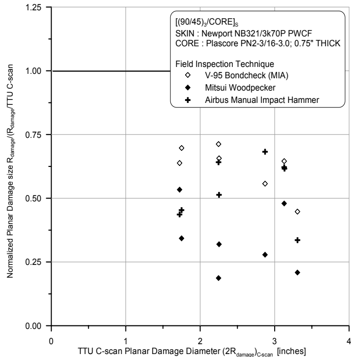
FIGURE 11. NORMALIZED DAMAGE SIZES FOR [(90/45)_3/CORE]_s HONEYCOMB CORE SANDWICH PANELS USING DIFFERENT FITS
