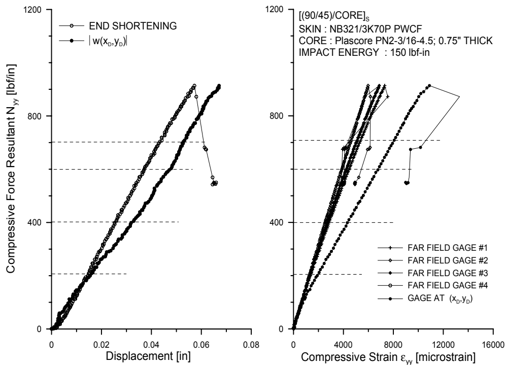
FIGURE 54. CAI TEST DATA FOR [(90/45)/CORE]_s SPECIMEN HONEYCOMB CORE IMPACTED WITH ENERGY LEVEL E_2=150 lbf-in
