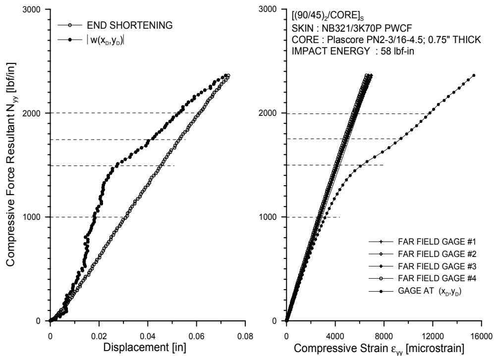
FIGURE 56. CAI TEST DATA FOR [(90/45)_2/CORE]_s SPECIMEN HONEYCOMB CORE IMPACTED WITH ENERGY LEVEL E_2=150 lbf-in
