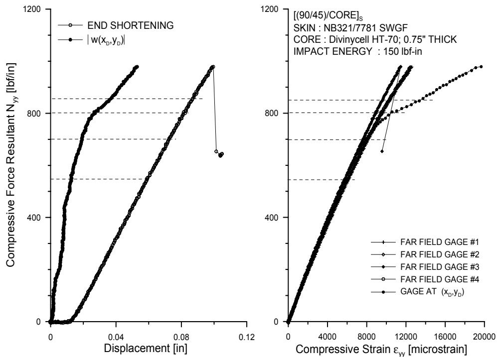
FIGURE 58. CAI TEST DATA FOR [(90/45)/CORE]_s SPECIMEN FOAM CORE IMPACTED WITH ENERGY LEVEL E_2=150 lbf-in
