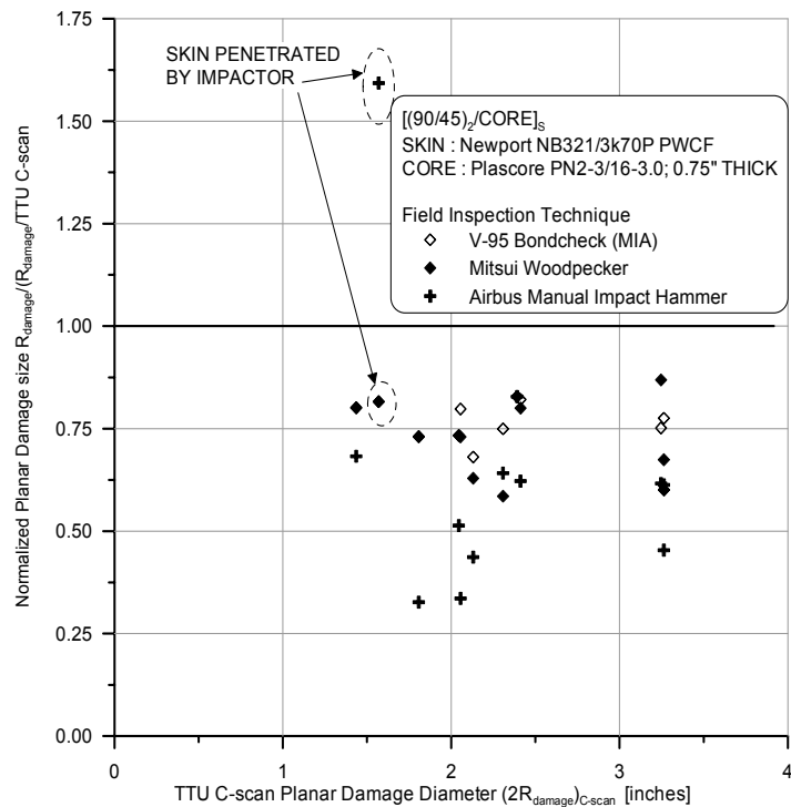
FIGURE 10. NORMALIZED DAMAGE SIZES FOR [(90/45)_2/CORE]_s HONEYCOMB CORE SANDWICH PANELS USING DIFFERENT FITS
