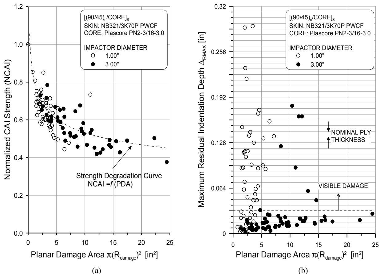
FIGURE 1. (a) NORMALIZED RESIDUAL STRENGTH FOR [(90/45)_N/\text{CORE}]_s ( N=1,2,3 ) 1 SANDWICH PANELS WITH HONEYCOMB CORE (3/8" AND 3/4" THICK) AND (b) VARIATION OF MAXIMUM RESIDUAL INDENTATION DEPTH WITH PLANAR DAMAGE AREA FOR THE SANDWICH PANELS
