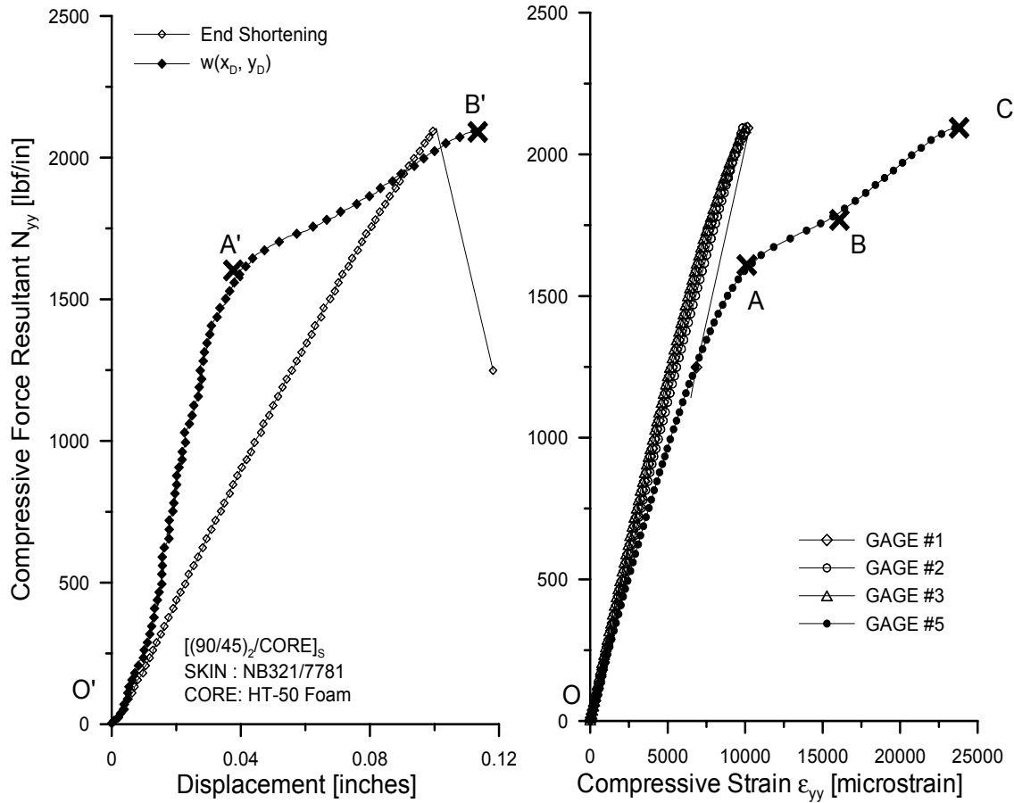
FIGURE 23. CAI TEST DATA FOR [(90/45)_2/CORE]_s SANDWICH PANEL WITH NB321/7781 SWGF FACESHEETS
