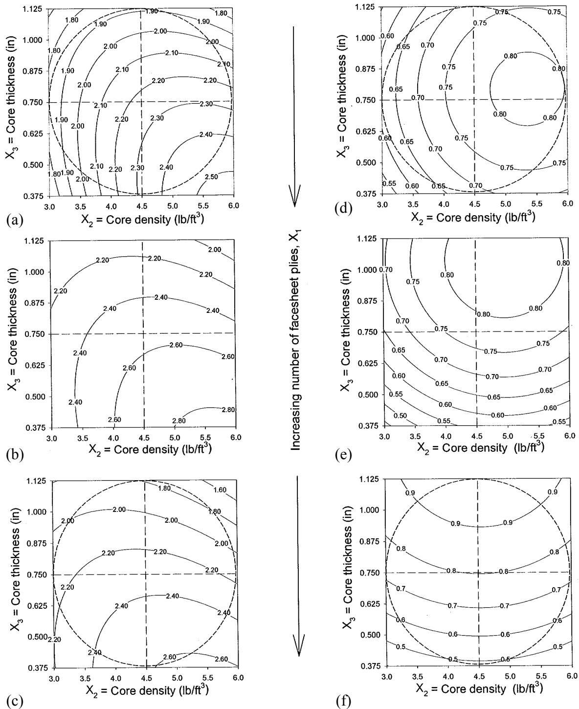
FIGURE 9. PREDICTED DAMAGE DIAMETER (in) FOR X_1 : (a) TWO, (b) FOUR, AND (c) SIX PLIES [13]; PREDICTED NORMALIZED RESIDUAL STRENGTH FOR X_1 : (d) TWO, (e) FOUR, AND (f) SIX PLIES
