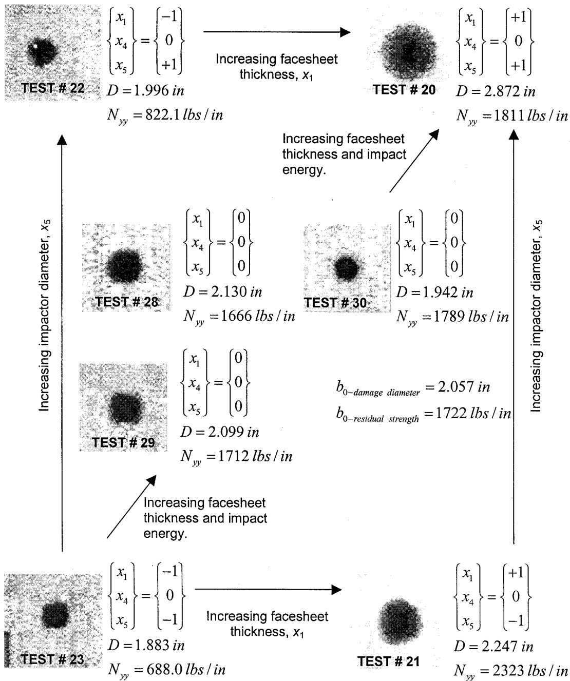
FIGURE 13. MEASURED DAMAGE DIAMETER [13] AND RESIDUAL STRENGTH FOR IMPACT ENERGY, X_4 = 120 in-lbs ( x_4 = 0 )
