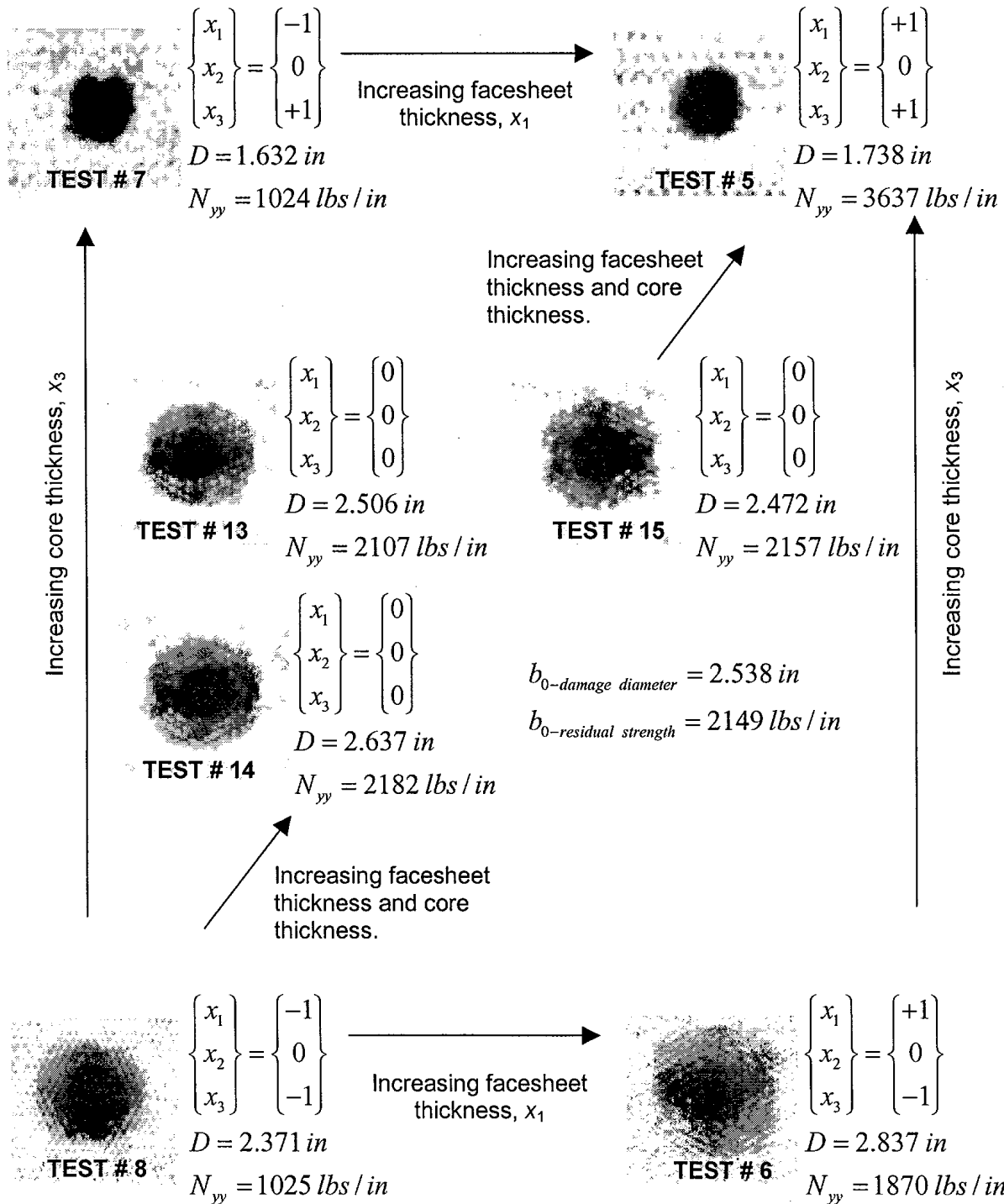
FIGURE 7. MEASURED DAMAGE DIAMETER [13] AND RESIDUAL STRENGTH FOR CORE DENSITY, X_2 = 4.5 lbs/ft 3 ( x_2 = 0 )
