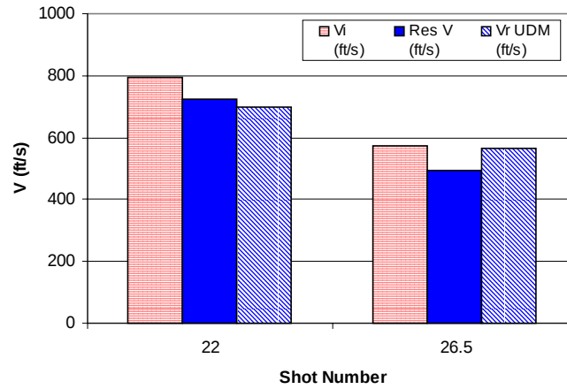
FIGURE 15. VELOCITY COMPARISON FOR IMPACTS INVOLVING SKIN AND HAT-STRINGER ELEMENTS
