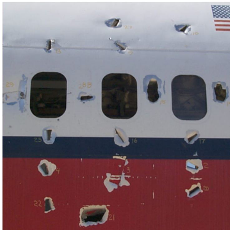
FIGURE 23. EXAMPLE EXTERIOR DAMAGE AREAS
