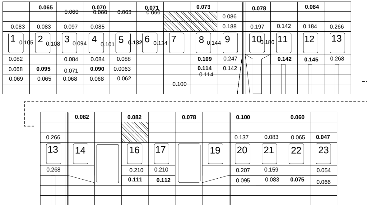
FIGURE 12. THICKNESS MAP OF THE PORTSIDE CABIN TEST AREA (inches)
