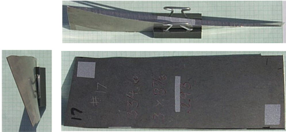
FIGURE 6. LARGE BLADE FRAGMENT USED IN SHOT 26B
