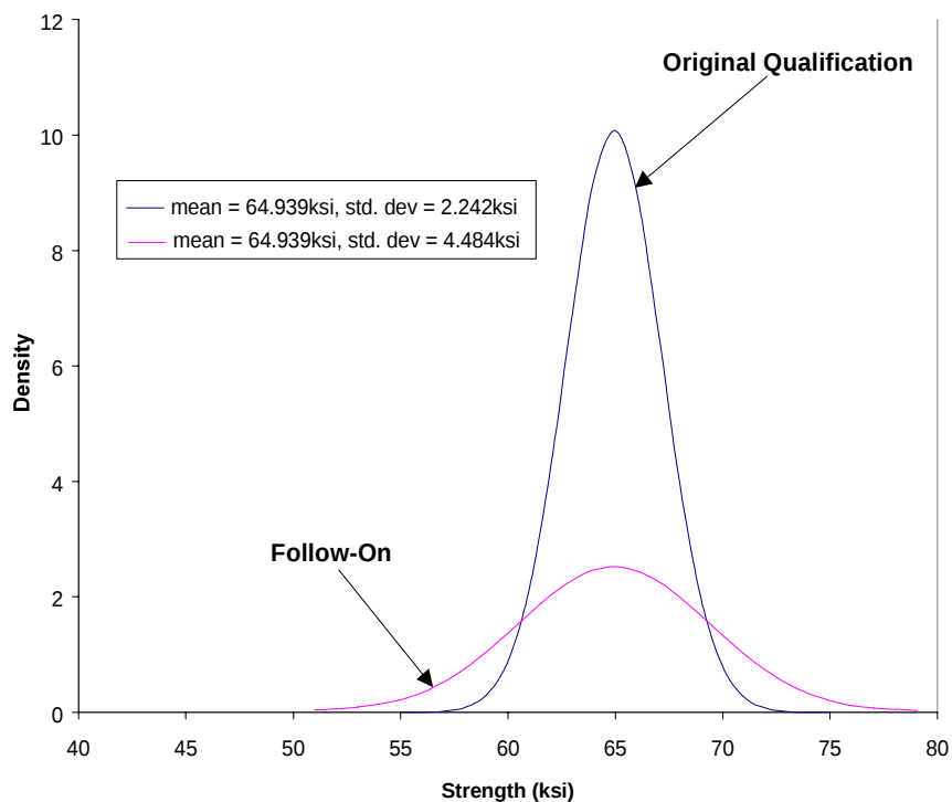
FIGURE 28. TWO NORMAL DISTRIBUTIONS, WITH EQUAL MEANS BUT UNEQUAL STANDARD DEVIATIONS
