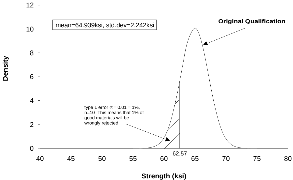
FIGURE 27. A NORMAL DISTRIBUTION, TEN SPECIMENS
