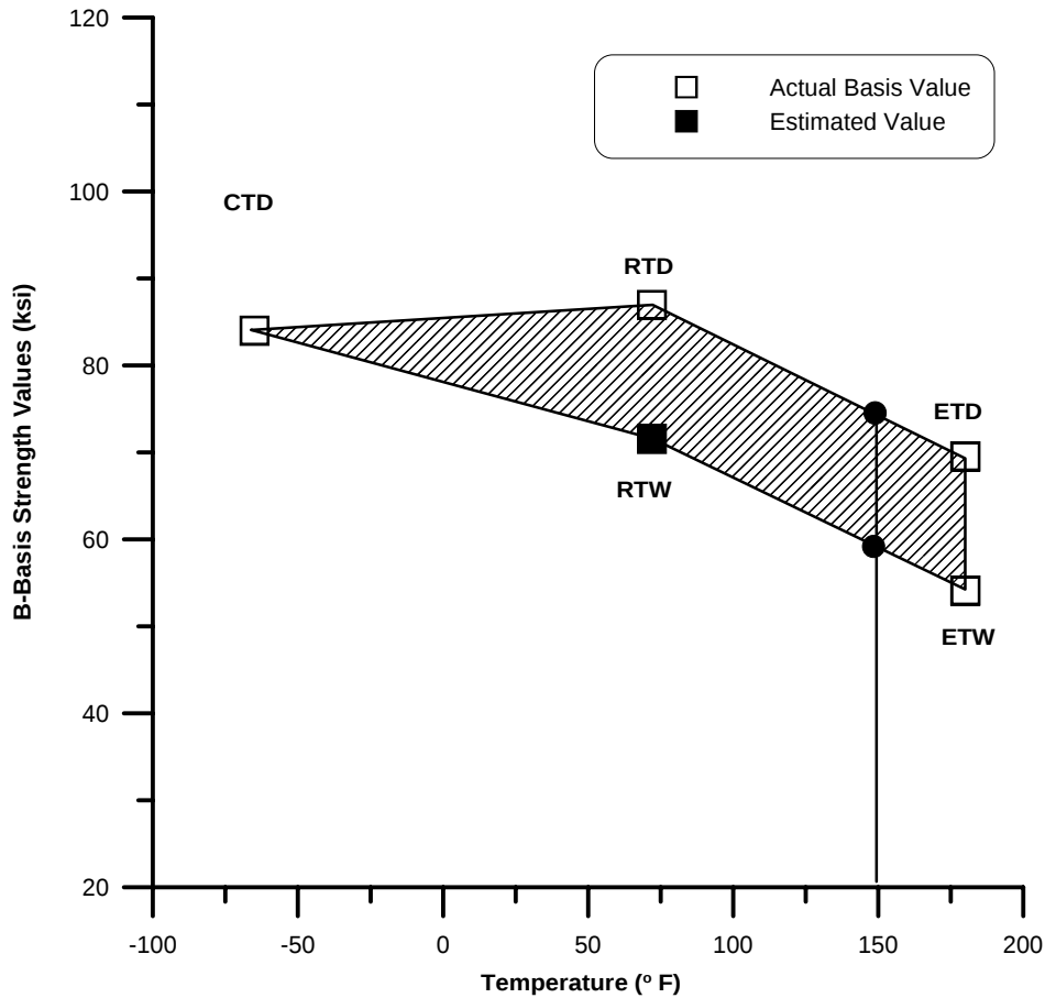
FIGURE 24. EXAMPLE OF 150°F INTERPOLATION FOR B-BASIS VALUES
