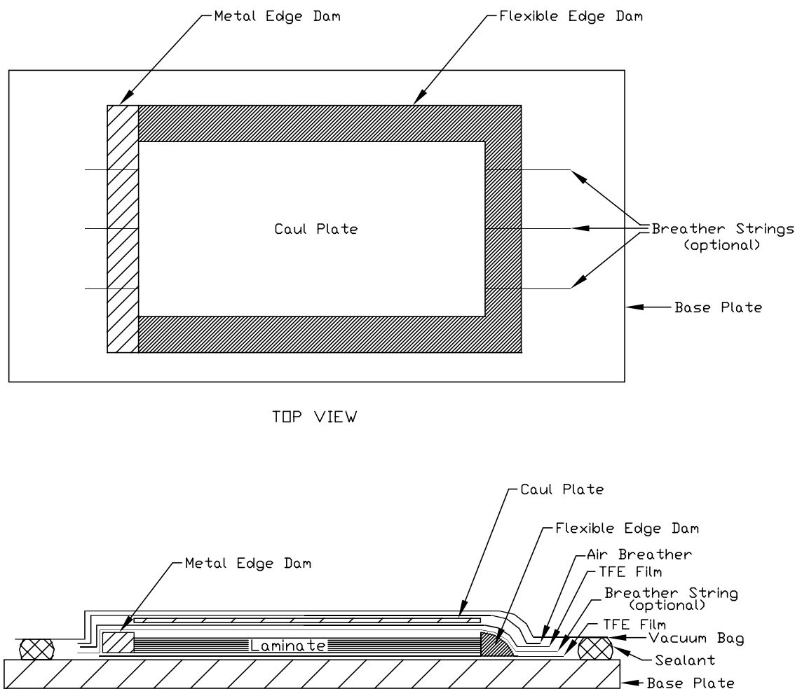
FIGURE C-1. RECOMMENDED LAY-UP TECHNIQUE (WITH FLEXIBLE EDGE DAM)
