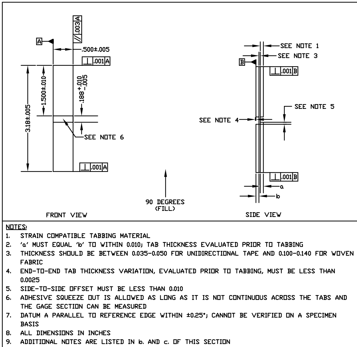
FIGURE 14. NINETY-DEGREE (FILL) WOVEN FABRIC AND UNIDIRECTIONAL COMPRESSION STRENGTH SPECIMENS
