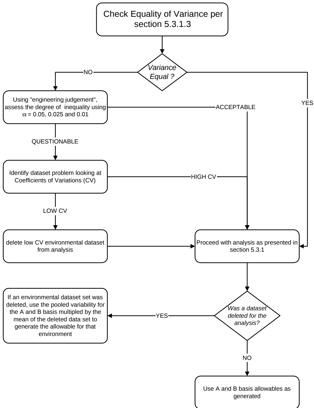
FIGURE 20. PROCUDURES TO OBTAIN DESIGN ALLOWABLES IN THE CASE OF VARIANCE INEQUALITY
