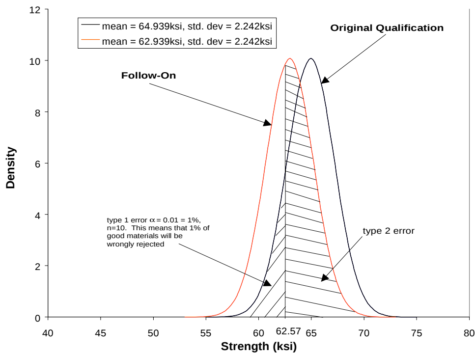
FIGURE 29. TWO NORMAL DISTRIBUTIONS OF EQUAL STANDARD DEVIATIONS, CLOSE BUT UNEQUAL MEANS, TEN SPECIMENS
