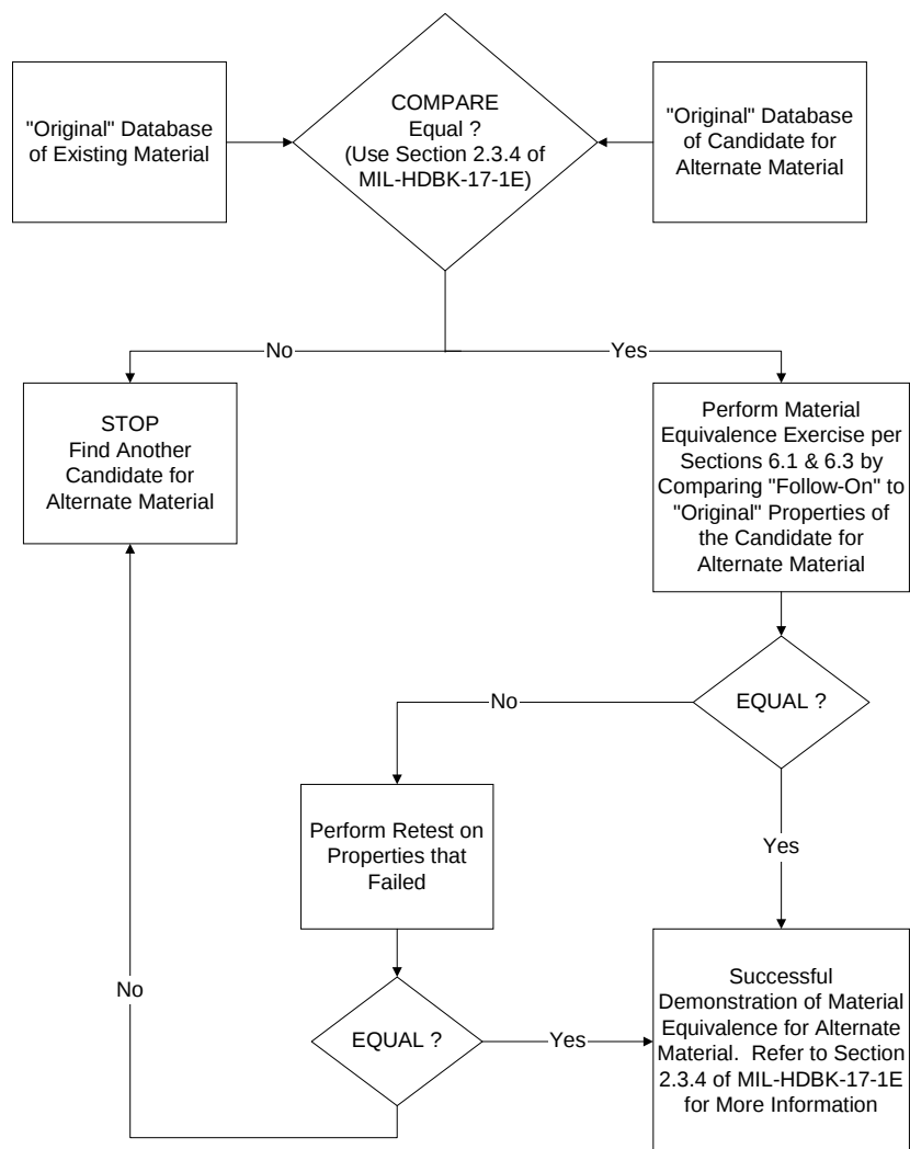
FIGURE 32. FLOWCHART ILLUSTRATING PROCEDURES FOR SELECTING AND DEMONSTRATING EQUIVALENCY FOR AN ALTERNATE MATERIAL
