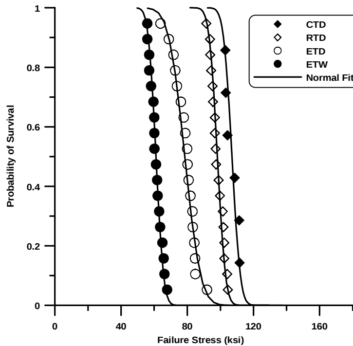
FIGURE 21. NORMALIZED FIT OF EXPERIMENTAL DATA FOR EACH ENVIRONMENT
