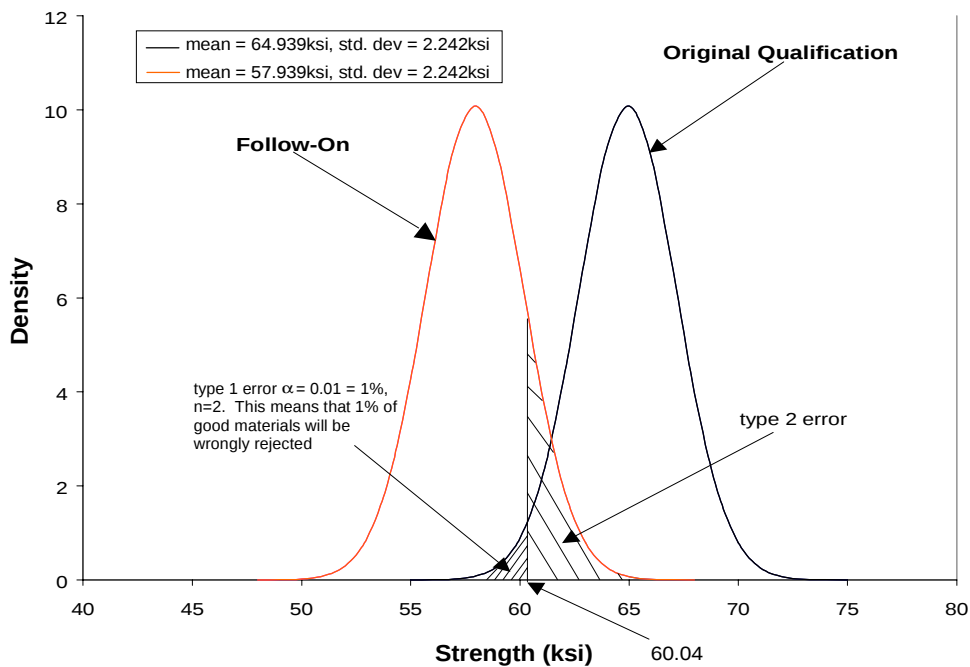
FIGURE 31. TWO NORMAL DISTRIBUTIONS OF EQUAL STANDARD DEVIATIONS, UNEQUAL MEANS, TWO SPECIMENS
