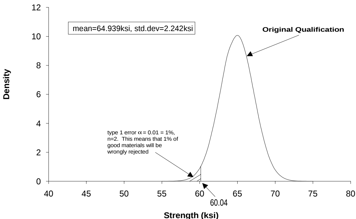
FIGURE 26. A NORMAL DISTRIBUTION, TWO SPECIMENS
