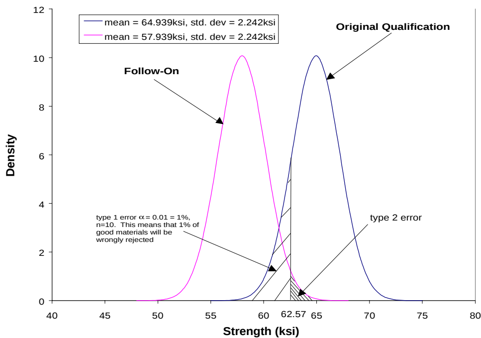
FIGURE 30. TWO NORMAL DISTRIBUTIONS OF EQUAL STANDARD DEVIATIONS, UNEQUAL MEANS, TEN SPECIMENS
