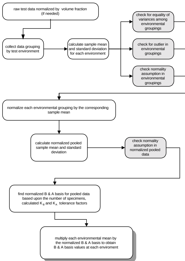
FIGURE 19. STEPWISE DATA REDUCTION PROCEDURE FOR DESIGN ALLOWABLE GENERATION
