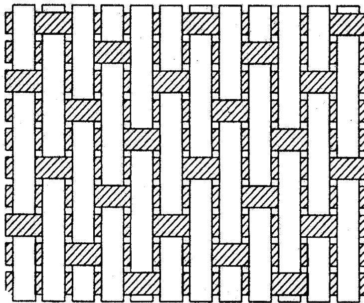
FIGURE 7. SATIN WEAVE FABRIC CONSTRUCTION (FIVE HARNESS SHOWN)
