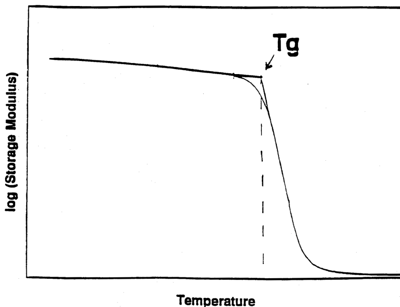
FIGURE 18. GLASS TRANSITION TEMPERATURE DETERMINATION FROM STORAGE MODULUS
