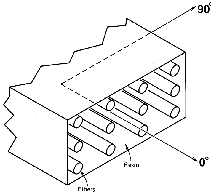
FIGURE 4. UNIDIRECTIONAL TAPE WITH DEFINED DIRECTIONS
