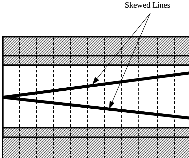
FIGURE 3. SKEWED LINES DRAWN ACROSS SUBPANEL USED FOR RECONSTRUCTION
