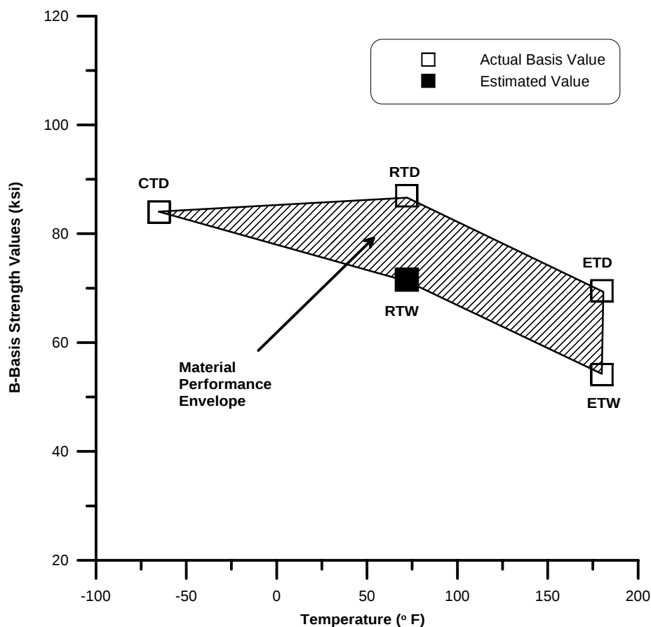
FIGURE 23. MATERIAL PERFORMANCE ENVELOPE
