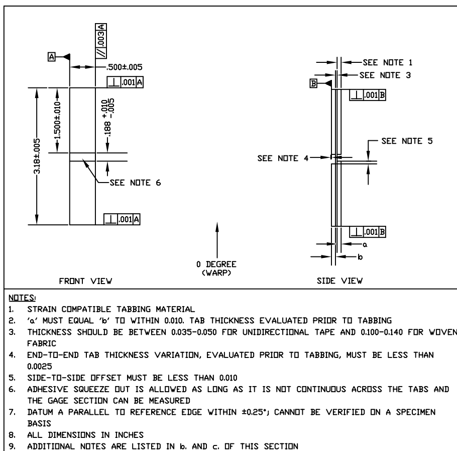
FIGURE 12. ZERO-DEGREE (WARP) WOVEN FABRIC AND UNIDIRECTIONAL COMPRESSION STRENGTH SPECIMENS
