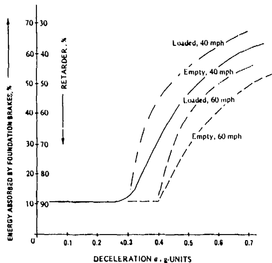
Figure 4-3. Distribution of Braking Energy Between Retarder and Foundation Brakes for 60 and 40 mph Stops for Optimum Lining Life Design
