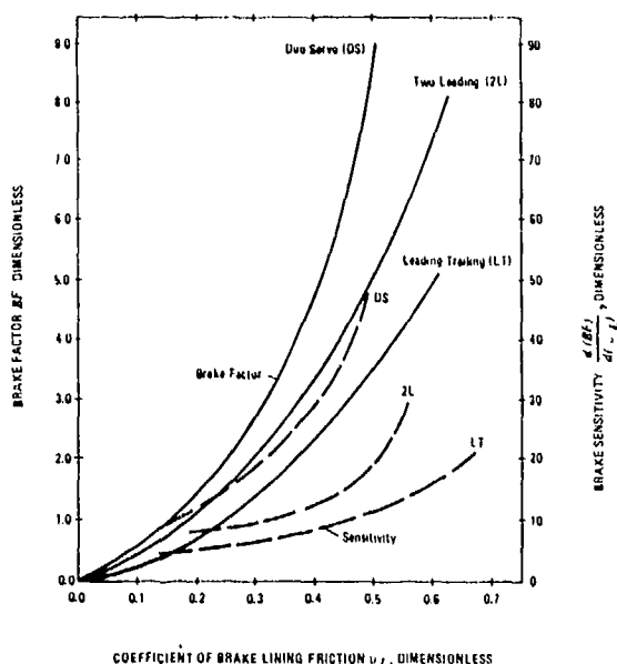
Figure 7-1. Brake Factor — Lining Friction Curves for Typical Drum Brakes
