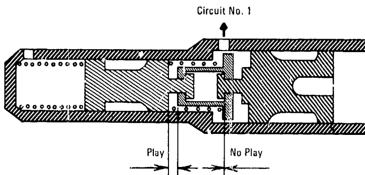
(C) Stepped Bore Master Cylinder, Brake Application With Leakage in Secondary Circuit Number 2
