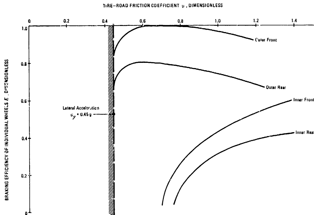
Figure 8-12. Braking Efficiency for Combined Braking and Turning (Fiat 124)
