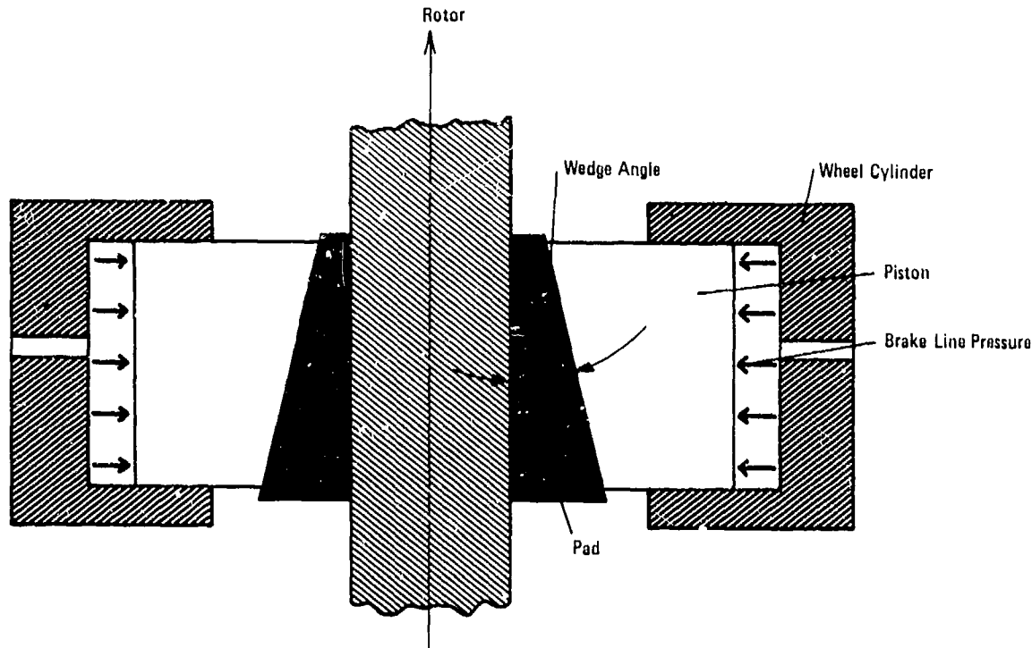
Figure 2-23. Self-Energizing of Caliper Disc Brake
