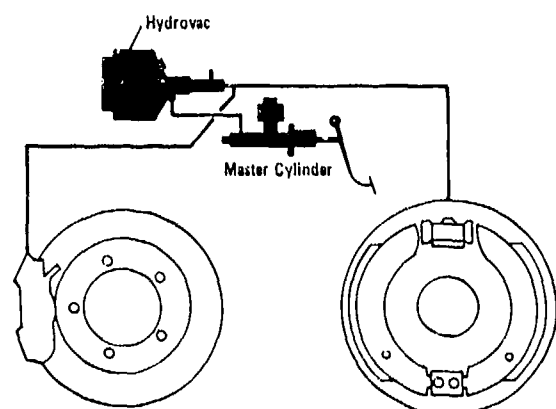
Figure 15-10. Hydrovac Brake System
