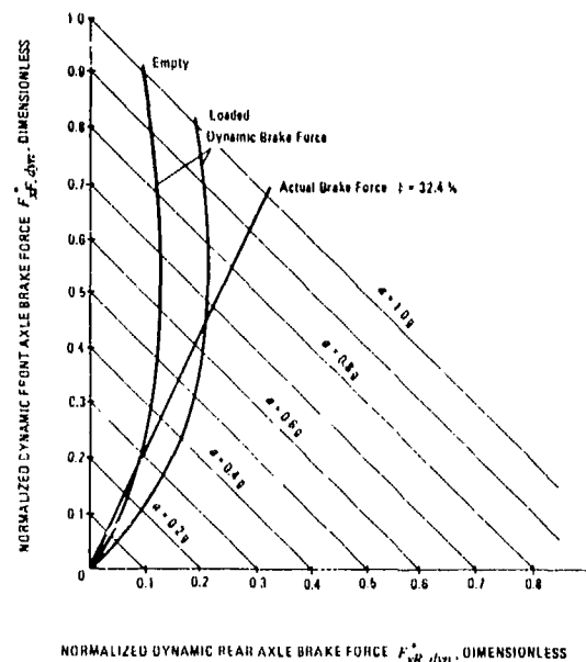
Figure 14-9. Normalized Dynamic and Actual Brake Forces, Vehicle No. 1
