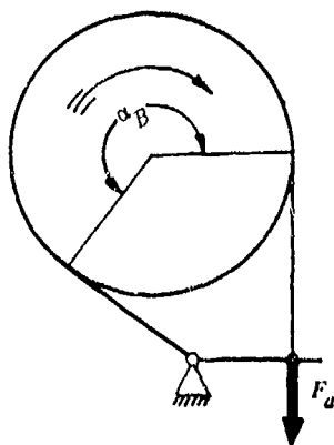
Figure 2-20. Single Application External Band Brake
