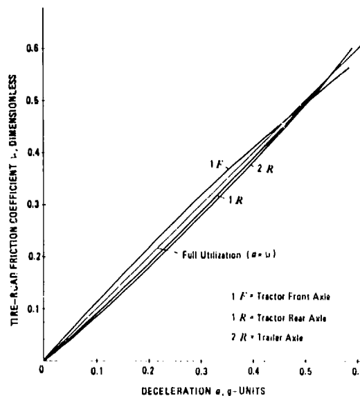
Figure 9-18. Tire-Road Friction Utilization, Case 7, W_2 = 11,500 lb
