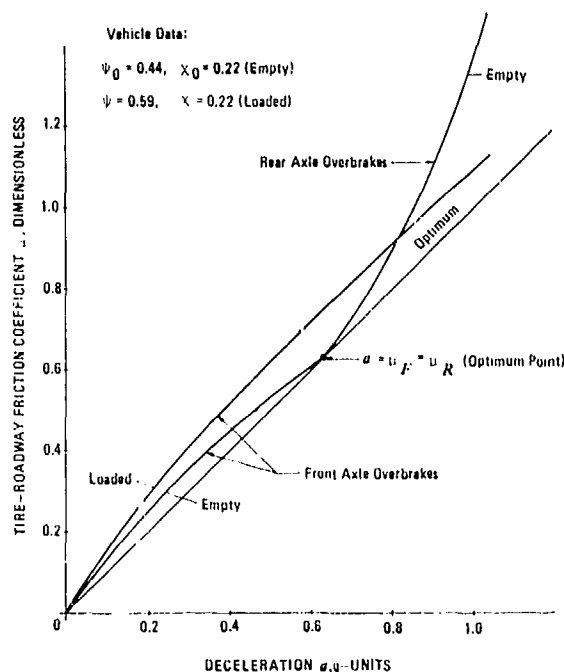
Figure 8-6 Tire-Road Friction Utilization
