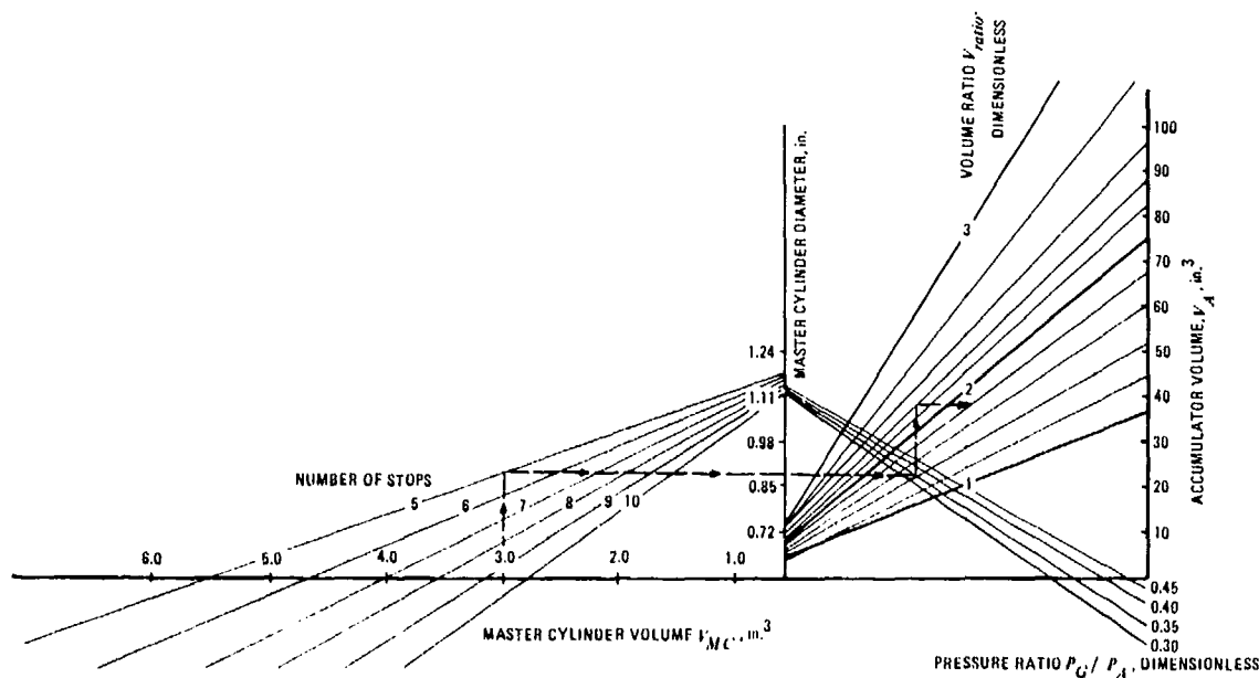
Figure 5-9. Accumulator Design Chart
