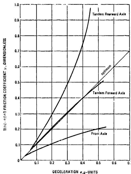
Figure 8-18. Tire-Road Friction Utilization for a Truck Equipped With Walking Beam Suspension
