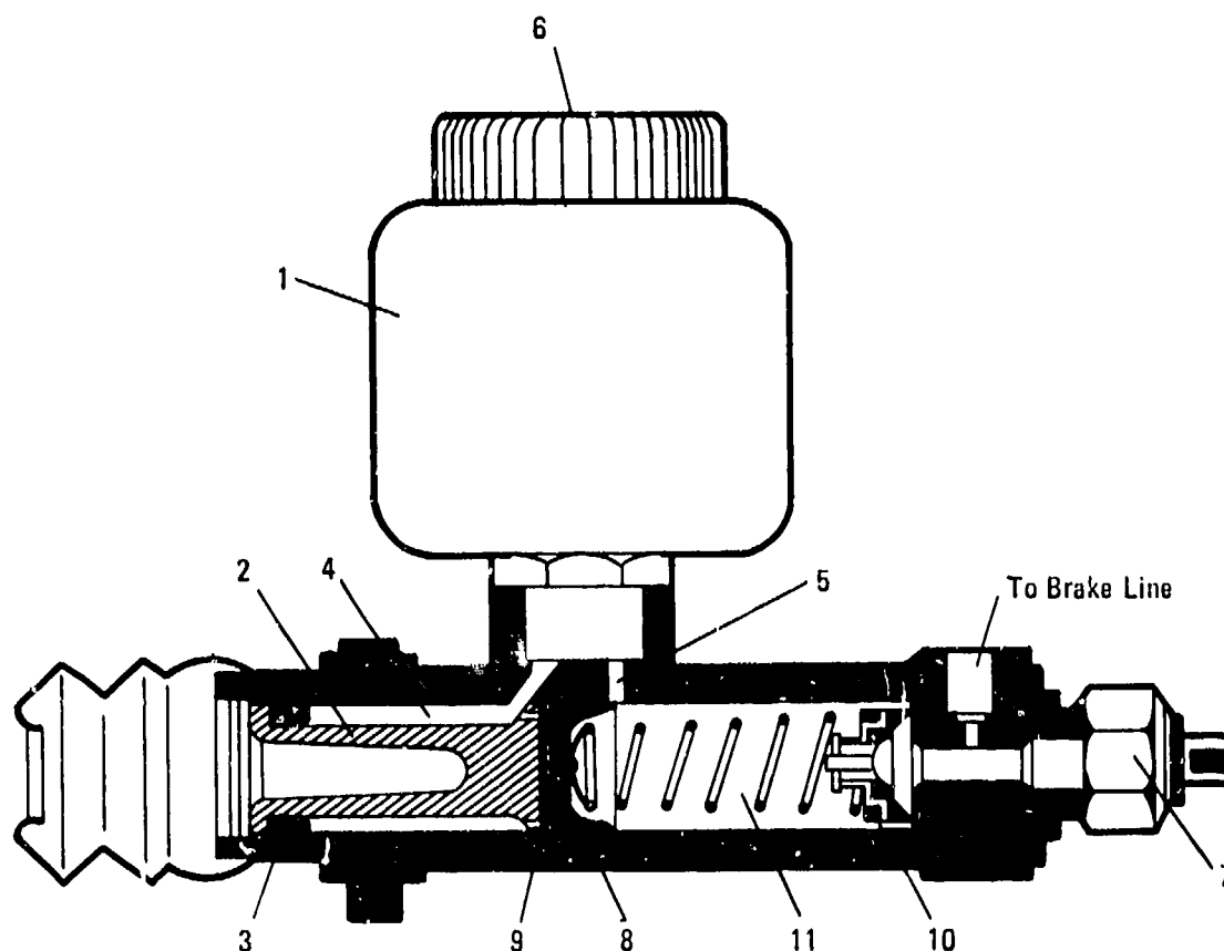
Figure 15-2. Master Cylinder
