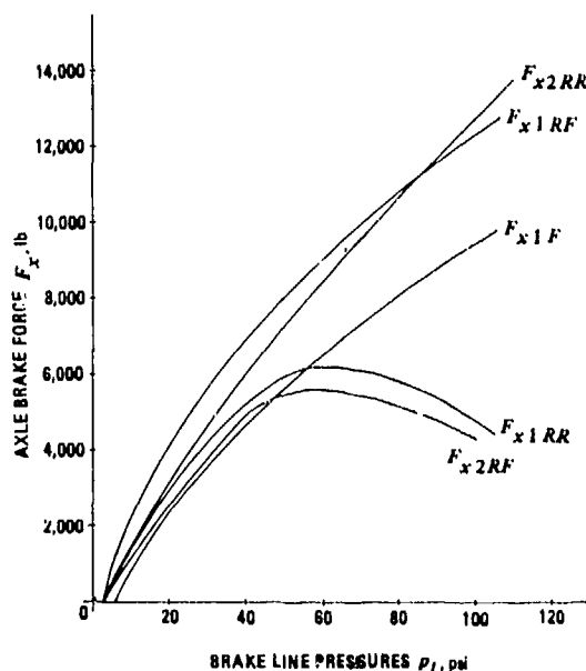
Figure 8-42. Axle Brake Forces
