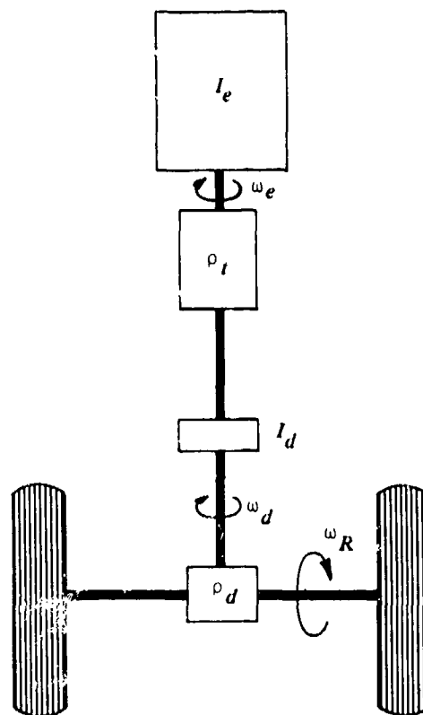
Figure 8-45. Rotational Inertias of a Rear Wheel Driven Vehicle
