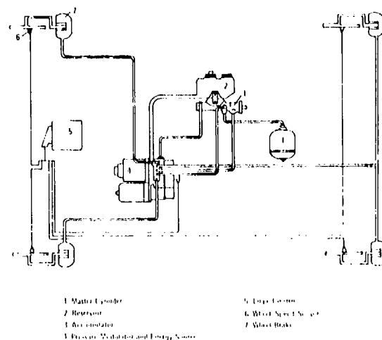
Figure 10-8. Schematic of Pump Pressurized Wheel Antilock System
