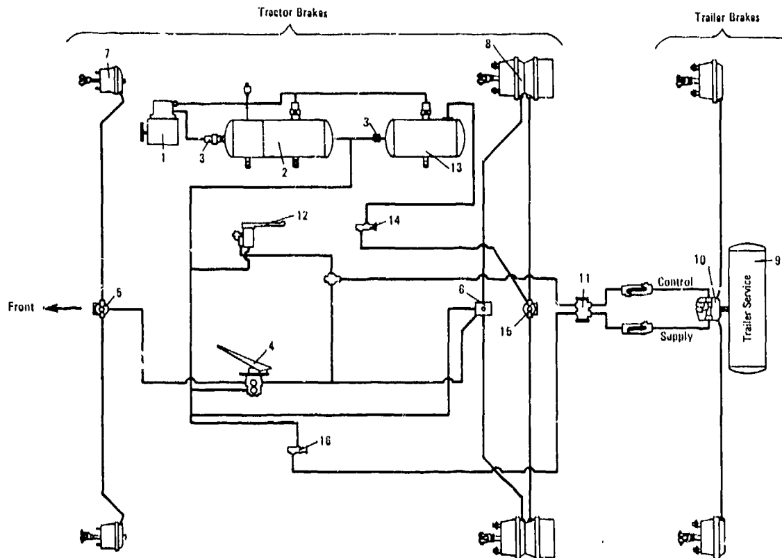
Figure 15-13. Tractor-Semitrailer Air Brake System
