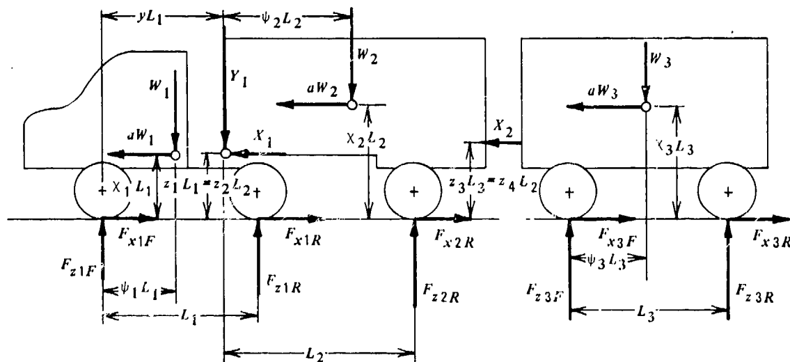
Figure 8-43. Forces Acting on a Tractor-Semitrailer-Double-Trailer Combination
