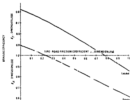
Figure 14-14. Braking Efficiency, Vehicle No. 3
