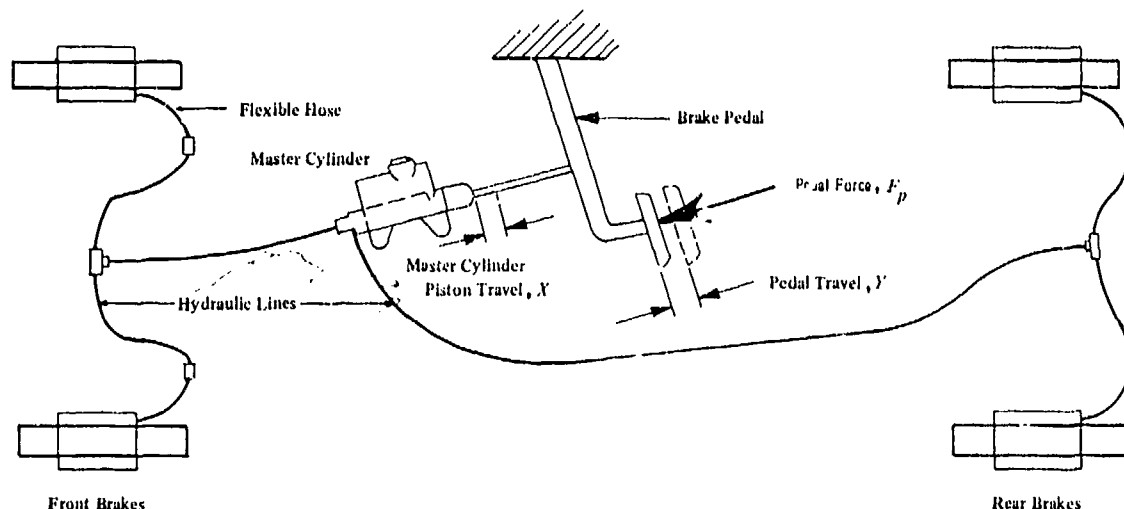
Figure 5-1. Hydraulic Brake System
