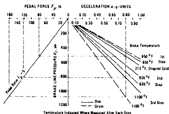
Figure 12-11. Fade Effectiveness Diagram
