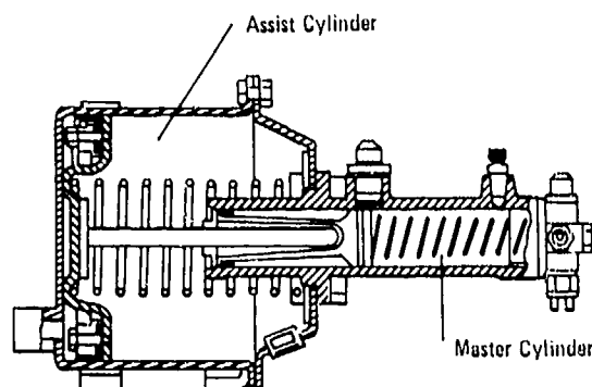
Figure 5-10. Air-Over-Hydraulic Brake Unit
