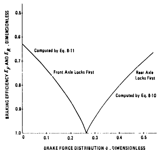
Figure 14-15. Braking Efficiency of Loaded Vehicle 1 as a Function of Brake Force Distribution \phi for a Tire-Road Friction Coefficient of 0.8
