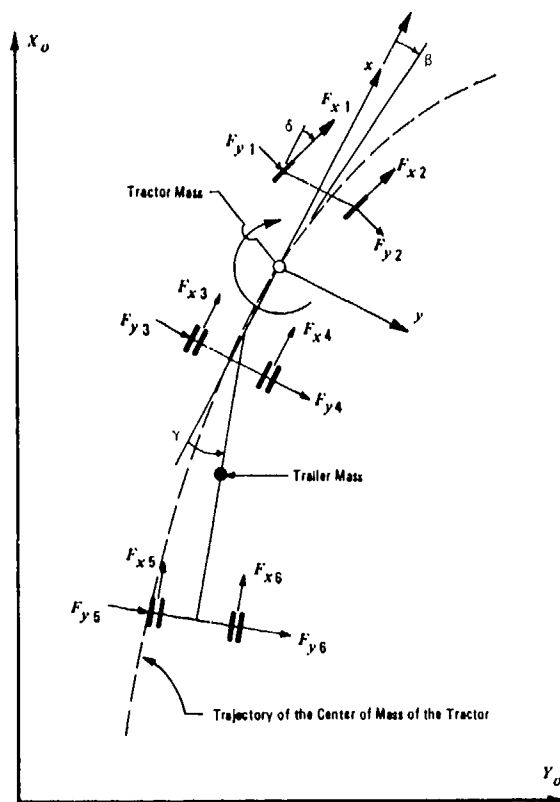
Figure 7-5. Tractor-Semitrailer Vehicle Model
