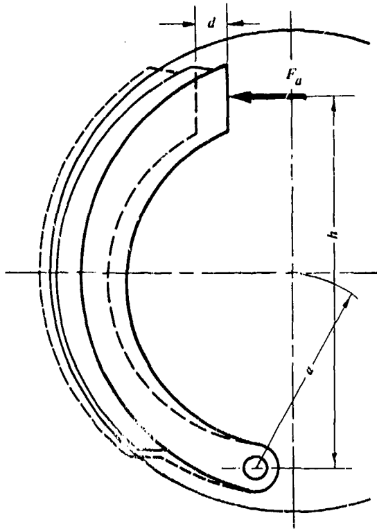
Figure 2-4. Brake Shoe Geometry
