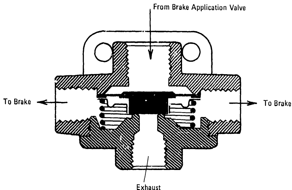
Figure 15-15. Quick-Release Valve
