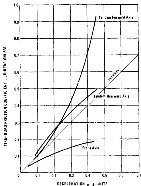
Figure 8-25. Tire-Road Friction Utilization for Truck Equipped With Two-Leaf-Two-Rod Suspension
