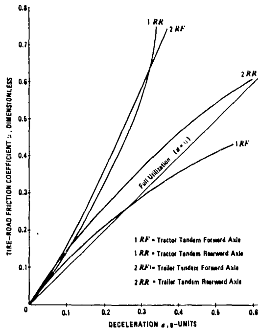
Figure 9-23. Tire-Road Friction Utilization for 3-S2 Tractor-Semitrailer Combination (Empty) With Standard Brakes (No Front Brakes)
