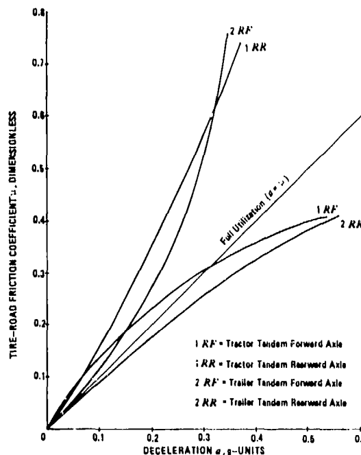
Figure 9-24. Tire-Road Friction Utilization for 3-S2 Tractor-Semitrailer Combination (Loaded) With Standard Brakes (No Front Brakes)
