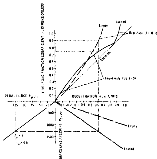
Figure 14-18. Braking Performance Diagram, Vehicle No. 6
