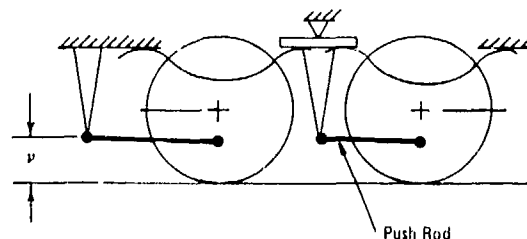
Figure 8-24. Two-Leaf-Two-Rod Suspension
