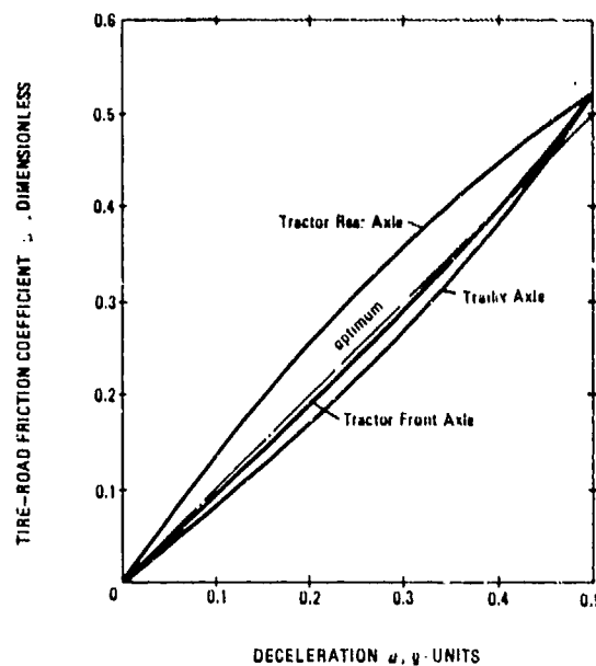
Figure 8-32. Tire-Road Friction Utilization for a Loaded Tractor-Semitrailer
