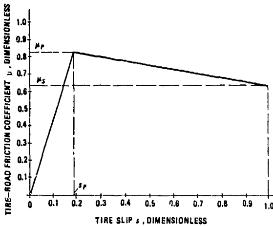
Figure 10-1. Idealized Tire-Road Friction Slip Characteristics
