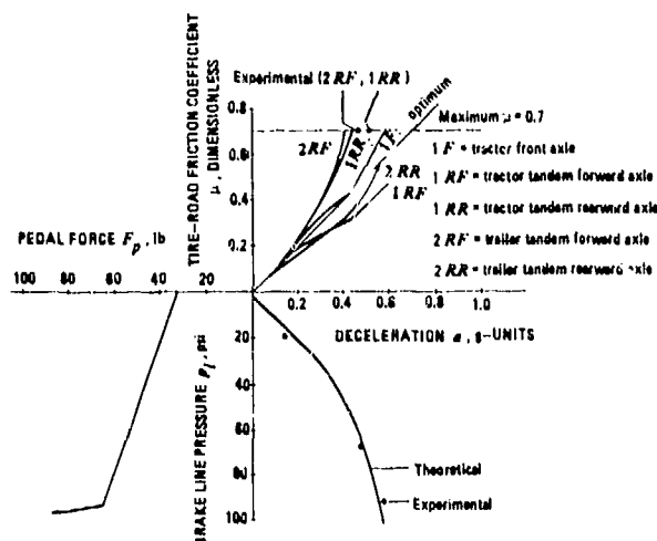
Figure 8-40. Braking Performance Diagram for a Loaded Tandem Axle Tractor — Tandem Axle Semitrailer Combination
