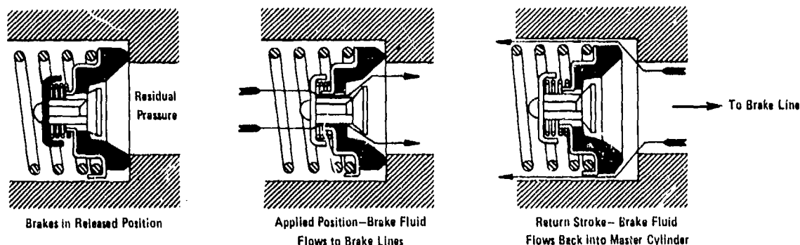
Figure 15-3. Residual-Pressure Check Valve Operation
