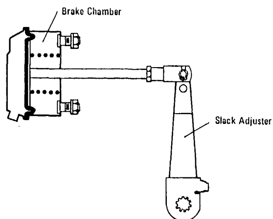
Figure 15-17. Air Brake Chamber
