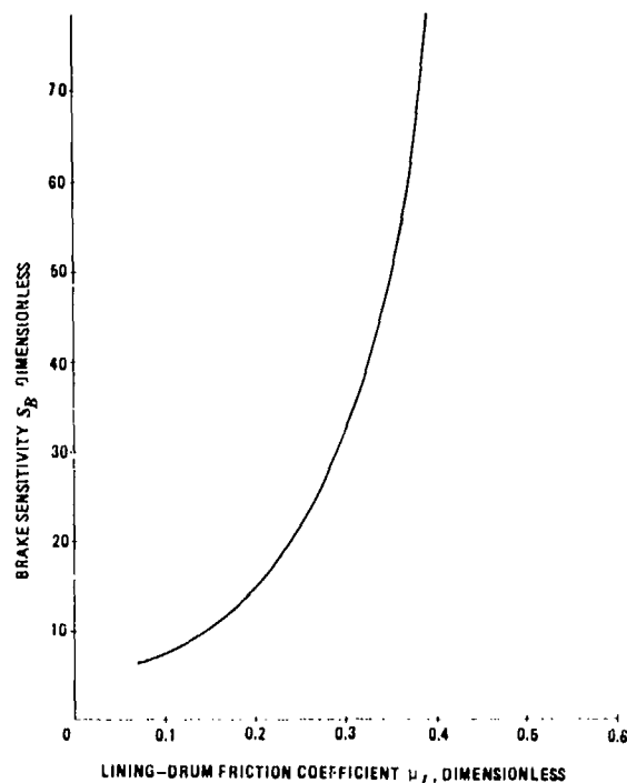
Figure 14-2. Brake Sensitivity
