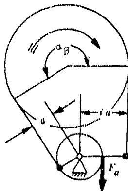
Figure 2-21. Opposing Application External Band Brake
