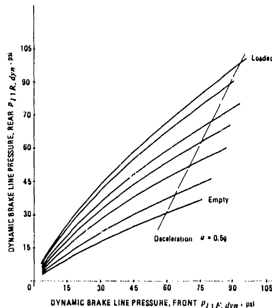
Figure 9-21. Dynamic Brake Line Pressures for the Tractor of a Tractor-Semitrailer Combination
