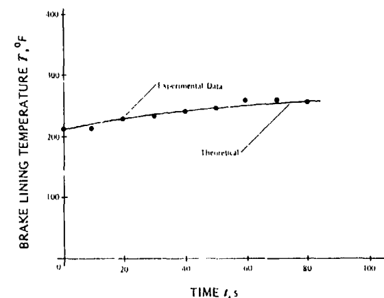
Figure 3-7. Brake Lining Temperature Attained in Brake Rating Test
