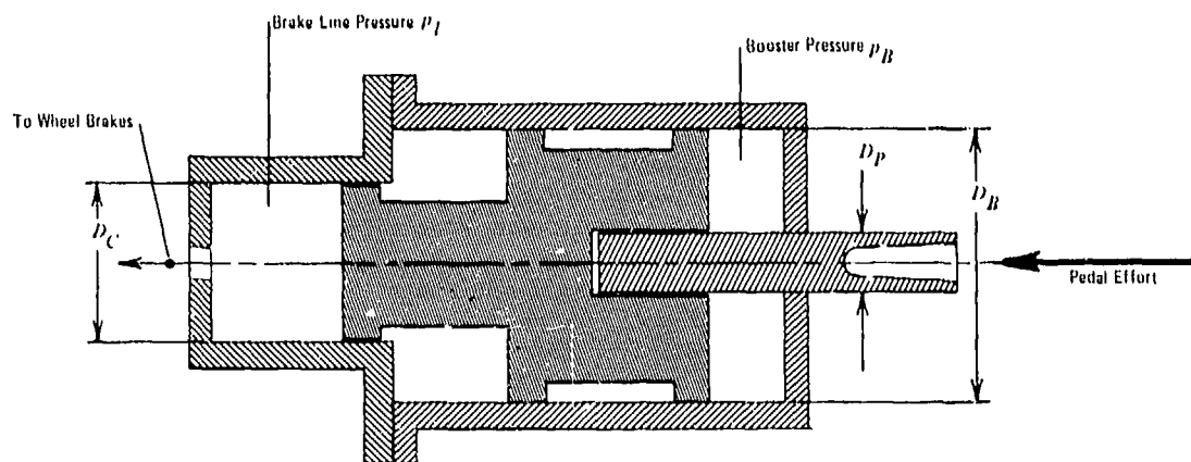
Figure 5-8. Schematic of Hydraulic Booster
