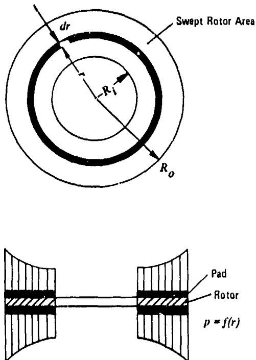
Figure 2-10. Pressure Distribution on a Disc Brake
