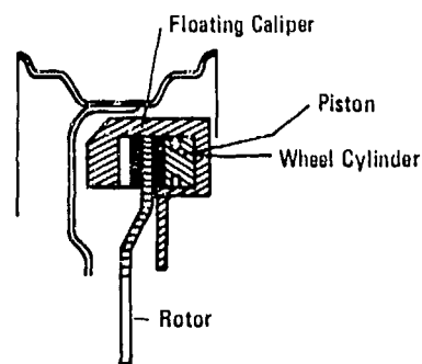
Single Piston-Floating Caliper Brake
