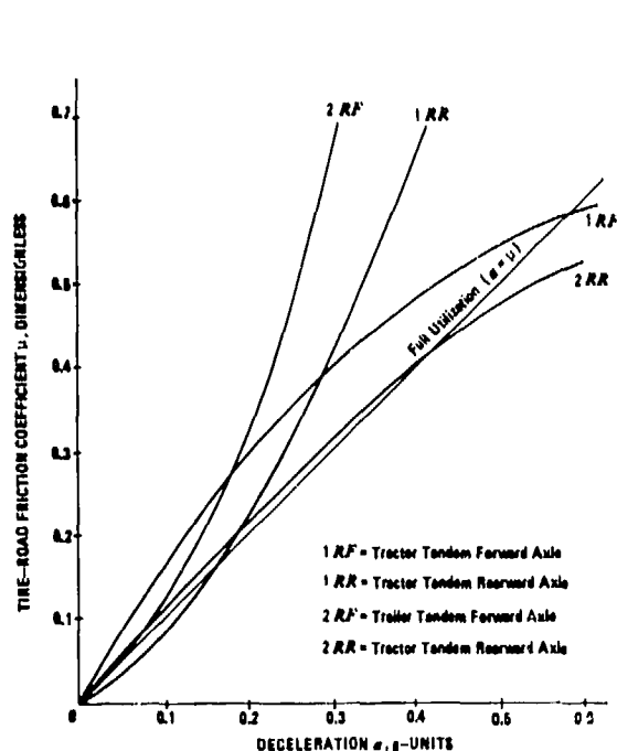
Figure 9-25. Tire-Road Friction Utilization for 3-S2 Tractor-Semitrailer (Empty) With Proportioning (No Front Brakes)
