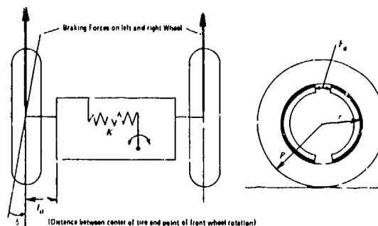
Figure 12-12. Steering Schematic
