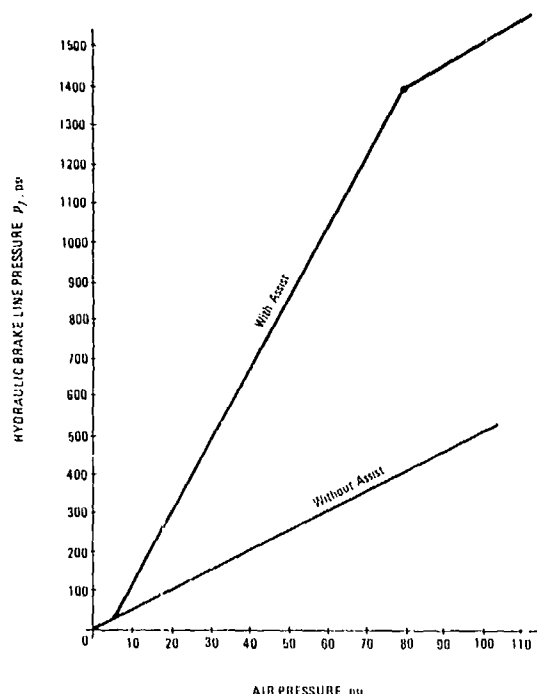
Figure 5-13. Air-Over-Hydraulic Brake Characteristic
