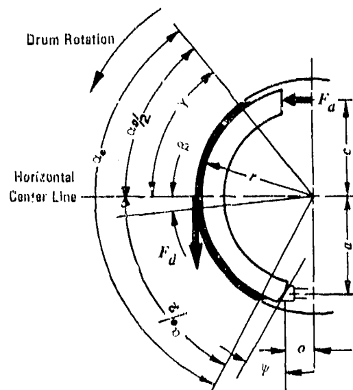
Figure 2-14. Leading Shoe With Inclined Abutment
