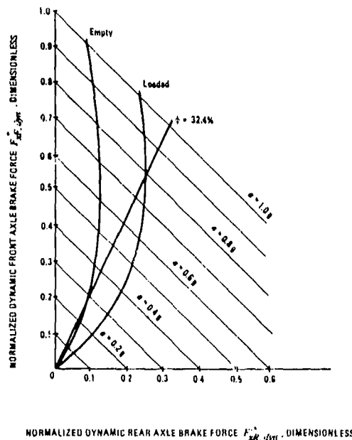
Figure 14-10. Normalized Dynamic and Actual Brake Forces, Vehicle No. 3
