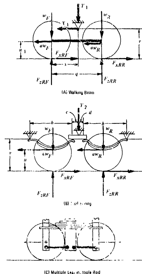
Figure 8-15. Tandem Axle Suspensions
