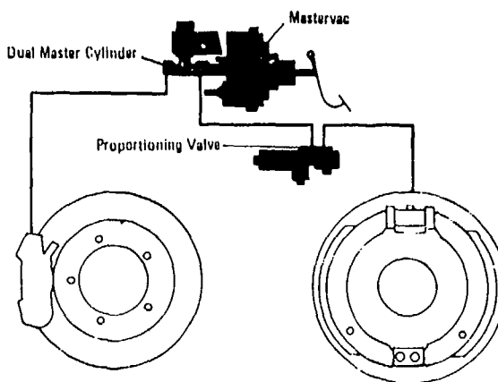
Figure 15-11. Dual Circuit Mastervac Brake System
