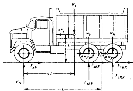
Figure 8-16. Forces Acting on a Tandem Axle Truck
