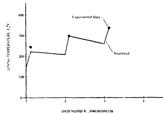
Figure 3-6. Brake Lining Temperature Attained in Fade Test
