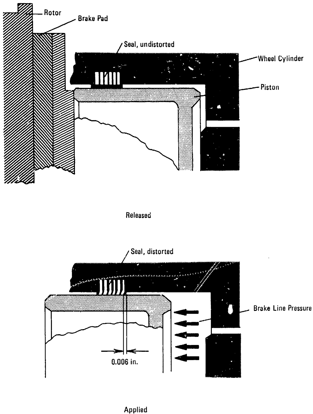
Figure 2-5. Disc Brake Clearance Adjustment
