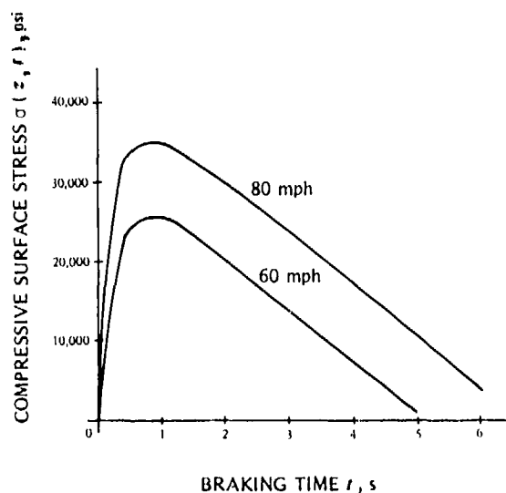
Figure 3-10. Thermal Stresses at the Surface Attained in Stops from 60 and 80 mph
