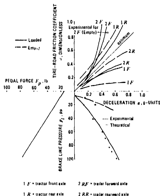
Figure 8-36. Braking Performance Diagram for a Tractor-Semitrailer Combination
