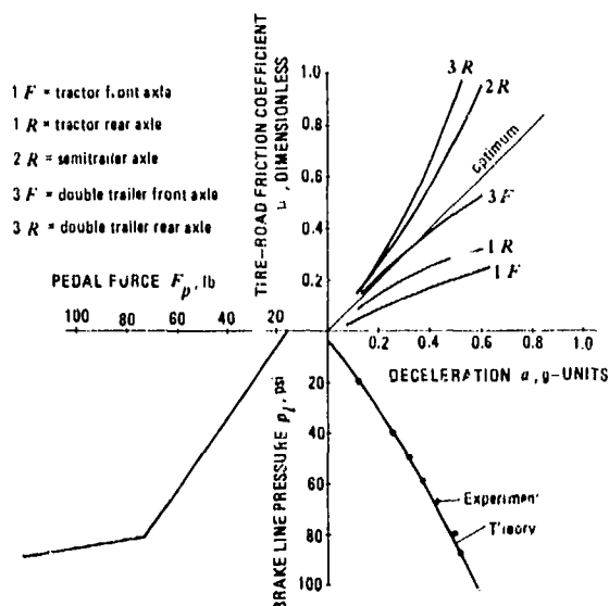
Figure 8-44. Braking Performance Diagram for a Tractor-Semitrailer-Double-Trailer Combination
