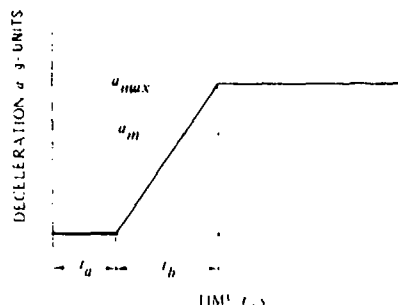
Figure 1-1. Idealized Deceleration Diagram
