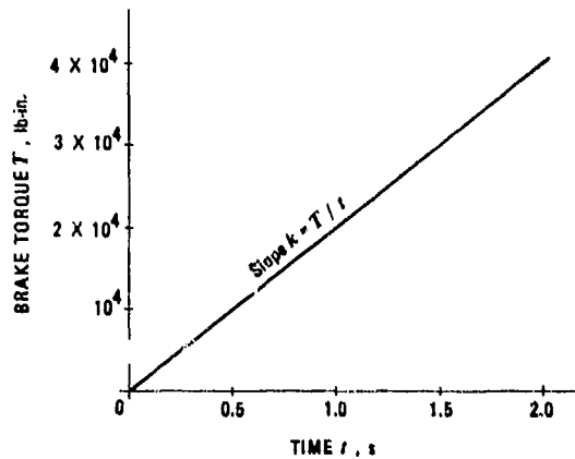
Figure 10-2. Brake Torque Rate — Induced by Driver
