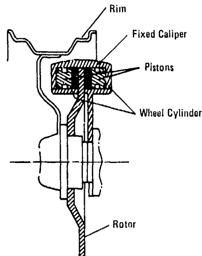
Opposing Piston-Fixed Caliper Brake
