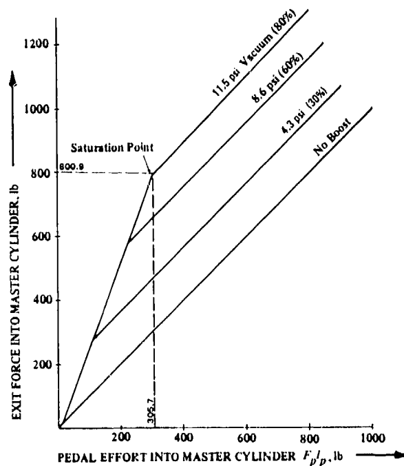
Figure 5-4. Mastervac Characteristics
