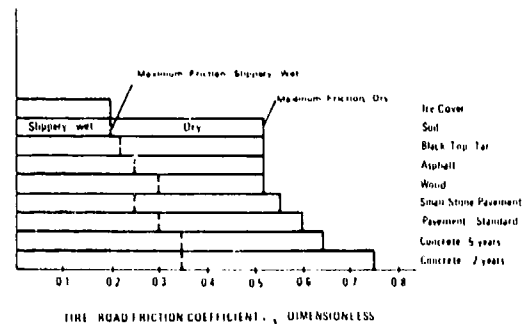
Figure 6-4. Typical Coefficient of Friction \mu_x Between Tire and Road for Truck Tire
