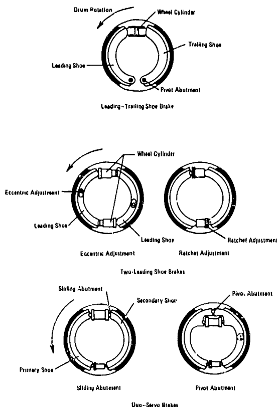
Figure 2-1. Basic Drum Brakes
