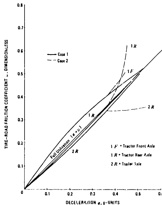
Figure 9-10. Tire-Road Friction Utilization, Cases 1 and 2, W_2 = 43,000 lb
