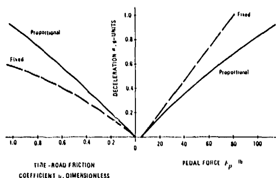
Figure 9-6. Pedal Force Required for Fixed and Variable Ratio Braking
