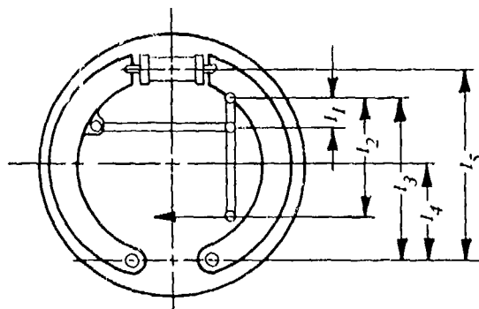
Figure 5-14. Schematic of Parking Brake
