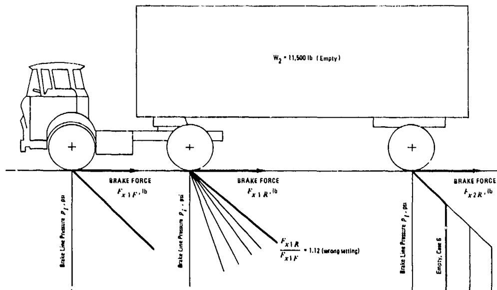
Figure 9-15. Schematic Brake Force Distribution, Case 6
