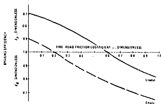
Figure 14-13. Braking Efficiency, Vehicle No. 1
