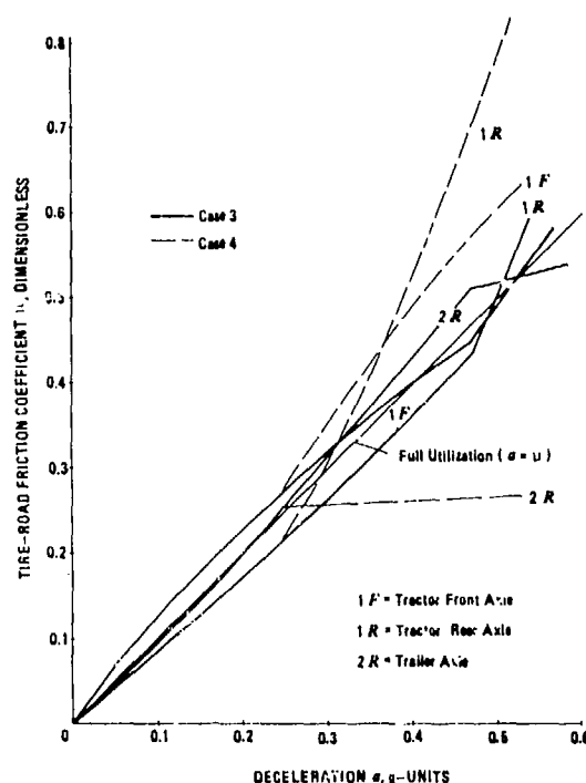
Figure 9-12. Tire-Road Friction Utilization, Cases 3 and 4, W_2 = 27,000 lb
