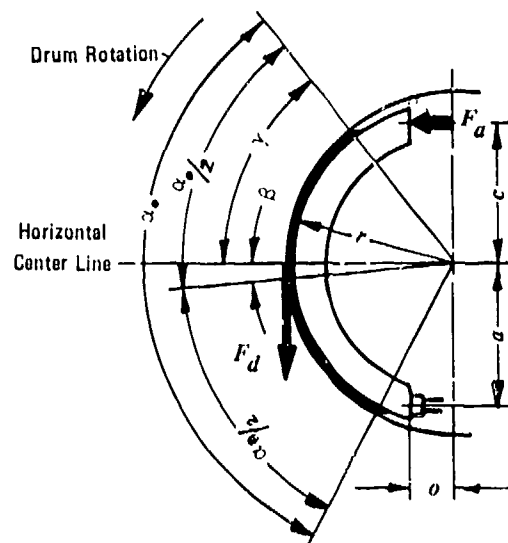
Figure 2-13. Leading Shoe With Parallel Sliding Abutment
