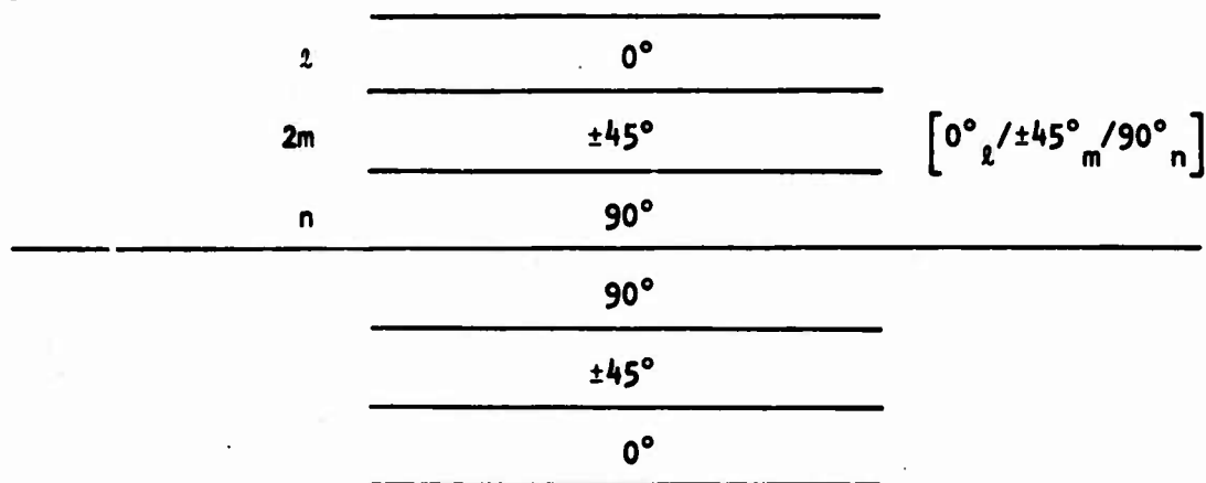
Figure 39. Laminate configuration.
