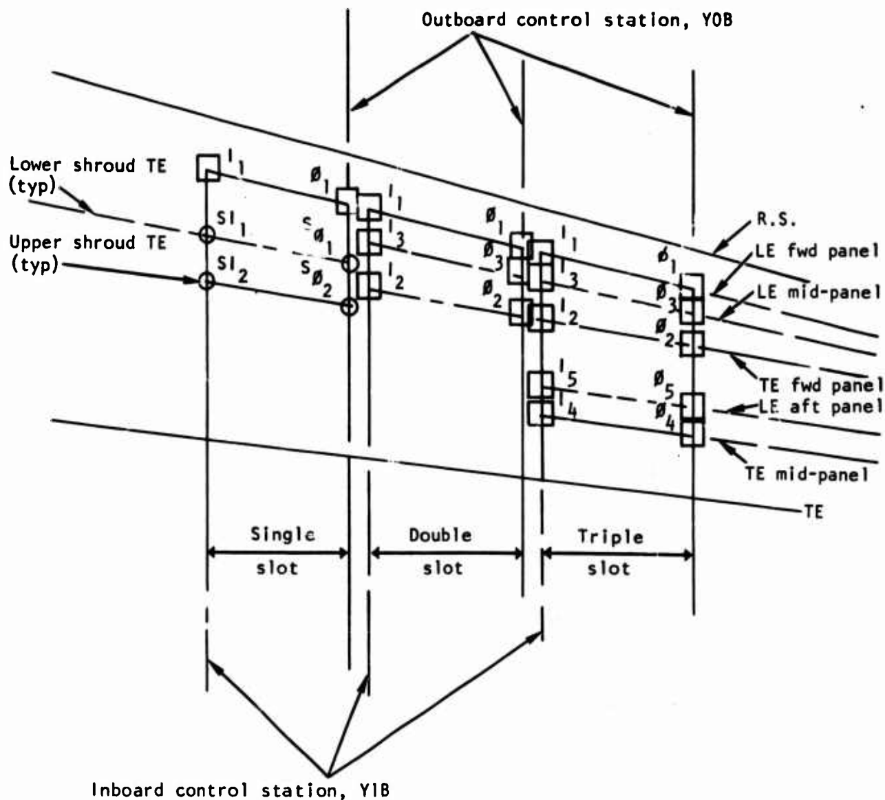
Schedule of required chordwise control point data
