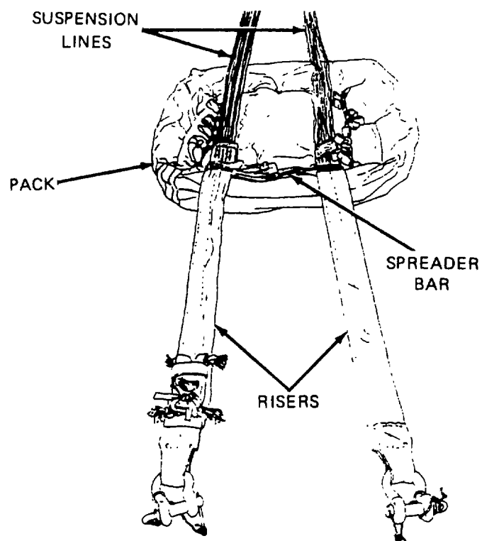
Figure 2-24. Suspension Line Stowage Preparation.
