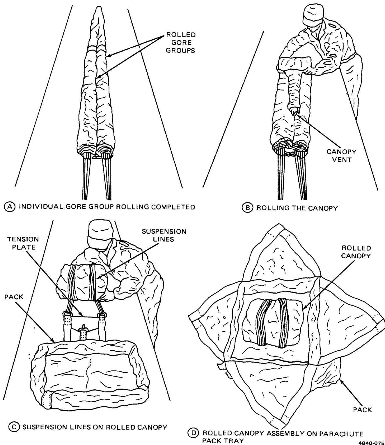
Figure 2-69. Rigger Rolling a Parachute Canopy Assembly.
