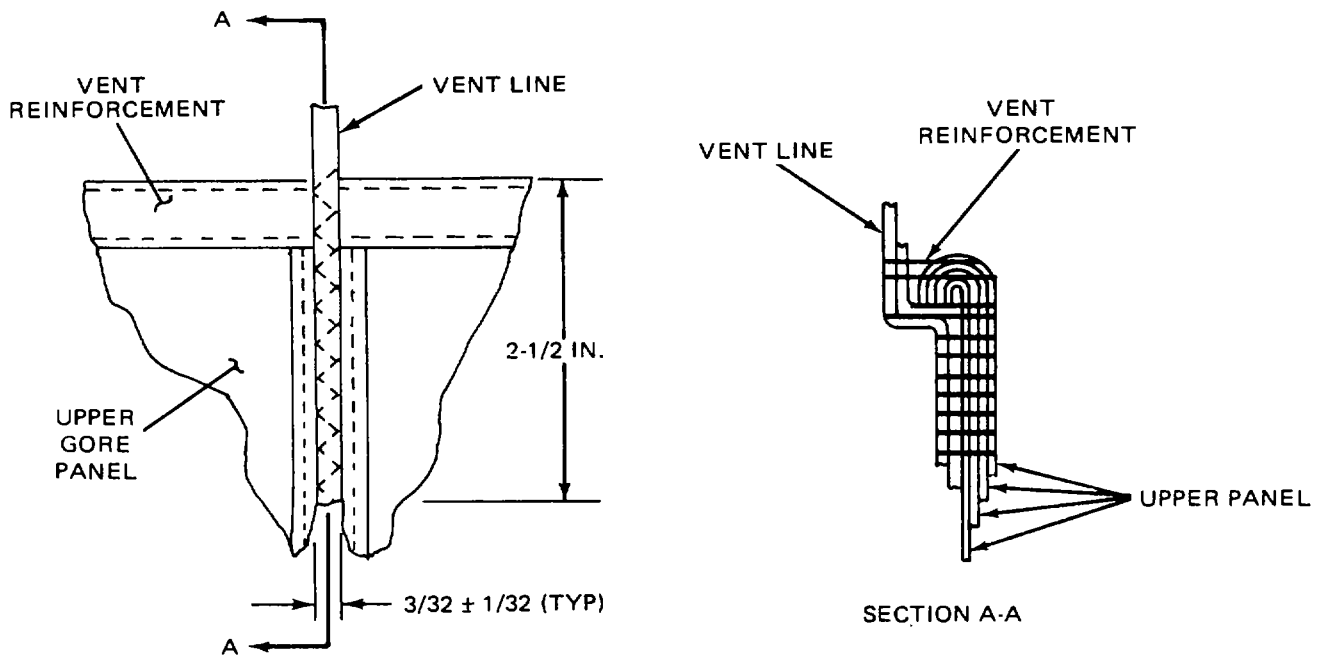
Figure 2-43. Vent Line Replacement Details.
