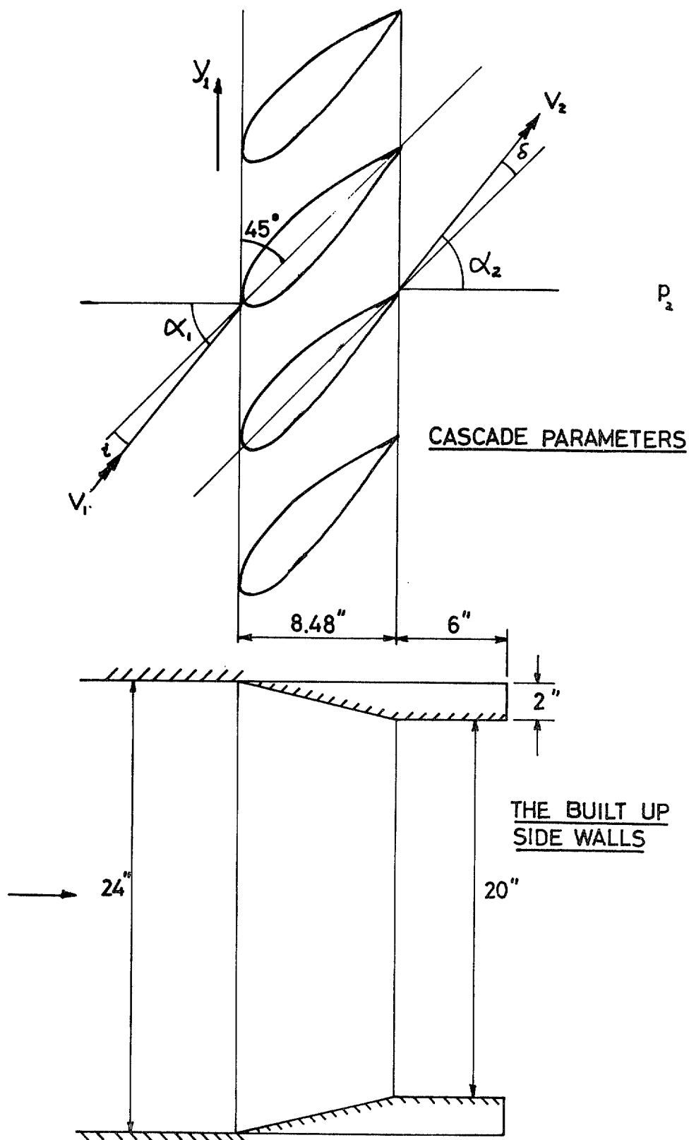
FIG. 8. Cascade geometry and nomenclature.
