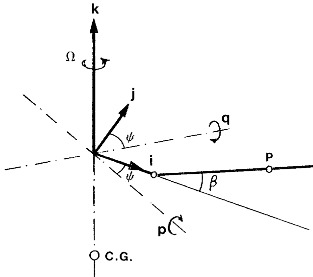
FIG. 2. Rotor coordinates.
