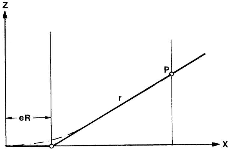
FIG. 1 Representation of hingeless blade.
