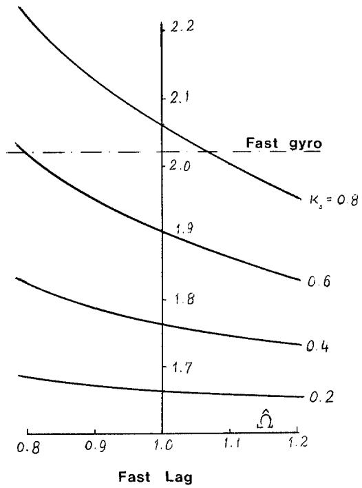
FIG. 6. Frequency ratios of lag modes.
