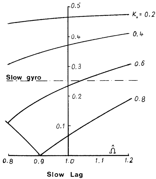
FIG. 6. Frequency ratios of lag modes.
