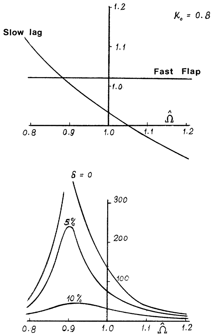
FIG. 12. Lag/flap ratios near resonance.
