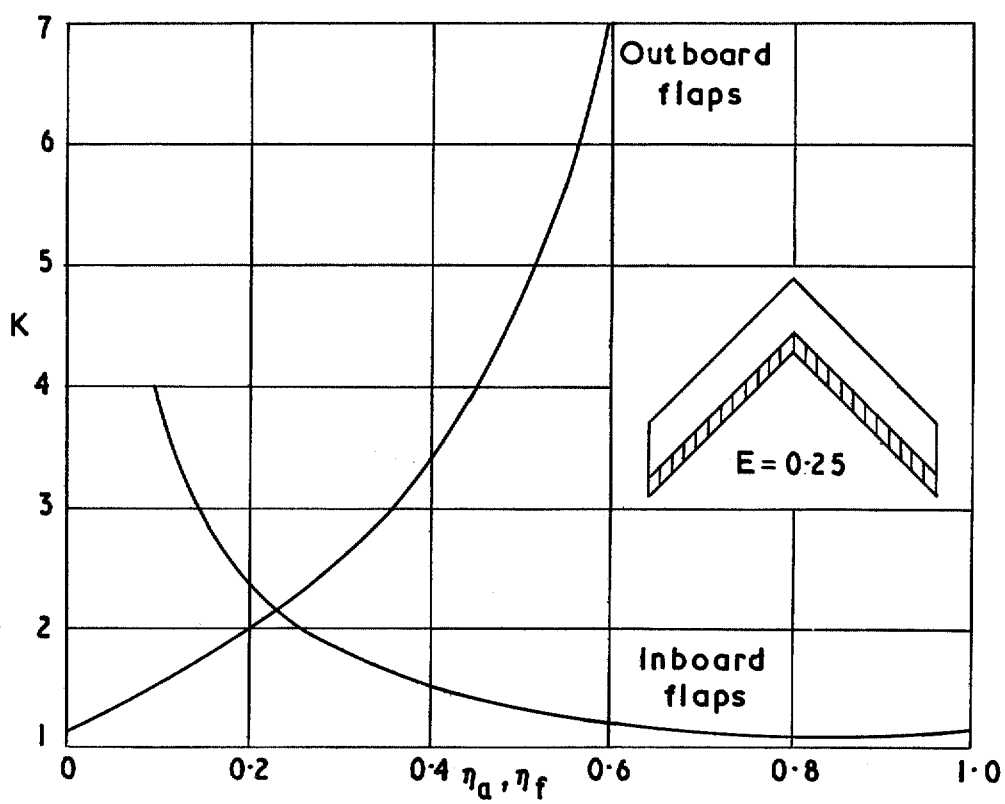
FIG. 3. Effects of flap span on vortex drag factor.
