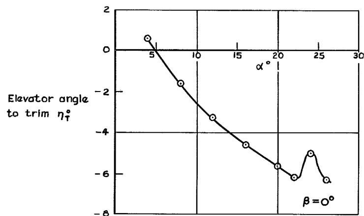
(b) \eta^\circ to trim v \alpha^\circ
