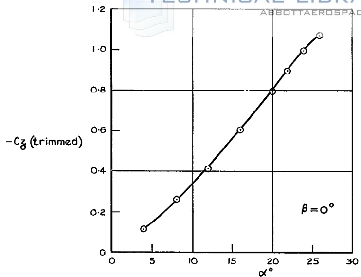
(a) -C_z(\text{trimmed}) v \alpha^\circ
