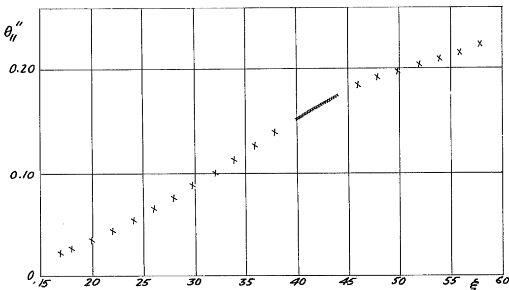
FIG. 7. Computer output for crossflow thickness calculation, Set 3.
