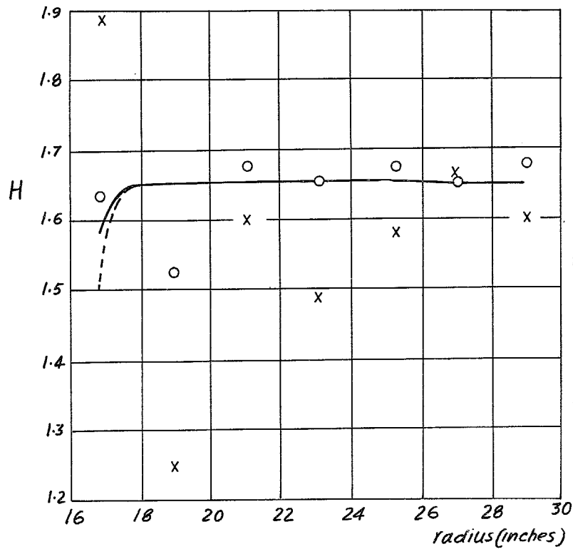
FIG. 12. Development of streamwise shape factor, Set 2.
