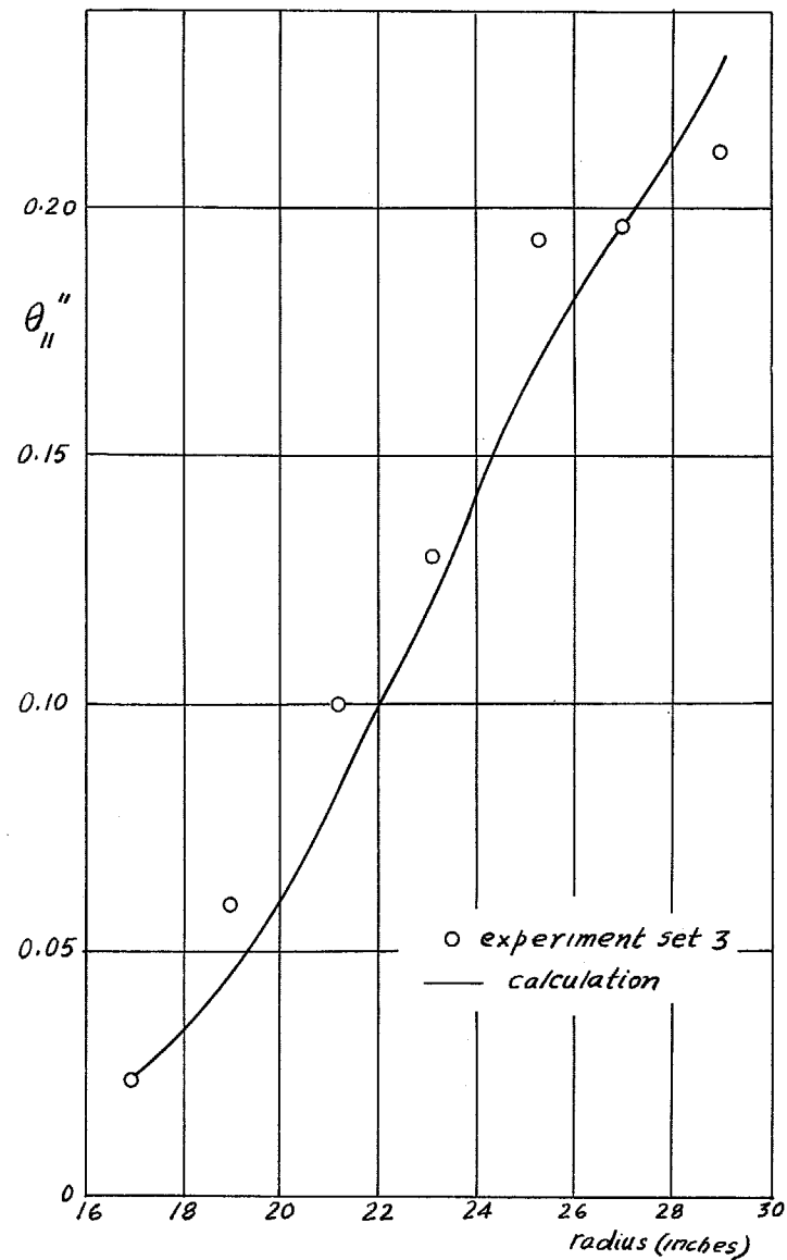
FIG. 8(b). Streamwise momentum thickness, Set 3.
