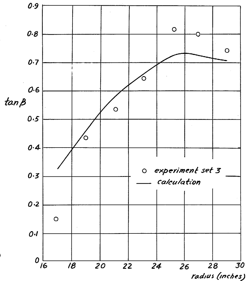
FIG. 15. Development of crossflow angle, Set 3.
