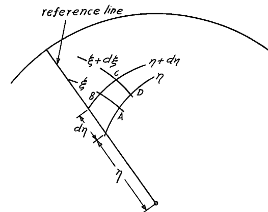
FIG. 2. Curvilinear co-ordinate system.
