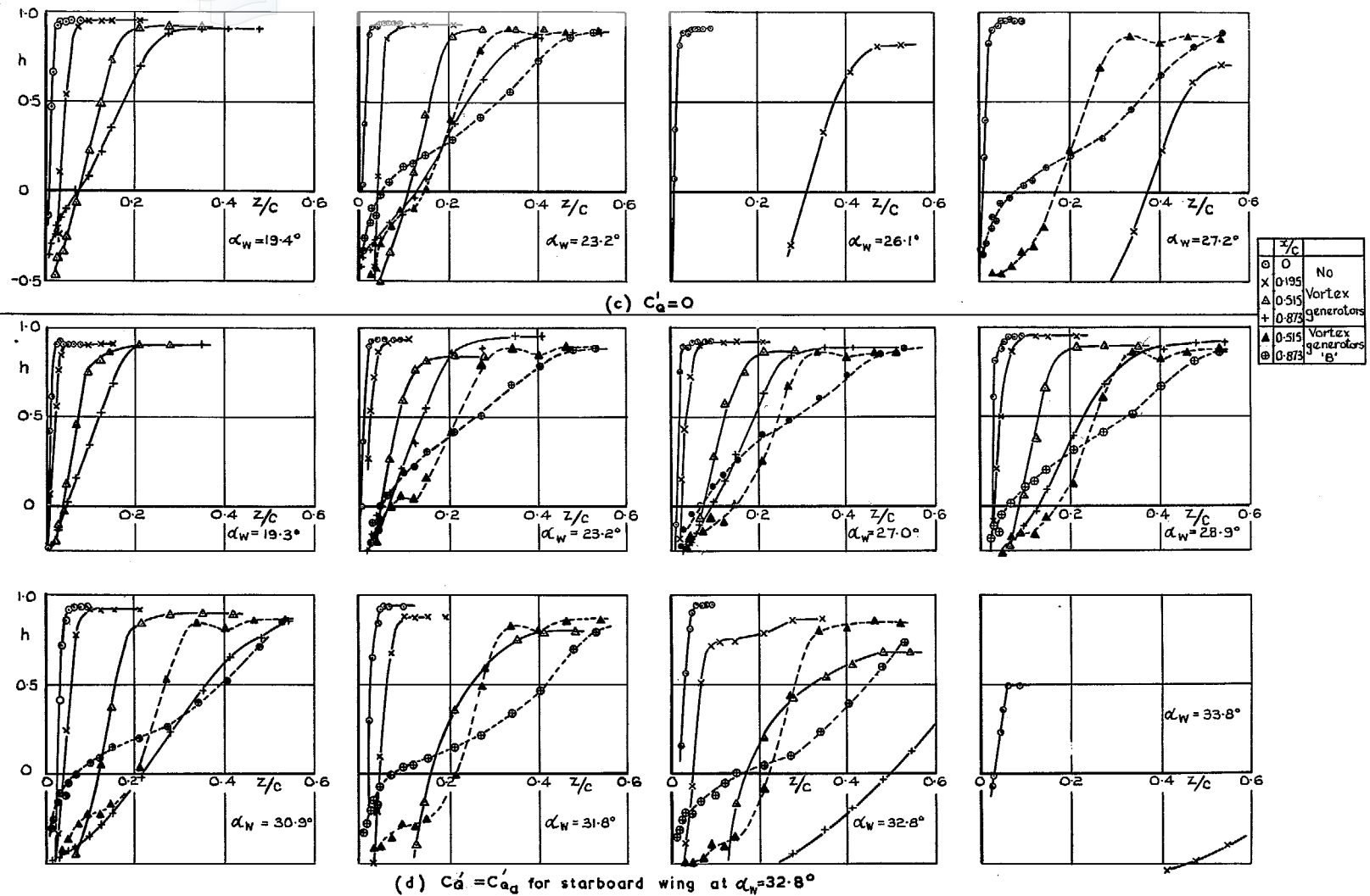
FIG. 26. The effect of distributed suction at knee of extending area L.E. flap on boundary-layer profiles. Starboard wing y = 0.656 h/2 , \delta_N = 31^\circ , \delta_R = 35^\circ , specimen G ( d = 0.026 in 1.75 per cent open area).
