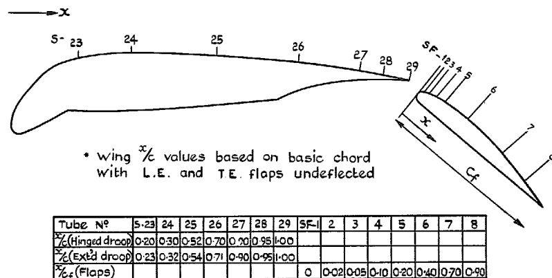
Fig. 6 Wing and T.E. flap static pressure details. 65.6% b/2 starboard wing only
