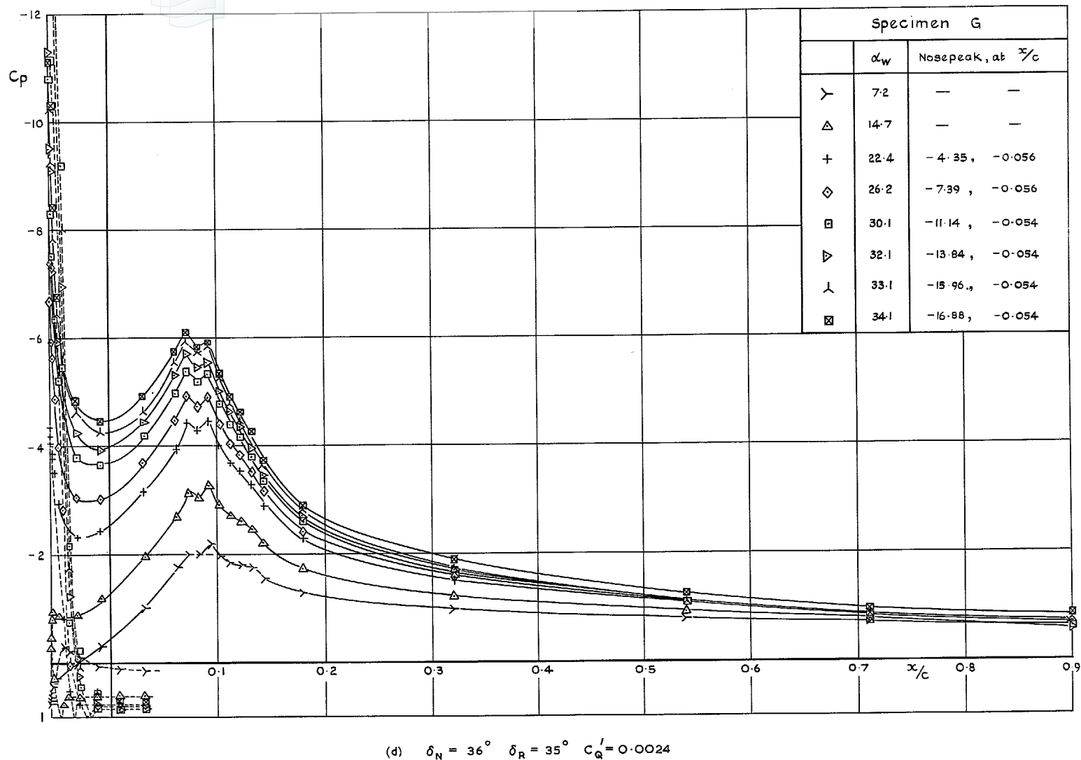
FIG. 25 (concl'd). The effect of distributed suction at knee of extending area L.E. flap on wing surface pressure distribution (0.656 b/2 , starboard wing).
