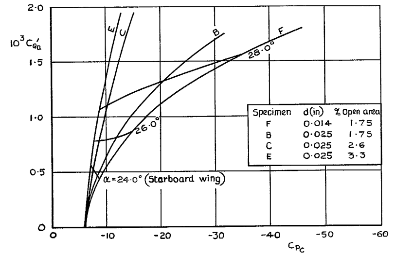
FIG. 22. The effect of open area ratio on C'_{Qa} vs C_{Pe} with distributed suction at knee of conventional L.E. flap. \delta_N = 32^\circ , \delta_R = 35^\circ .
