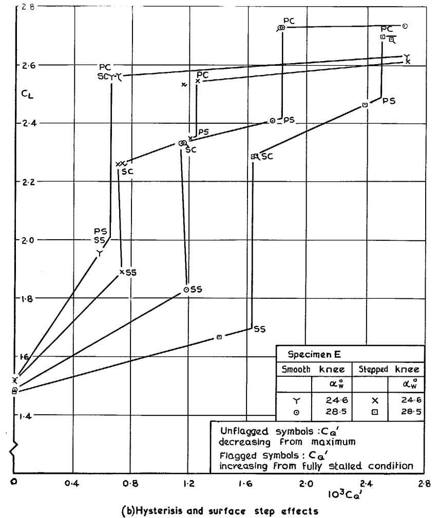
FIG. 14. Typical effects of distributed suction at knee of conventional L.E. flap on C_L and C_D at fixed incidence. \delta_N = 32^\circ . \delta_R = 35^\circ .
