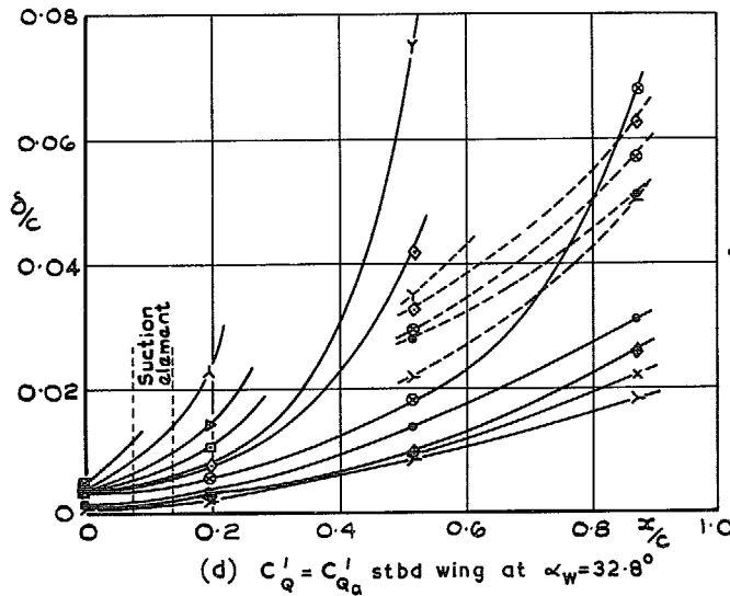
FIG. 27. The effect of distributed suction at knee of extending-area L.E. flap on boundary-layer thickness \delta_N = 31^\circ \delta_R = 35^\circ specimen G ( d = 0.026 in, 1.75 per cent open area).
