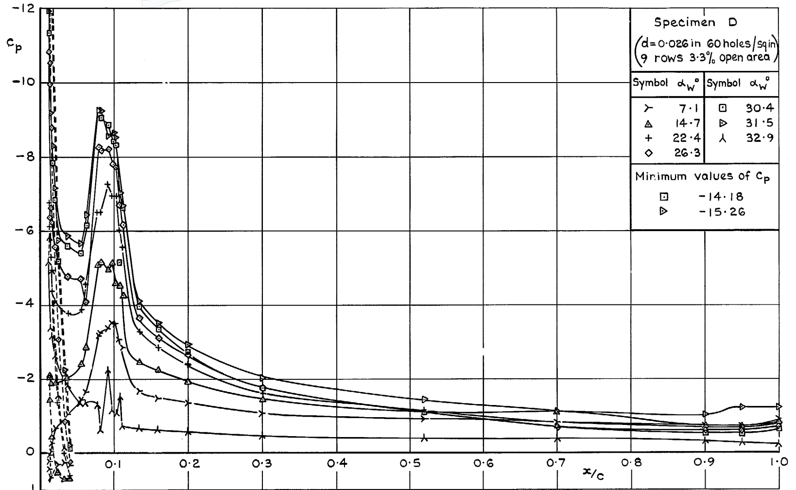
FIG. 16 (concl'd). The effect of distributed suction at knee of conventional L.E. flap on wing surface pressure distribution ( 0.656 b/2 , starboard wing).
