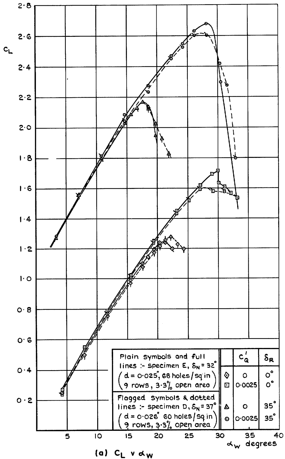
FIG. 13. The effect of distributed suction at knee of conventional L.E. flap on force and moment characteristics.
