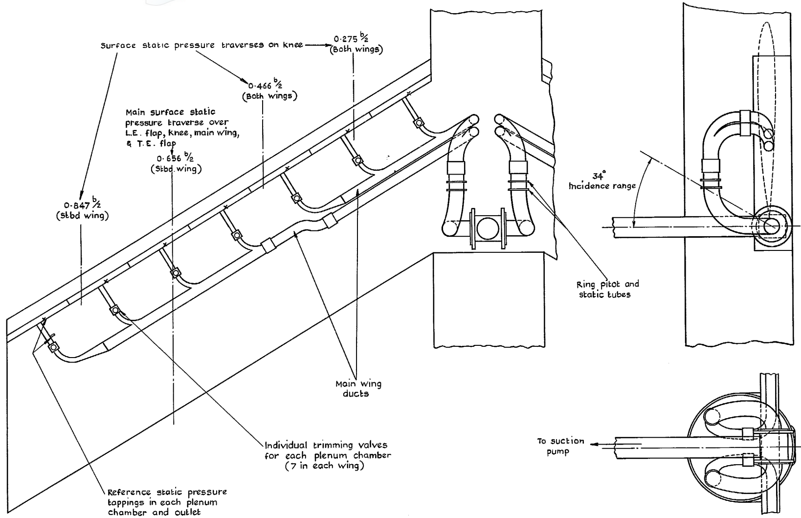
FIG. 3. Details of wing ducting and Instrumentation.
