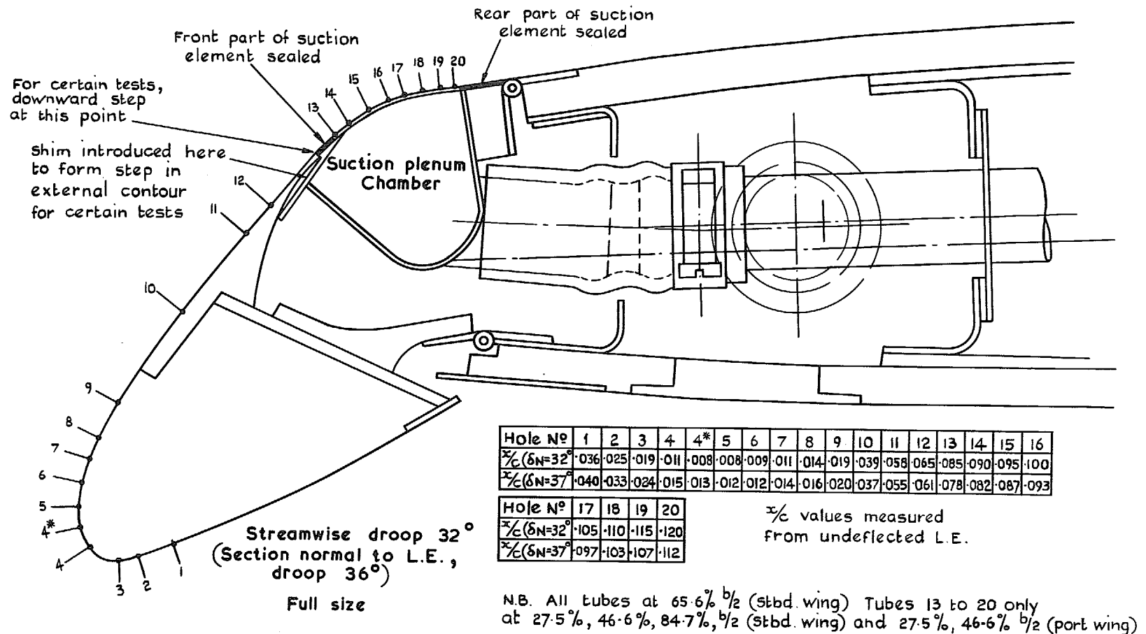
FIG. 4. Conventional L.E. flap arrangement.
