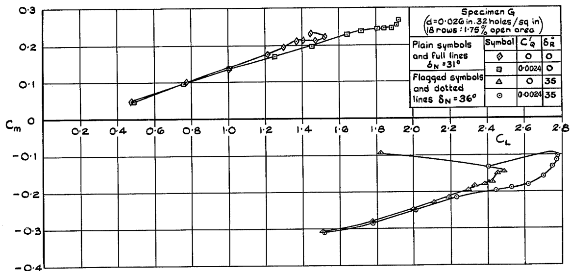
(c) C_m v C_L
