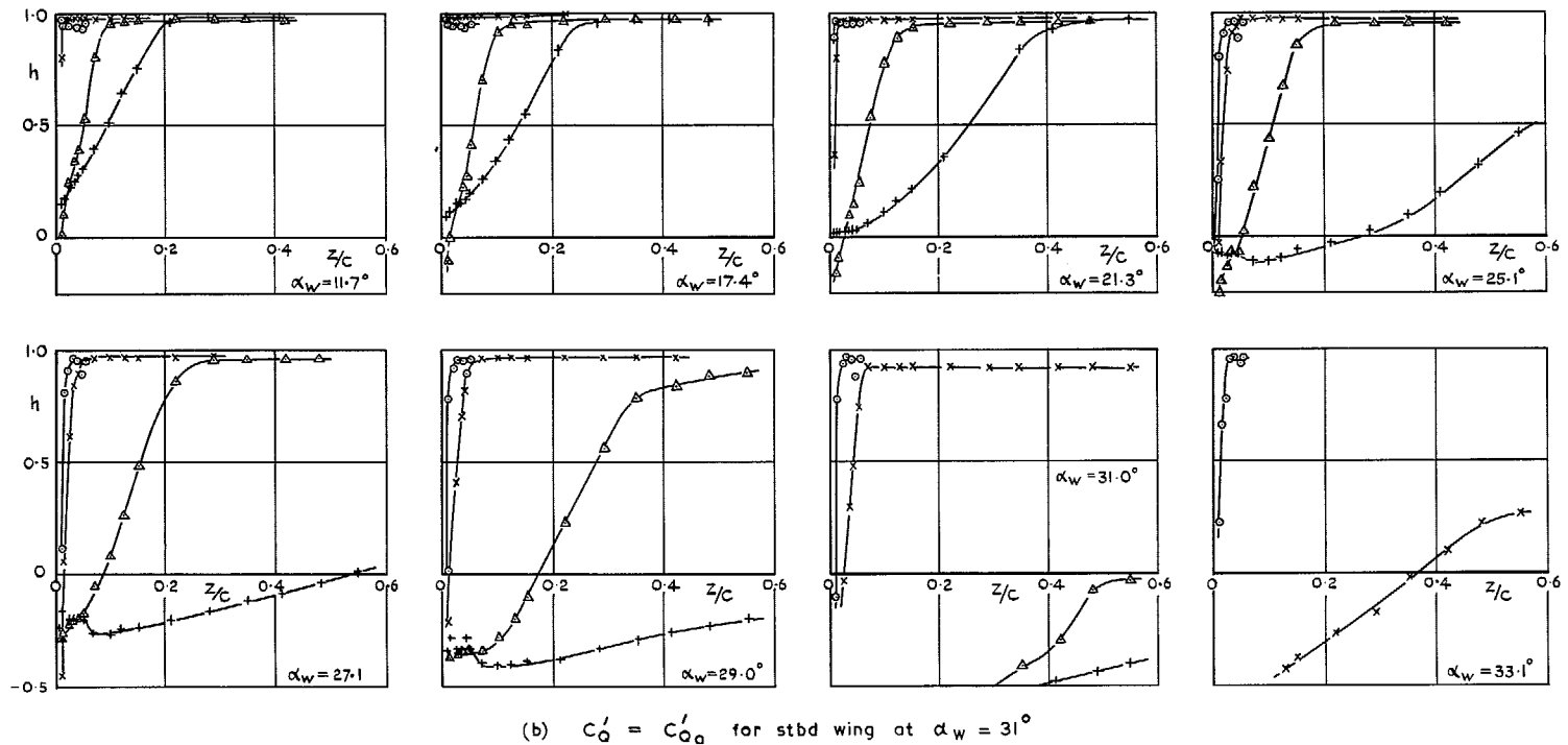
FIG. 18. The effect of distributed suction at knee of conventional L.E. flap on boundary layer profiles, starboard wing, y = 0.656 b/2 \delta_L = 32^\circ \delta_R = 0^\circ Specimen E ( d = 0.025 in, 3.3 per cent open area).
