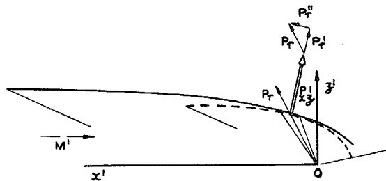
(b) COMPONENTS PARALLEL TO THE PLANE x'Oz'
