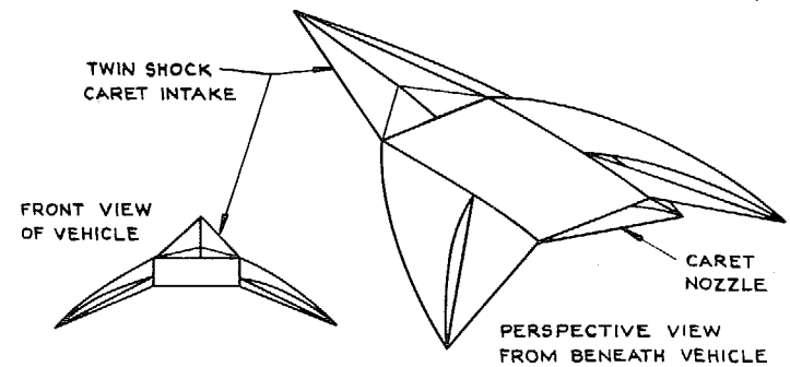
(b) VEHICLE CONFIGURATION
