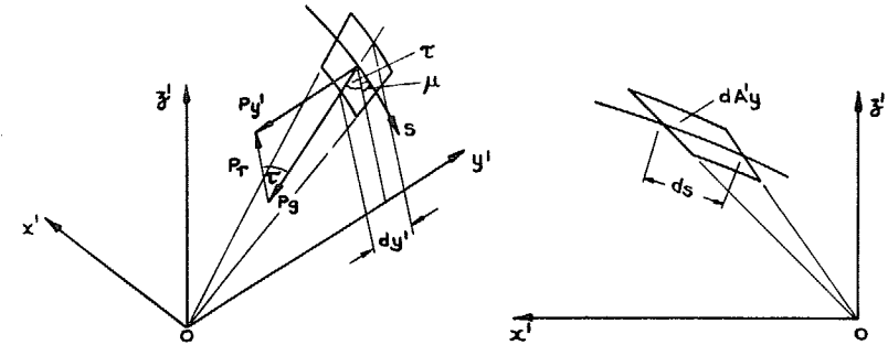
(c) LATERAL COMPONENTS OF AREA AND PRESSURE FORCE
