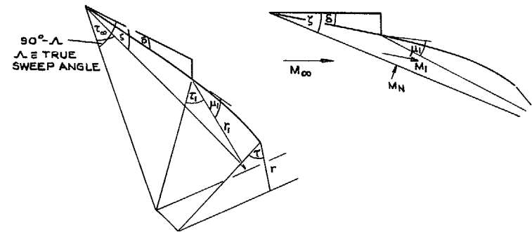
(e) GEOMETRY OF WEDGE-SPAR-PLUS-SAIL
