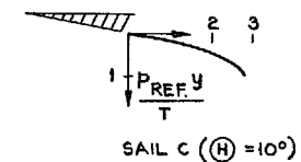
(c) TYPICAL SAIL PROFILES
