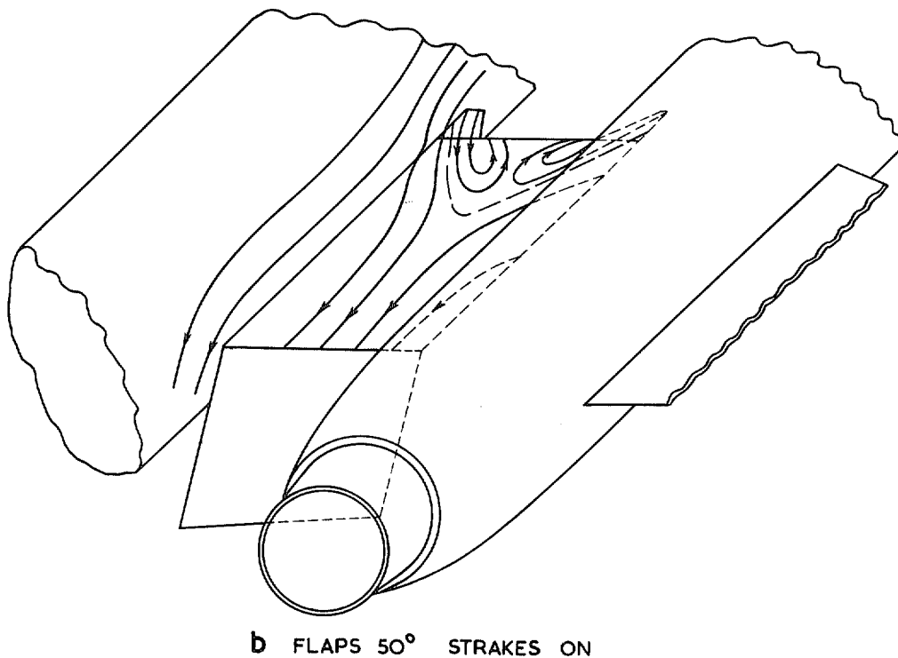
FIG. 4 a and b. Surface flow patterns on inner wing, \alpha = 8^\circ approx.
