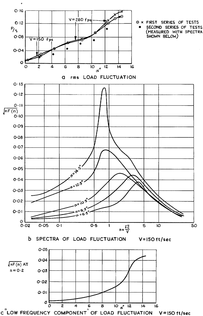
FIG. 16 a - c. Local load fluctuations at 0.5c on inner wing. Flaps 50^\circ , strakes on.
