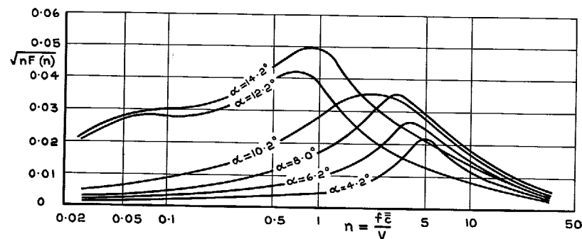
b SPECTRA OF LOAD FLUCTUATION V=150 ft/sec
