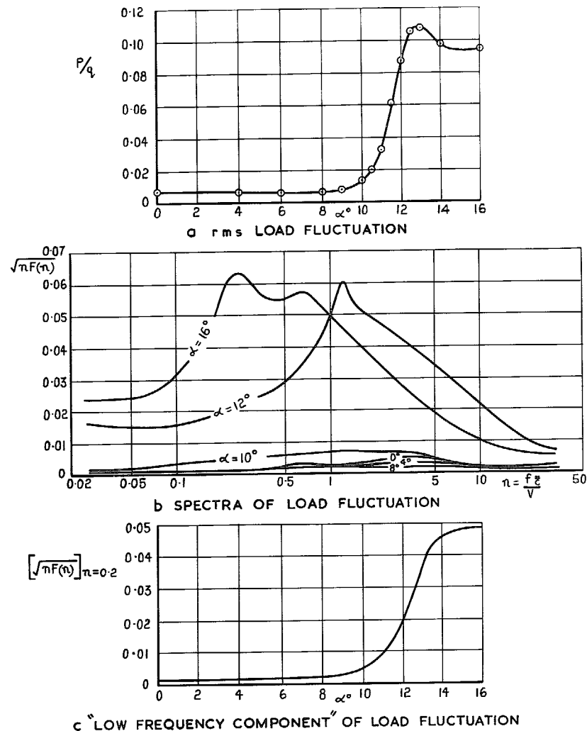
FIG. 20a-c. Local load fluctuations at position "C" on outer wing. Flaps 50^\circ , strakes on, V = 150 ft/sec.
