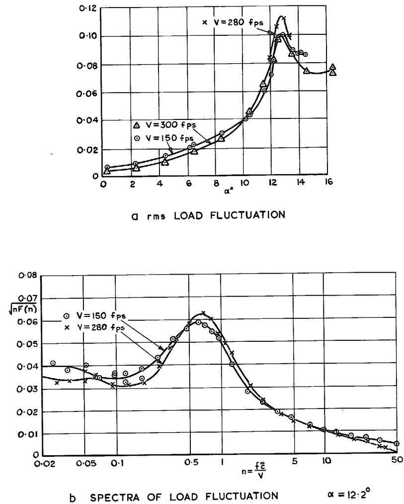
FIG. 15a and b. Effect of wind speed on local load fluctuations at 0.85c on inner wing. Flaps 0^\circ , strakes on.
