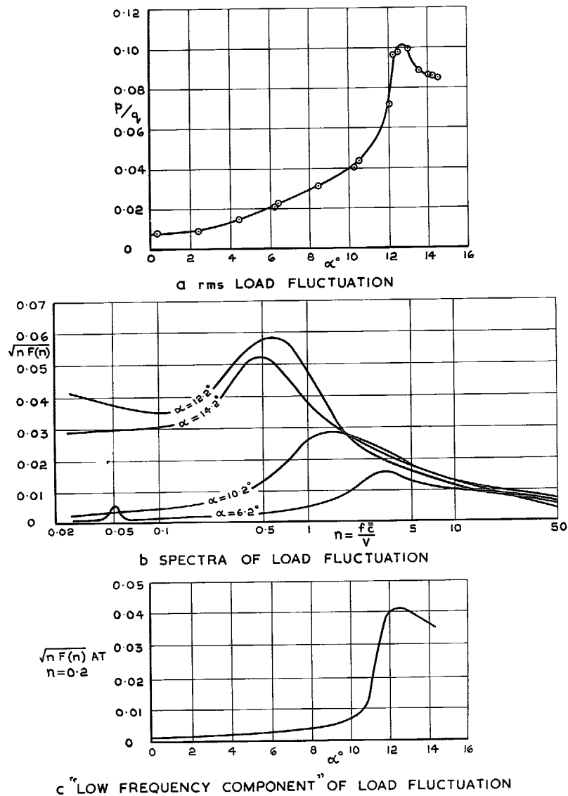
FIG. 14a - c. Local load fluctuations at 0.85c on inner wing. Flaps 0^\circ , strakes on, V = 150 ft/sec.
