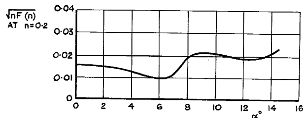
c "LOW FREQUENCY COMPONENT" OF LOAD FLUCTUATION
