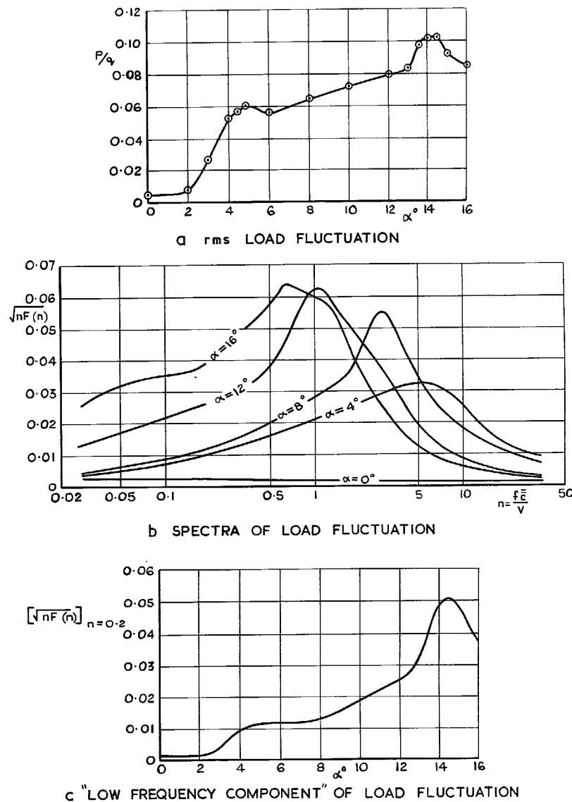
FIG. 19a-c. Local load fluctuations at position "B" on outer wing. Flaps 50^\circ , strakes on, V = 150 ft/sec.
