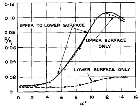
a rms PRESSURE FLUCTUATION
