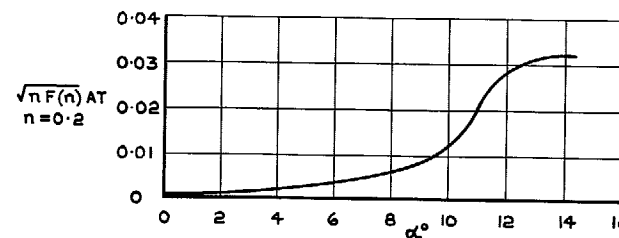
c "LOW FREQUENCY COMPONENT" OF LOAD FLUCTUATION V=150 ft/sec
