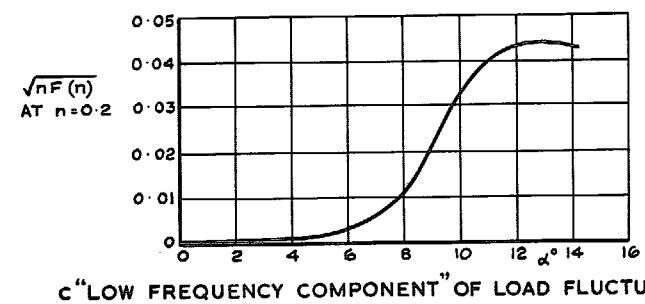
FIG. 8 a - c. Local load fluctuations at 0.85c on inner wing. Flaps 0°, no strakes, V = 150 ft/sec.
