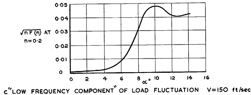
FIG. 7 a - c. Local load fluctuations at 0.5c on inner wing. Flaps 0°, no strakes.
