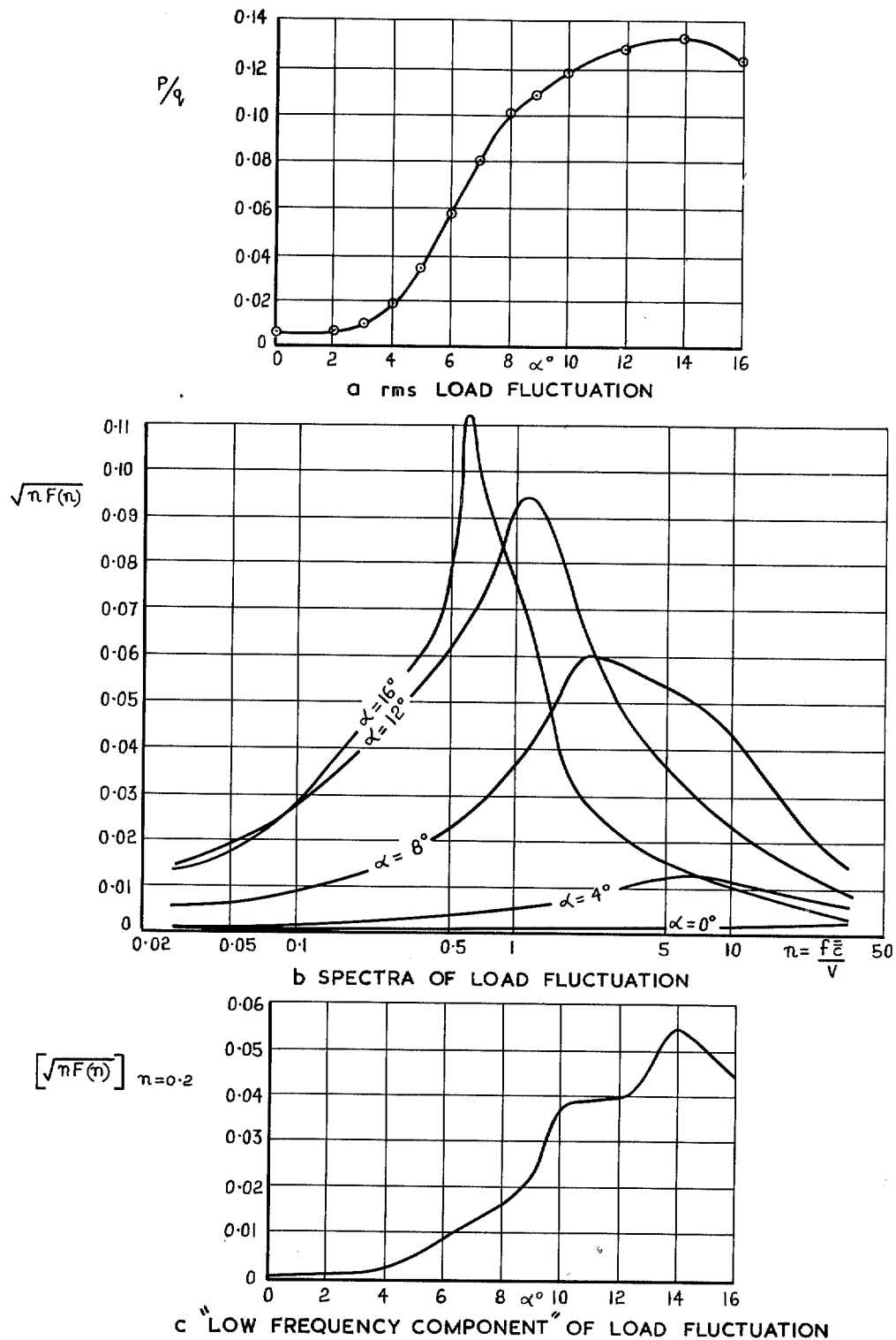
FIG. 21 a-c. Local load fluctuations at position "D" on outer wing. Flaps 50°, strakes on, V = 150 ft/sec.
