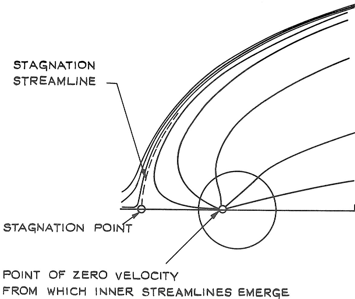
FIG. 5. Flow with stagnation point, \phi_{2a} or \phi_{2b} of Section 5.1.
