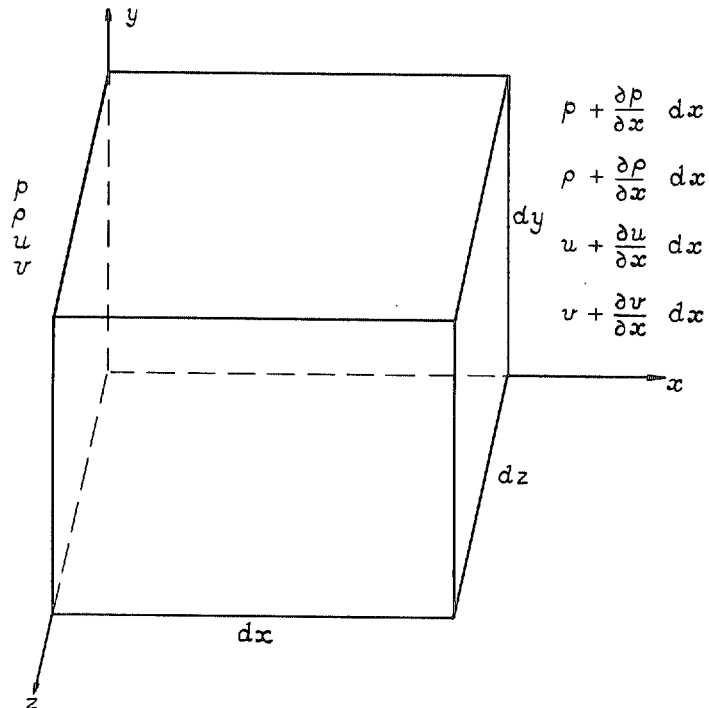
FIG. 2. Conservation diagram.
