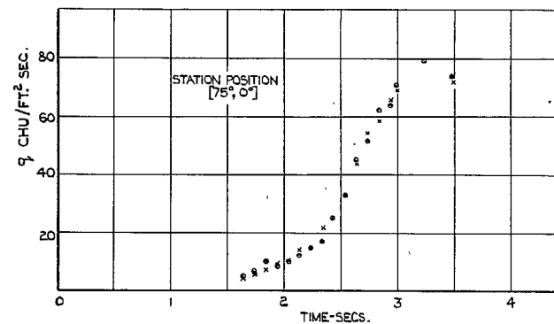
FIG. 20d (contd.). Local heat-transfer histories for head 8—stations [75^\circ, 0^\circ] , [90^\circ, 0^\circ] and [1.45D, 0^\circ] .
