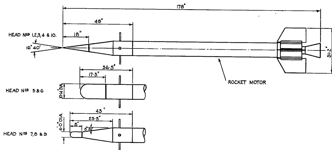
FIG. 1. Sketch of test vehicles.
