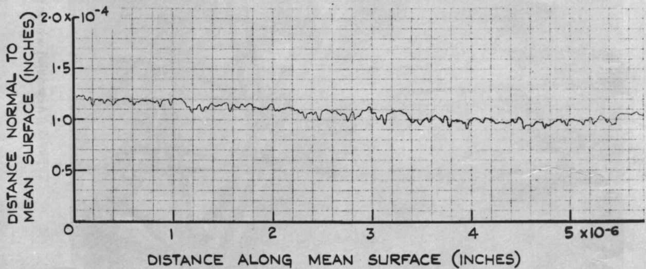
SMOOTH 10 inch HEMISPHERICAL HEAD (5) (C.L.A. \div 3.5 \times 10^{-6} inches)
