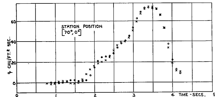
FIG. 20b (contd.). Local heat-transfer histories for head 5—stations [70^\circ, 0^\circ] , [90^\circ, 0^\circ] & [1.45D, 0^\circ] .
