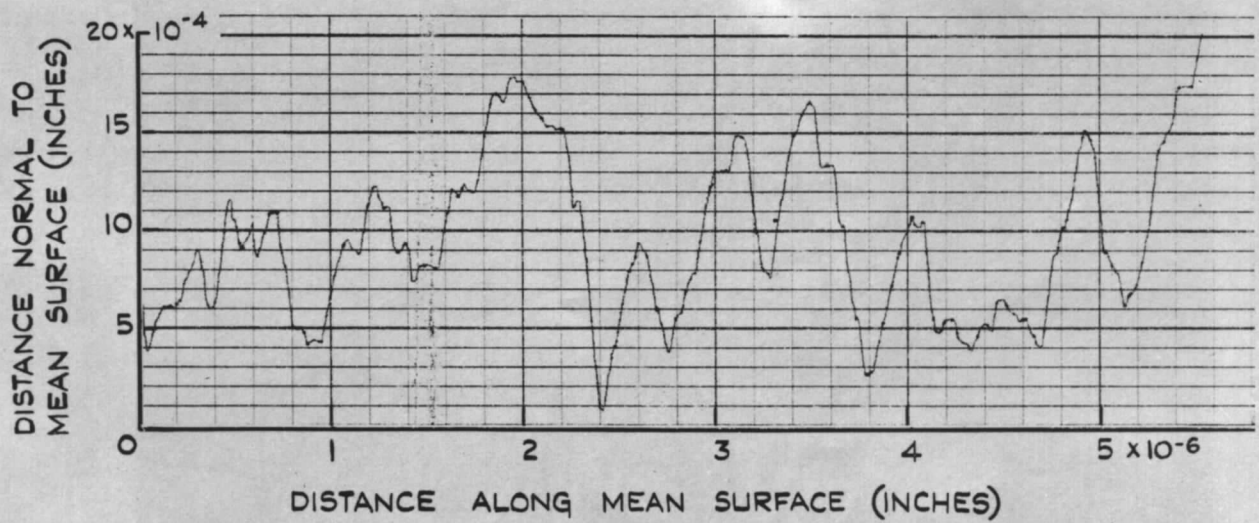
ROUGH 10 inch HEMISPHERICAL HEAD (6) (C.L.A. \div 200 \times 10^{-6} inches)
