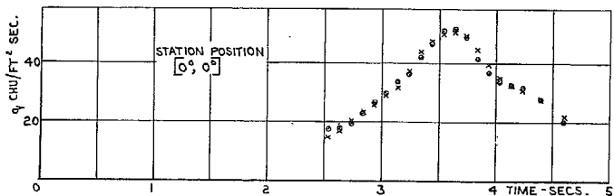
FIG. 20c. Local heat-transfer histories for head 6-stations [0^\circ, 0^\circ] & [30^\circ, 0^\circ] .
