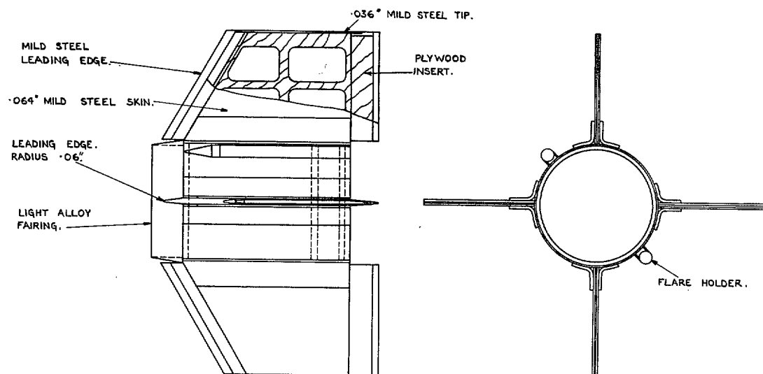
FIG. 2. Fin assembly.
