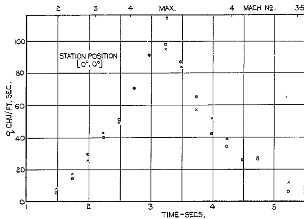
FIG. 20e. Local heat-transfer histories for head 9 - station [0^\circ, 0^\circ] .
