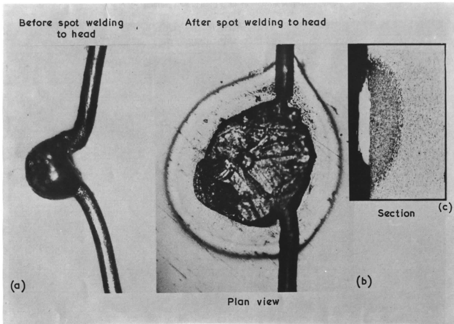
FIG. 7. Thermocouple weld (magnifications \times 100 ).
