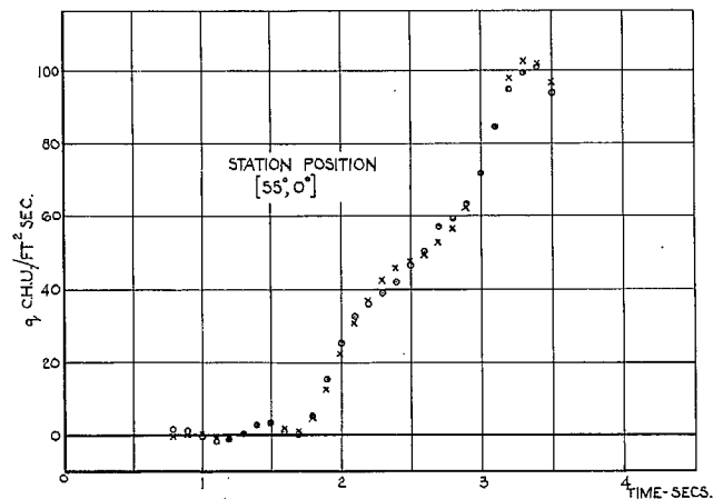
FIG. 20b (contd.). Local heat-transfer histories for head 5—stations [55^\circ, 0^\circ] and [60^\circ, 0^\circ] .
