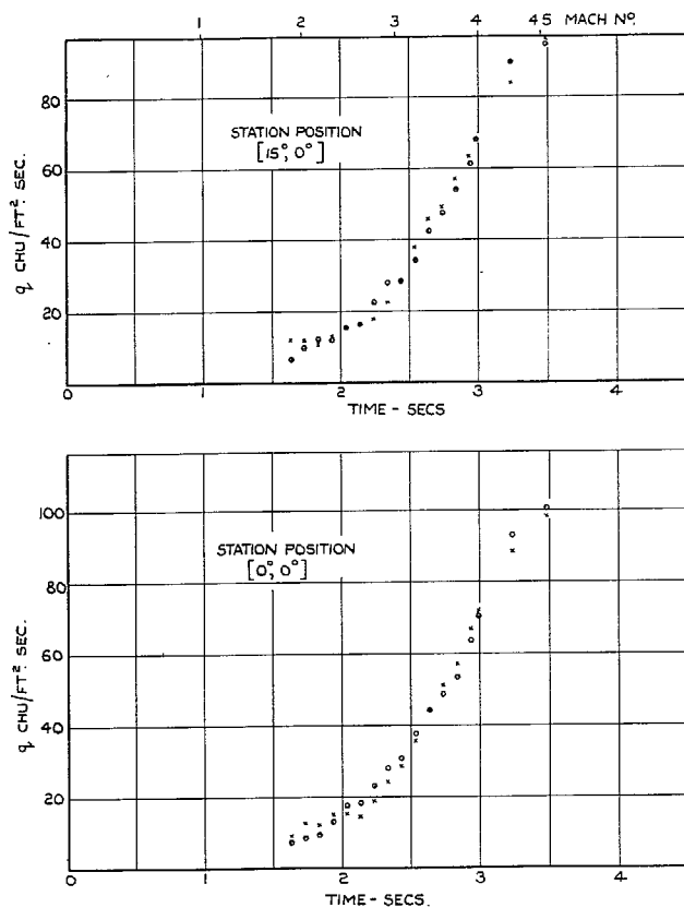
FIG. 20d. Local heat-transfer histories for head 8-stations [0°, 0°] and [15°, 0°].
