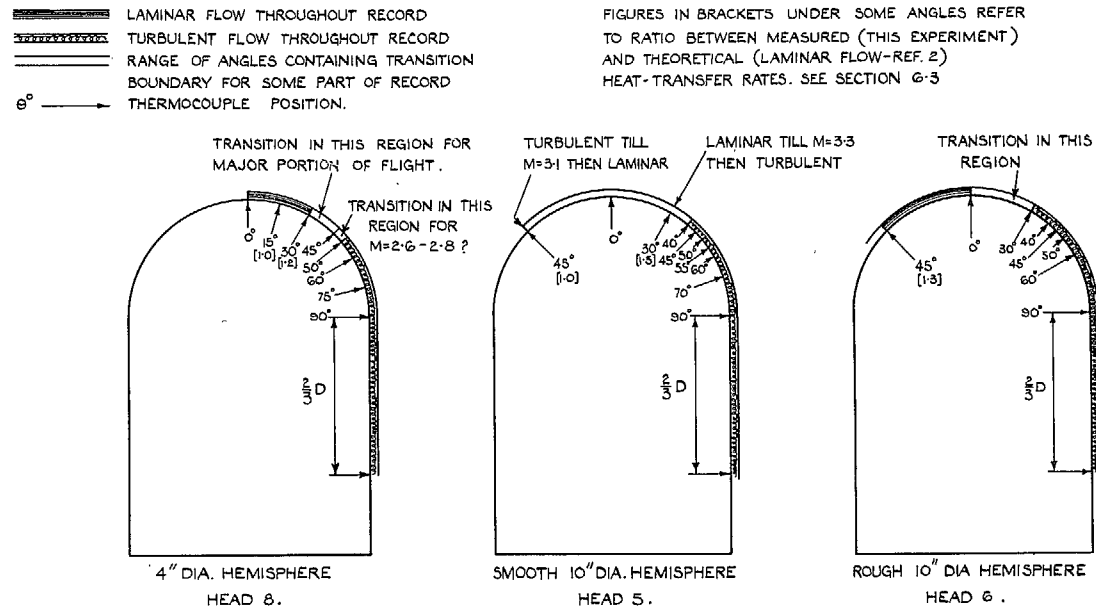
FIG. 27. Flow regimes on hemispherical heads.
