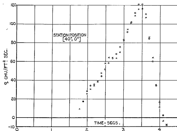
FIG. 20b (contd.). Local heat-transfer histories for head 5—stations [40°, 0°] and [50°, 0°].
