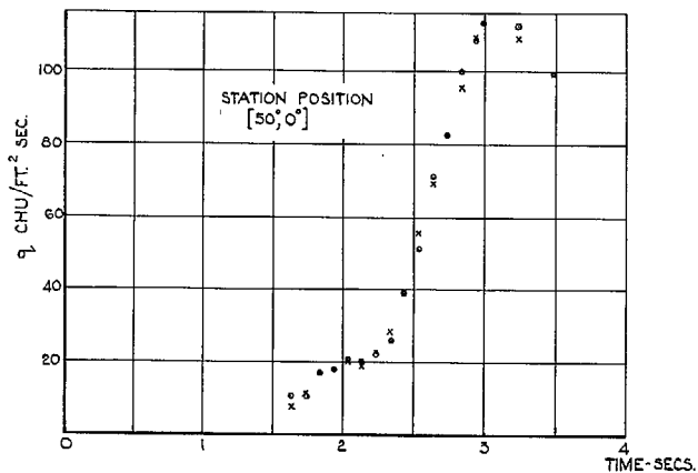
FIG. 20d (contd.). Local heat-transfer histories for head 8—stations [50^\circ, 0^\circ] and [60^\circ, 0^\circ] .
