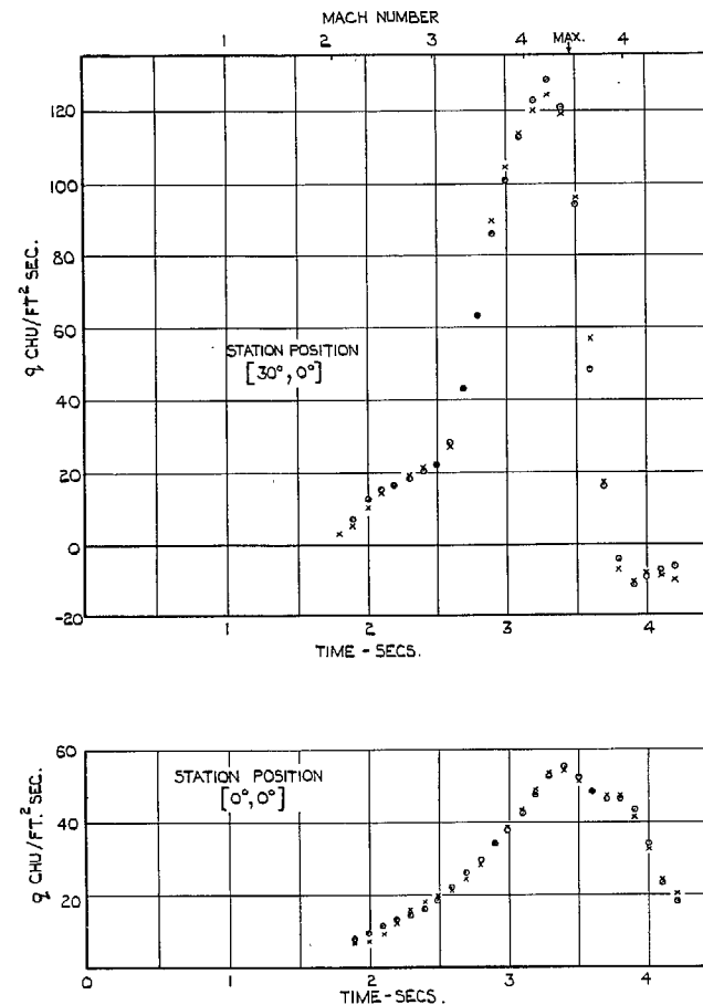
FIG. 20b. Local heat-transfer histories for head 5—stations [0°, 0°] and [30°, 0°].
