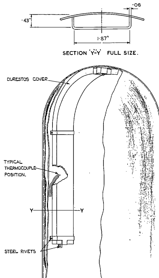
FIG. 9. Insulating durestos covers on 10 in. hemispheres.
