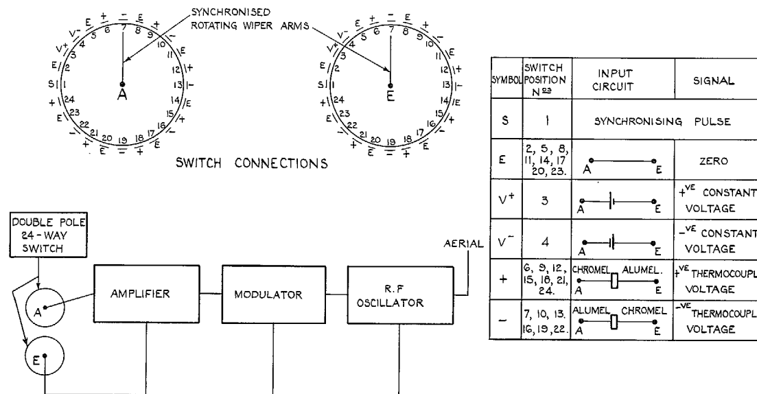
FIG. 12. Block diagram of telemetry equipment.
