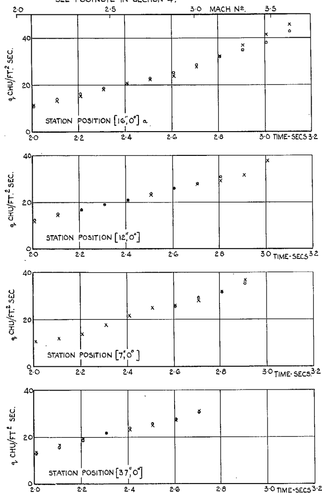
FIG. 20a(contd.). Local heat-transfer-rate histories for conical head 3.
