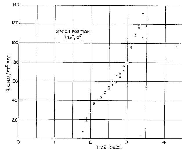
FIG. 20b (contd.). Local heat-transfer histories for head 5—stations [45°, 0°] and [45°, 180°].
