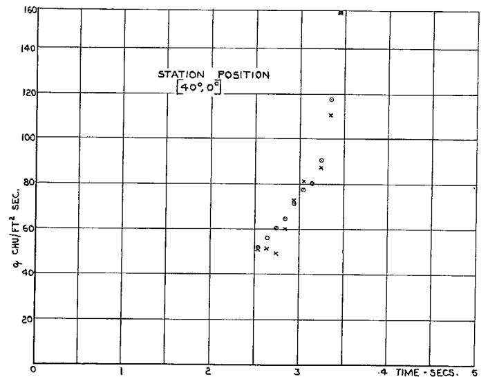
FIG. 20c (contd.). Local heat-transfer histories for head 6-stations [40^\circ, 0^\circ] & [50^\circ, 0^\circ] .
