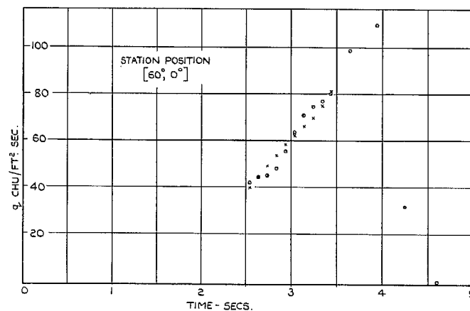
FIG. 20c (contd.). Local heat-transfer histories for head 6—stations [60^\circ, 0^\circ] , [90^\circ, 0^\circ] and [1.45D, 0^\circ] .
