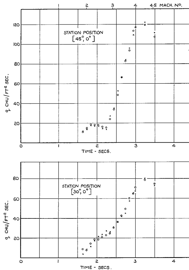
FIG. 20d (contd.). Local heat-transfer histories for head 8-stations [30°, 0°] and [45°, 0°].
