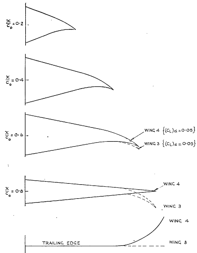
FIG. 4. Details of wing cross-sections: wings 3 and 4.
