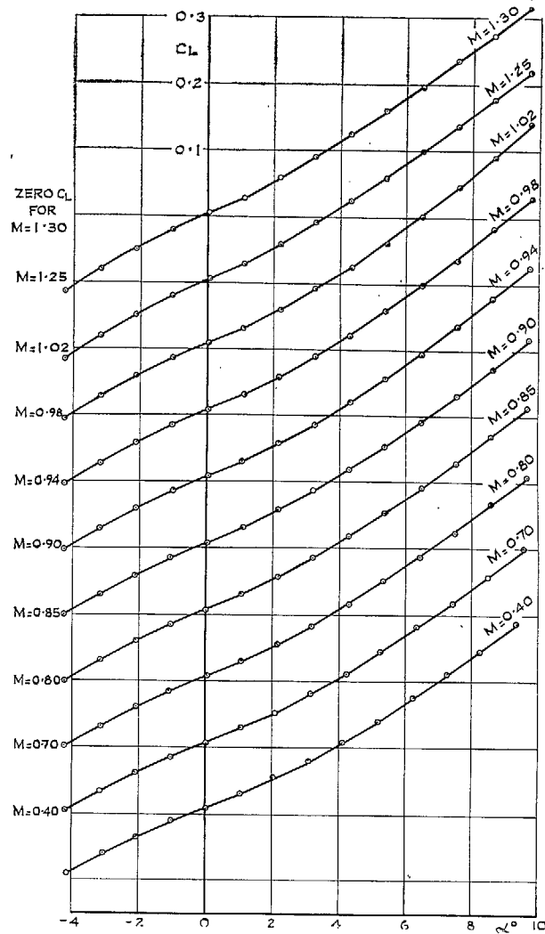
FIG. 12. Variation of C_L with \alpha : Wing 1.
