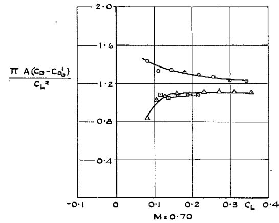
FIGS. 27a and b. Variation with C_L of the lift-dependent drag factor: wings 1, 2 and 3.
