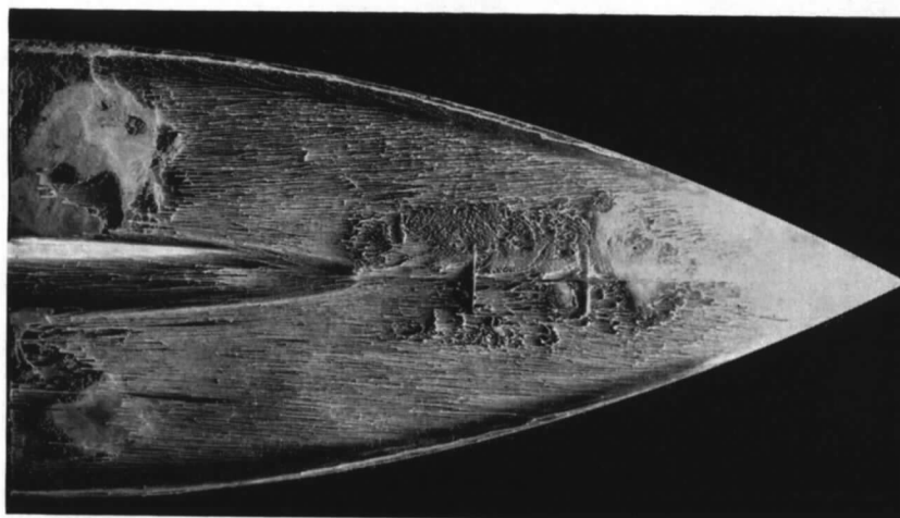
FIG. 11a. Oil-flow photographs. Wing 1. \alpha \div 2^\circ .
