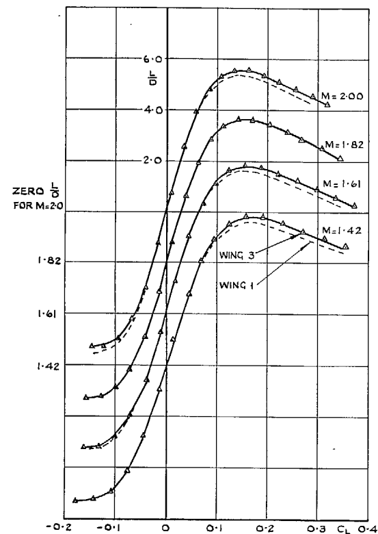
FIG. 8. Variation of L/D with C_L : wings 1 and 3.
