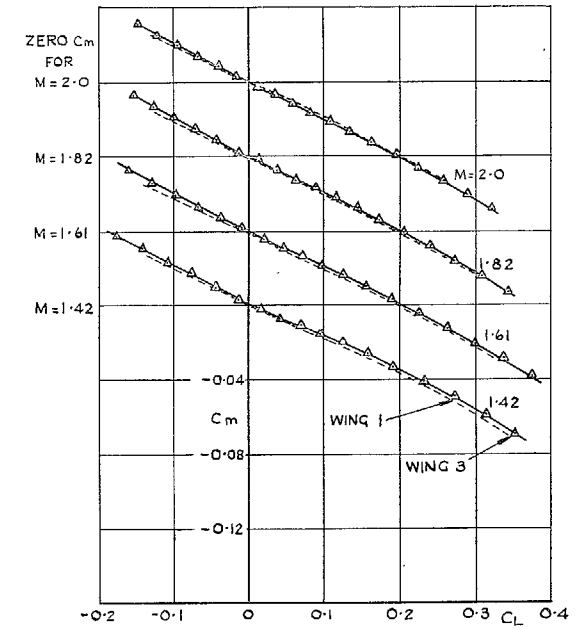
FIG. 6. Variation of C_m with C_L : wings 1 and 3.
