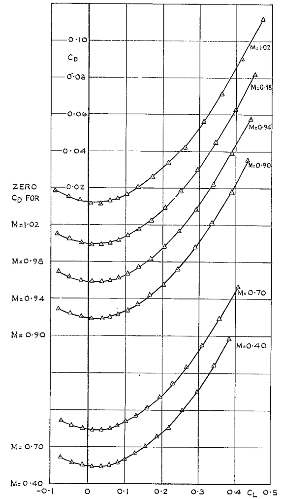
FIG. 20. Variation of C_D with C_L : wing 3.
