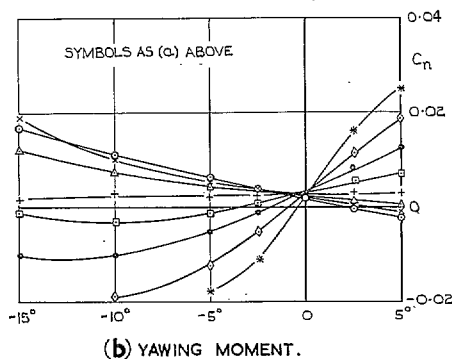
FIGS. 40a and 40b. Typical variation of rolling moment (a) and yawing moment (b) with sideslip. Wing C. A = 1 ; t_0/c_0 = 0.12 .
