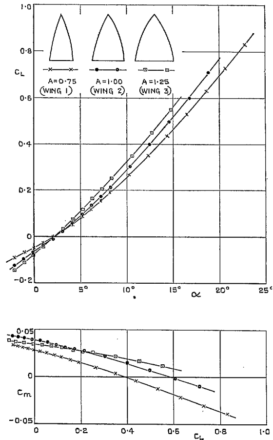
FIG. 43. Effect of aspect ratio on lift and pitching-moment characteristics of flat-plate gothic wings.
