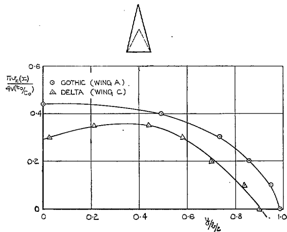
(a) GOTHIC AND DELTA WINGS WITH DIAMOND CROSS-SECTIONS
