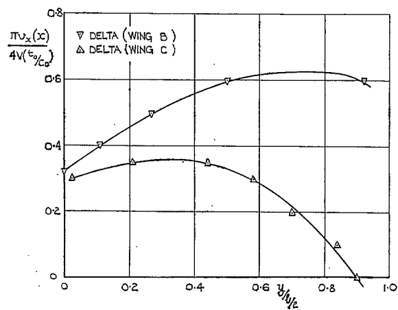
(b) DELTA WINGS
