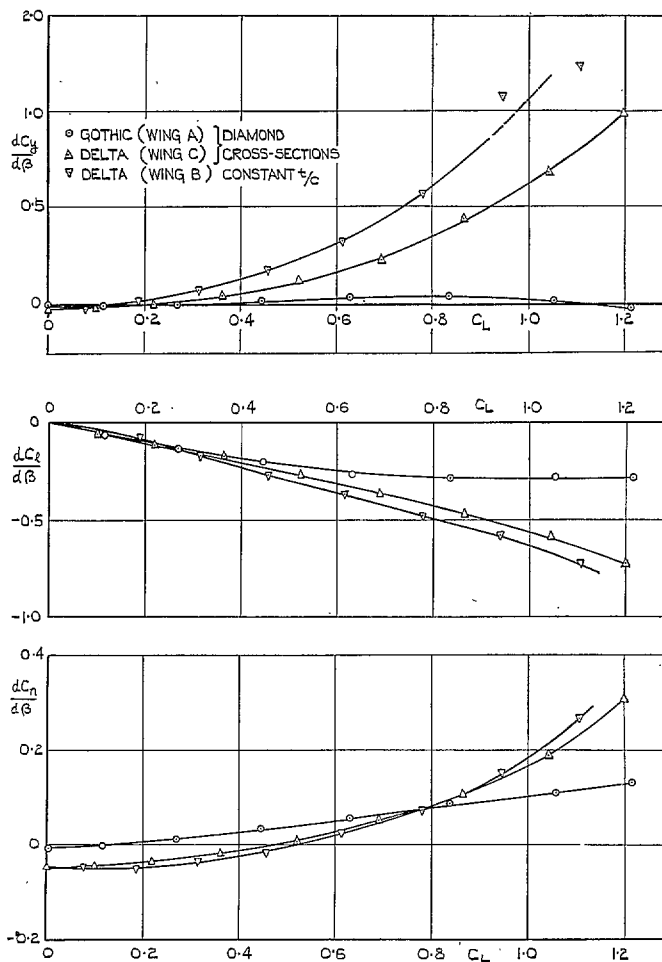
FIG. 41. Static sideslip derivatives for thick wings of aspect ratio 1. Wings A, B and C. t_0/c_0 = 0.12 .
