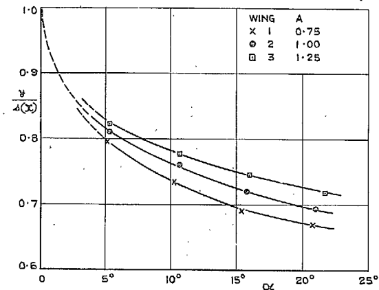
FIG. 14. Spanwise position of points of inflexion on flat-plate gothic wings.
