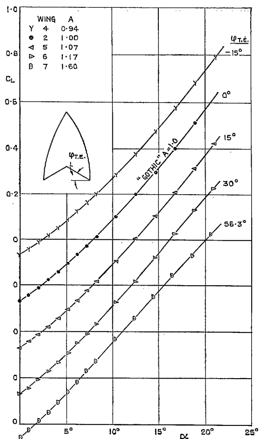
FIG. 47. Effect of trailing-edge sweep on lift of wing with 'A = 1 gothic' leading-edge shape (Flat-plate models).
