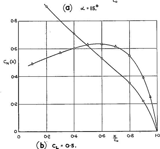
FIGS. 69a and 69b. Comparison of longitudinal distribution of local cross-load coefficient on gothic and delta wings. A = 1.0 .
