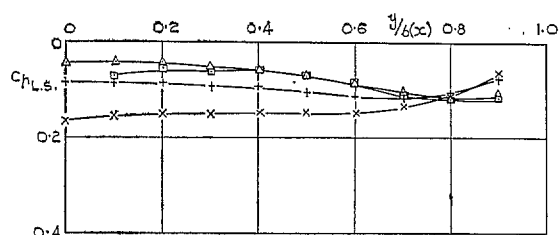
FIG. 59. Wing C. Upper and lower surface pressure coefficients along lines of constant x/c_0 . \alpha = 15.33 deg.
