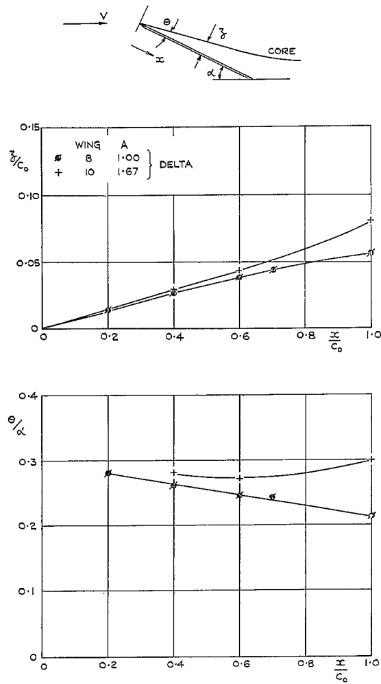
FIG. 20. Side elevation of vortex-core path on flat-plate delta wings of various aspect ratios. \alpha \approx 15 deg.
