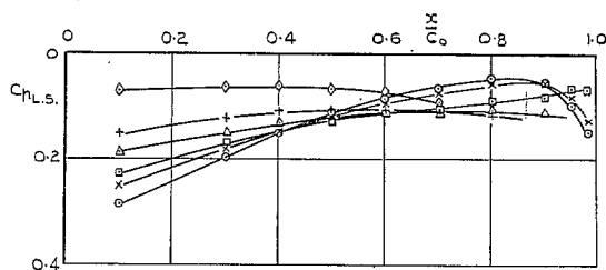
FIG. 58. Wing C. Upper and lower surface pressure coefficients on rays from apex. \alpha = 15.33 deg.
