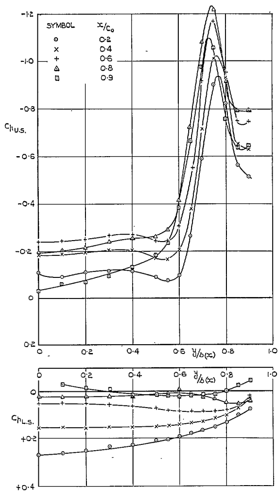
FIG. 57. Wing B. Upper and lower surface pressure coefficients along lines of constant x/c_0 . \alpha = 15.29 deg.
