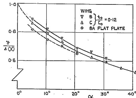
FIG. 12. Effect of thickness on spanwise position of suction peaks on delta wings of aspect ratio 1.
