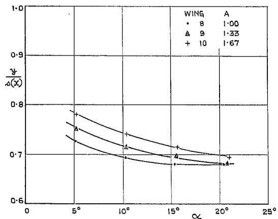
FIG. 16. Spanwise position of points of inflexion on flat-plate delta wings.
