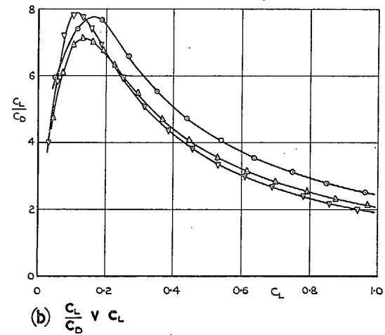
FIGS. 35a and 35b. Lift/drag ratio of wings A, B and C. A = 1 ; t_0/c_0 = 0.12 .
