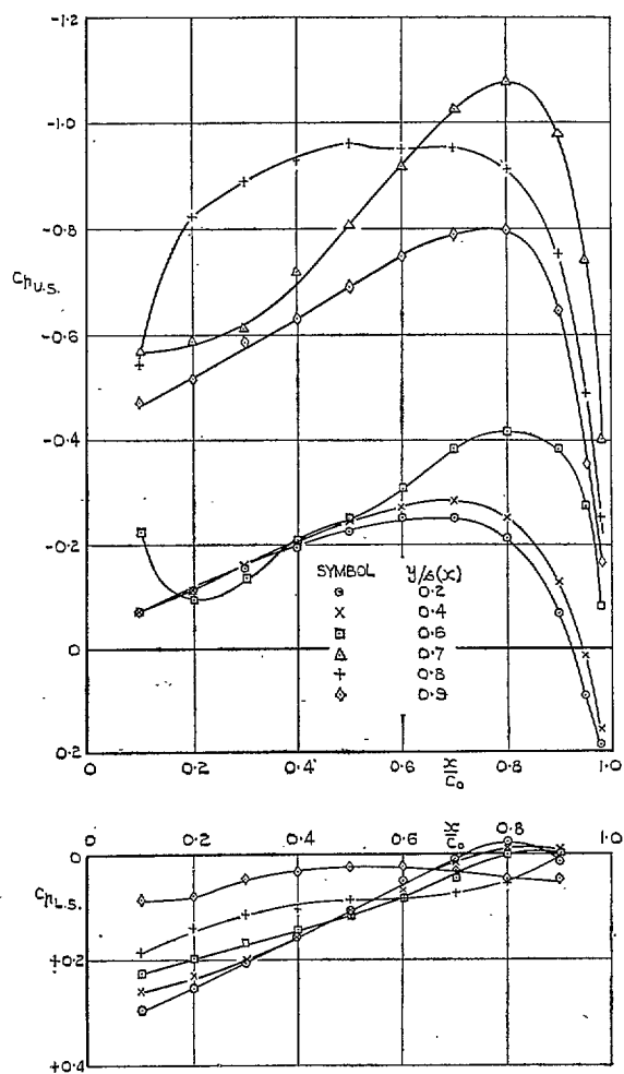
FIG. 56. Wing B. Upper and lower surface pressure coefficients on rays from apex. \alpha = 15.29 deg.
