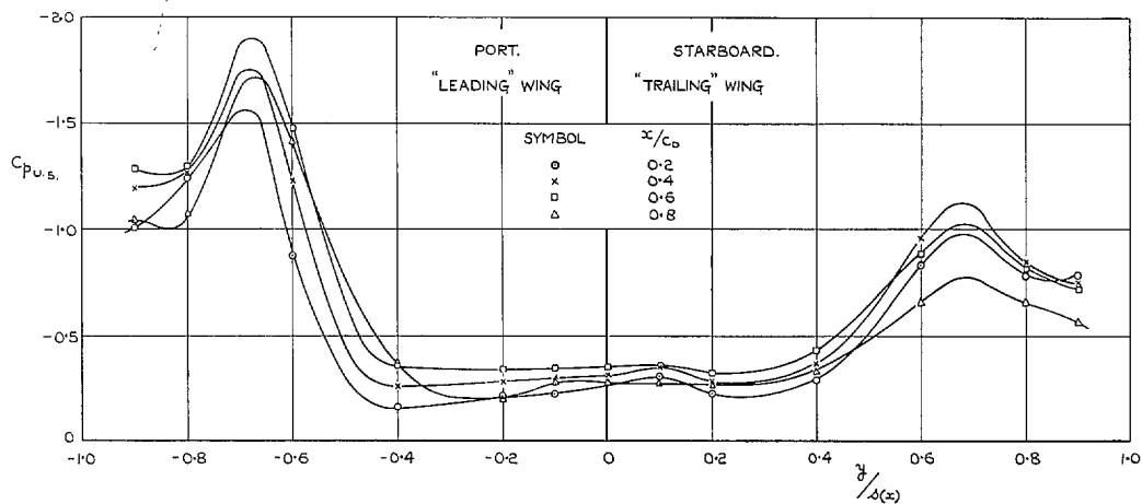
FIG. 25. Typical upper-surface pressure distribution on yawed wing (Wing C). \alpha = 20.48 \text{ deg}; \psi = 5 \text{ deg}.
