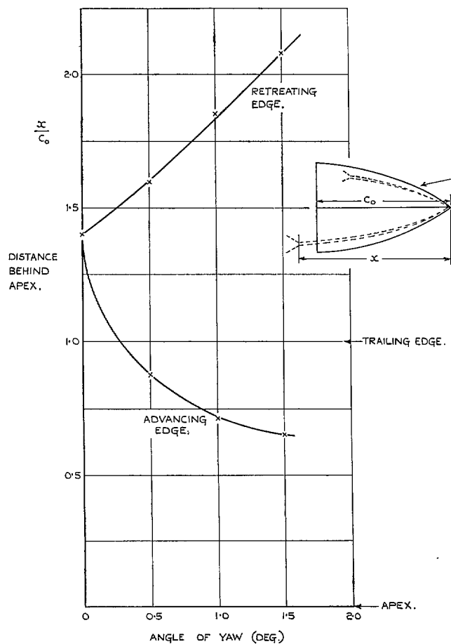
FIG. 26. Wing A. \alpha = 23 \text{ deg}. Position of breakdown of vortex core.
