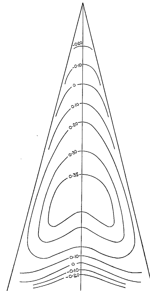
FIG. 52. Wing C. Isobar pattern at zero incidence. Values plotted: \{\pi v_x(x)\}/\{4V(t_0/c_0)\} .
