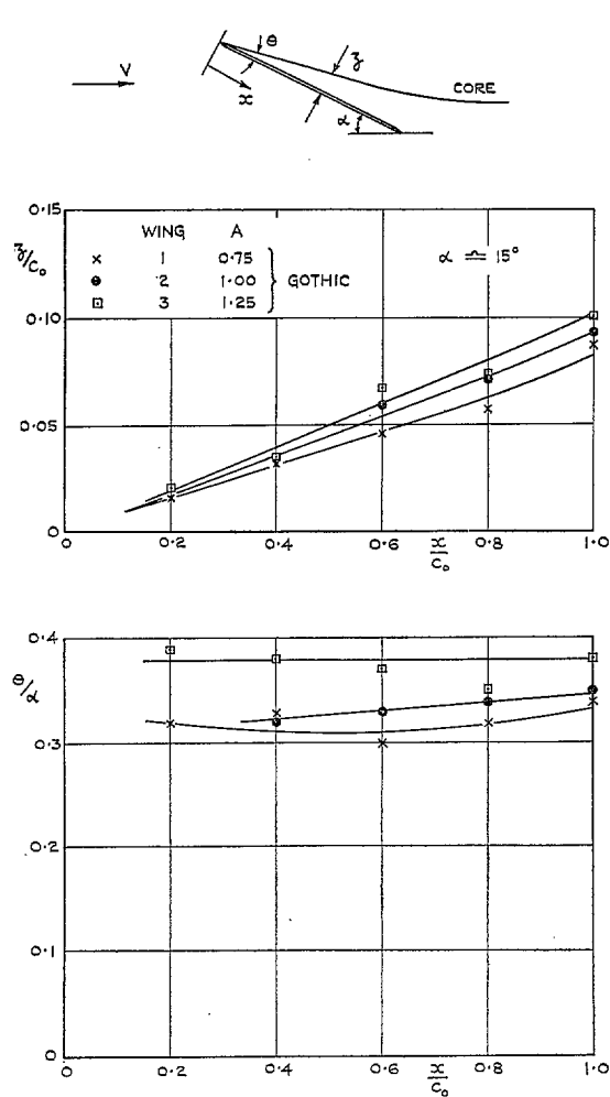
FIG. 19. Side elevation of vortex-core path on flat-plate gothic wings of various aspect ratios. \alpha \approx 15 deg.
