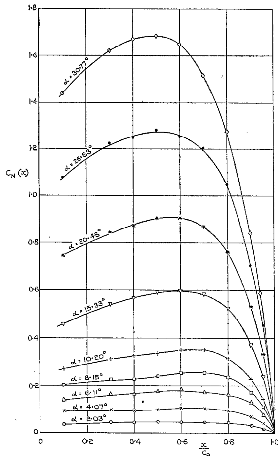
FIG. 68. Wing C. Longitudinal distribution of local cross-load coefficient.
