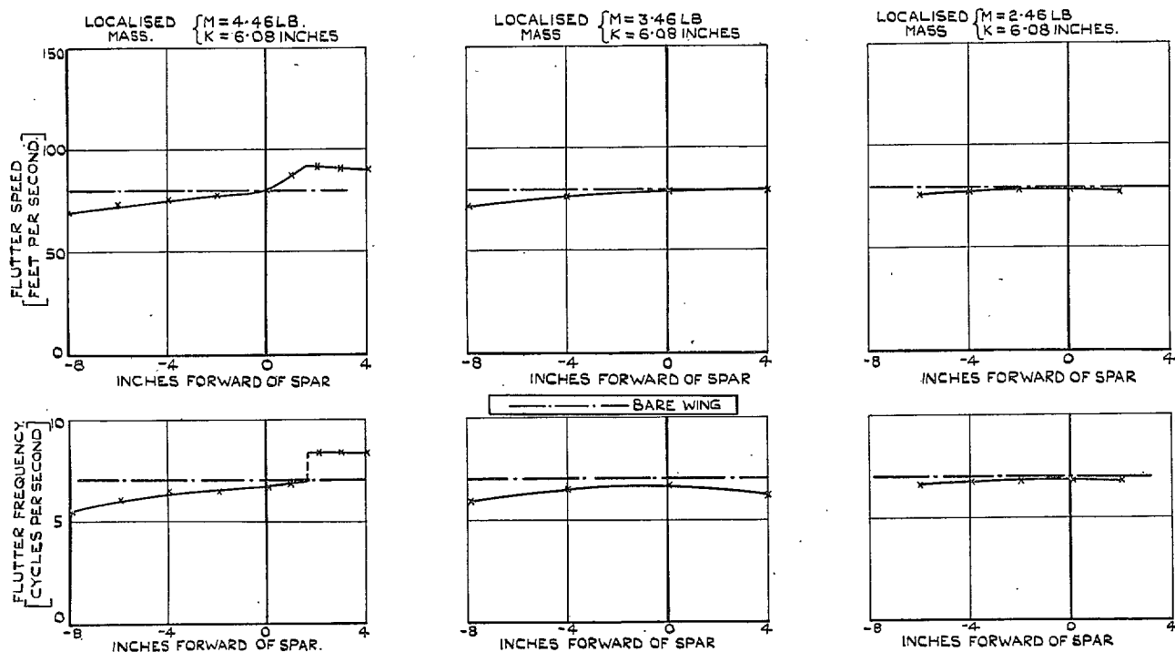
FIG. 17. The effect of chordwise position of a localised mass at 0.25 span (13-deg sweepback).
