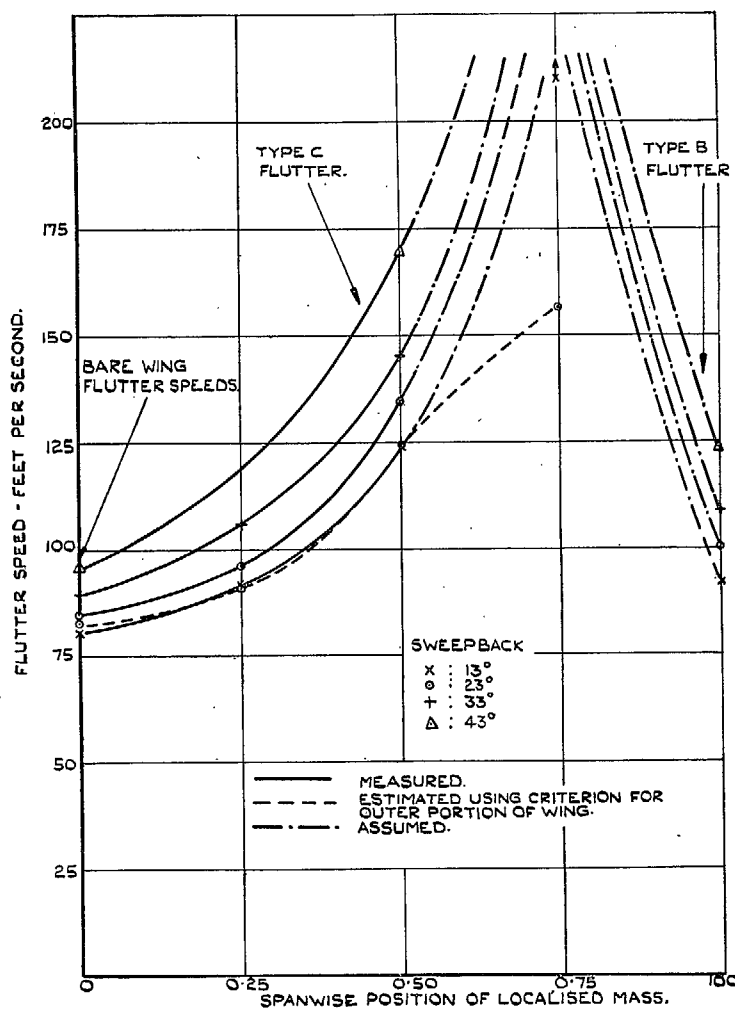
FIG. 30. The overtone flutter speeds.
