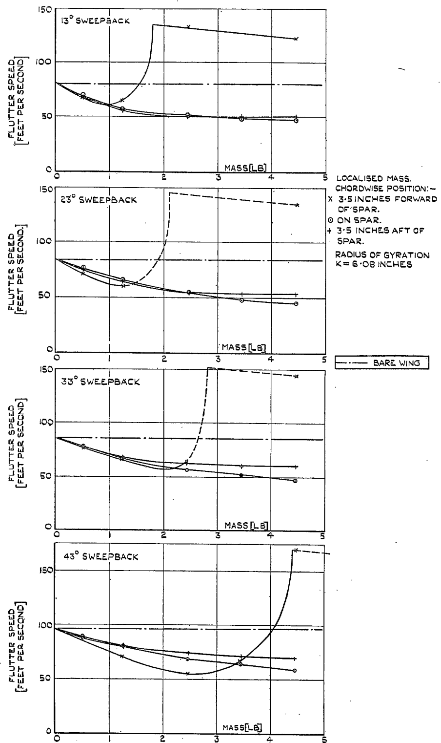
FIG. 22. The variation of flutter speed with mass at 0.5 span (Constant radius of gyration).
