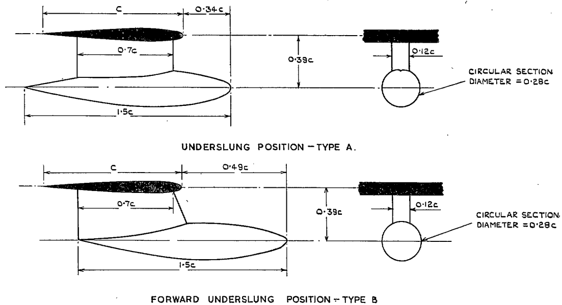
FIG. 3. Aerodynamic shapes at half-span section.
