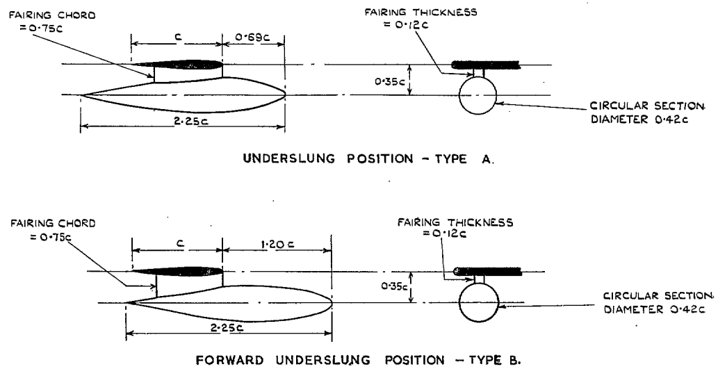
FIG. 4. Aerodynamic shapes at tip section.
