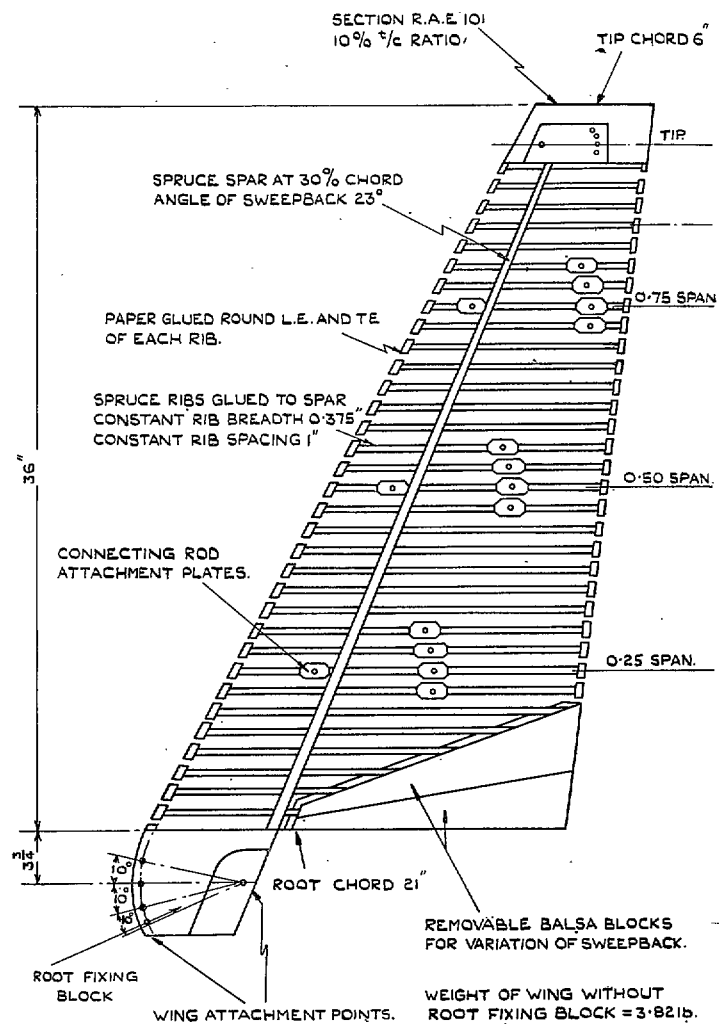
FIG. 2. Model-wing details.
