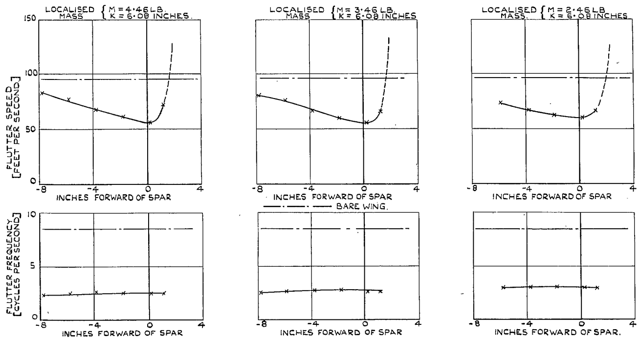
FIG. 12. The effect of chordwise position of a localized mass at 0.75 span (43-deg sweepback).
