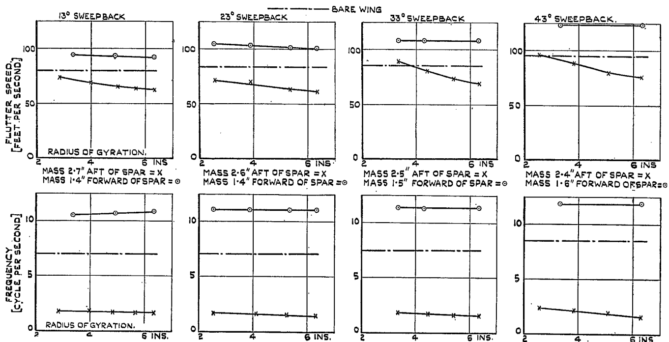
FIG. 24. The effect of radius of gyration of a mass 4.46 lb at the tip.
