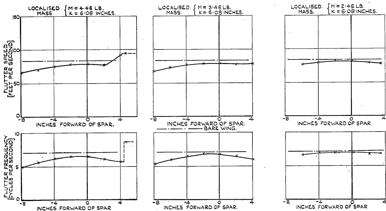
FIG. 18. The effect of chordwise position of a localised mass at 0.25 span (23-deg sweepback).
