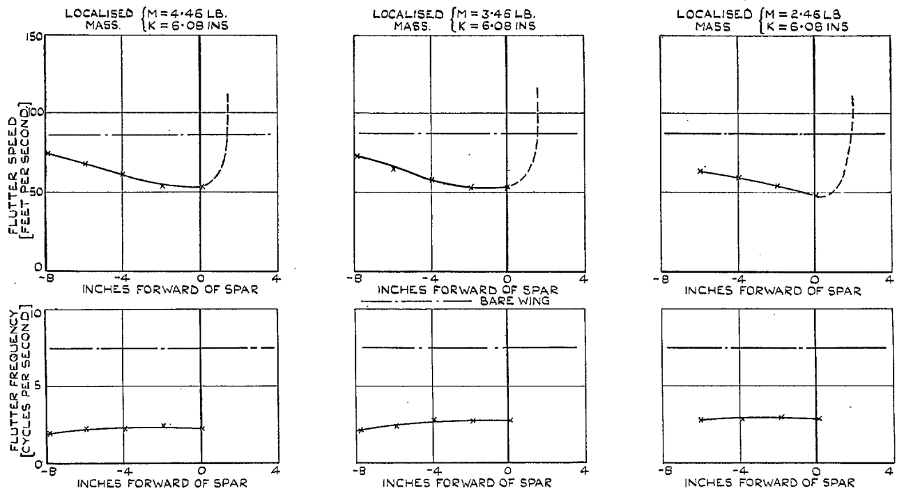
FIG. 11. The effect of chordwise position of a localized mass at 0.75 span (33-deg sweepback).
