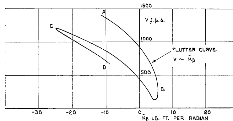
FIG. 2. Stick-free flutter of a hypothetical elevator system.
