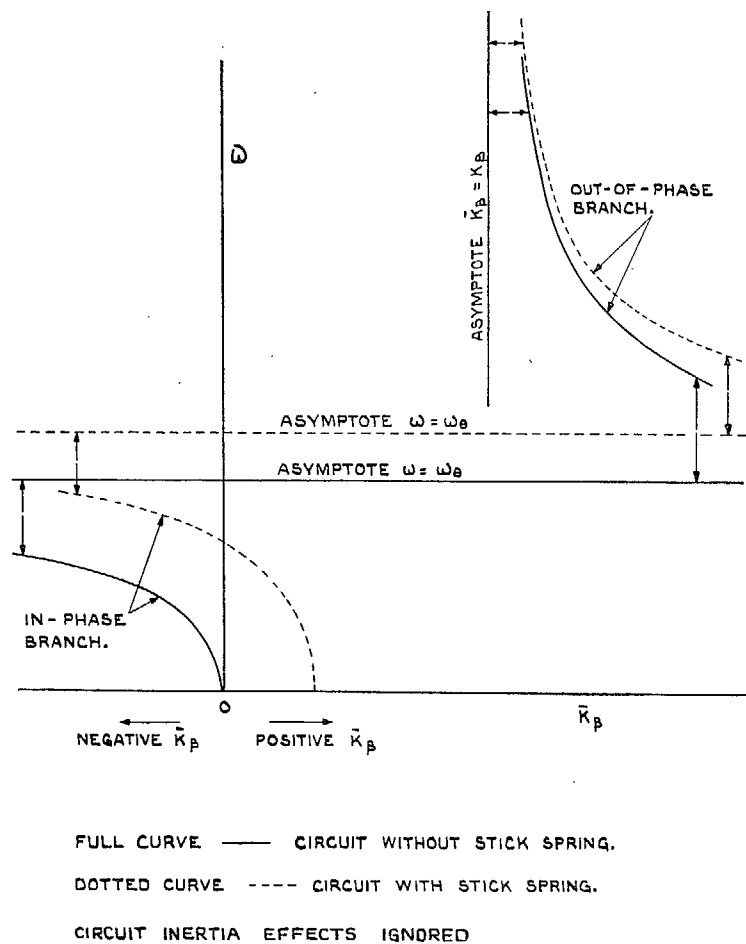
FIG. 1. Circuit curves for system with and without stick spring.
