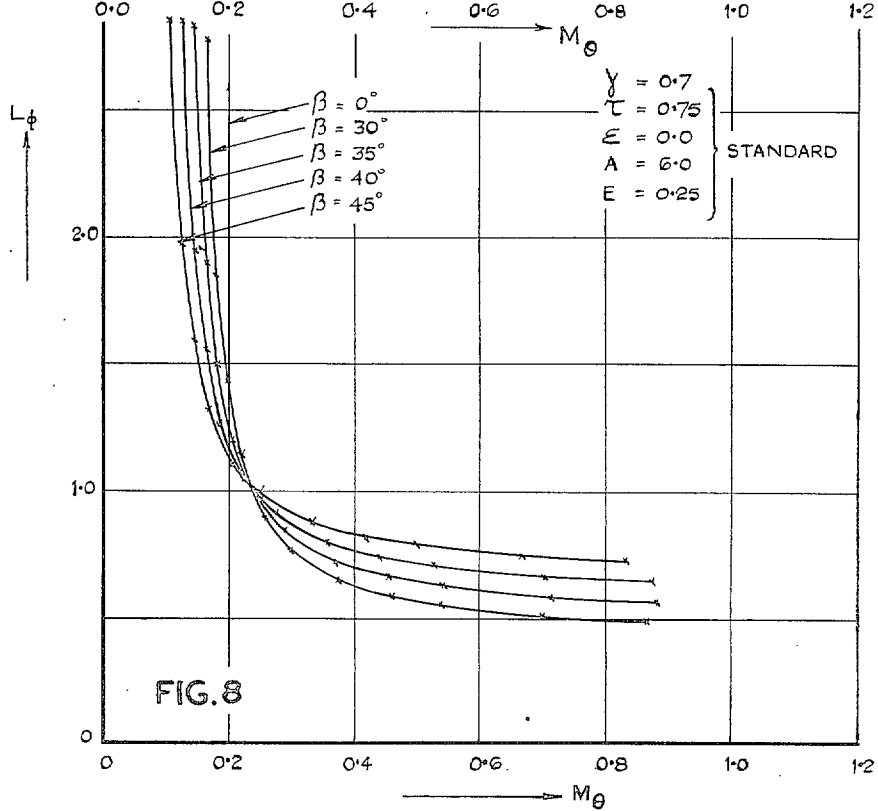
FIGS. 7 and 8. Variation of aileron reversal speed with wing stiffness. Effect of aileron span.
