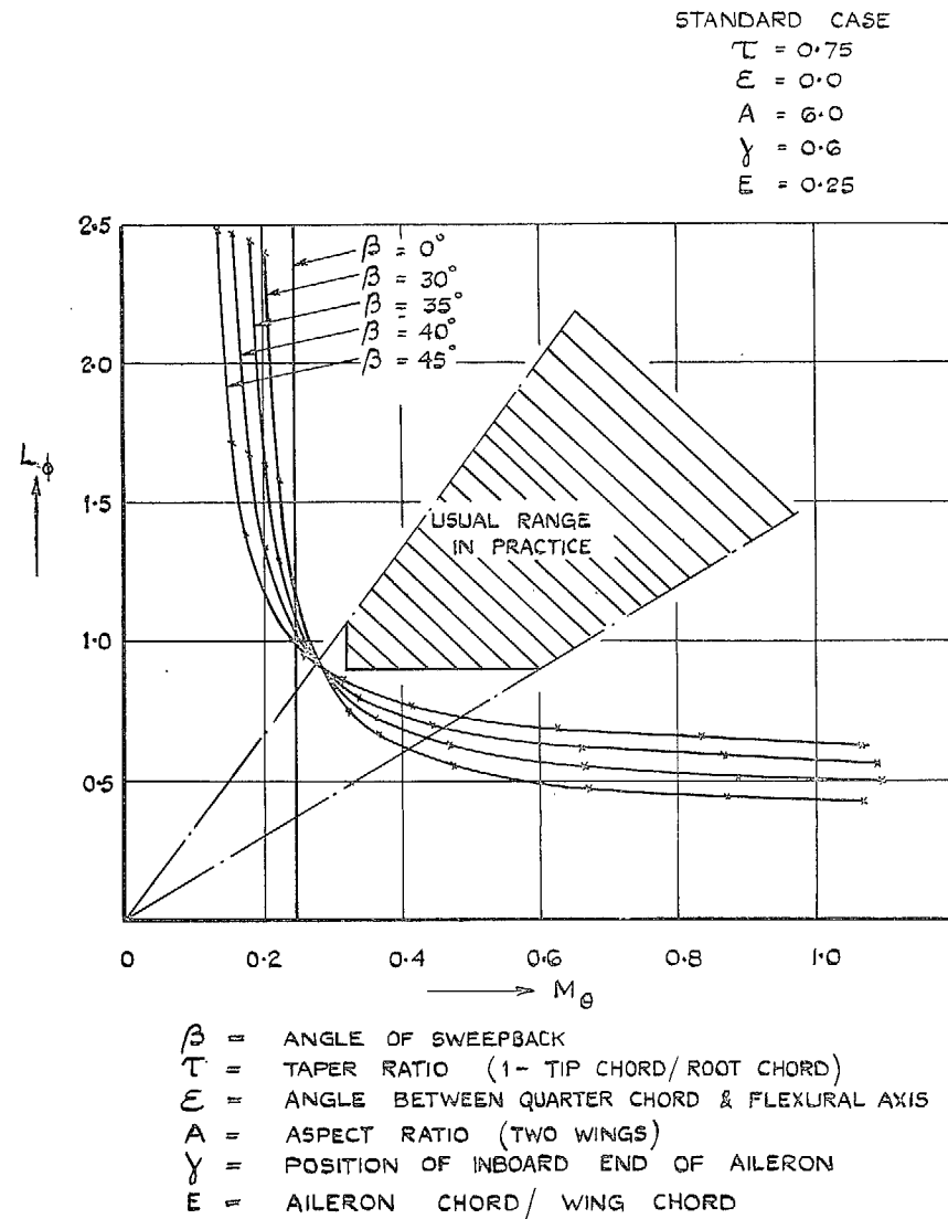
FIG. 2. Variation of aileron reversal speed with wing stiffness. Standard wing.
