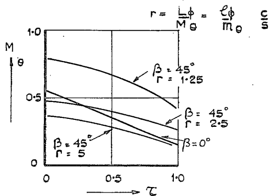
A. VARIATION WITH TAPER ( \tau = 1 - \text{TIP CHORD / ROOT CHORD} )
