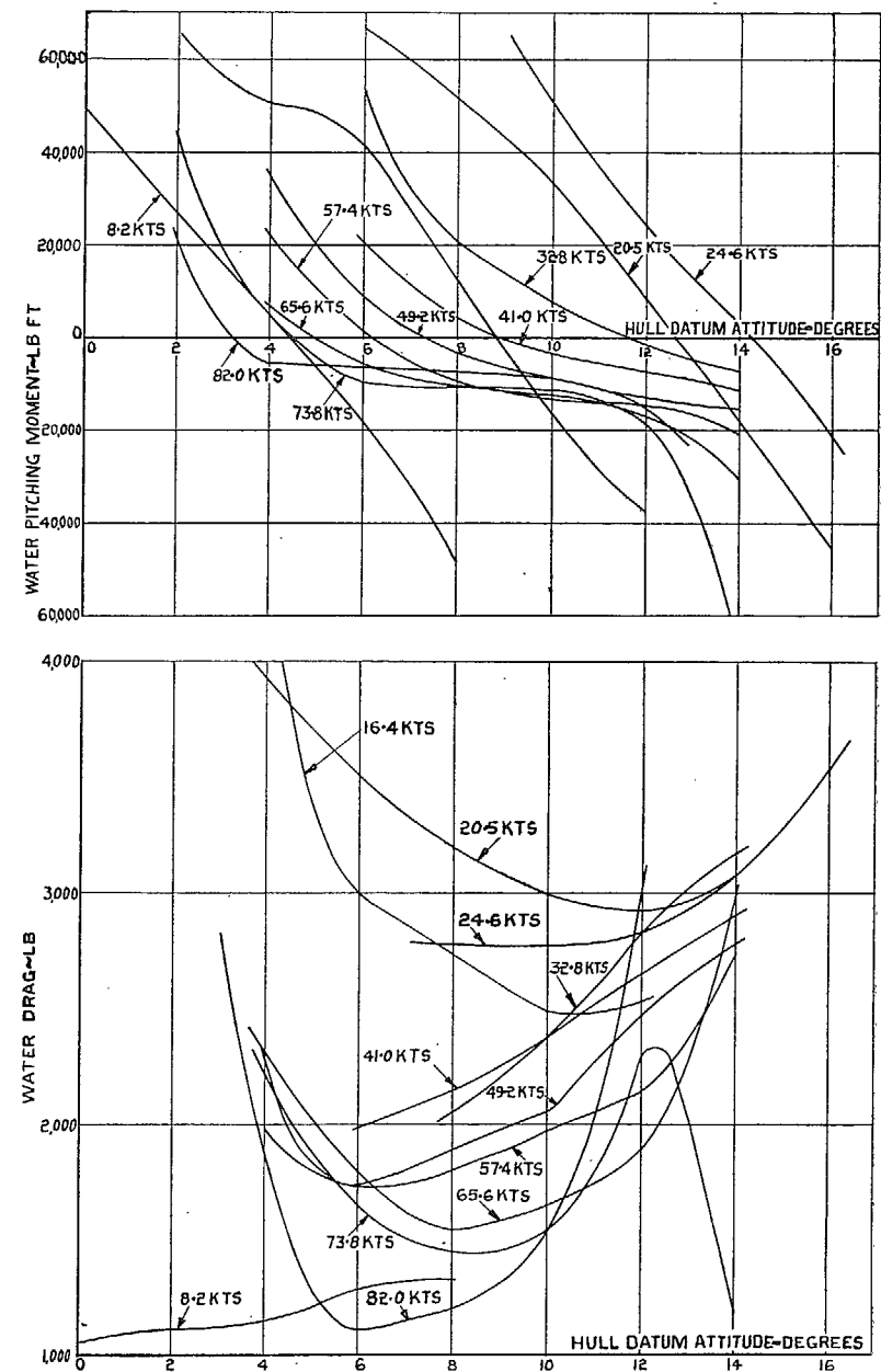
FIG. 17. Take-off at normal load 15,200 lb, flaps 33 deg. Resistance and pitching-moment tests. Final lines.
