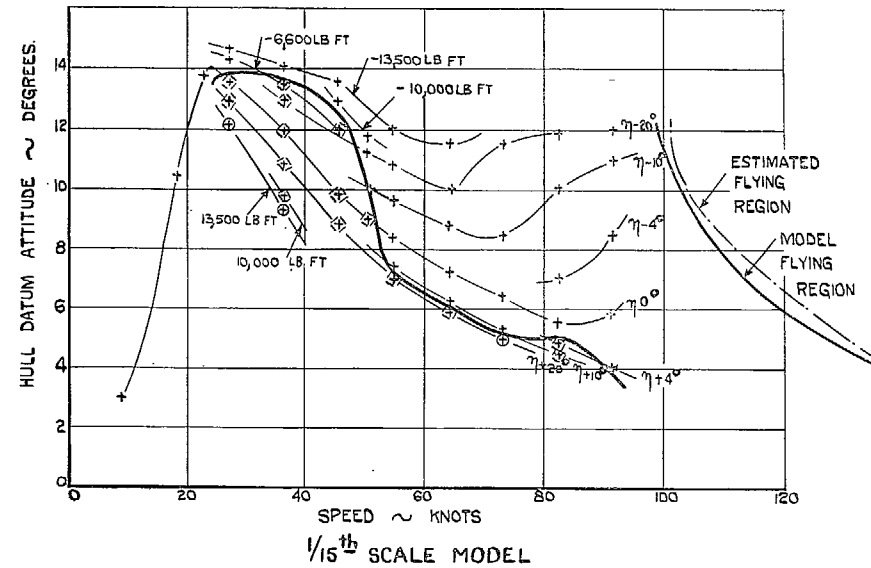
FIG. 10. Take-off at overload 17,250 lb, flaps up. Stability tests. Final lines.
