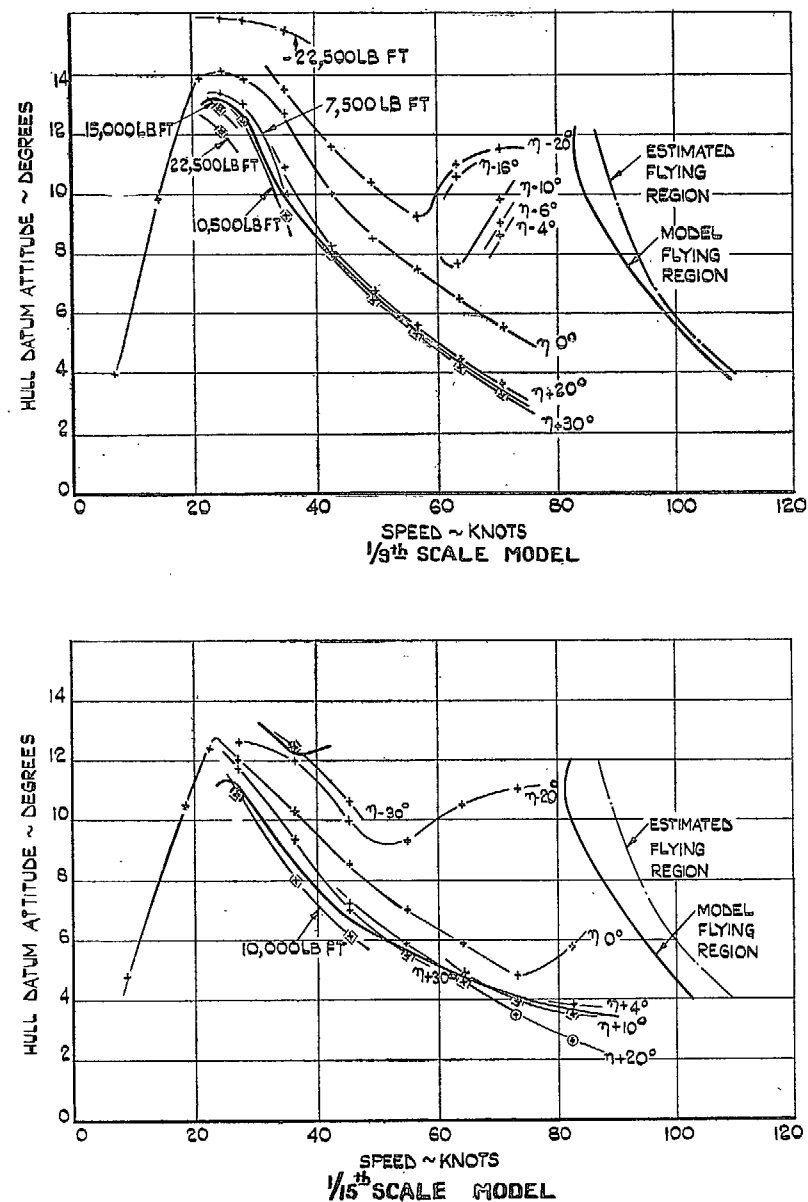
FIG. 7. Take-off at normal load 15,200 lb, flaps 33 deg. Stability tests. Final lines.
