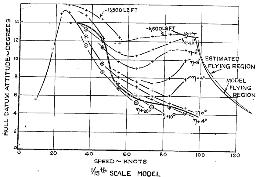
FIG. 12. Landing case at 15,200 lb, flaps up. Stability tests. Final lines.
