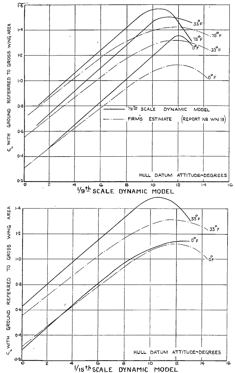
FIG. 5. Model lifts. Wing leading edge slats fitted.
