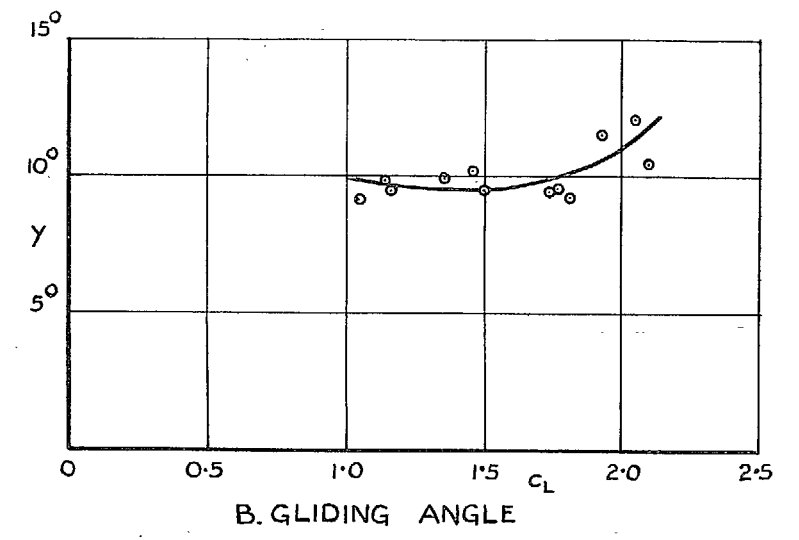
FIG. 12. Youngman Flaps Extended under Body—Set for Landing.
