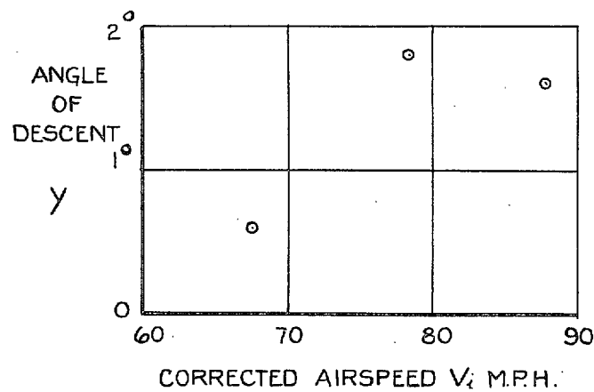
FIG. 14. Youngman Flaps Extended under Body—Set for Landing.—Rumble Approach at about \frac{1}{8} Throttle (2,300 r.p.m.— 2\frac{1}{4} lb/sq in boost pressure).
