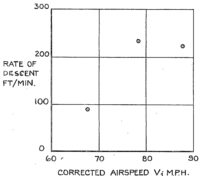
FIG. 14. Youngman Flaps Extended under Body—Set for Landing.—Rumble Approach at about \frac{1}{8} Throttle (2,300 r.p.m.— 2\frac{1}{4} lb/sq in boost pressure).
