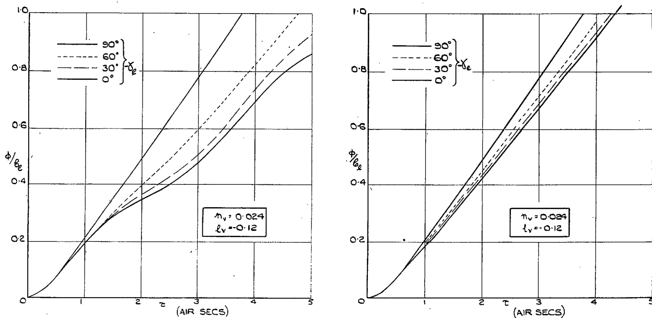
FIG. 11. Response in Angle of Bank to Applied Rolling Moment for Varying Angle of Dive.
