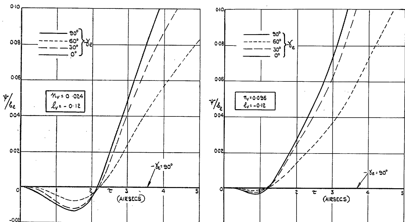
FIG. 12. Response in Angle of Yaw to Applied Rolling Moment with Varying Angle of Dive.
