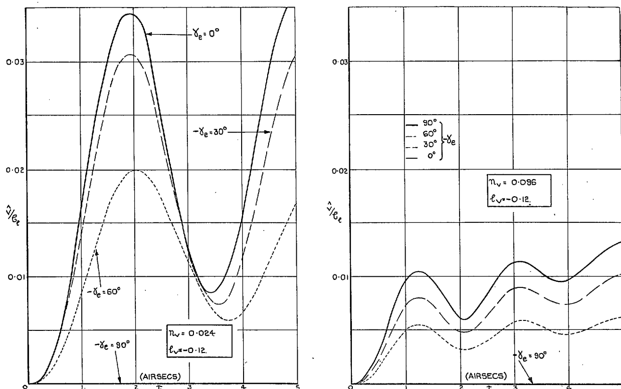
FIG. 9. Response in Angle of Sideslip to Applied Rolling Moment with Varying Angle of Dive.
