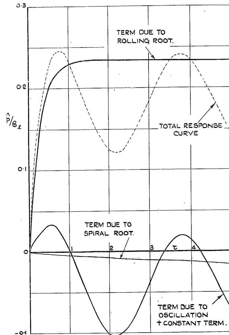
FIG. 2. Response in Rate of Roll to an Applied Rolling Moment Showing the Contributions of the Three Modes of Motion when l = -0.12, \eta_v = 0.024 .
